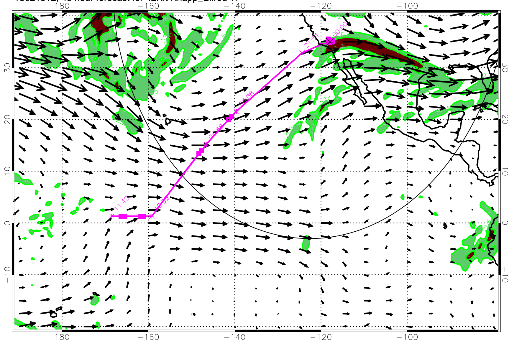
13021512, 48 hour forecast for 42Kft Knapp_Ellrod TI
