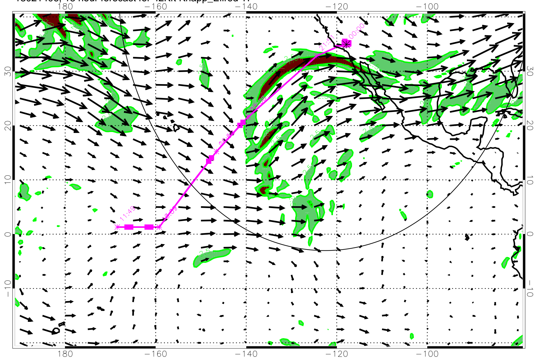
13021406, 18 hour forecast for 42Kft Knapp_Ellrod TI
