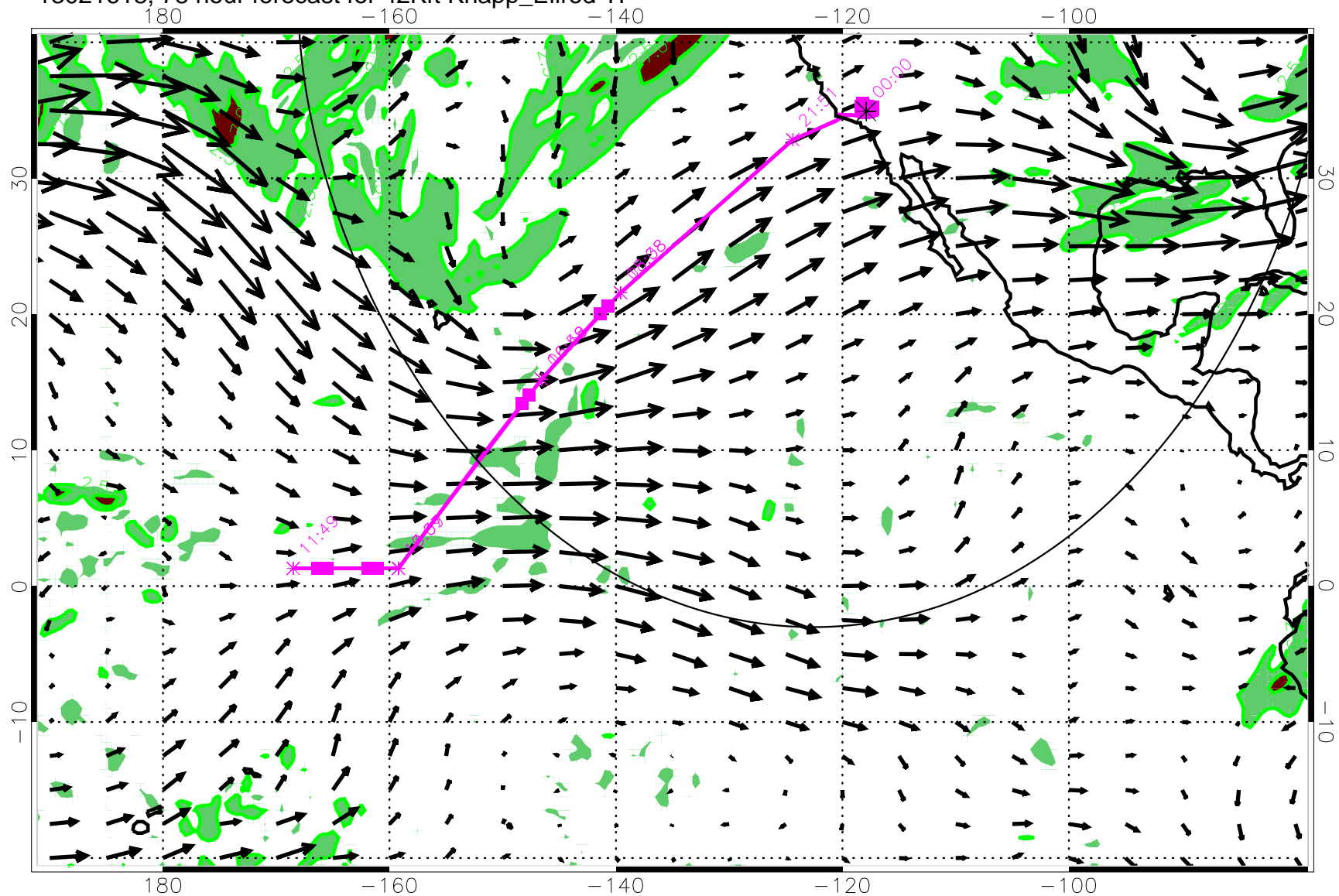
13021618, 78 hour forecast for 42Kft Knapp_Ellrod TI
