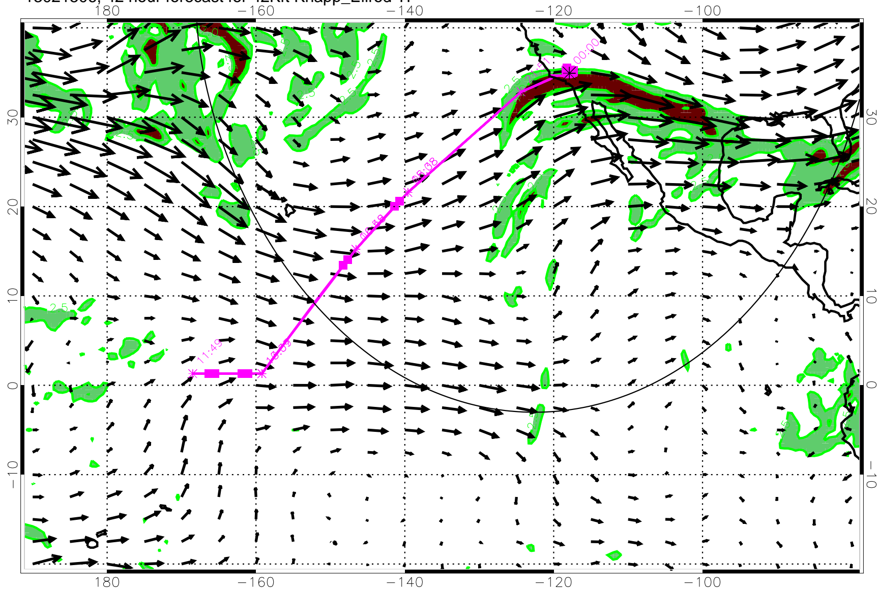
13021506, 42 hour forecast for 42Kft Knapp_Ellrod TI
