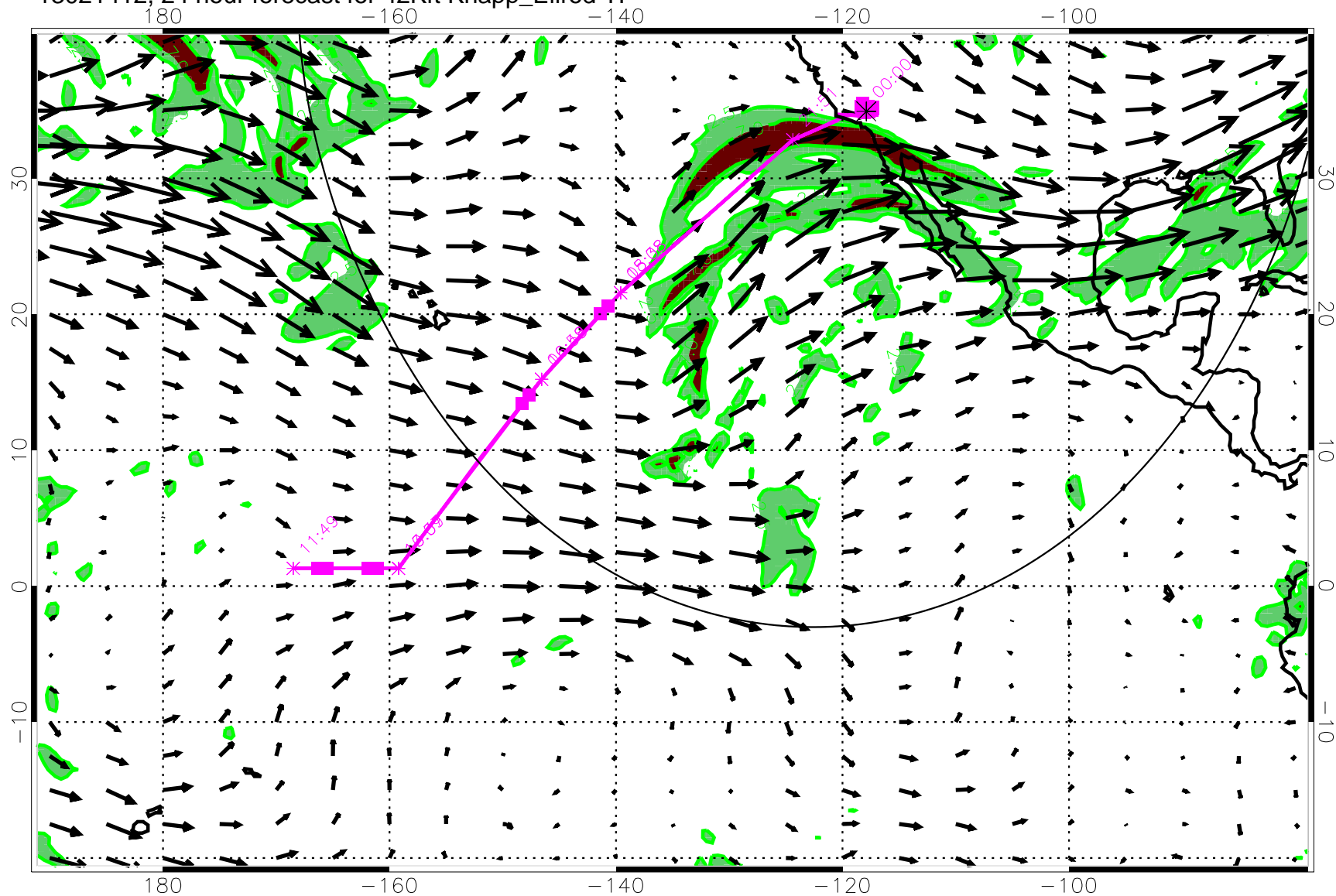
13021412, 24 hour forecast for 42Kft Knapp_Ellrod TI
