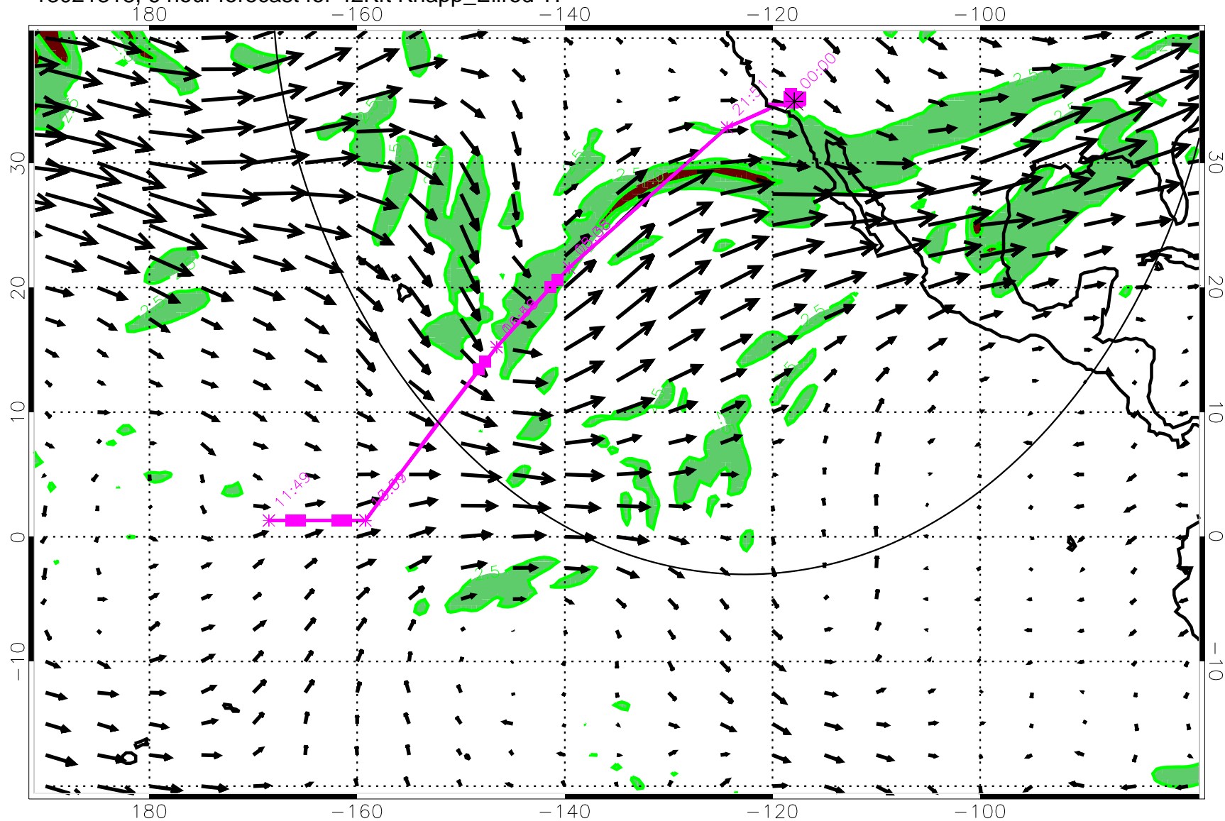
13021318, 6 hour forecast for 42Kft Knapp_Ellrod TI
