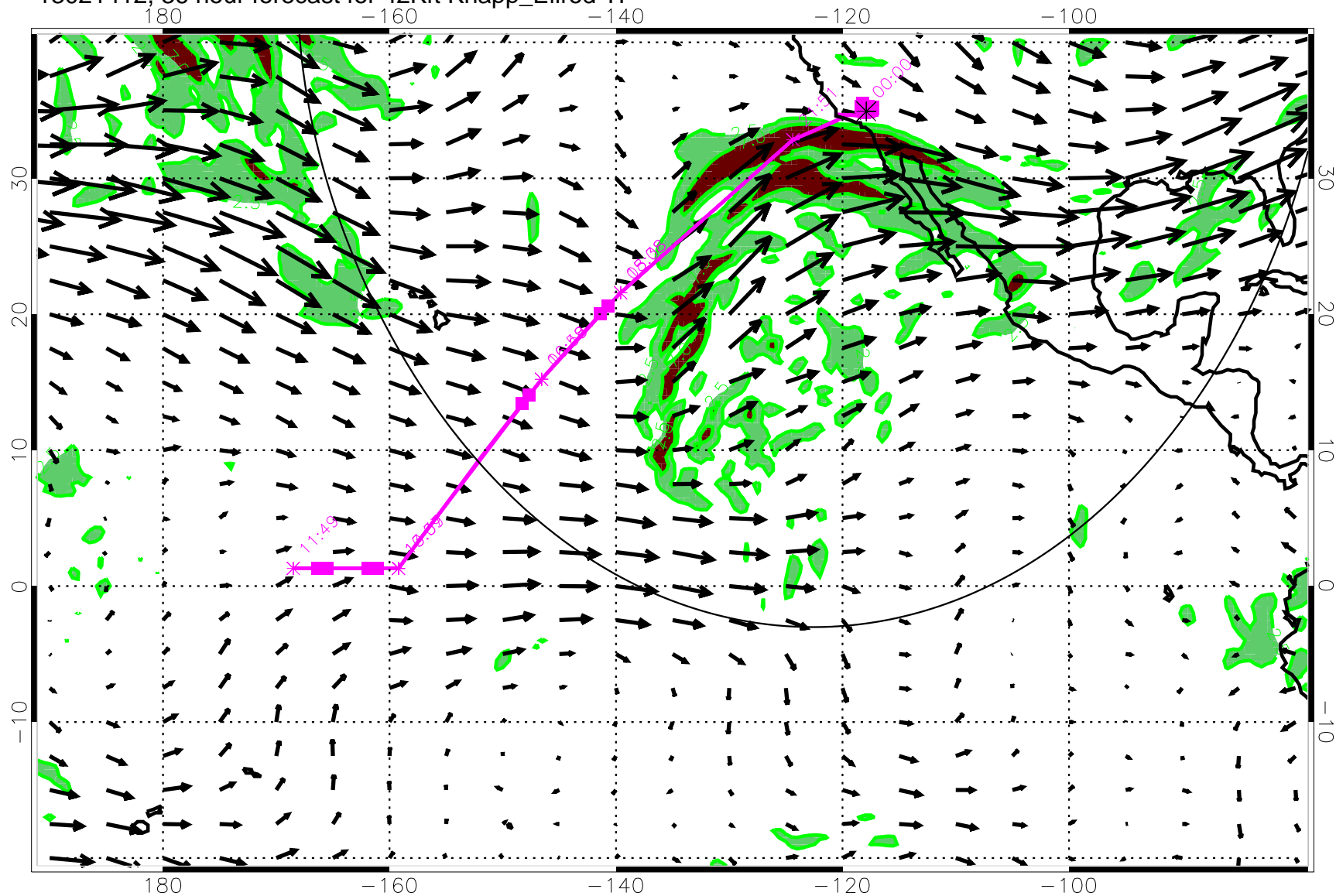
13021412, 36 hour forecast for 42Kft Knapp_Ellrod TI
