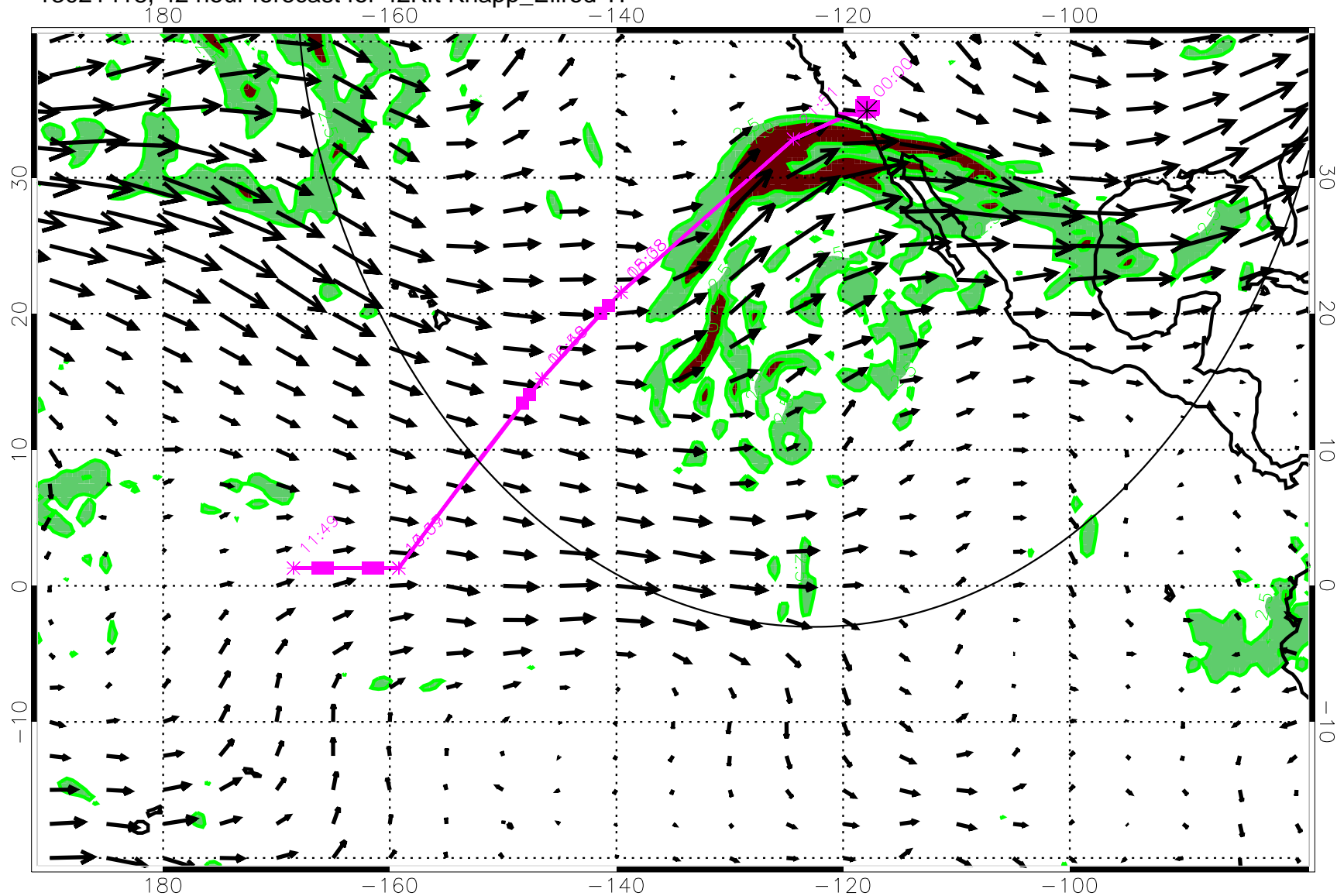
13021418, 42 hour forecast for 42Kft Knapp_Ellrod TI
