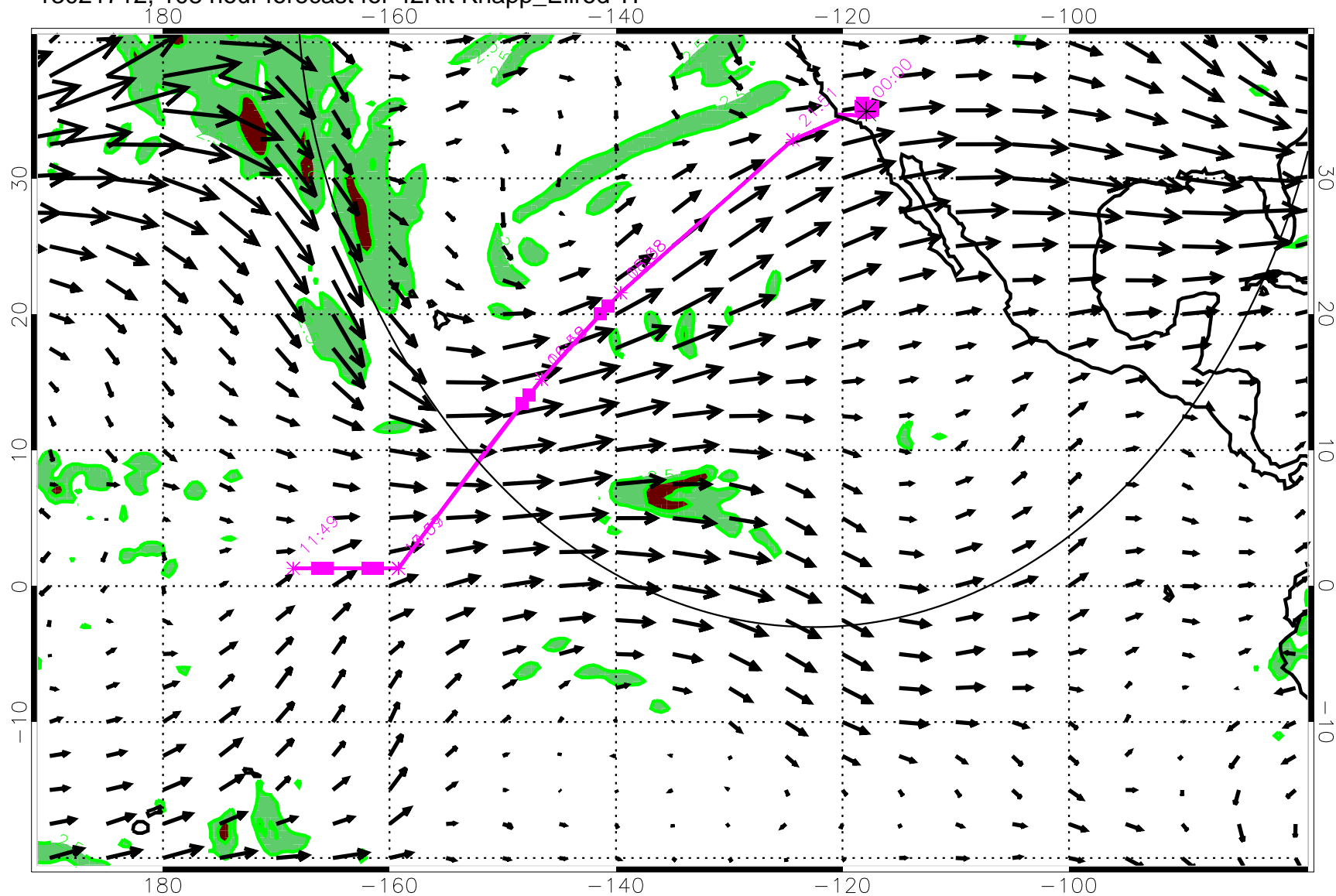
13021712, 108 hour forecast for 42Kft Knapp_Ellrod T1
