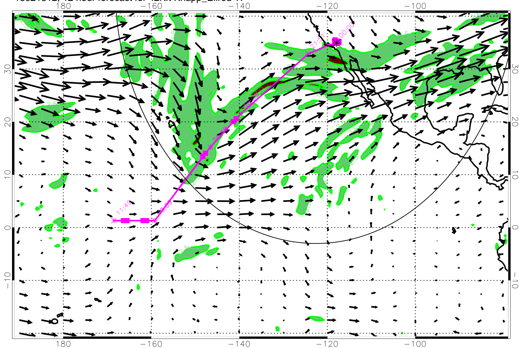
13021312, 12 hour forecast for 42Kft Knapp_Ellrod TI
