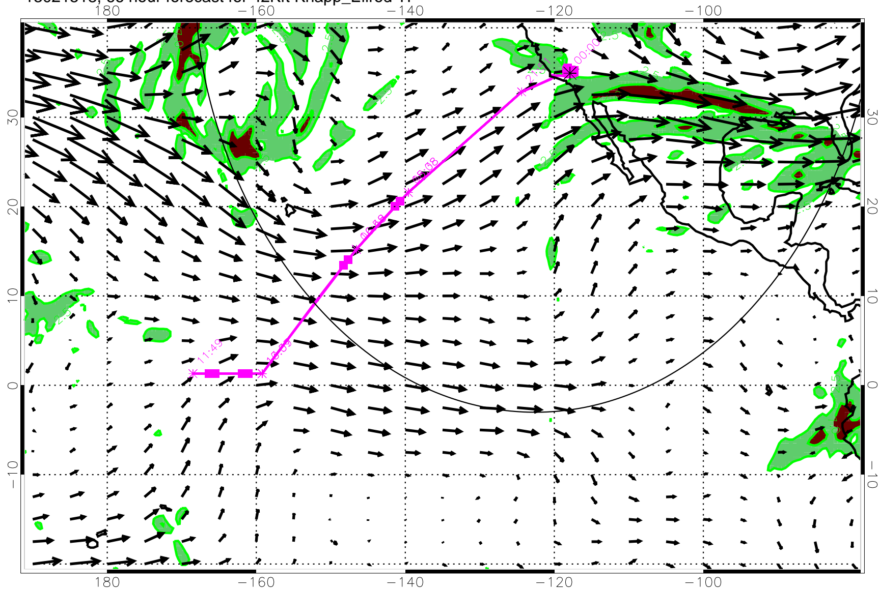
13021518, 66 hour forecast for 42Kft Knapp_Ellrod TI
