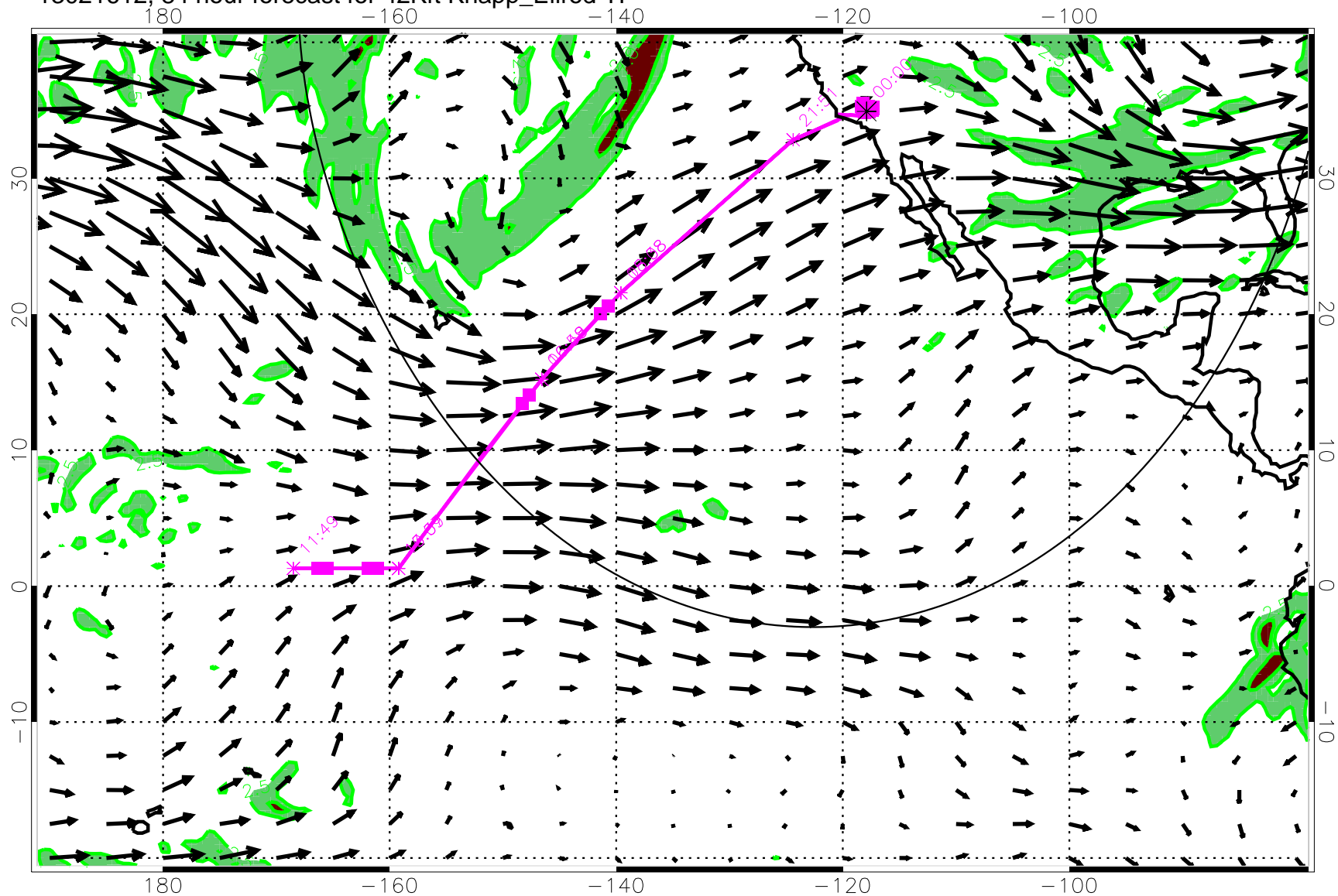
13021612, 84 hour forecast for 42Kft Knapp_Ellrod TI
