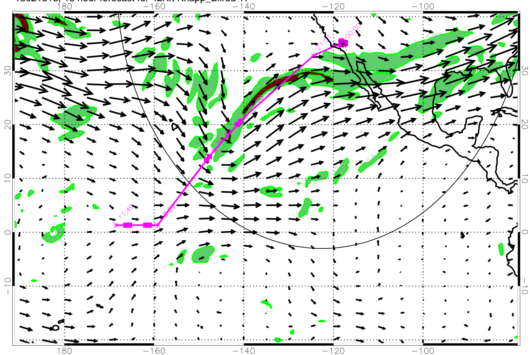
13021318, 18 hour forecast for 42Kft Knapp_Ellrod TI
