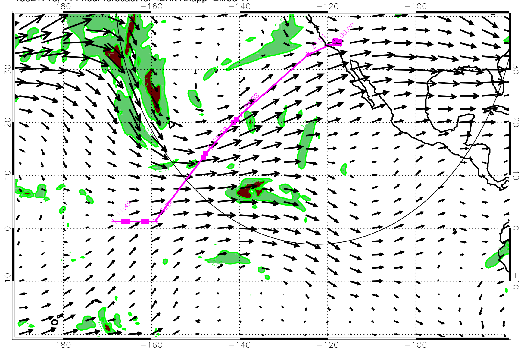
13021718, 114 hour forecast for 42Kft Knapp_Ellrod T1
