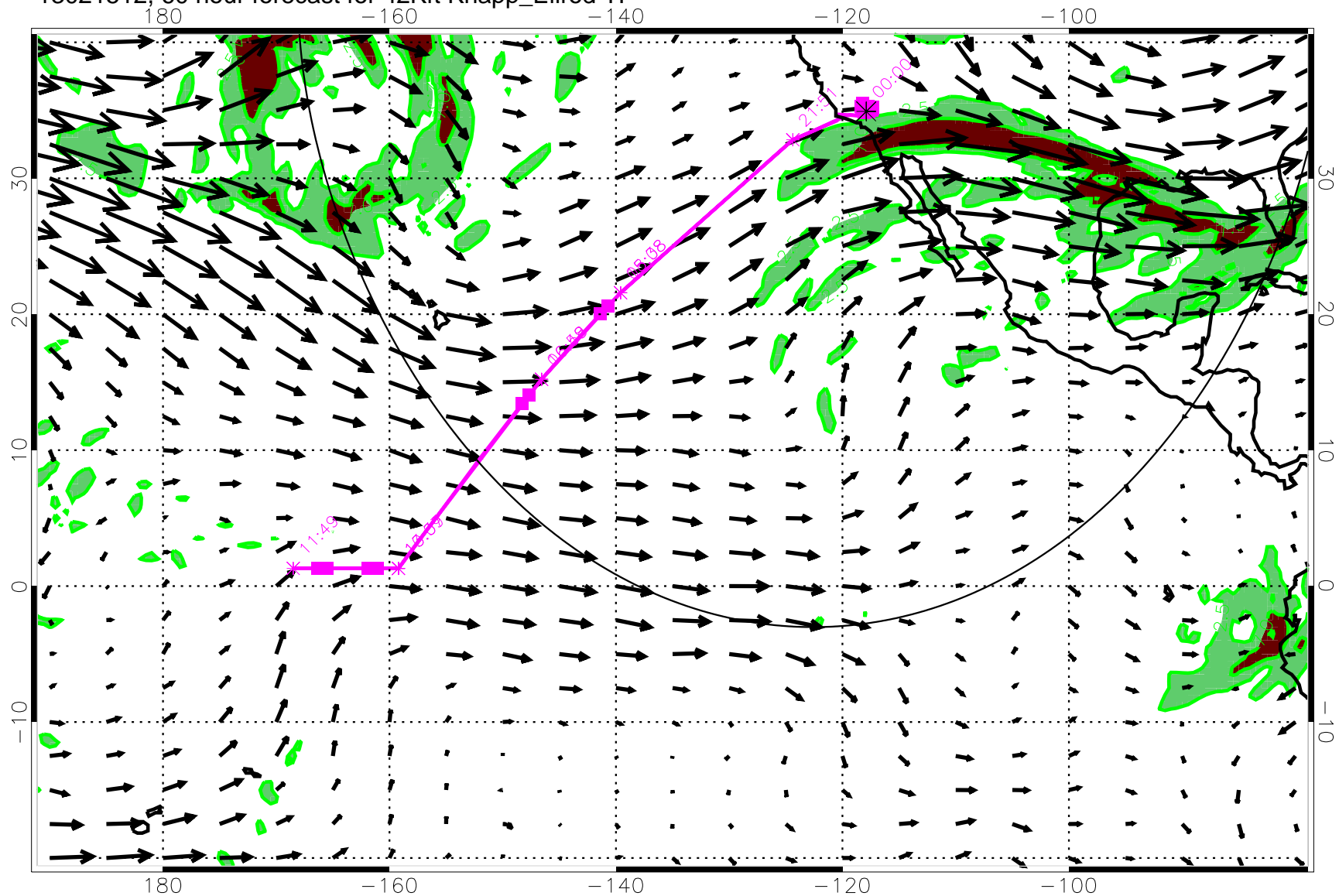
13021512, 60 hour forecast for 42Kft Knapp_Ellrod TI
