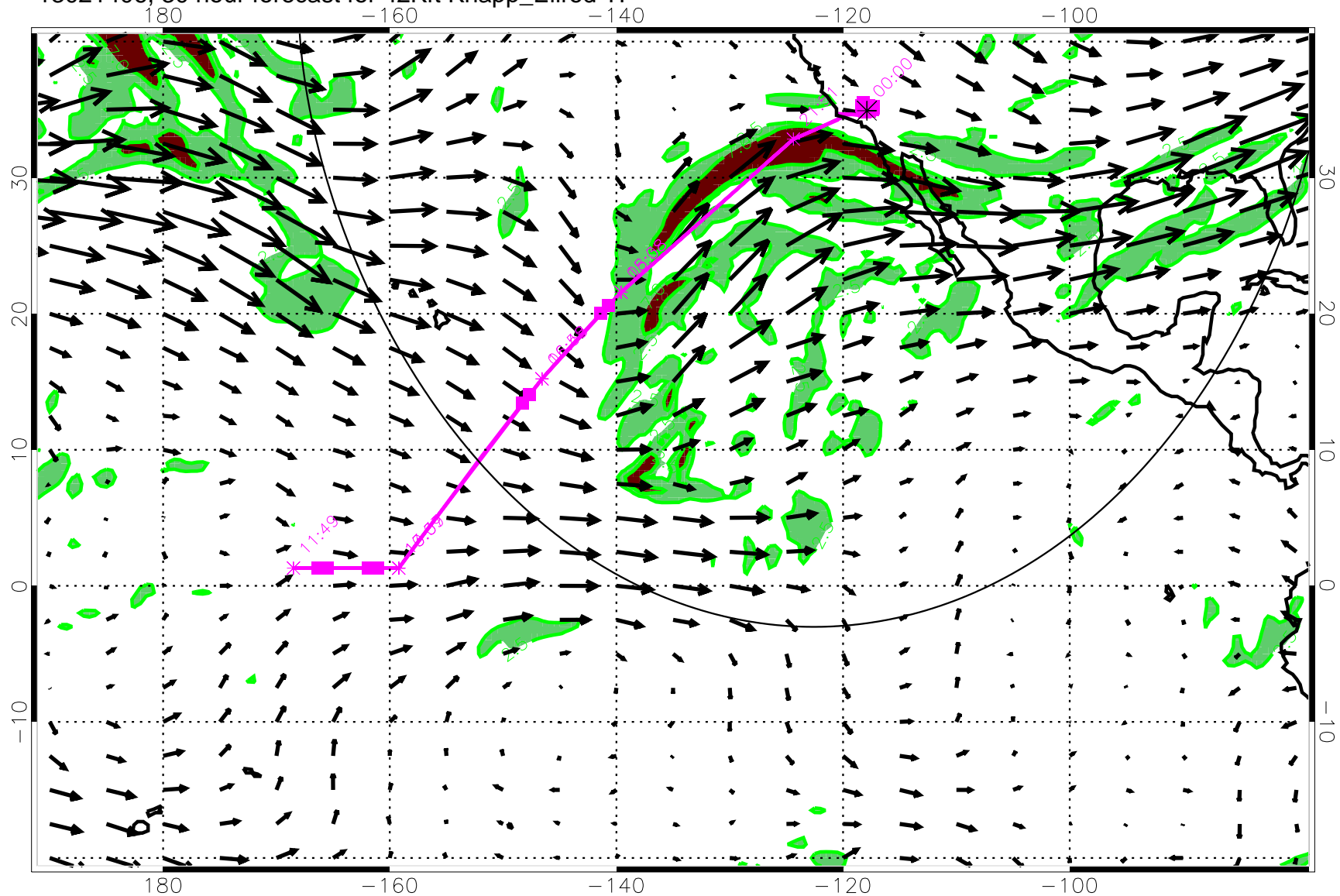
13021406, 30 hour forecast for 42Kft Knapp_Ellrod TI
