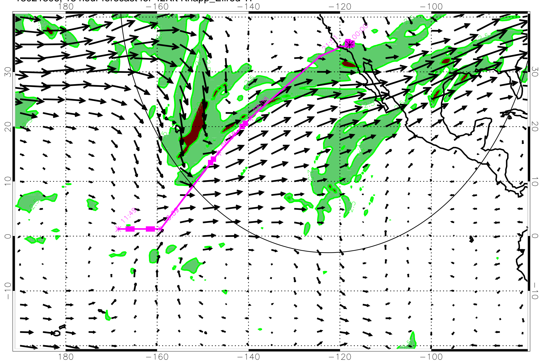
13021306, 18 hour forecast for 42Kft Knapp_Ellrod TI
