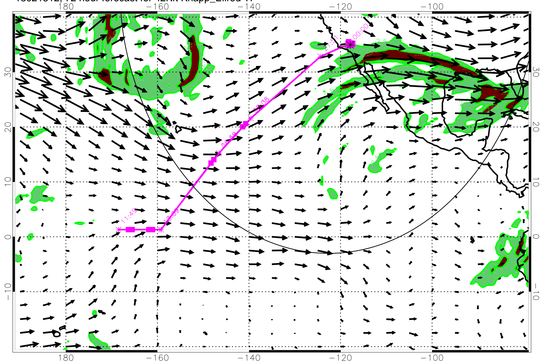
13021512, 72 hour forecast for 42Kft Knapp_Ellrod TI
