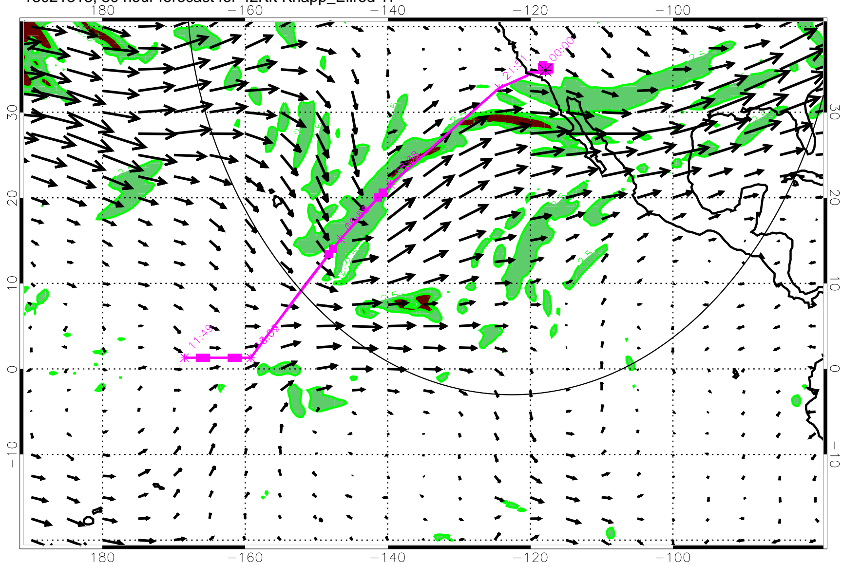
13021318, 30 hour forecast for 42Kft Knapp_Ellrod TI
