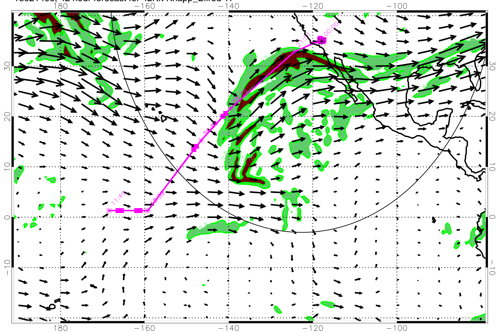
13021406, 42 hour forecast for 42Kft Knapp_Ellrod TI
