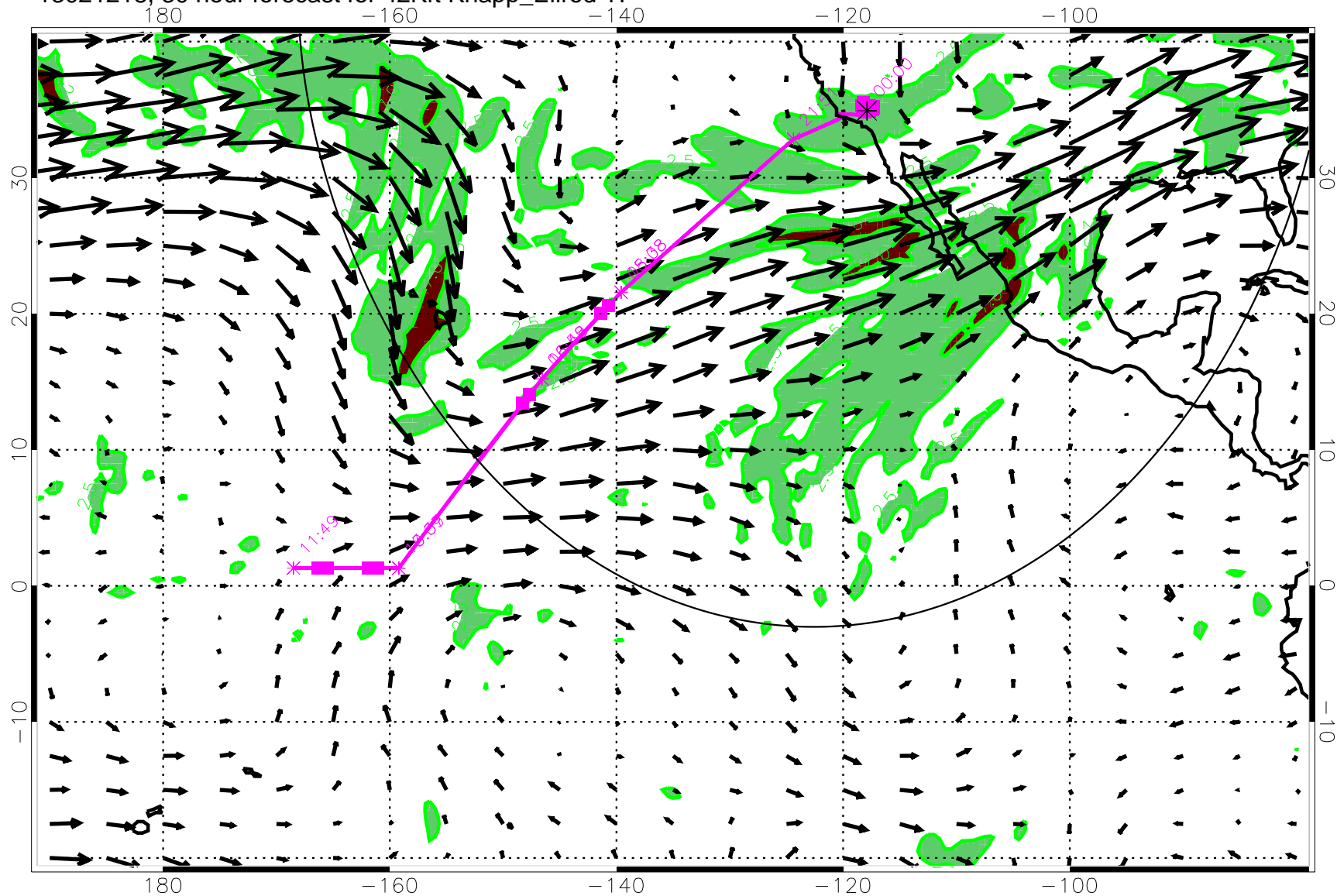
13021218, 30 hour forecast for 42Kft Knapp_Ellrod TI
