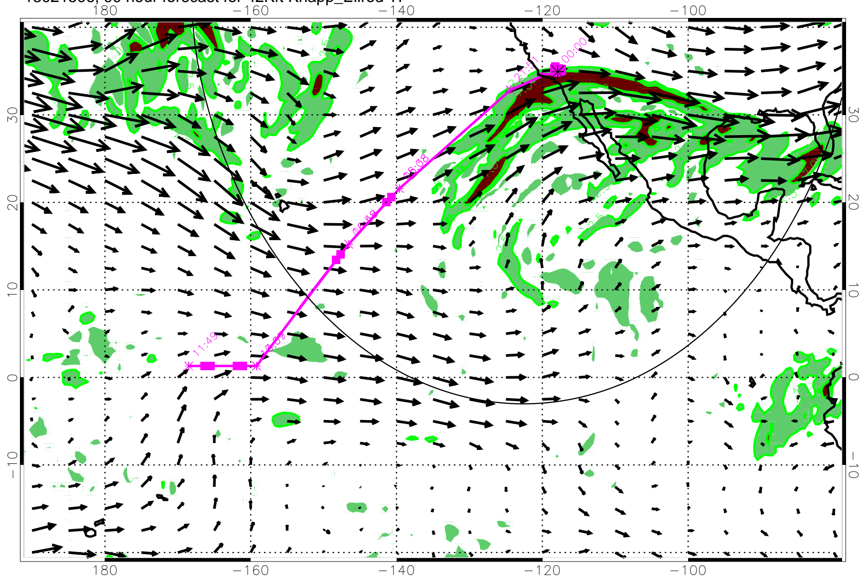
13021506, 90 hour forecast for 42Kft Knapp_Ellrod TI
