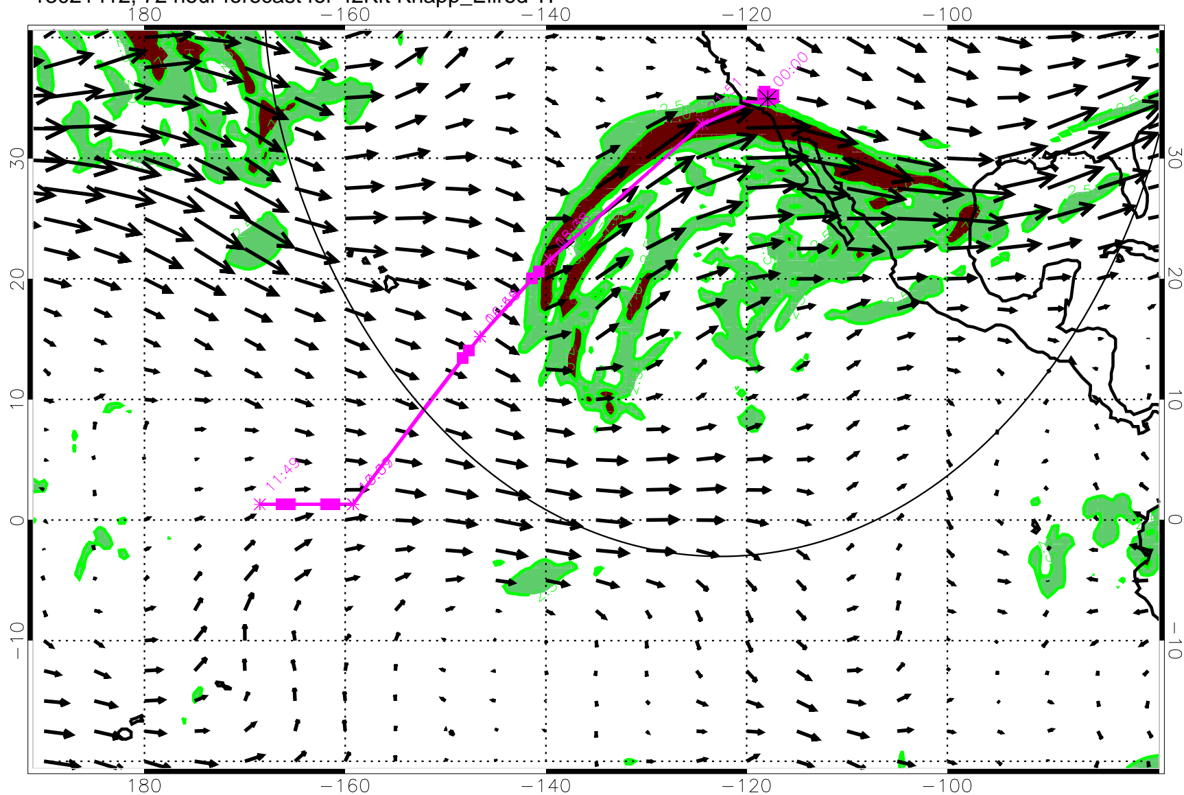
13021412, 72 hour forecast for 42Kft Knapp_Ellrod TI
