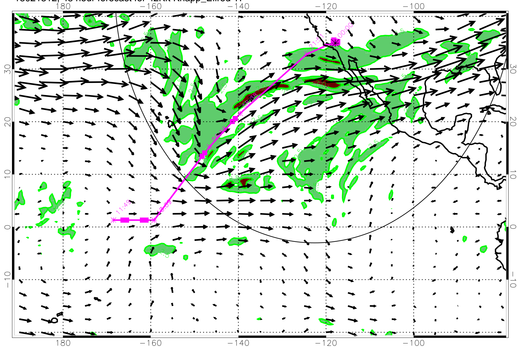
13021312, 48 hour forecast for 42Kft Knapp_Ellrod TI
