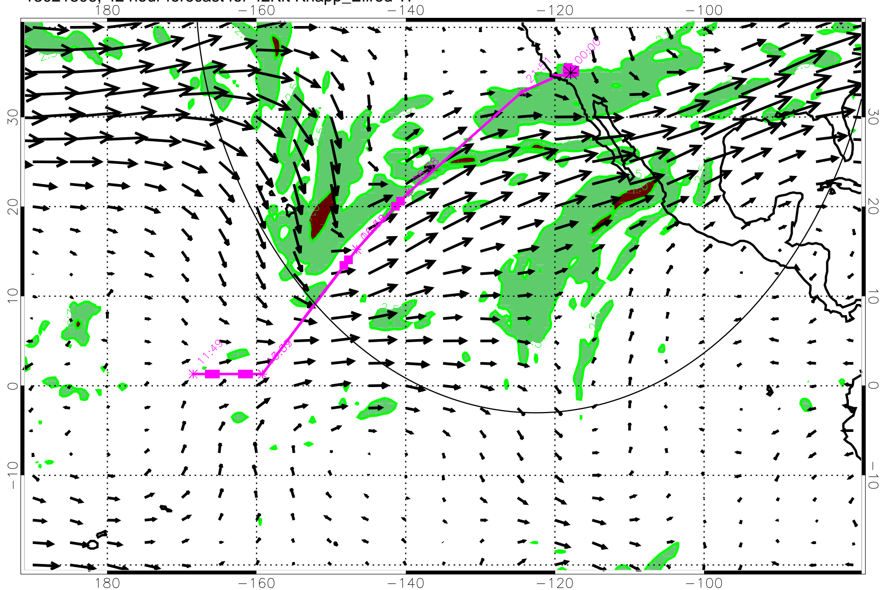
13021306, 42 hour forecast for 42Kft Knapp_Ellrod TI
