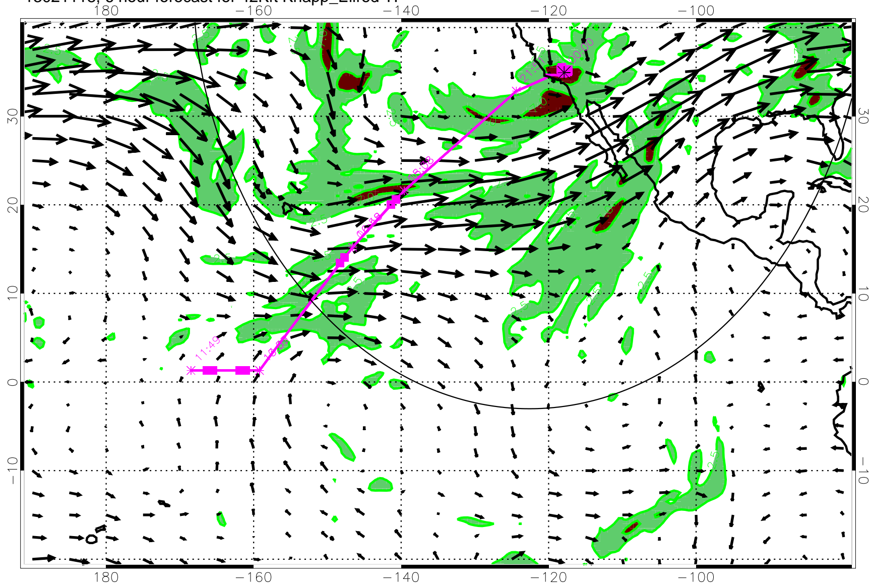
13021118, 6 hour forecast for 42Kft Knapp_Ellrod TI
