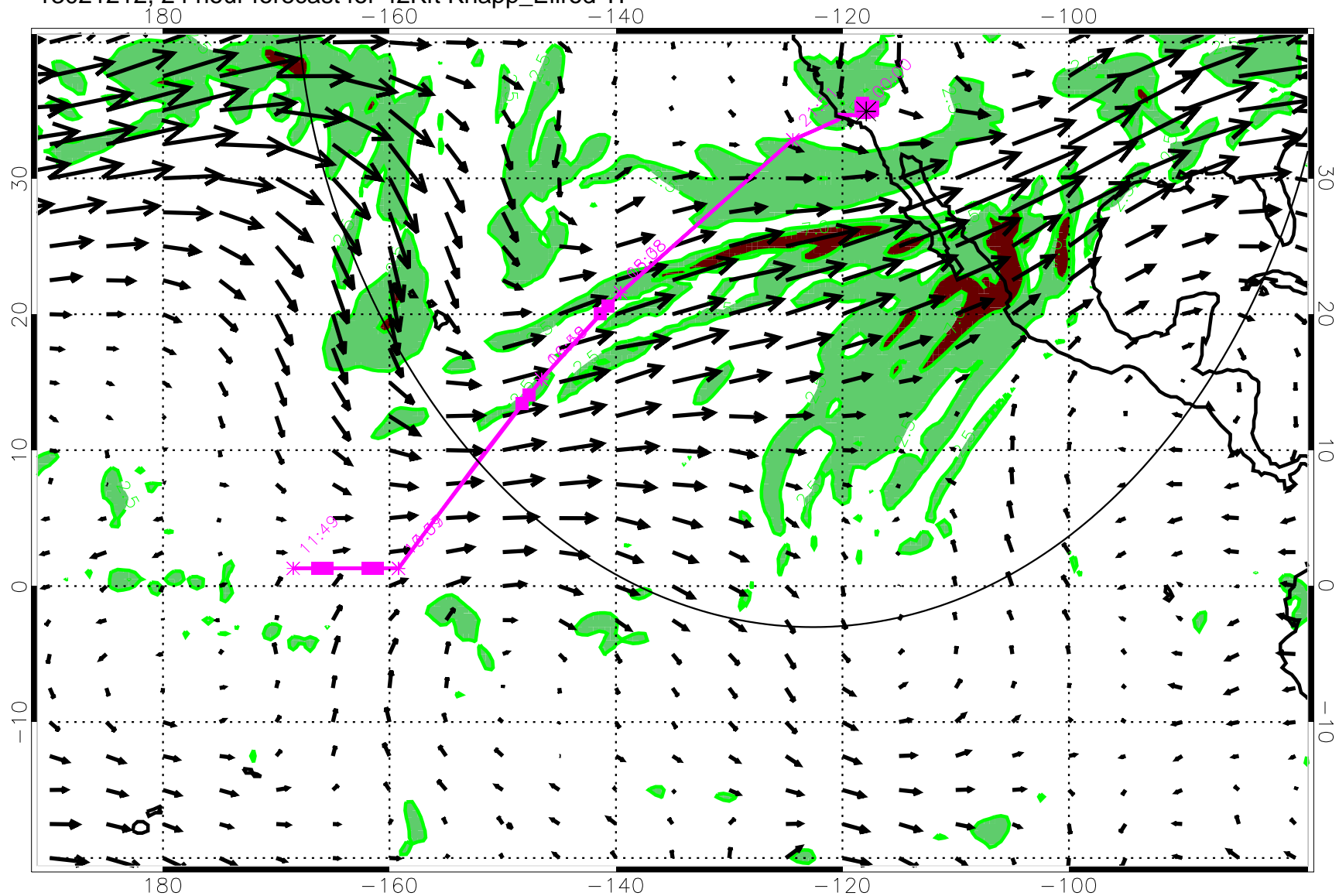
13021212, 24 hour forecast for 42Kft Knapp_Ellrod TI
