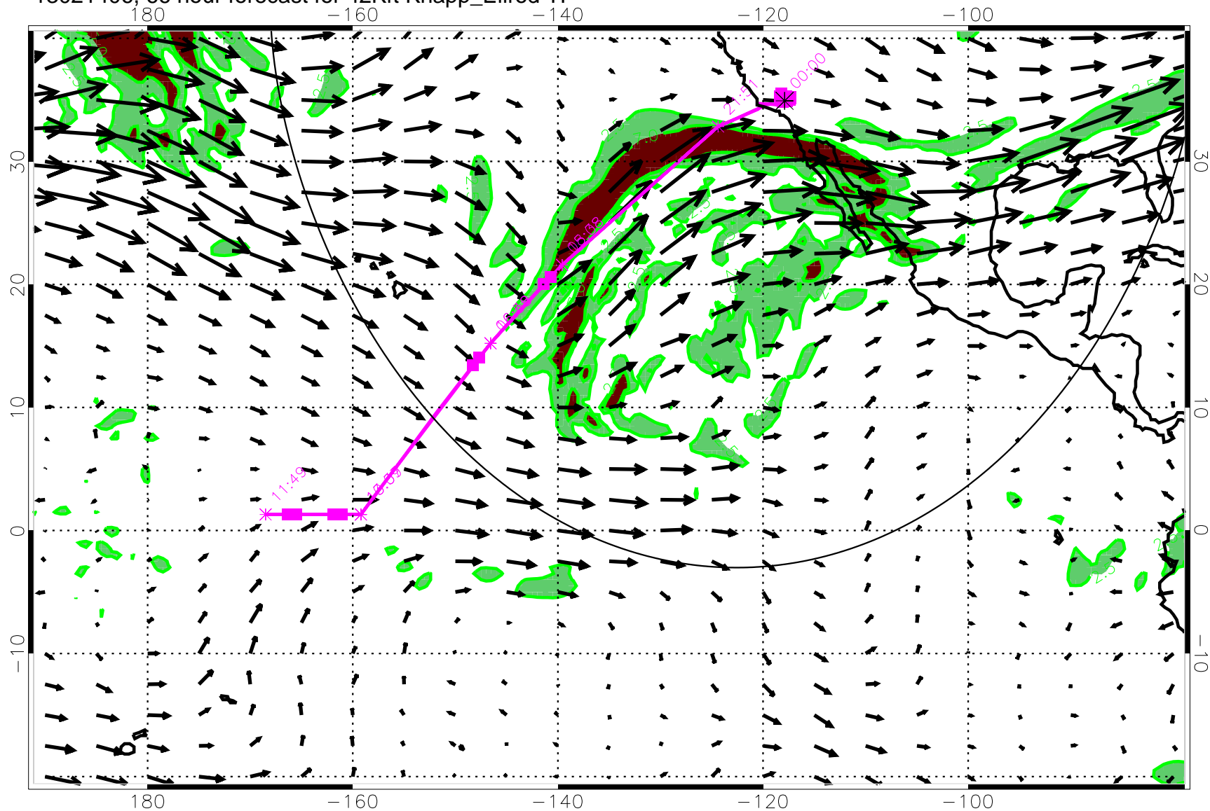
13021406, 66 hour forecast for 42Kft Knapp_Ellrod TI
