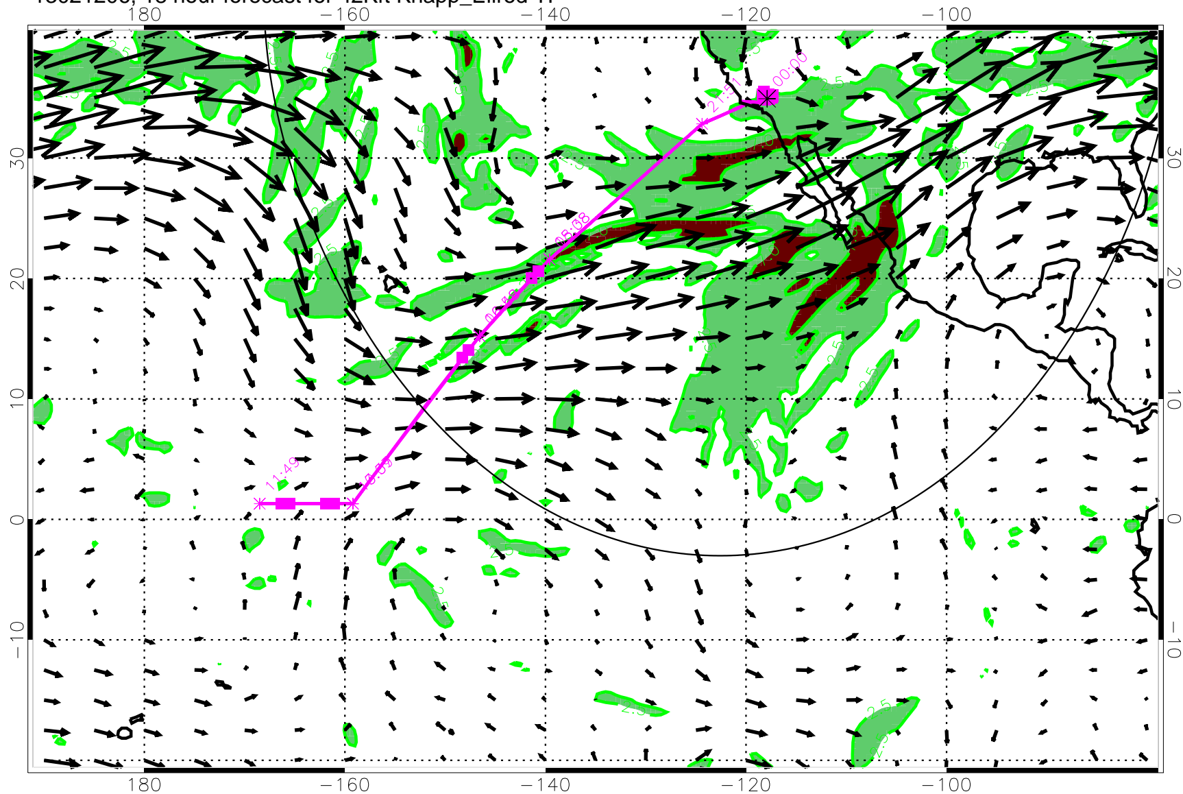
13021206, 18 hour forecast for 42Kft Knapp_Ellrod TI
