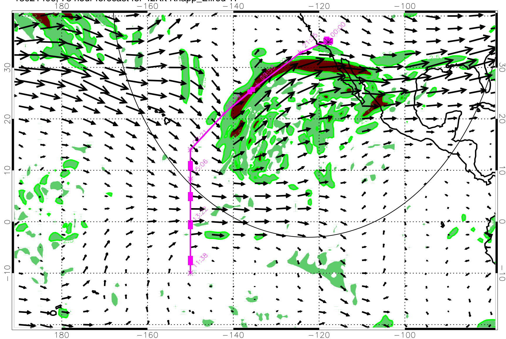
13021406, 78 hour forecast for 42Kft Knapp_Ellrod TI
