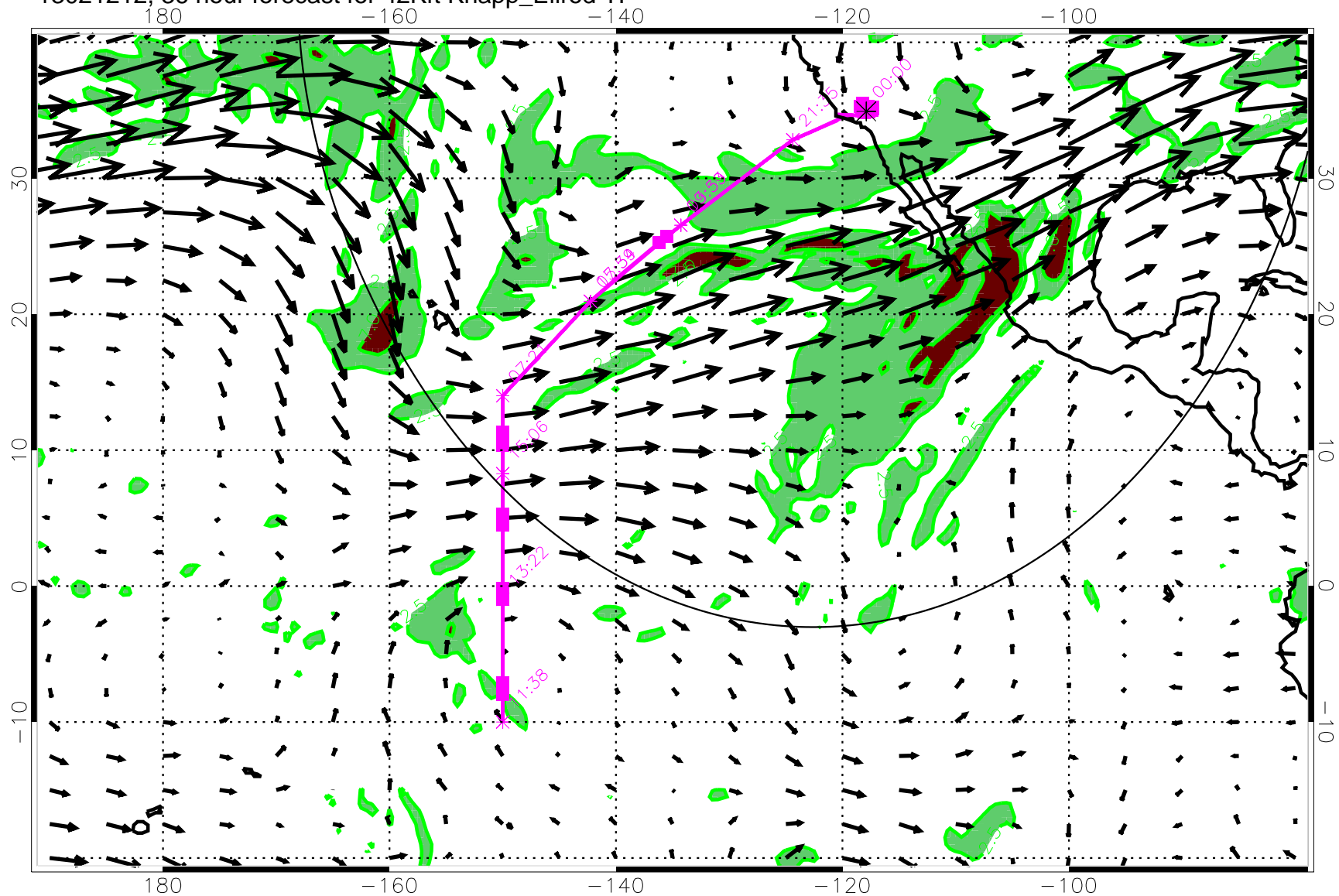
13021212, 36 hour forecast for 42Kft Knapp_Ellrod TI
