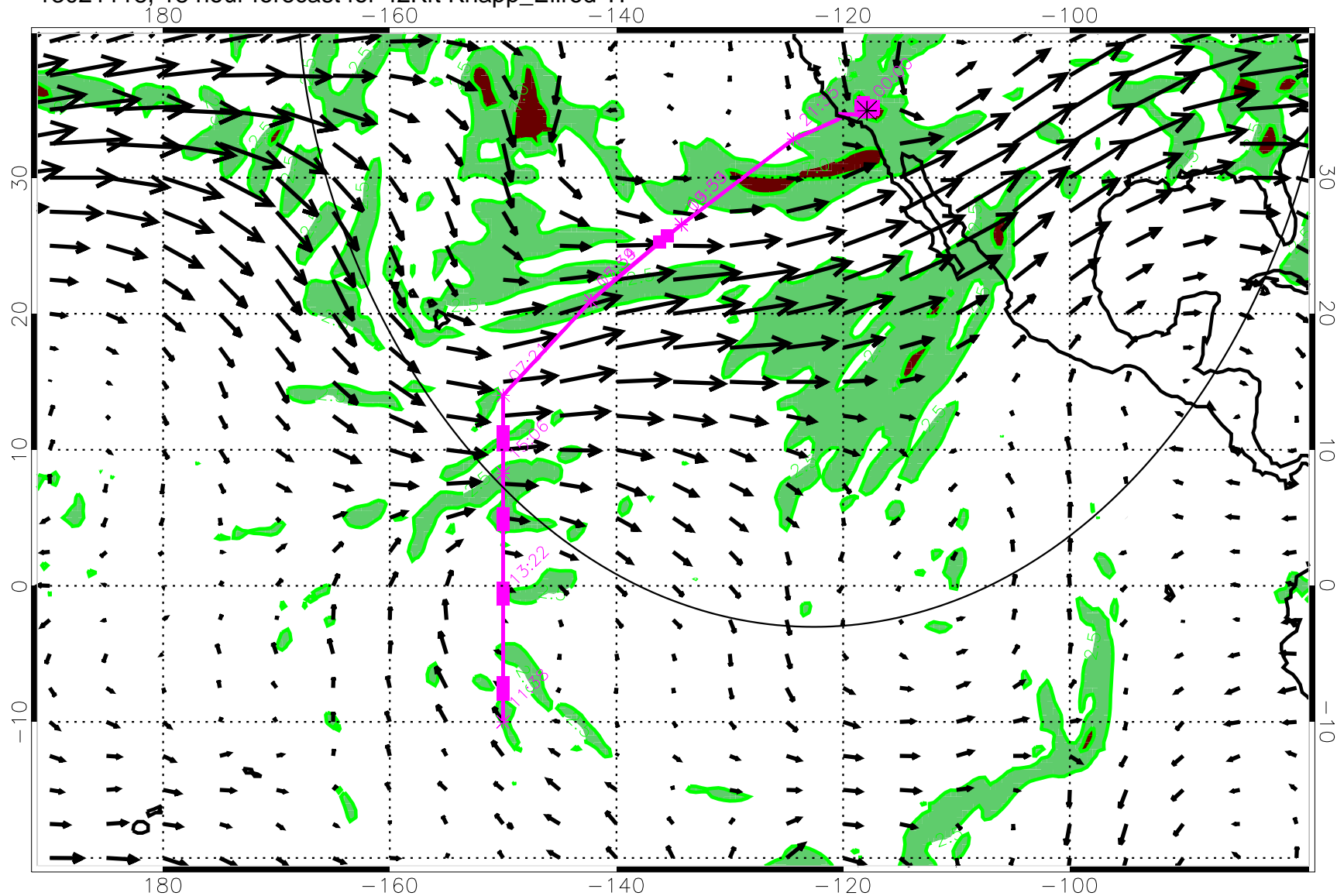
13021118, 18 hour forecast for 42Kft Knapp_Ellrod TI
