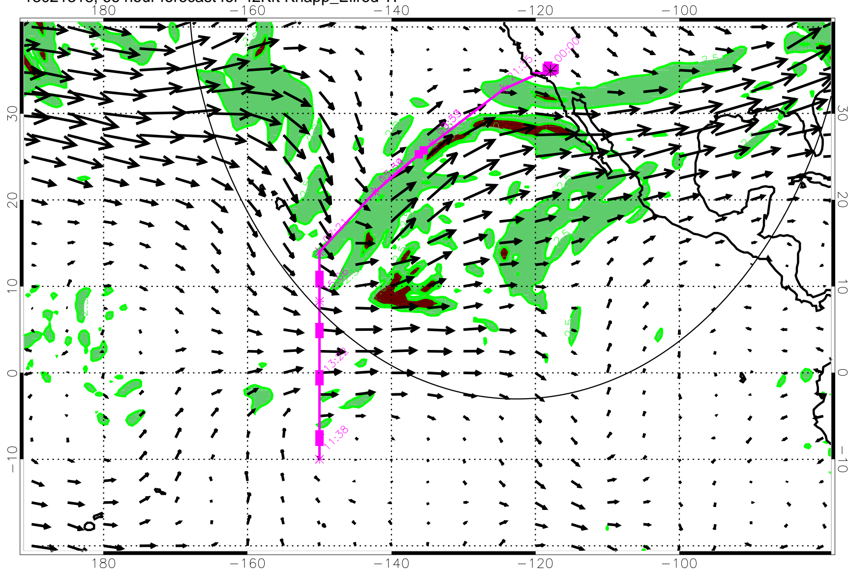
13021318, 66 hour forecast for 42Kft Knapp_Ellrod TI
