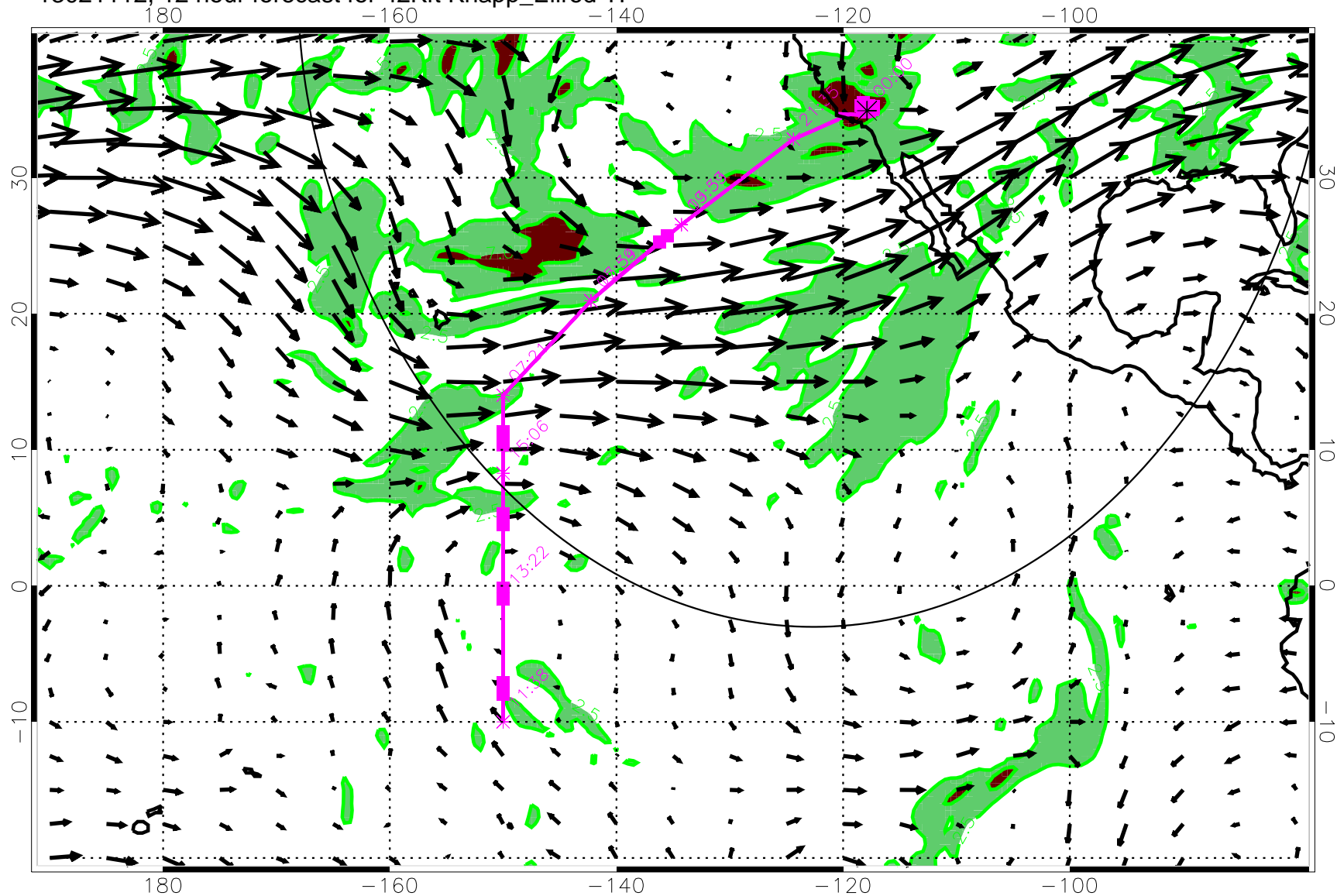
13021112, 12 hour forecast for 42Kft Knapp_Ellrod TI
