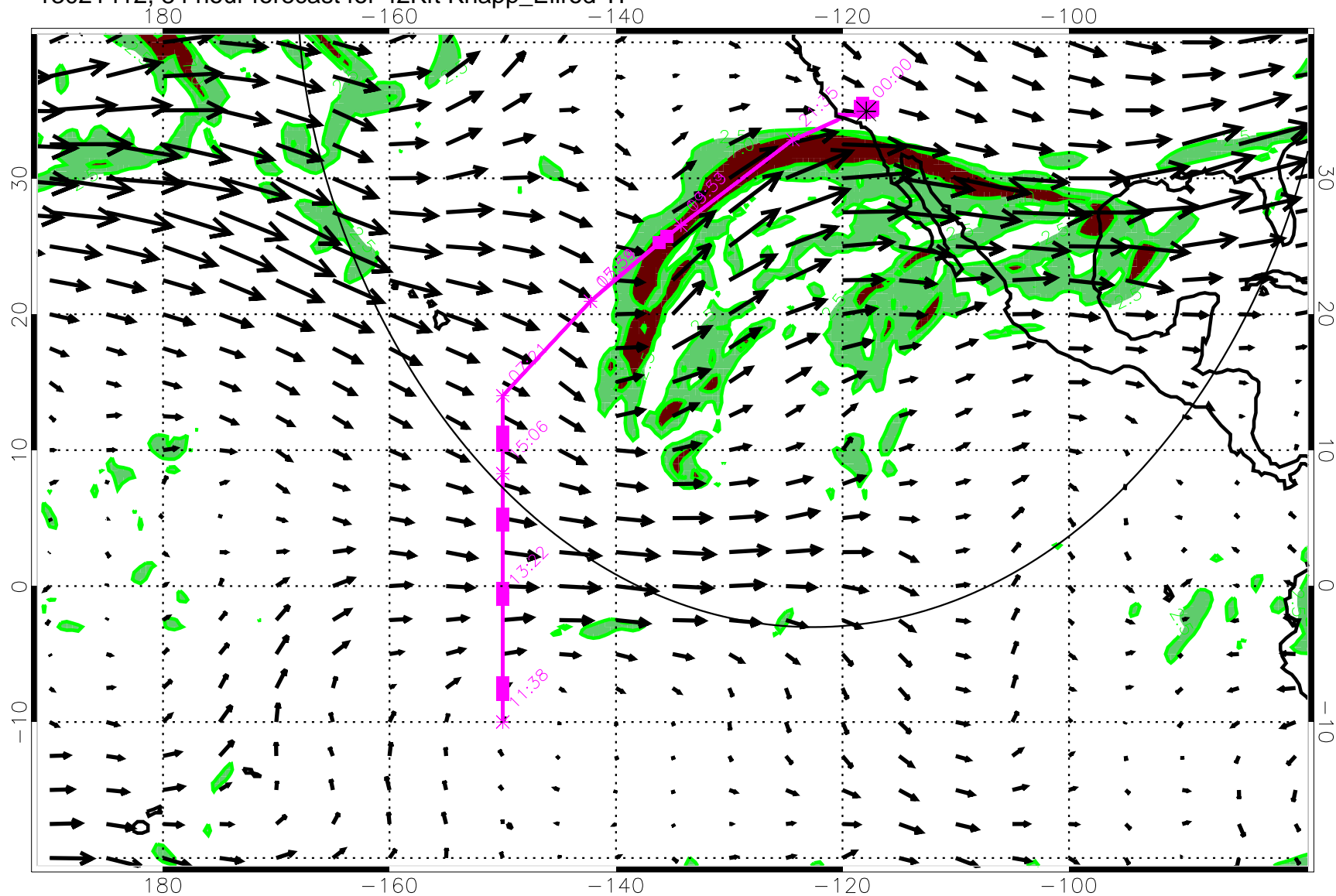
13021412, 84 hour forecast for 42Kft Knapp_Ellrod TI
