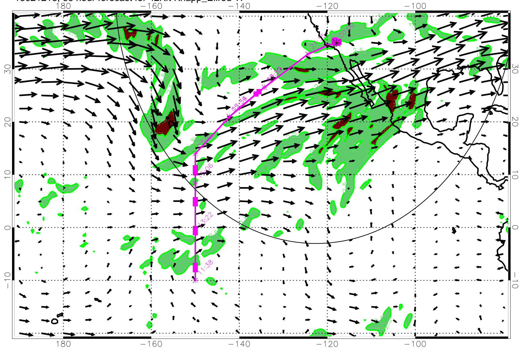
13021218, 66 hour forecast for 42Kft Knapp_Ellrod TI
