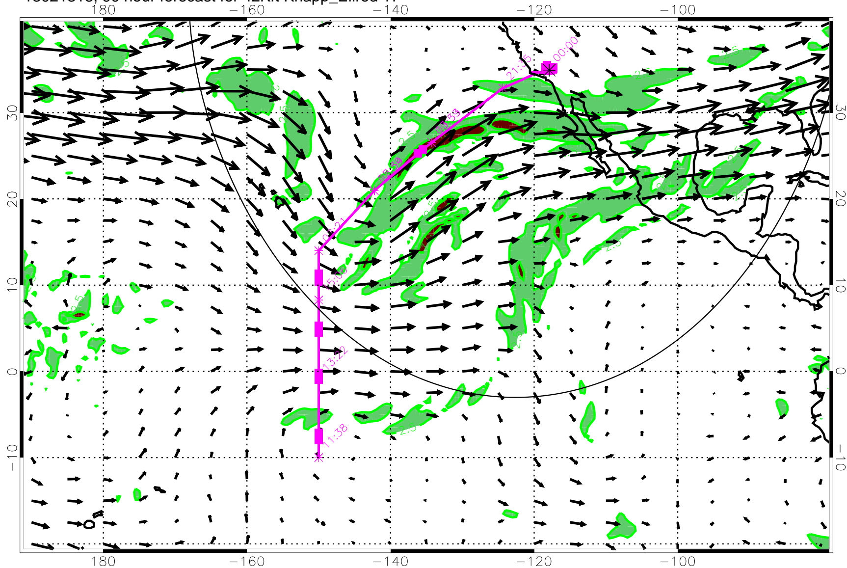
13021318, 90 hour forecast for 42Kft Knapp_Ellrod TI
