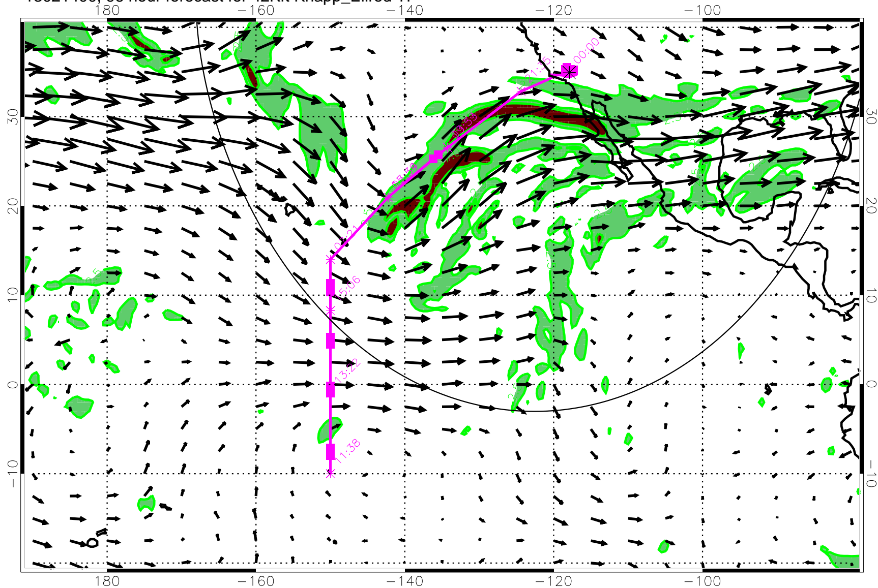
13021400, 96 hour forecast for 42Kft Knapp_Ellrod TI
