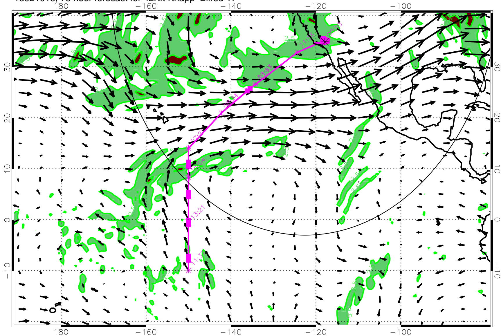
13021018, 78 hour forecast for 42Kft Knapp_Ellrod TI
