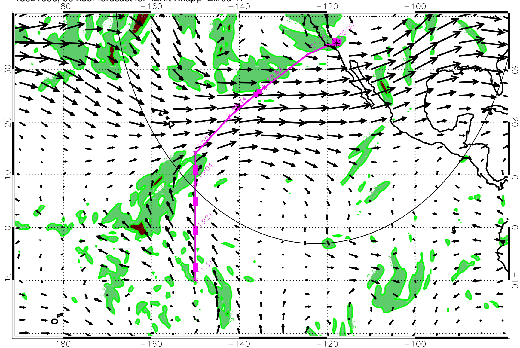
13021006, 66 hour forecast for 42Kft Knapp_Ellrod TI
