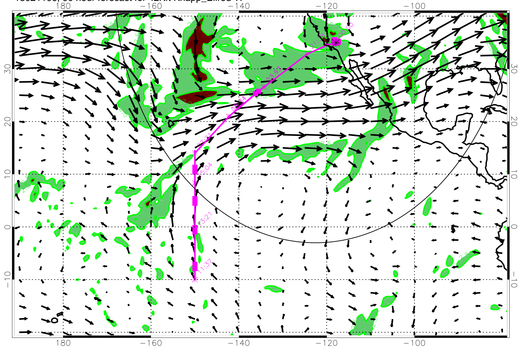
13021106, 90 hour forecast for 42Kft Knapp_Ellrod TI
