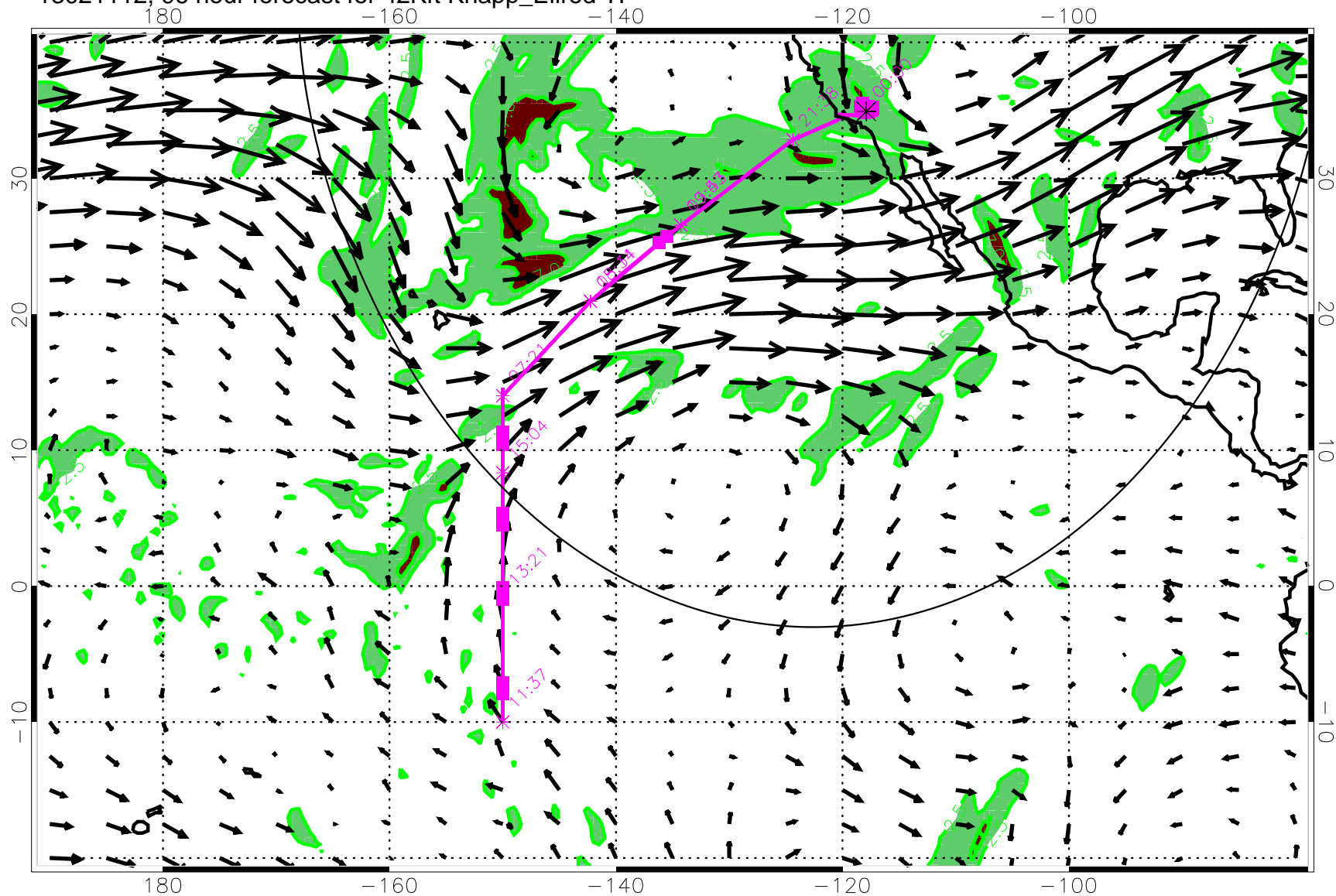
13021112, 96 hour forecast for 42Kft Knapp_Ellrod TI
