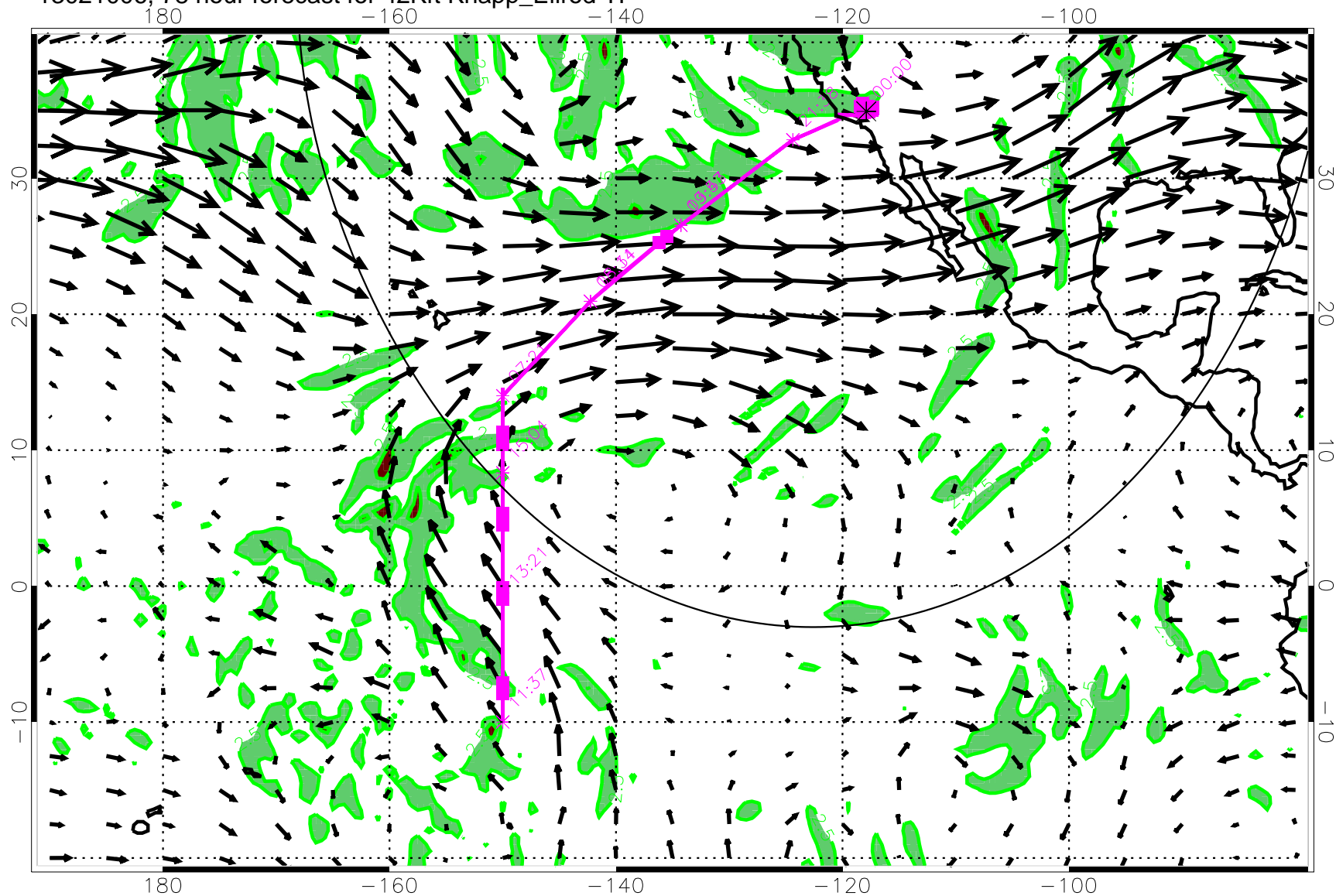
13021006, 78 hour forecast for 42Kft Knapp_Ellrod TI
