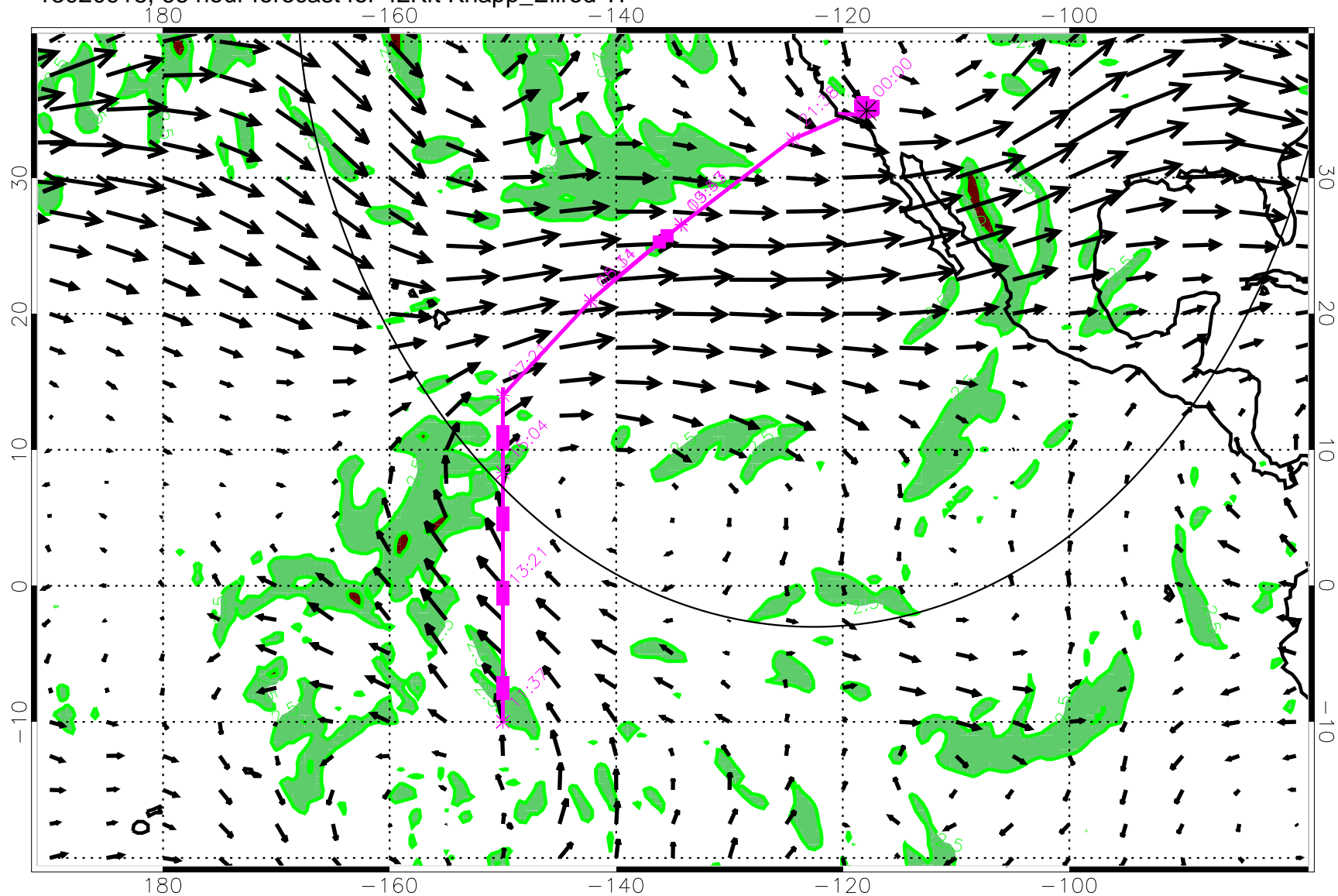
13020918, 66 hour forecast for 42Kft Knapp_Ellrod TI
