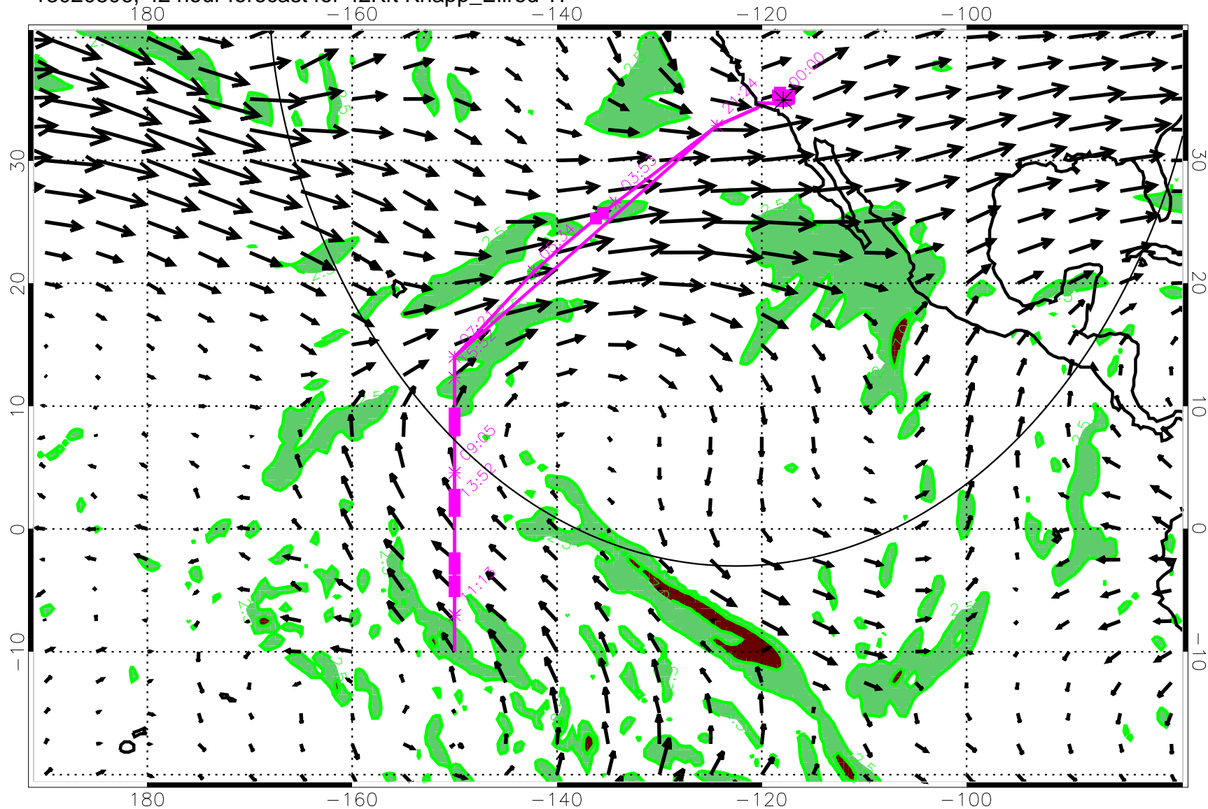
13020806, 42 hour forecast for 42Kft Knapp_Ellrod TI
