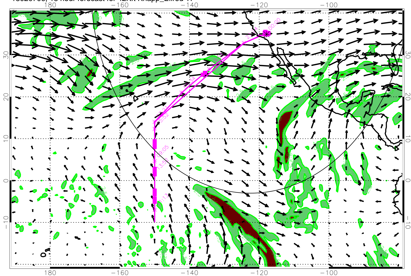
13020706, 18 hour forecast for 42Kft Knapp_Ellrod TI
