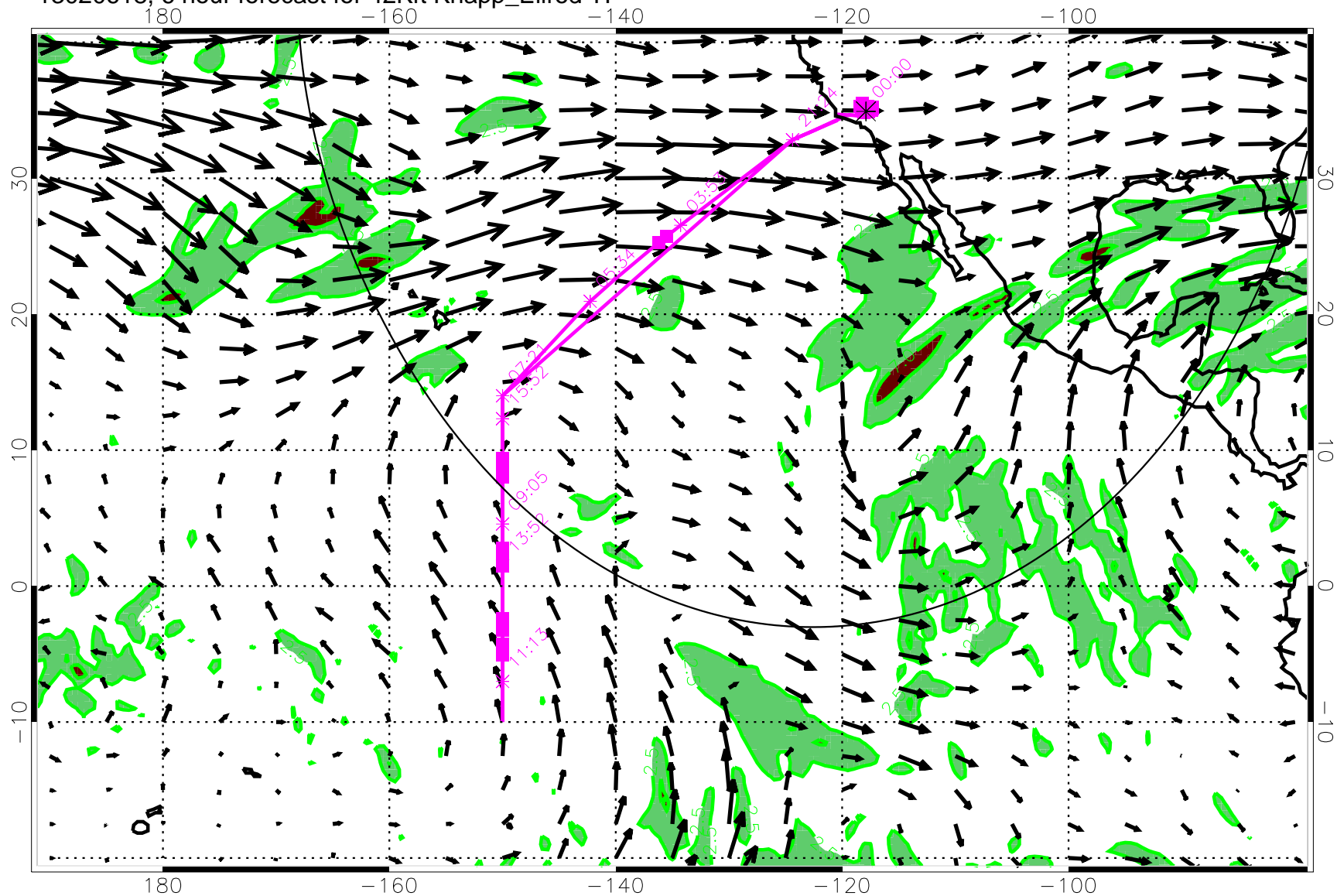
13020618, 6 hour forecast for 42Kft Knapp_Ellrod TI
