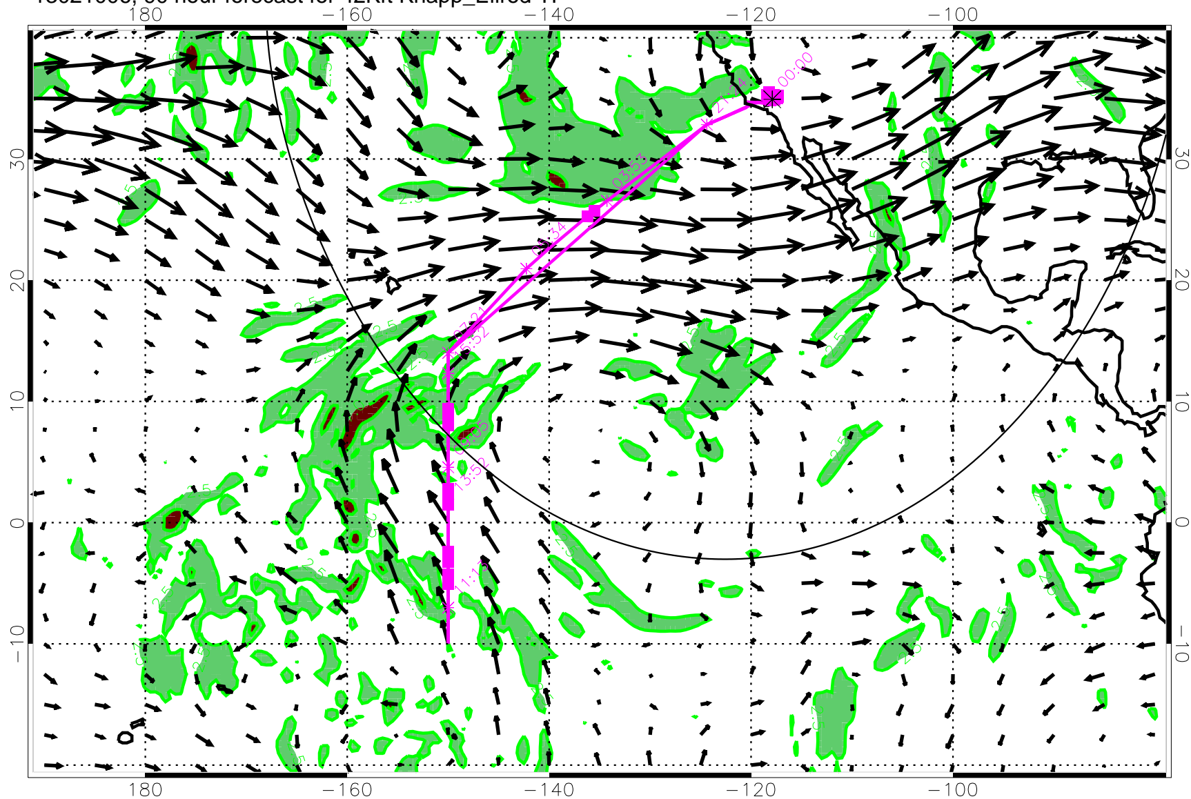
13021006, 90 hour forecast for 42Kft Knapp_Ellrod TI
