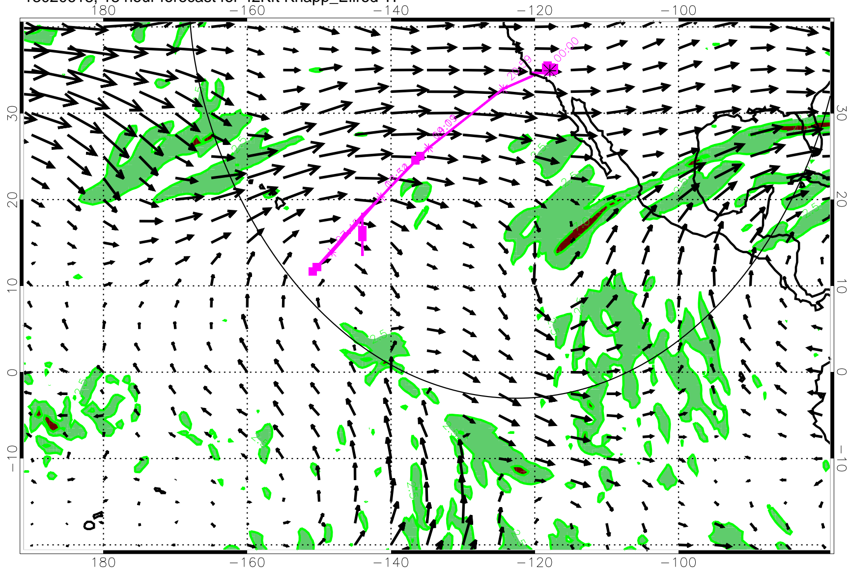
13020618, 18 hour forecast for 42Kft Knapp_Ellrod TI
