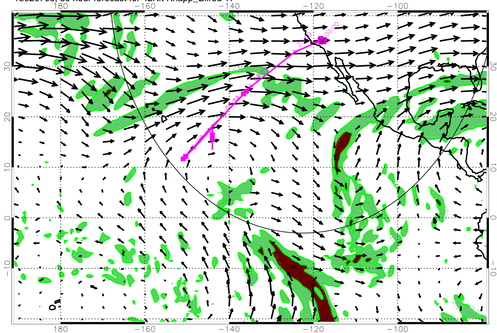
13020706, 30 hour forecast for 42Kft Knapp_Ellrod TI
