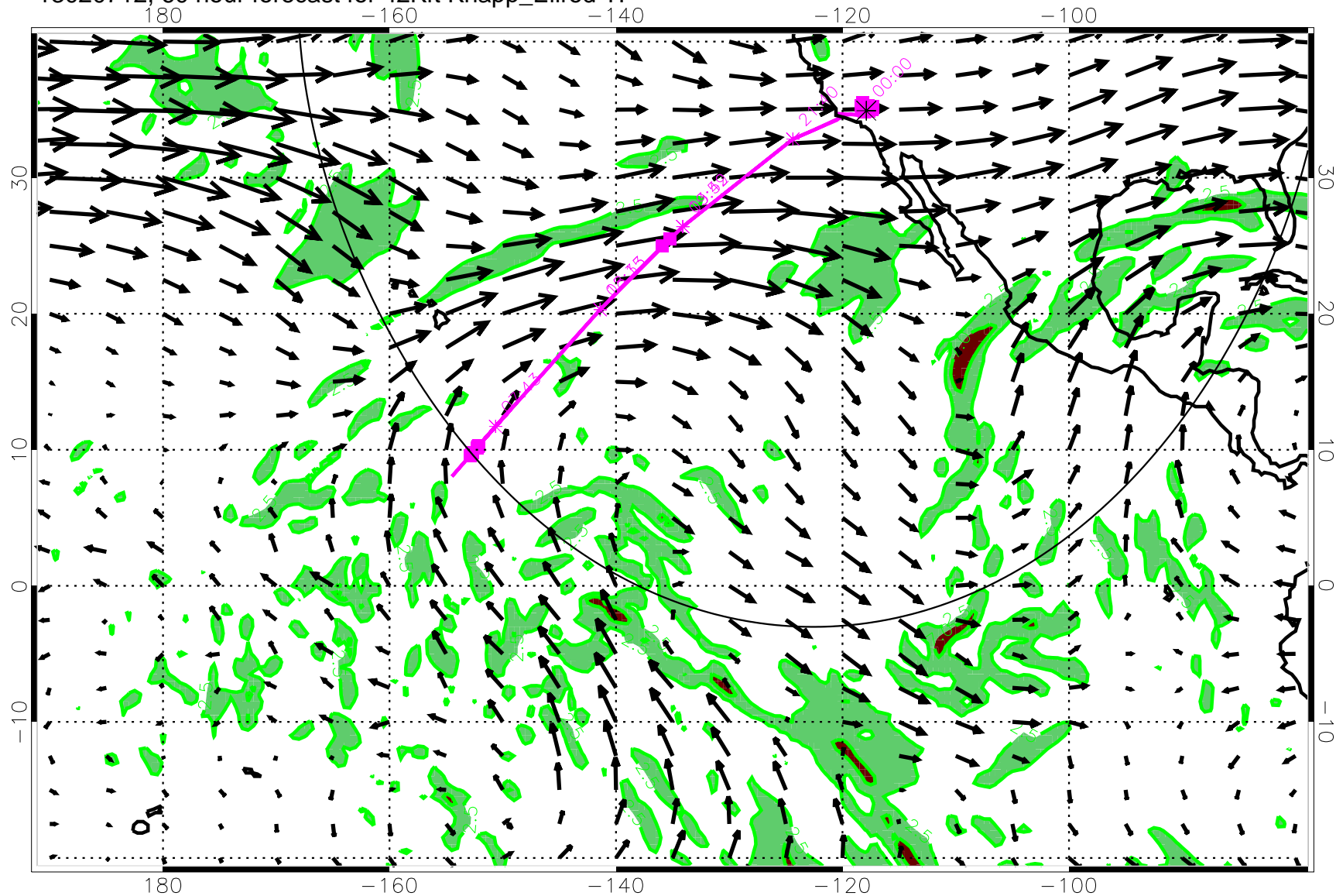
13020712, 60 hour forecast for 42Kft Knapp_Ellrod TI
