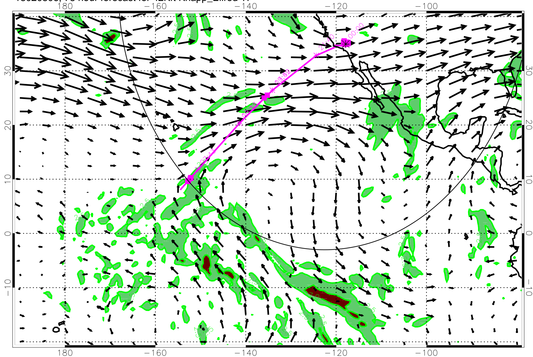
13020806, 78 hour forecast for 42Kft Knapp_Ellrod TI
