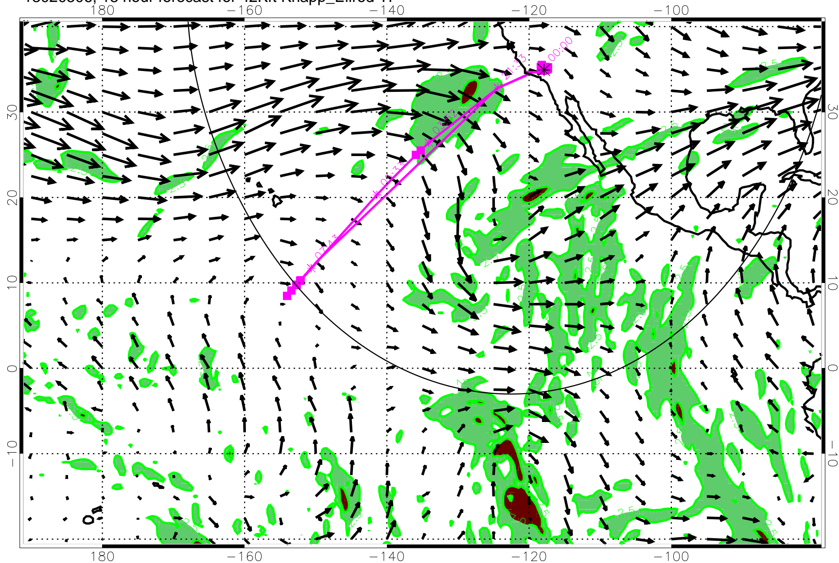
13020506, 18 hour forecast for 42Kft Knapp_Ellrod TI
