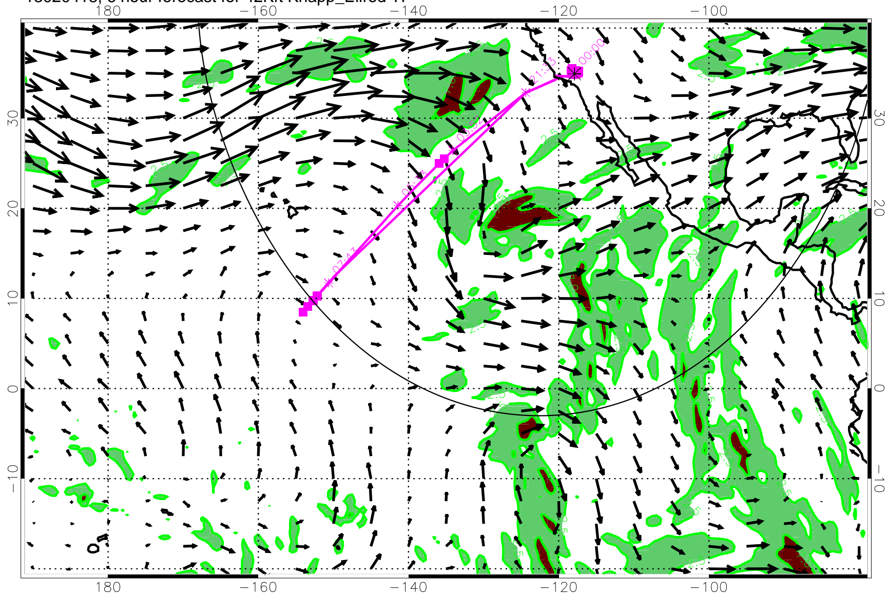
13020418, 6 hour forecast for 42Kft Knapp_Ellrod TI
