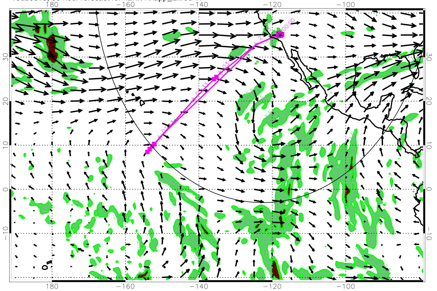
13020518, 30 hour forecast for 42Kft Knapp_Ellrod T1
