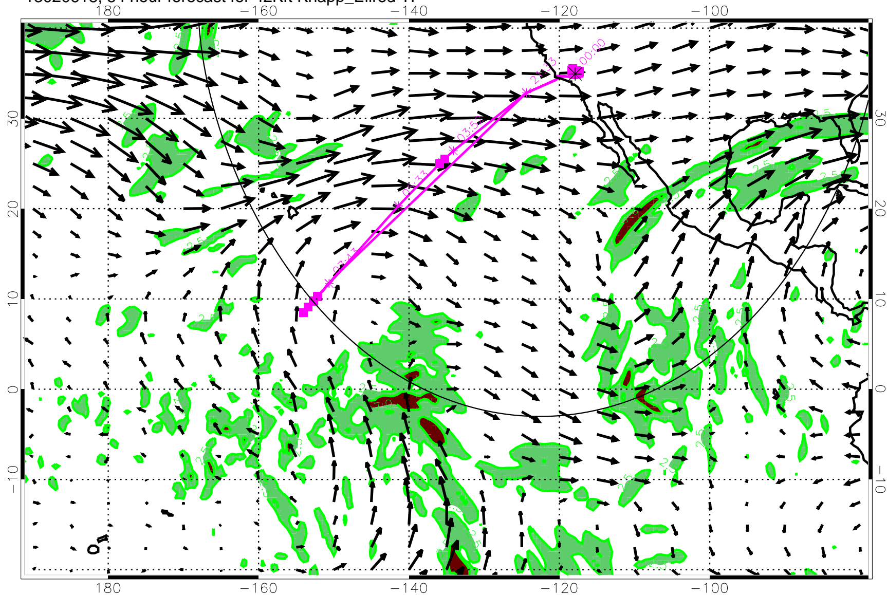
13020618, 54 hour forecast for 42Kft Knapp_Ellrod TI
