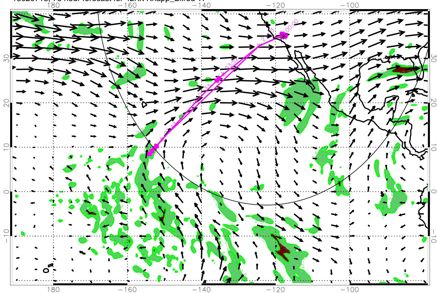
13020718, 78 hour forecast for 42Kft Knapp_Ellrod TI
