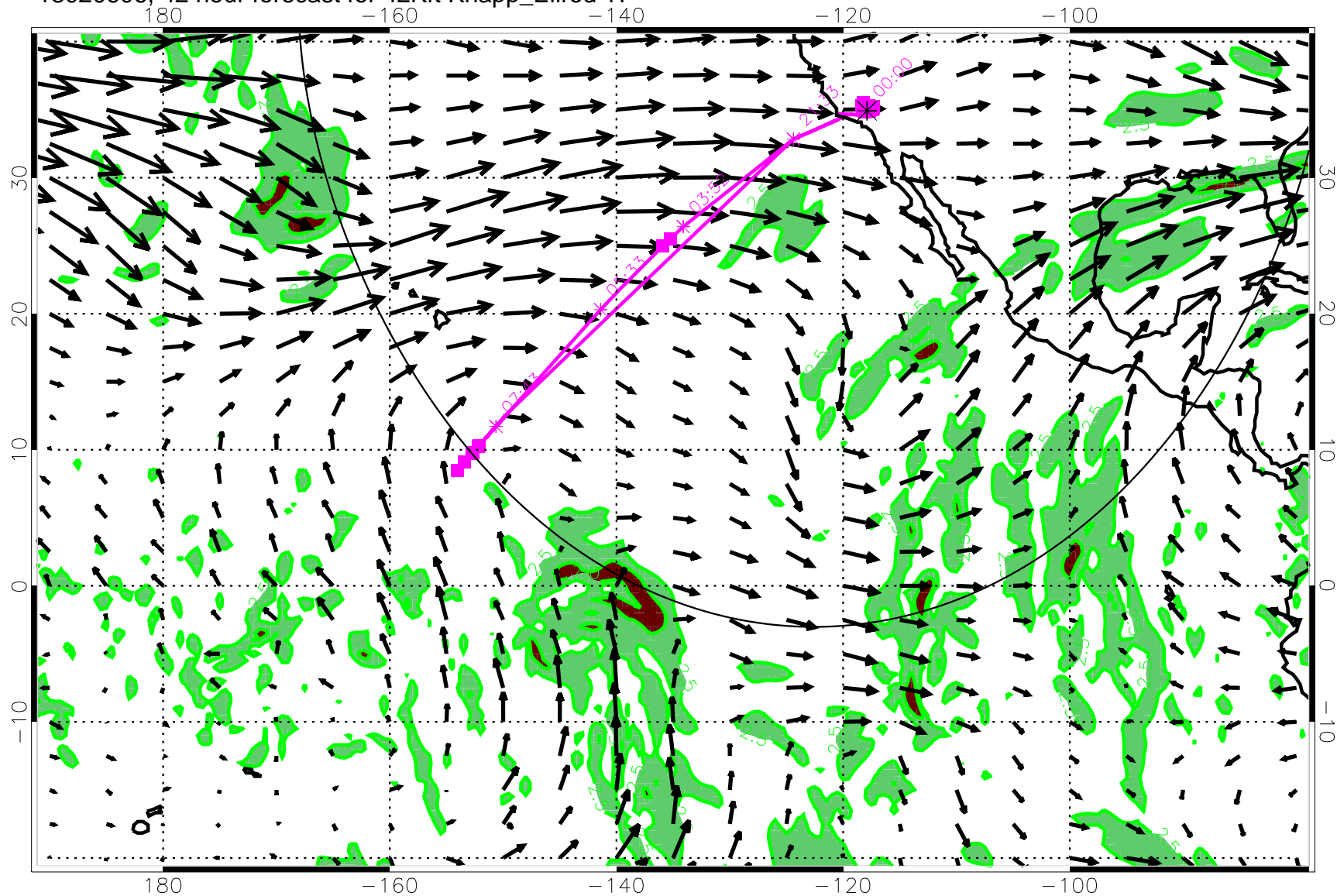
13020606, 42 hour forecast for 42Kft Knapp_Ellrod TI
