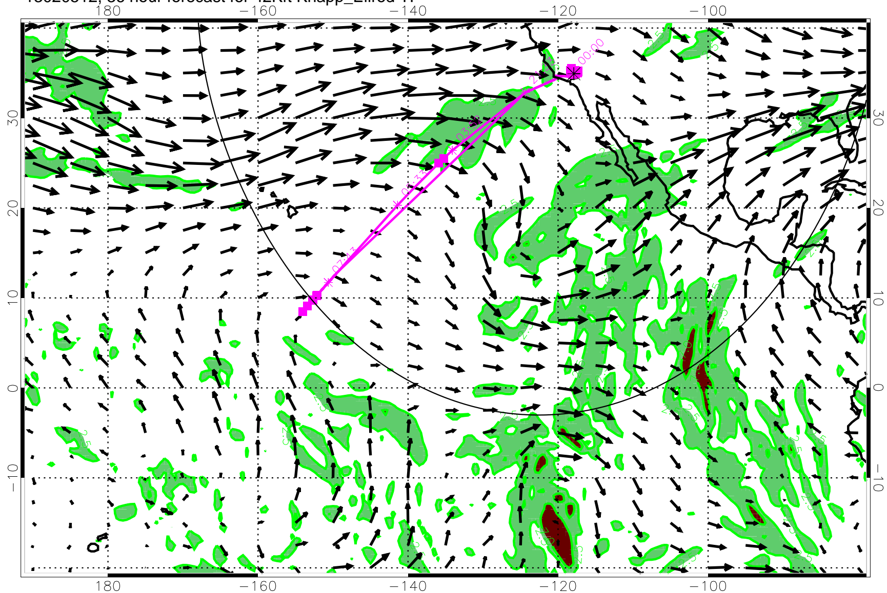
13020512, 36 hour forecast for 42Kft Knapp_Ellrod TI
