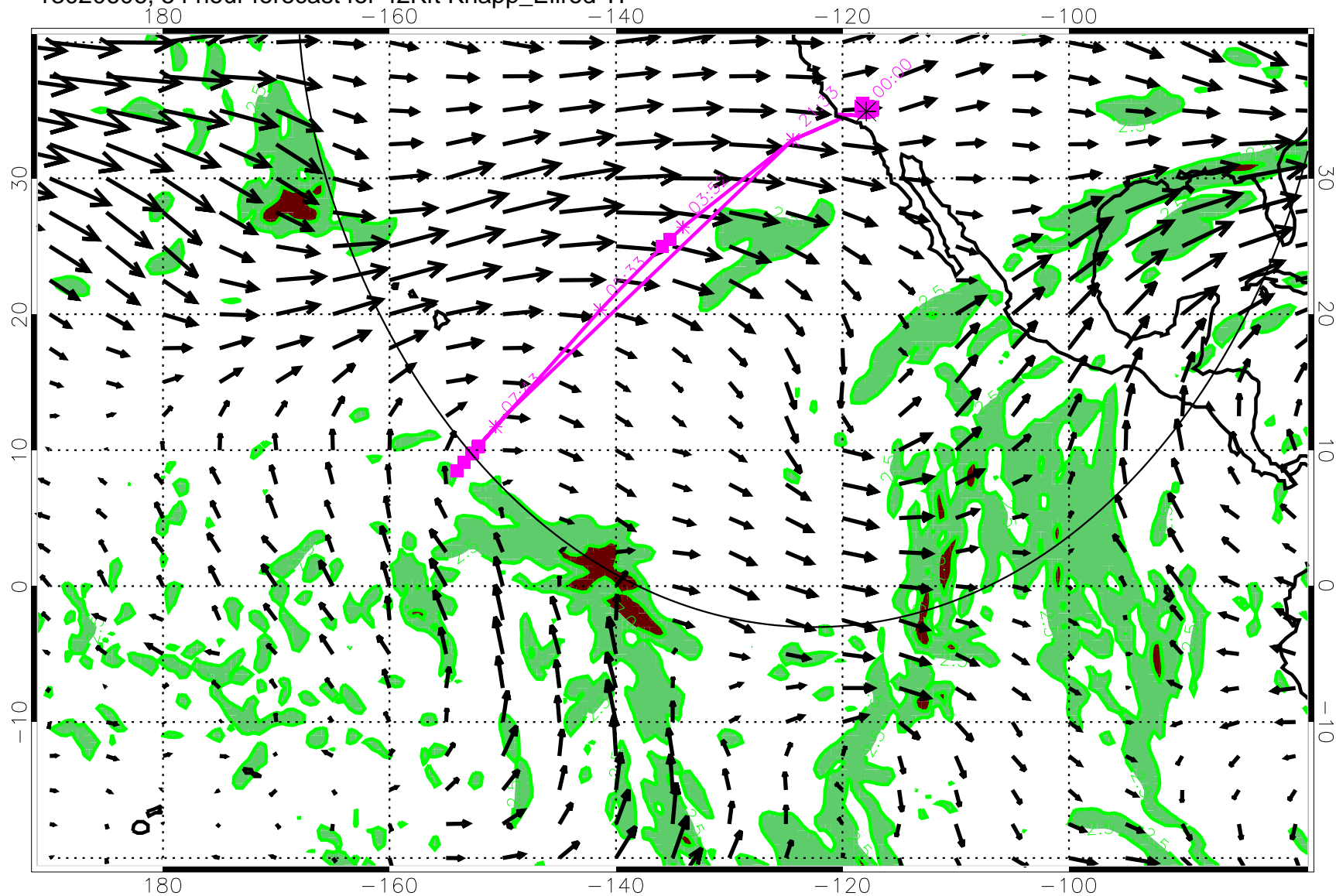
13020606, 54 hour forecast for 42Kft Knapp_Ellrod TI
