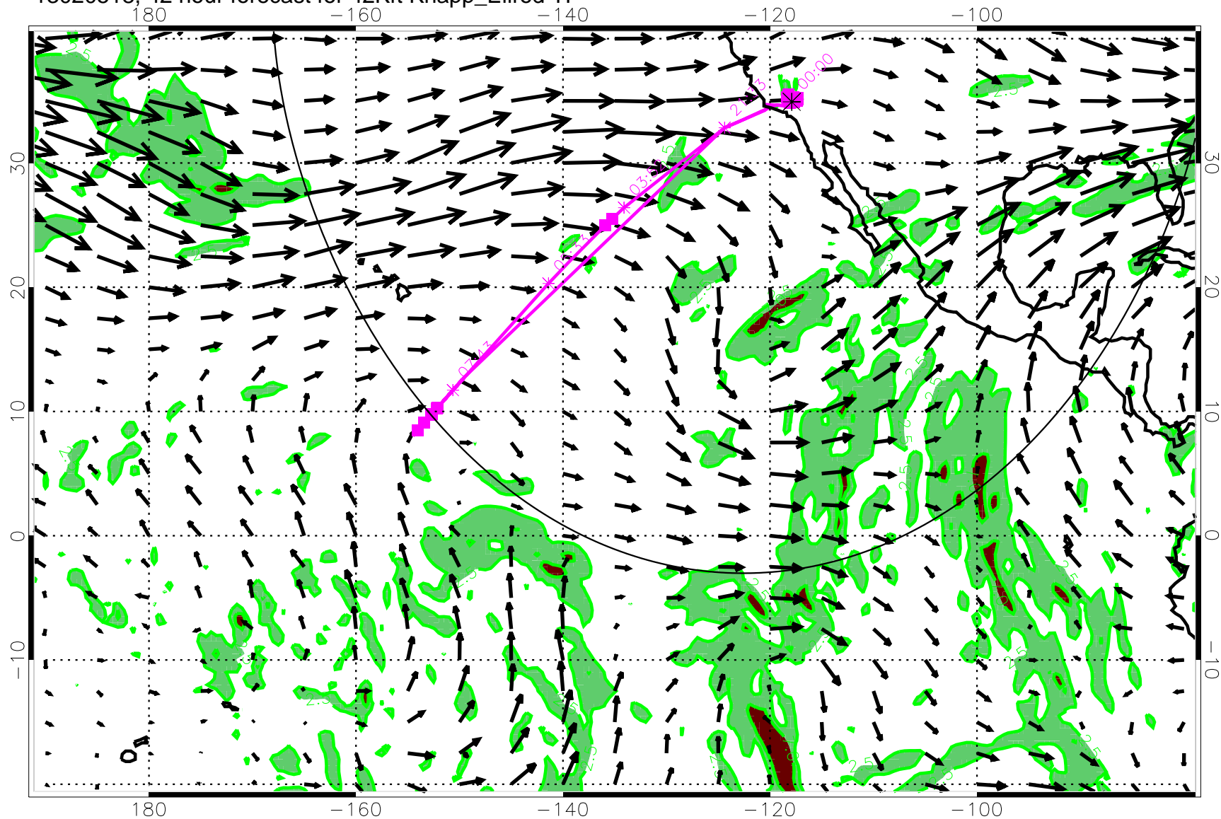
13020518, 42 hour forecast for 42Kft Knapp_Ellrod TI
