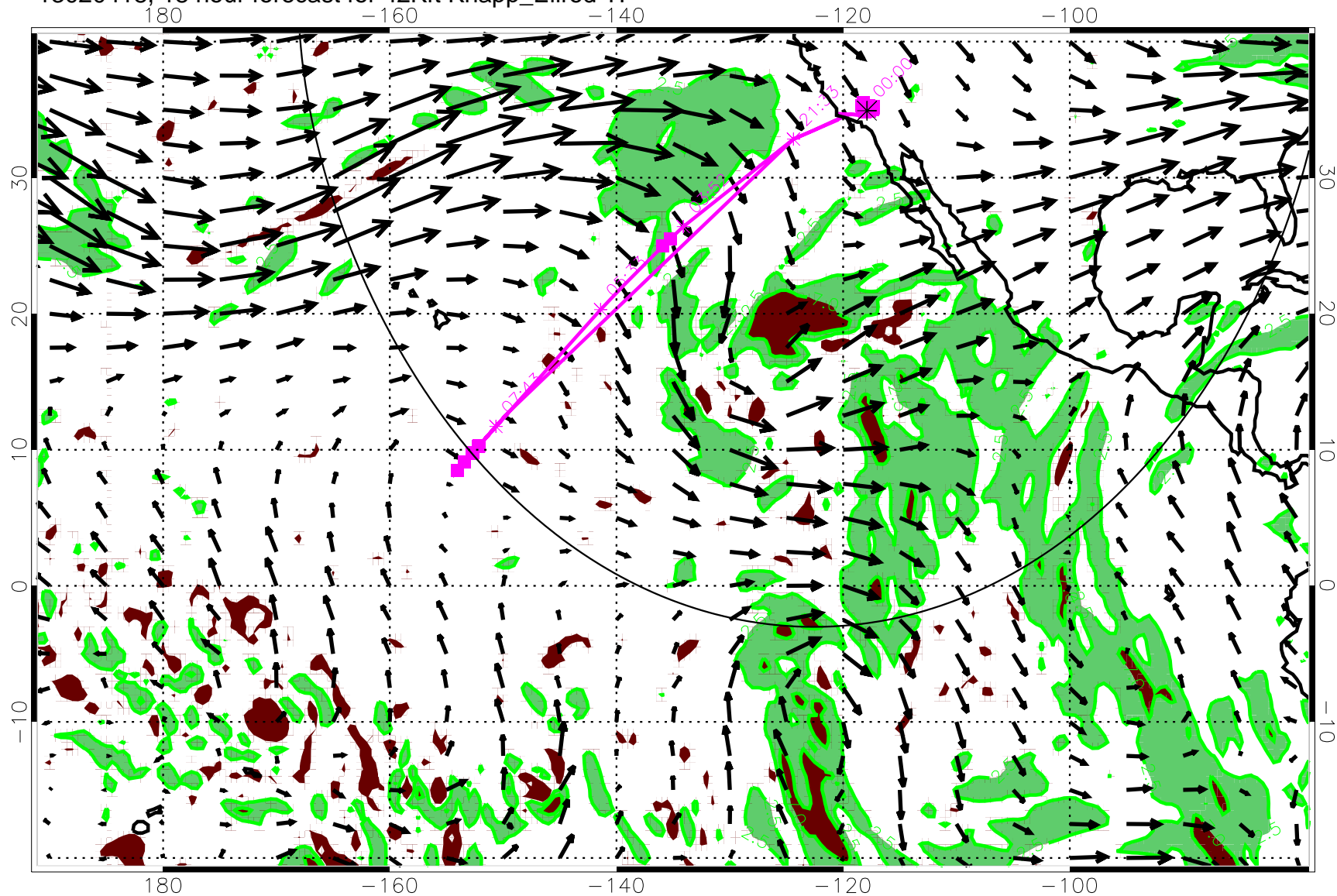
13020418, 18 hour forecast for 42Kft Knapp_Ellrod TI
