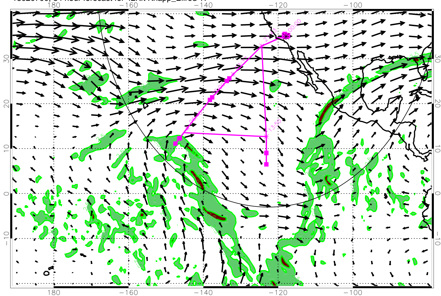
13020700, 84 hour forecast for 42Kft Knapp_Ellrod TI
