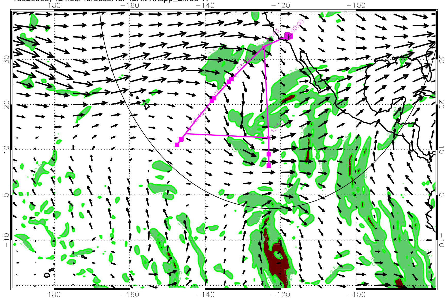
13020506, 42 hour forecast for 42Kft Knapp_Ellrod TI
