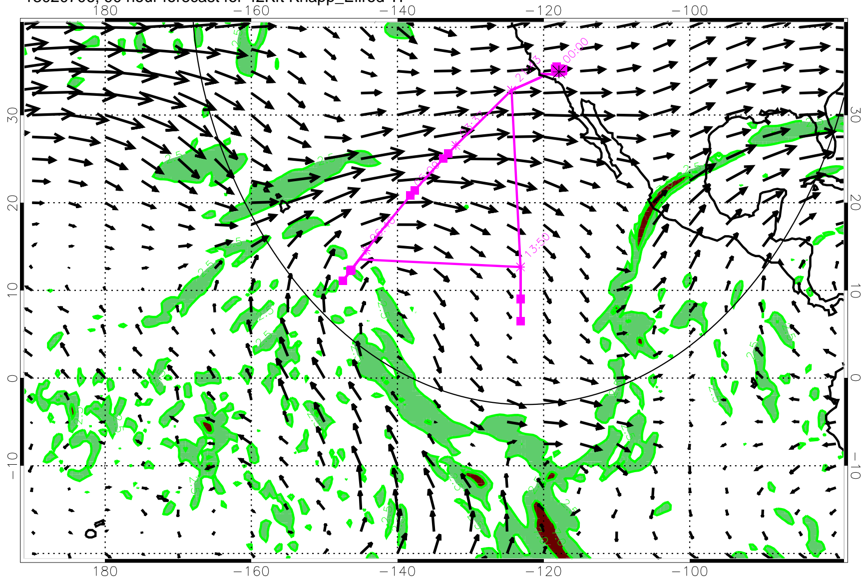
13020706, 90 hour forecast for 42Kft Knapp_Ellrod TI
