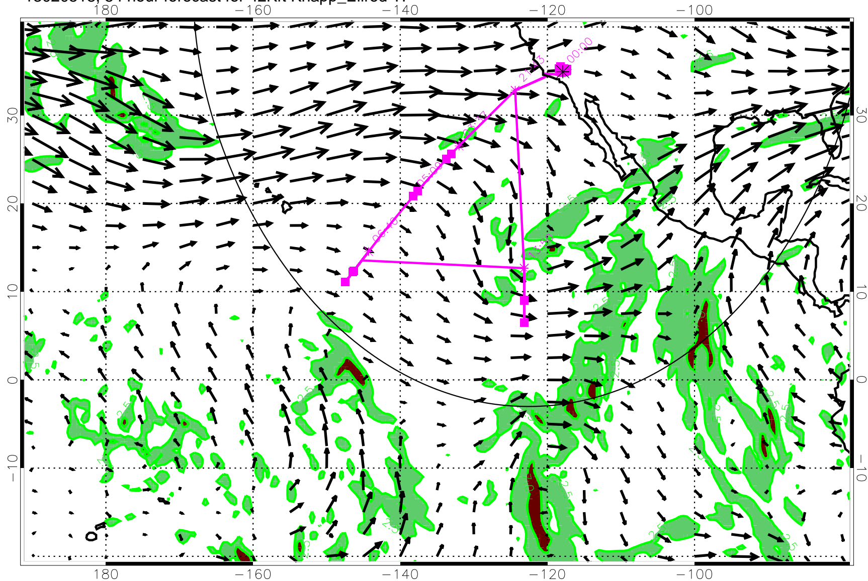
13020518, 54 hour forecast for 42Kft Knapp_Ellrod TI
