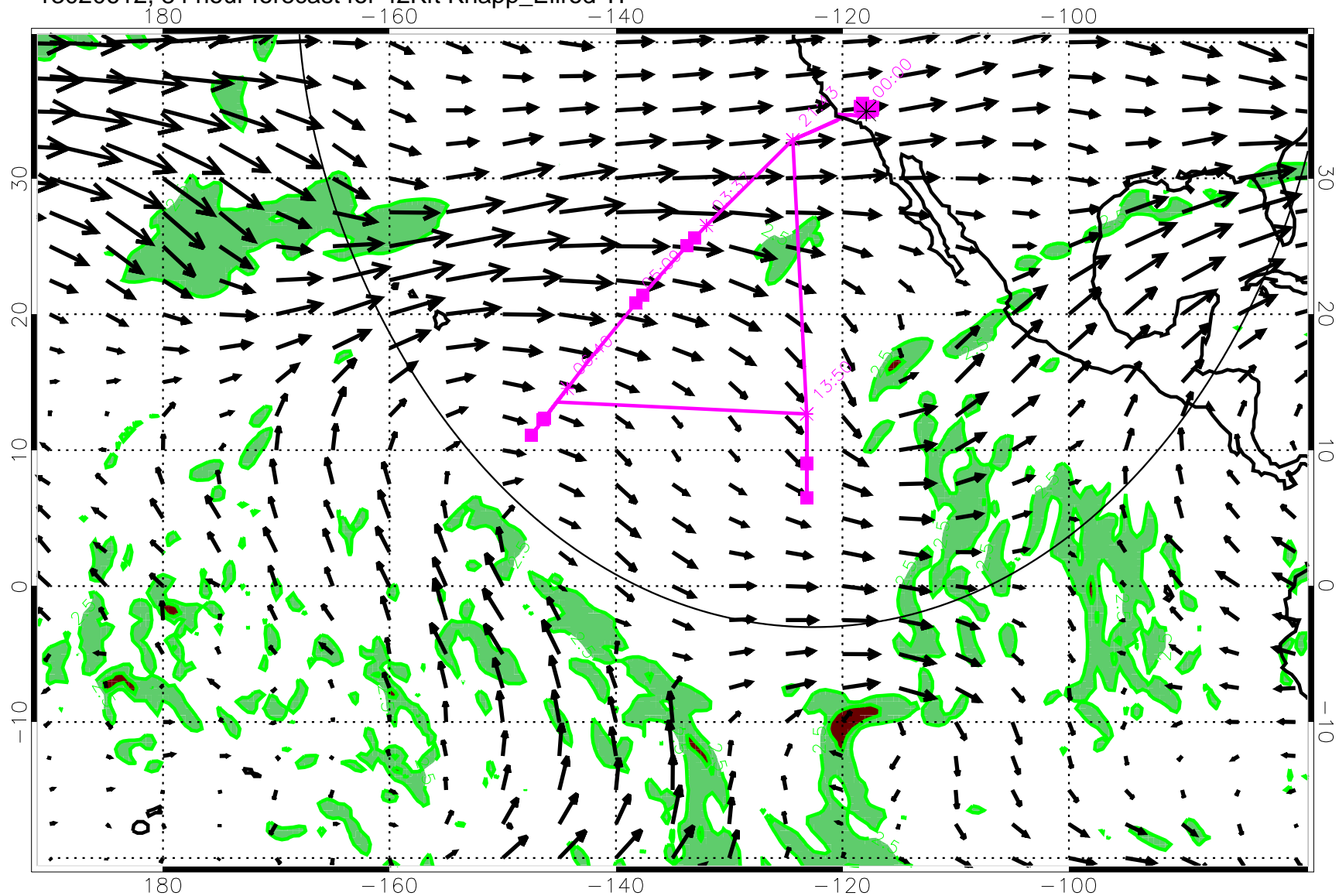
13020612, 84 hour forecast for 42Kft Knapp_Ellrod TI
