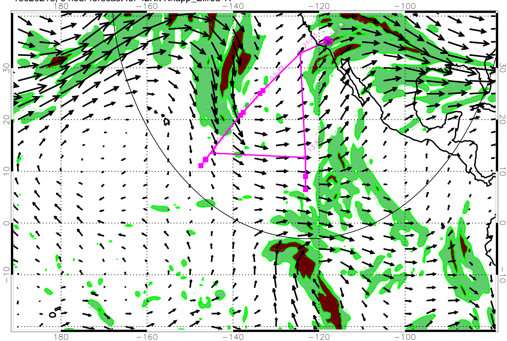
13020218, 6 hour forecast for 42Kft Knapp_Ellrod TI
