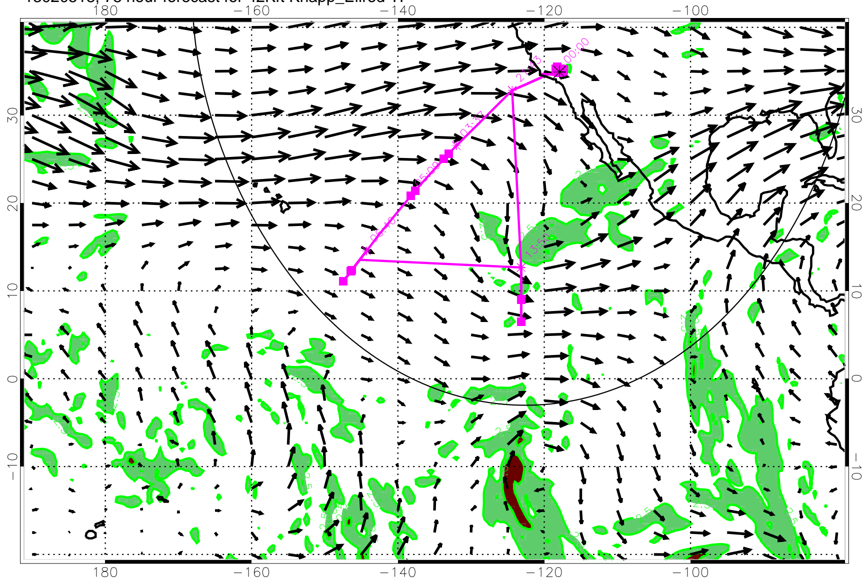
13020518, 78 hour forecast for 42Kft Knapp_Ellrod TI
