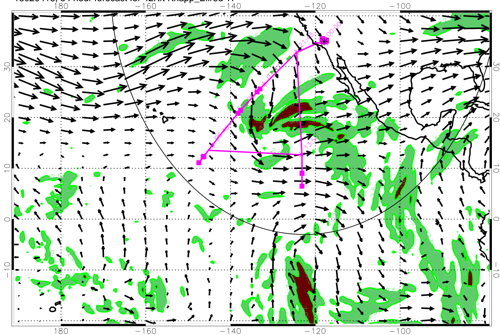
13020418, 54 hour forecast for 42Kft Knapp_Ellrod TI
