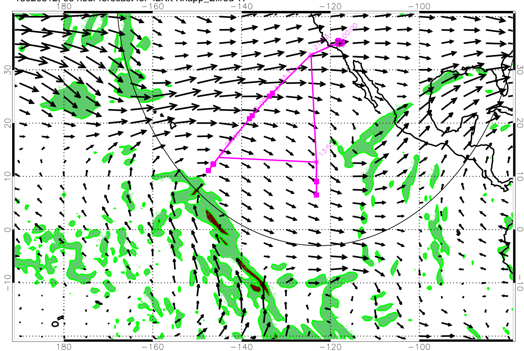
13020612, 96 hour forecast for 42Kft Knapp_Ellrod TI
