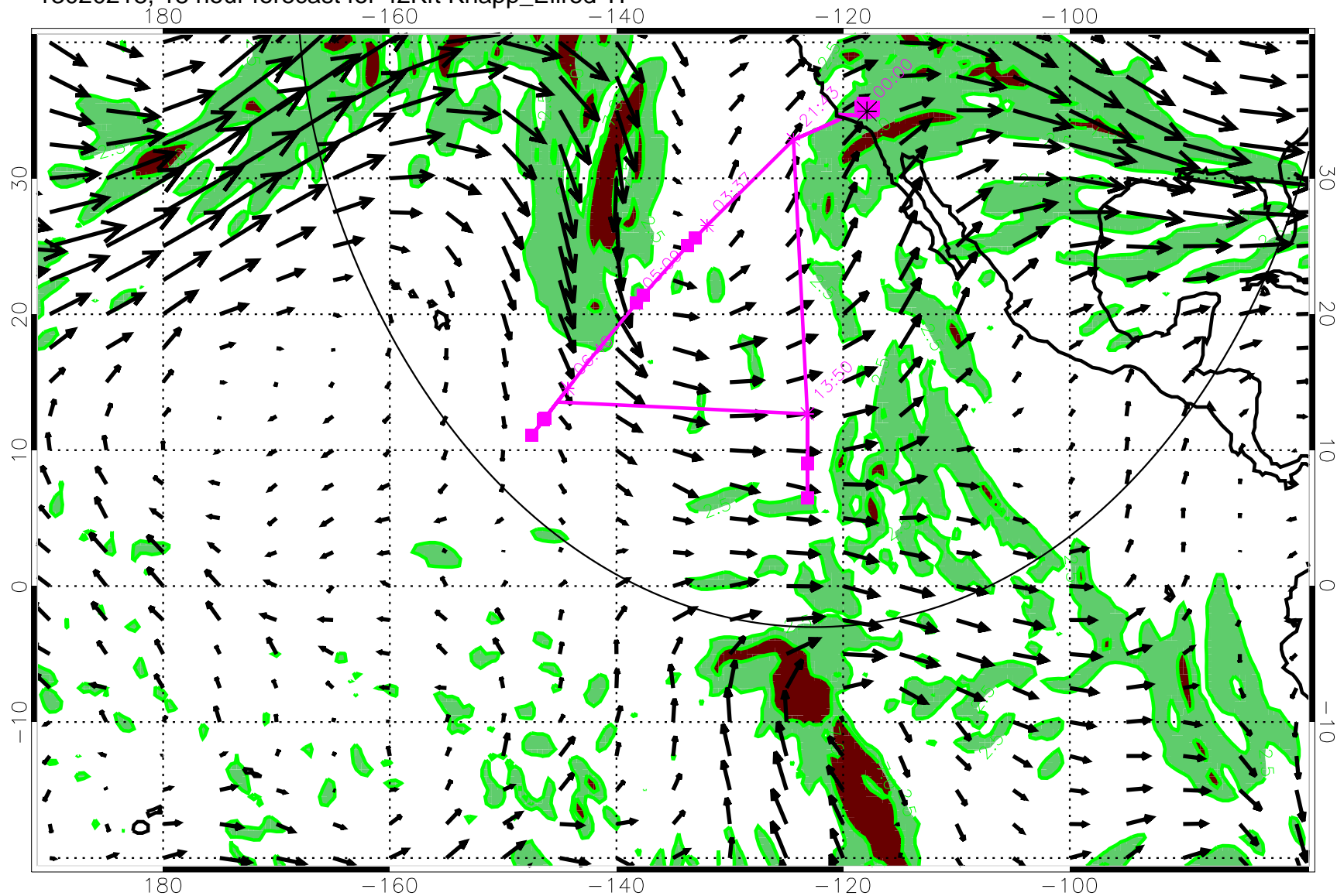
13020218, 18 hour forecast for 42Kft Knapp_Ellrod TI
