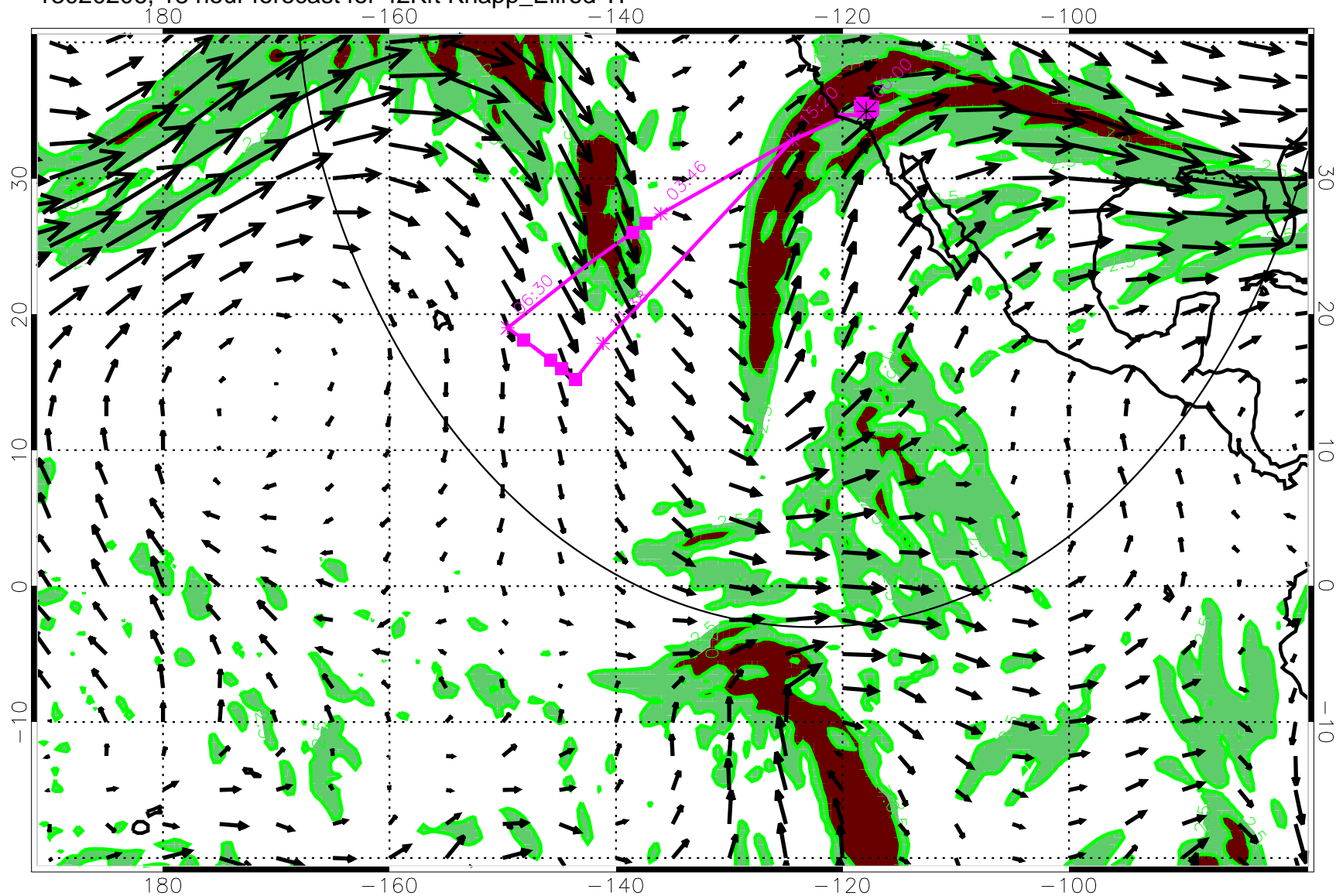
13020206, 18 hour forecast for 42Kft Knapp_Ellrod TI
