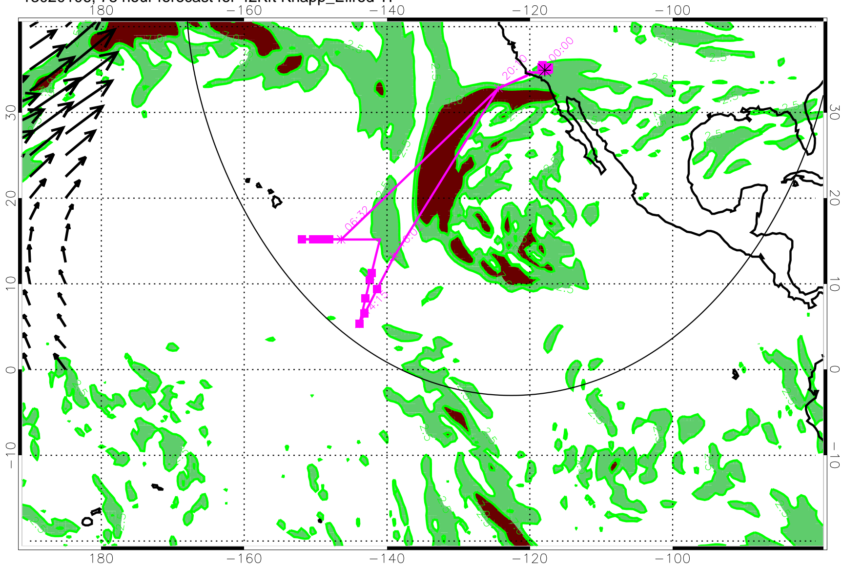
13020106, 78 hour forecast for 42Kft Knapp_Ellrod TI
