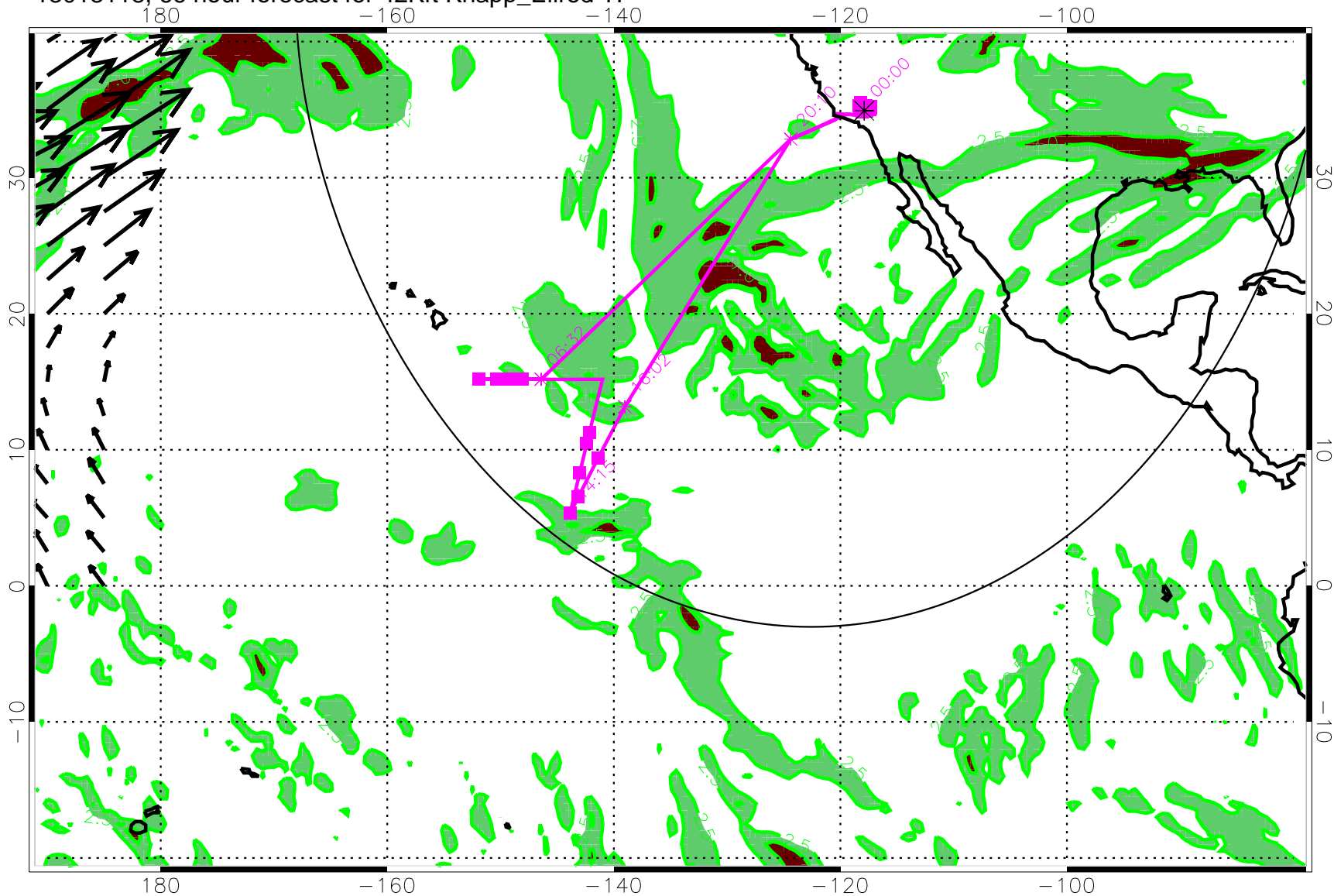
13013118, 66 hour forecast for 42Kft Knapp_Ellrod TI
