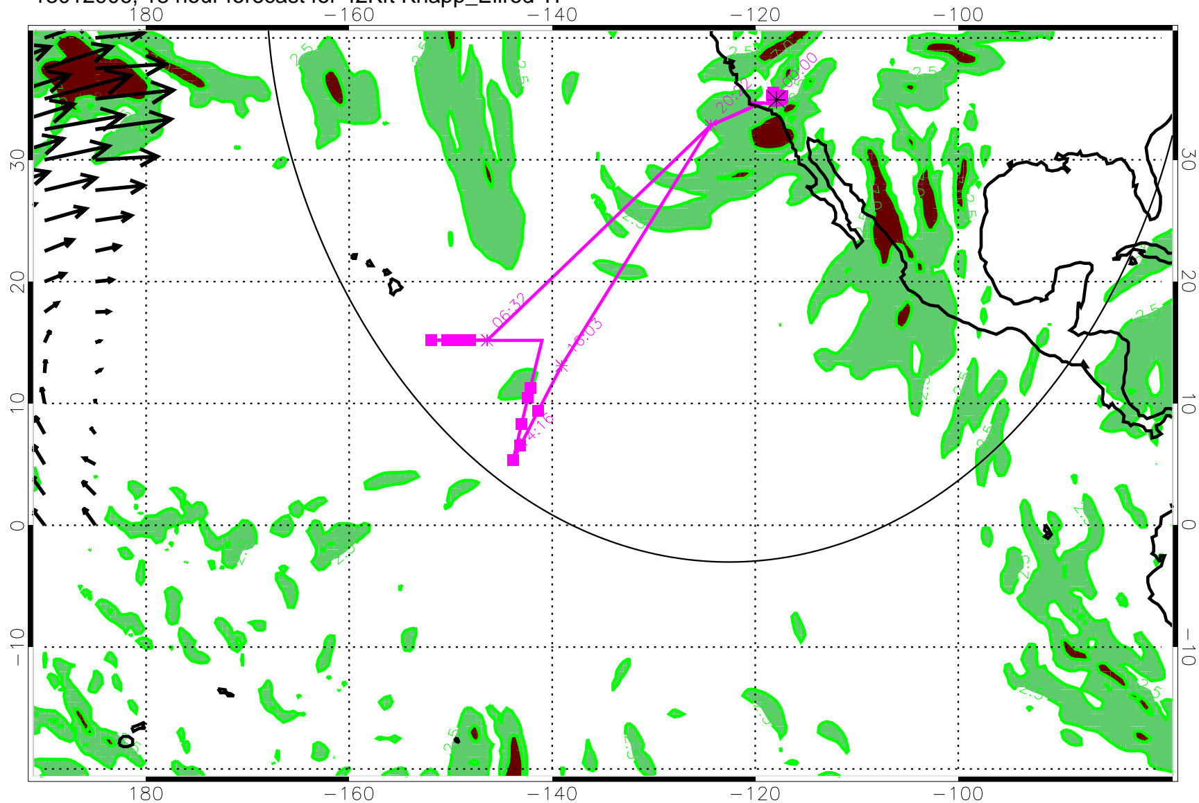
13012906, 18 hour forecast for 42Kft Knapp_Ellrod TI
