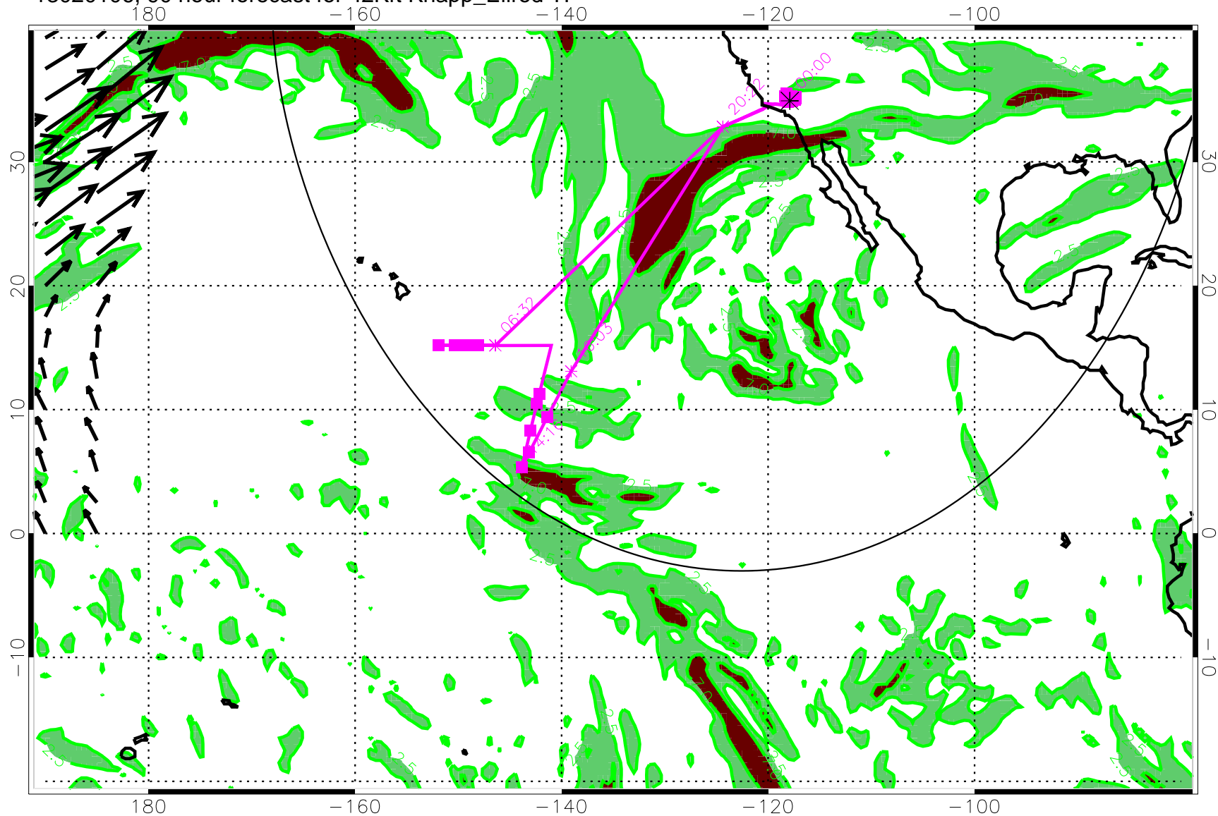
13020106, 90 hour forecast for 42Kft Knapp_Ellrod TI
