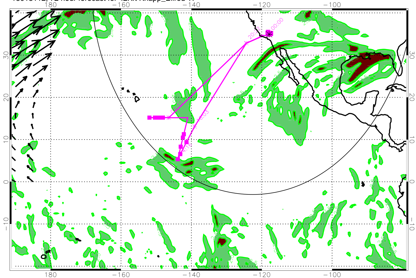
13013112, 72 hour forecast for 42Kft Knapp_Ellrod TI
