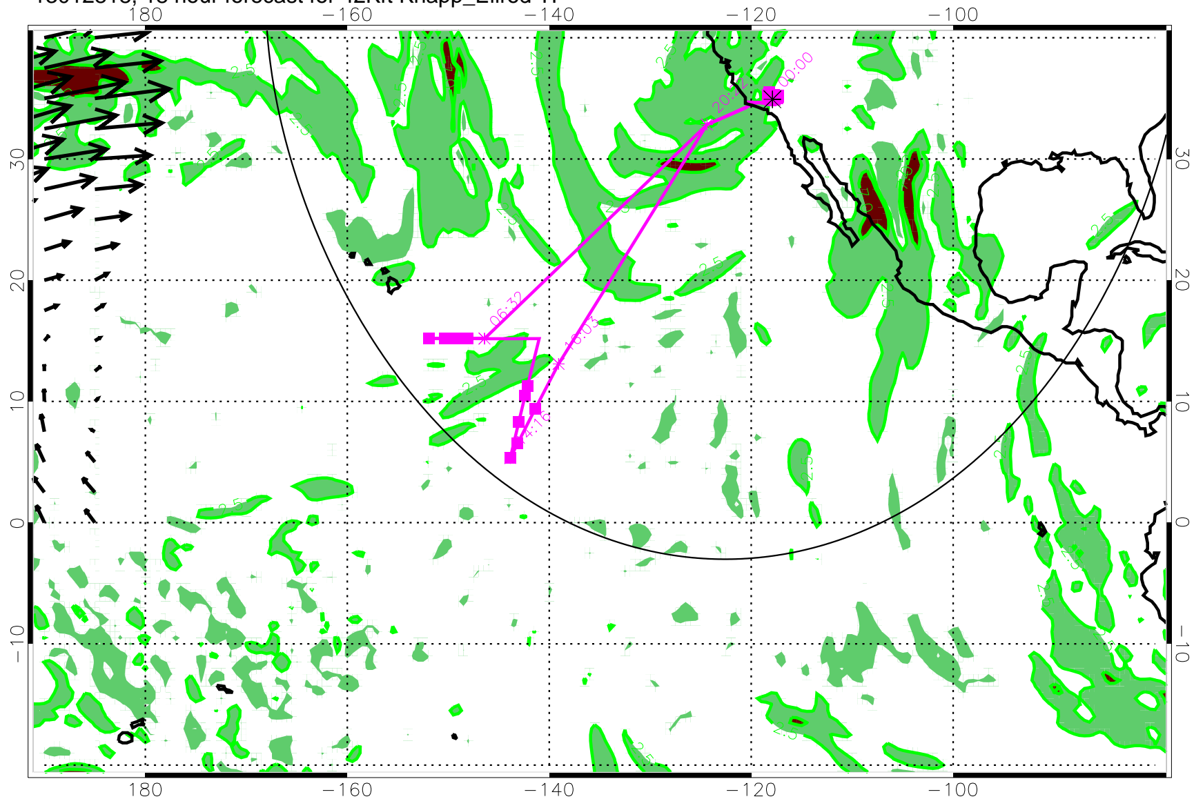
13012818, 18 hour forecast for 42Kft Knapp_Ellrod TI
