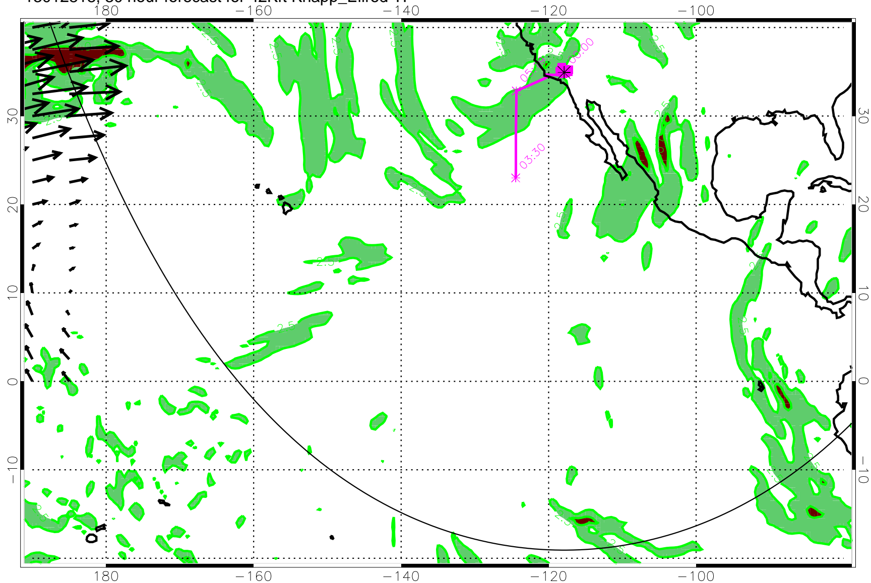
13012818, 30 hour forecast for 42Kft Knapp_Ellrod TI
