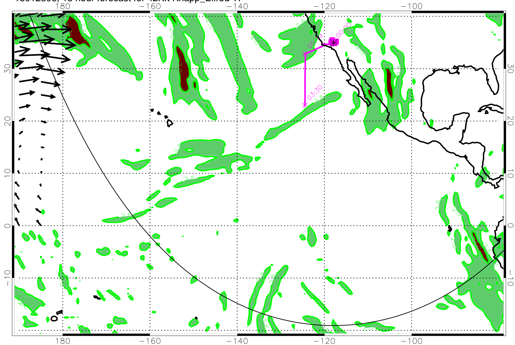
13012806, 18 hour forecast for 42Kft Knapp_Ellrod TI
