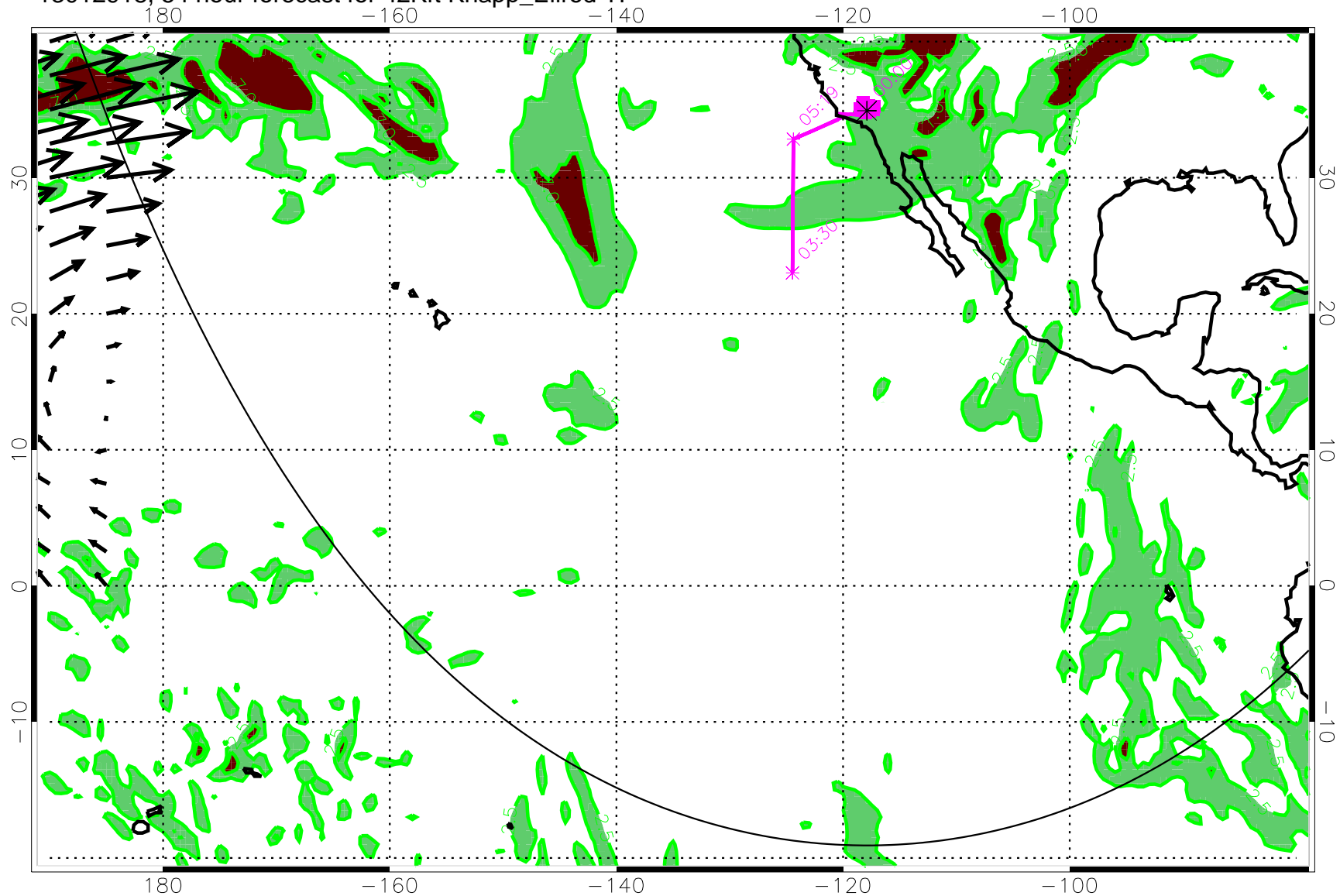
13012918, 54 hour forecast for 42Kft Knapp_Ellrod TI
