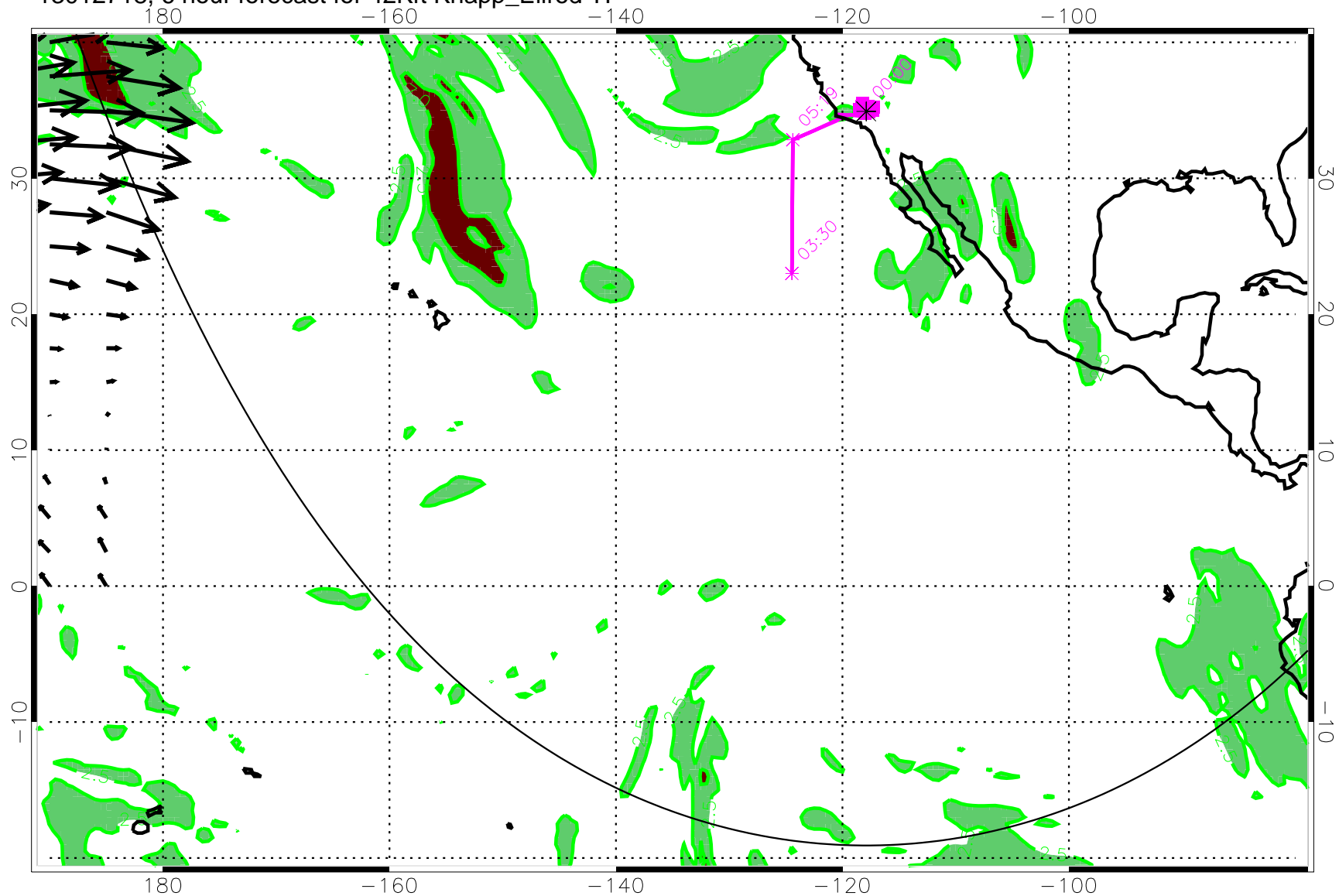
13012718, 6 hour forecast for 42Kft Knapp_Ellrod TI
