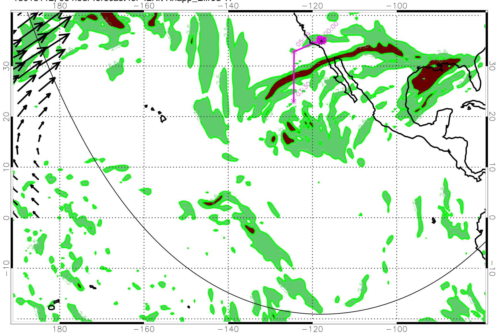
13013112, 96 hour forecast for 42Kft Knapp_Ellrod TI
