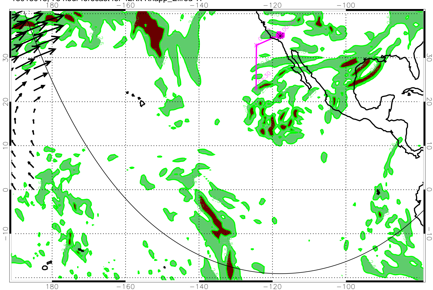
13013018, 78 hour forecast for 42Kft Knapp_Ellrod TI
