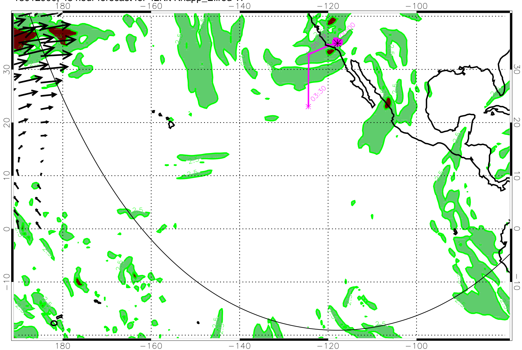
13012900, 48 hour forecast for 42Kft Knapp_Ellrod TI
