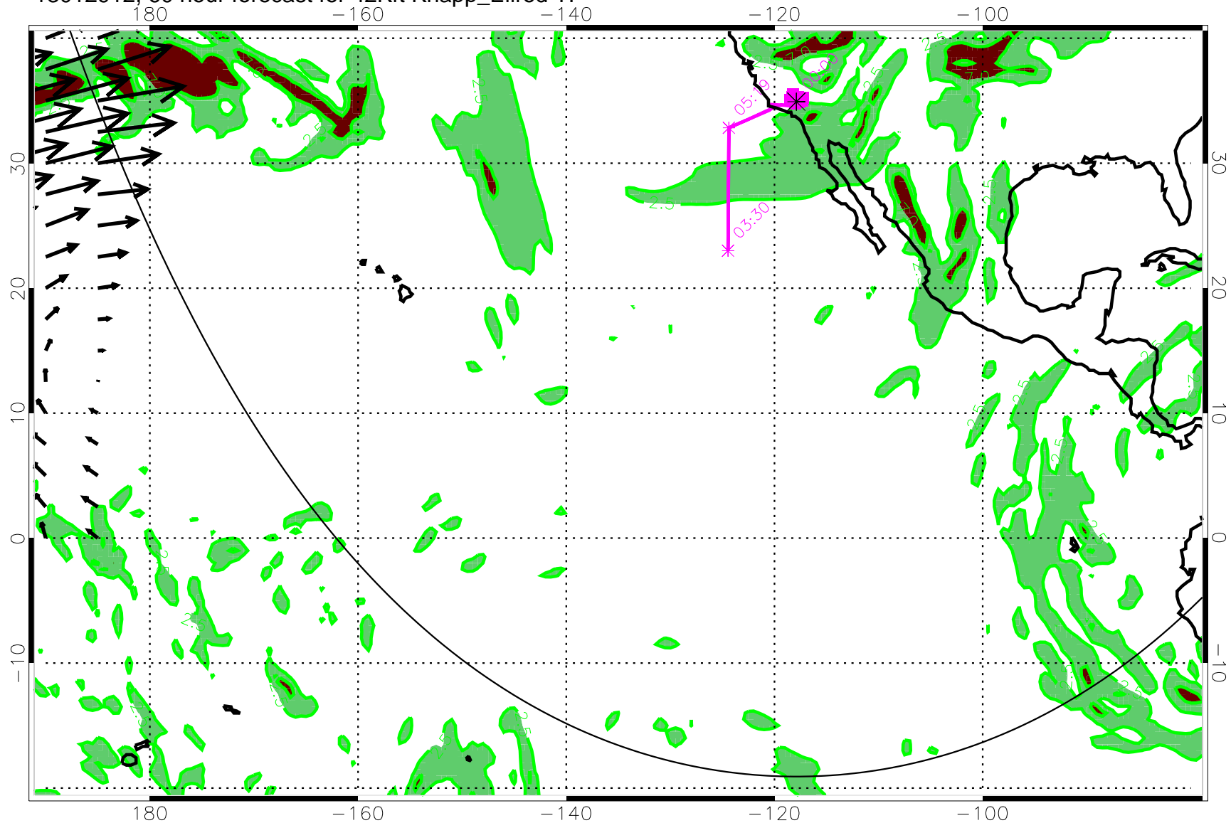
13012912, 60 hour forecast for 42Kft Knapp_Ellrod TI
