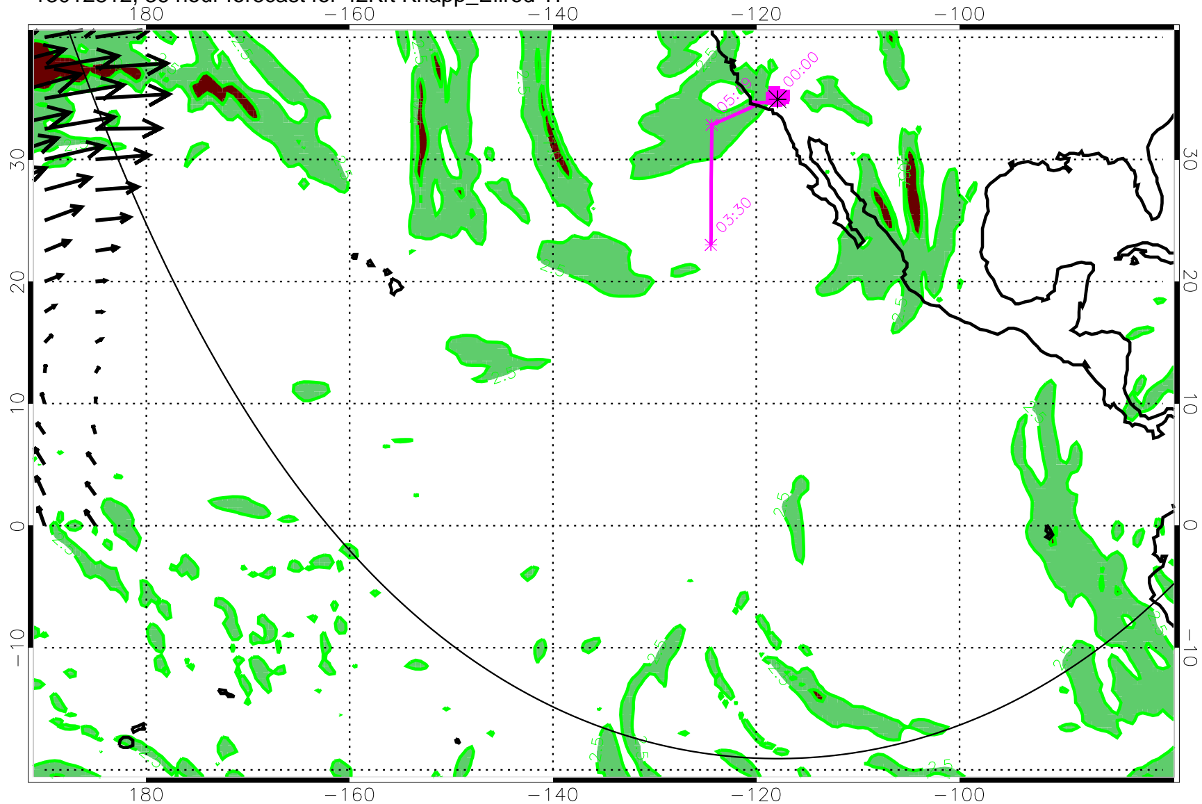
13012812, 36 hour forecast for 42Kft Knapp_Ellrod TI
