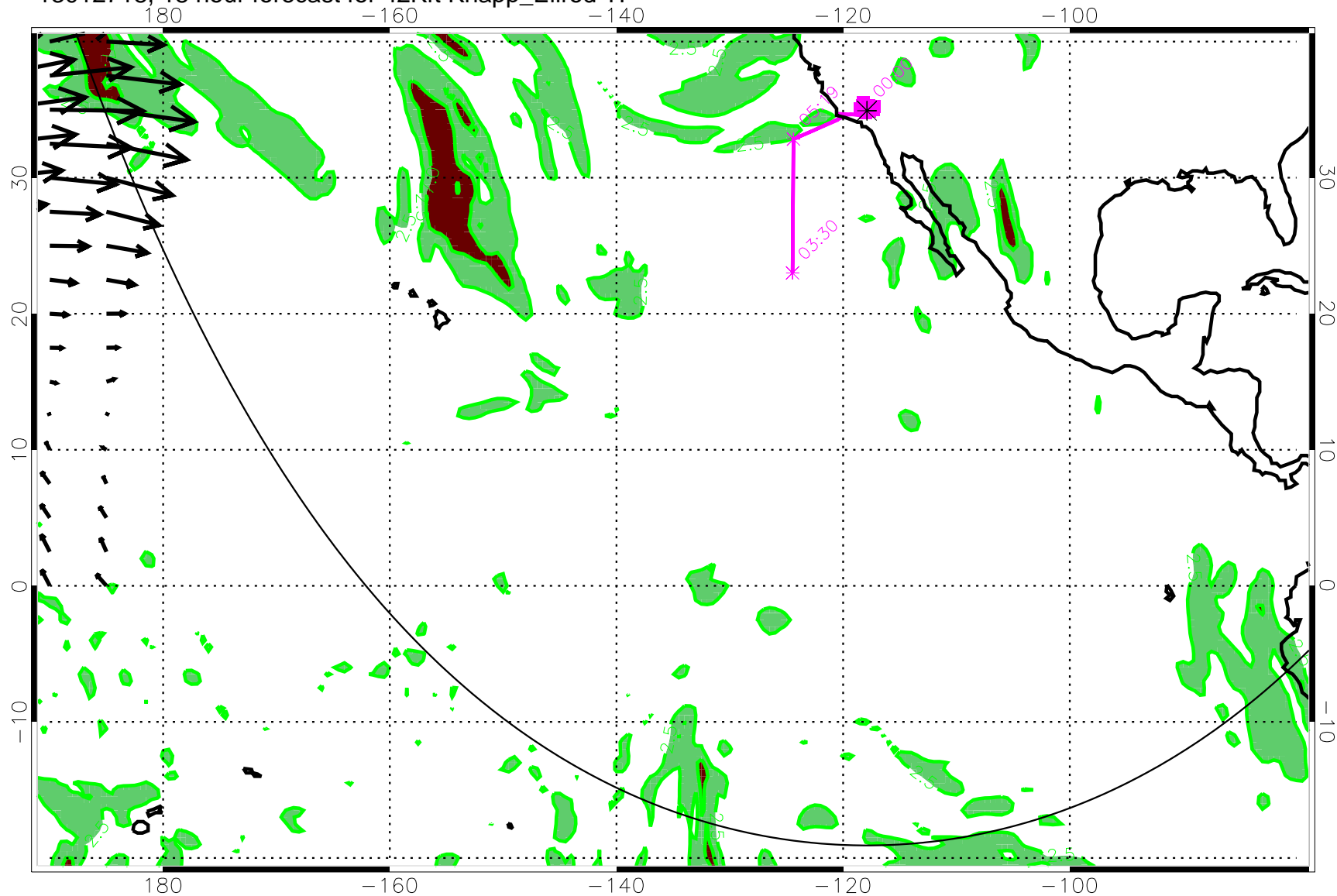
13012718, 18 hour forecast for 42Kft Knapp_Ellrod TI
