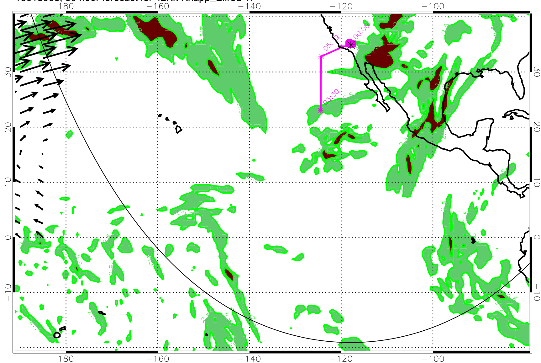
13013006, 90 hour forecast for 42Kft Knapp_Ellrod TI
