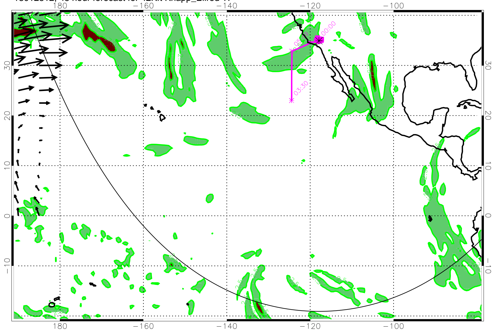
13012812, 48 hour forecast for 42Kft Knapp_Ellrod TI
