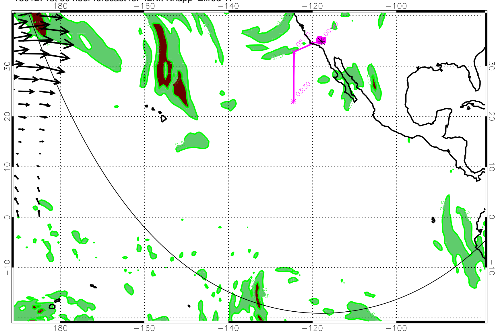
13012718, 30 hour forecast for 42Kft Knapp_Ellrod TI
