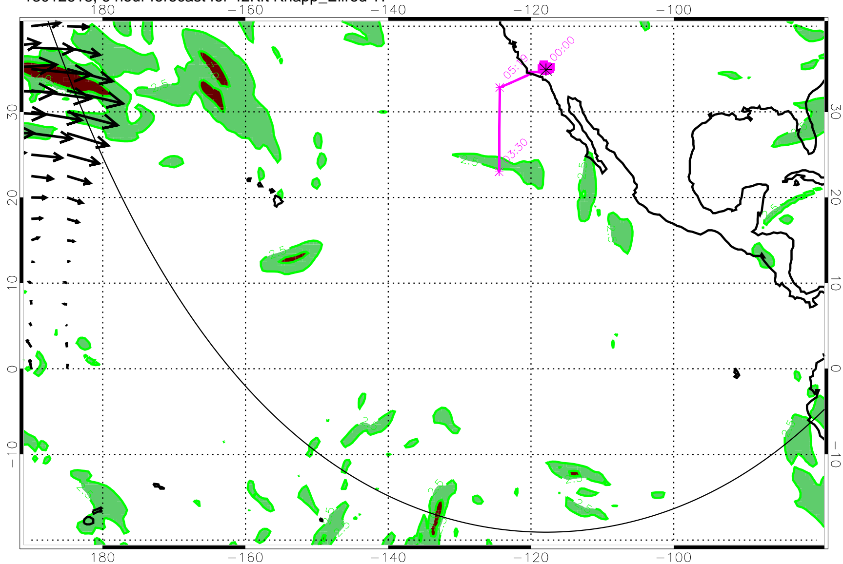
13012618, 6 hour forecast for 42Kft Knapp_Ellrod TI
