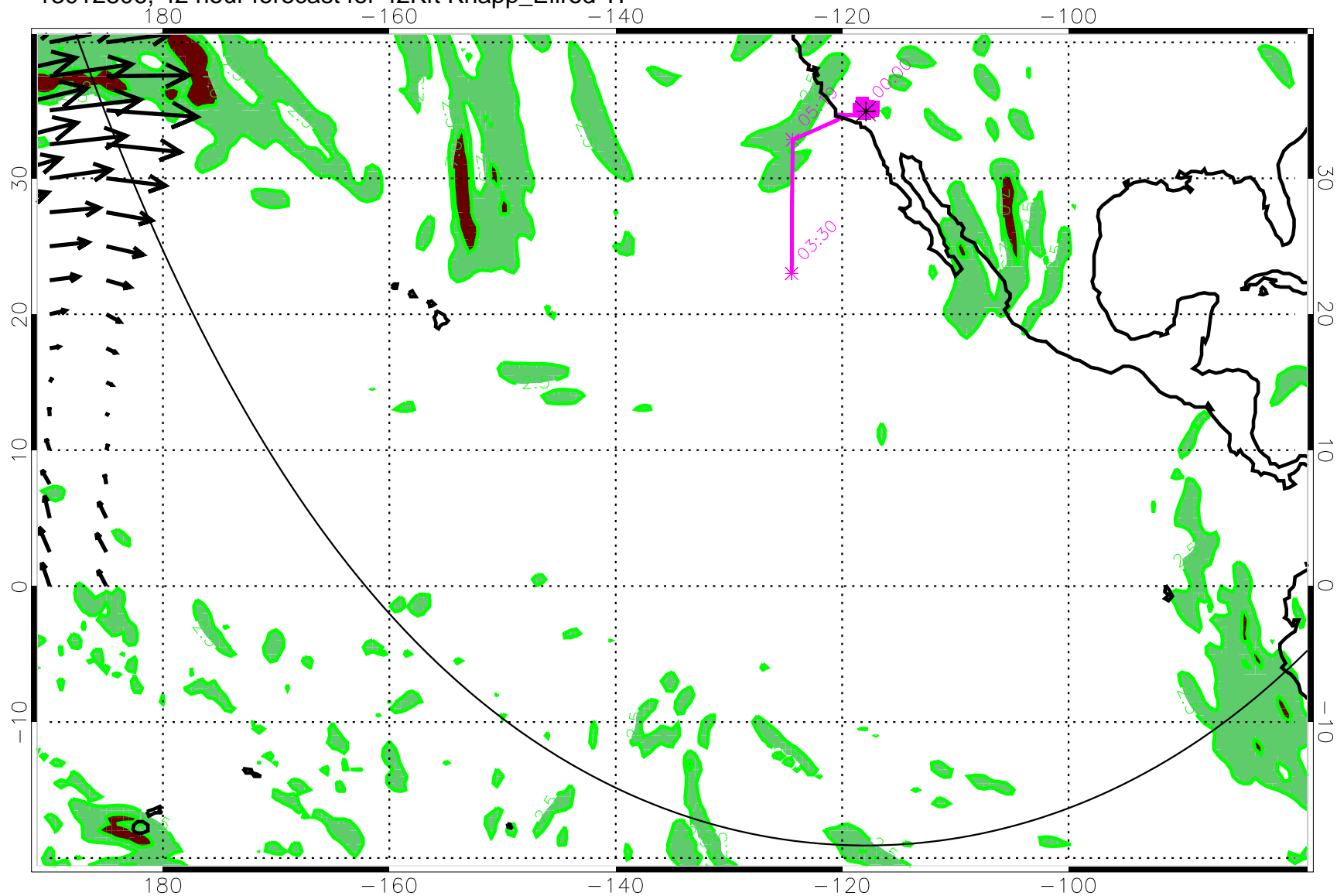
13012806, 42 hour forecast for 42Kft Knapp_Ellrod TI
