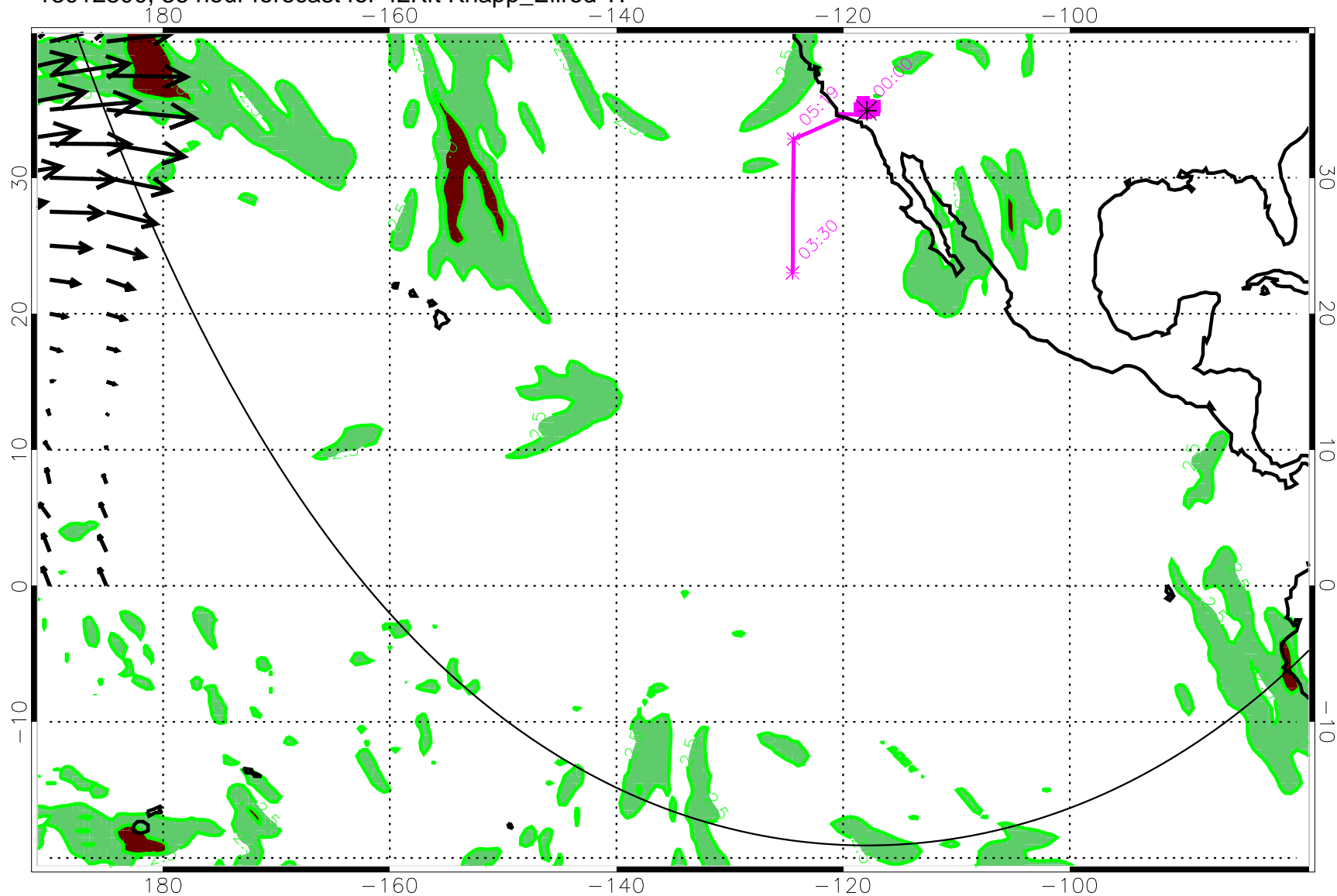
13012800, 36 hour forecast for 42Kft Knapp_Ellrod TI
