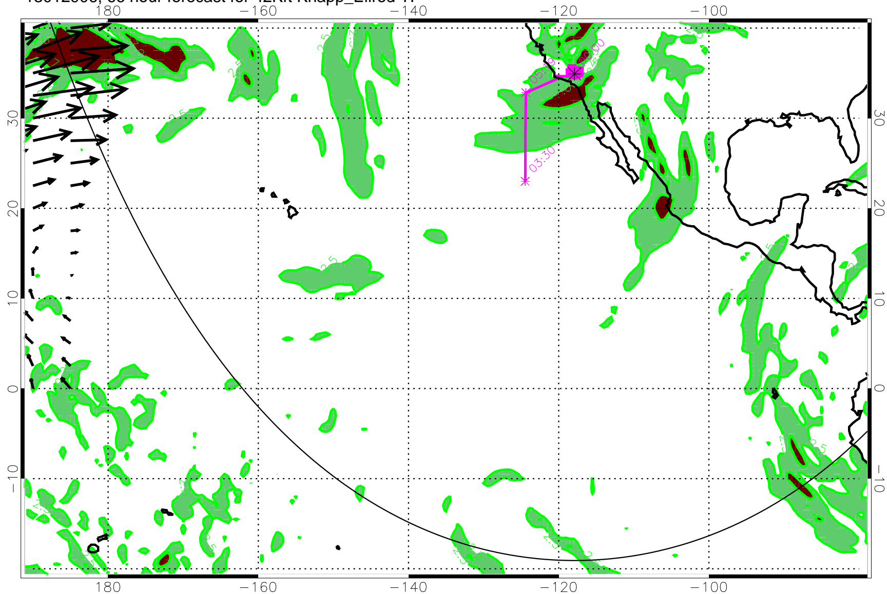
13012906, 66 hour forecast for 42Kft Knapp_Ellrod TI
