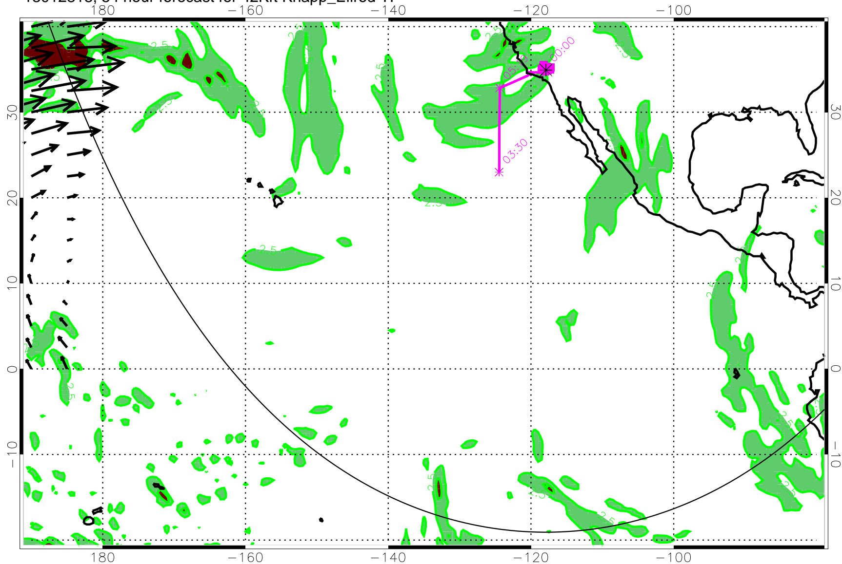
13012818, 54 hour forecast for 42Kft Knapp_Ellrod TI
