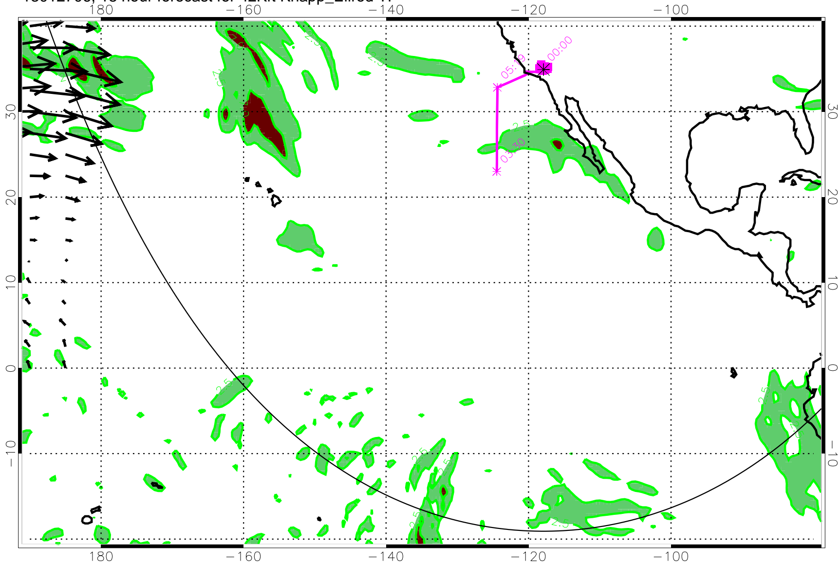
13012706, 18 hour forecast for 42Kft Knapp_Ellrod TI
