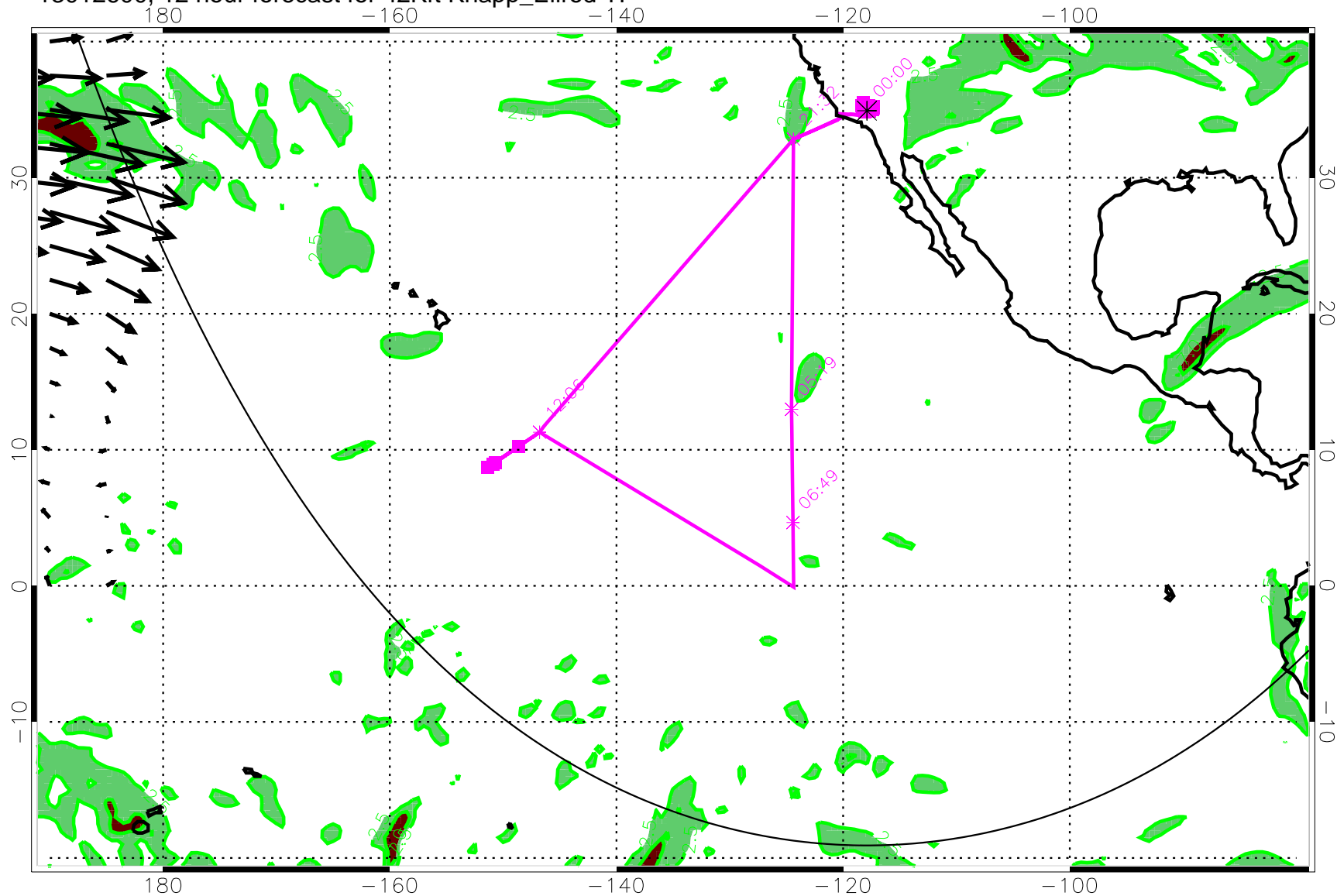
13012600, 12 hour forecast for 42Kft Knapp_Ellrod TI
