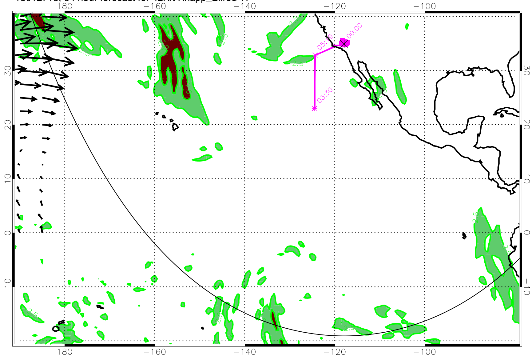
13012718, 54 hour forecast for 42Kft Knapp_Ellrod TI
