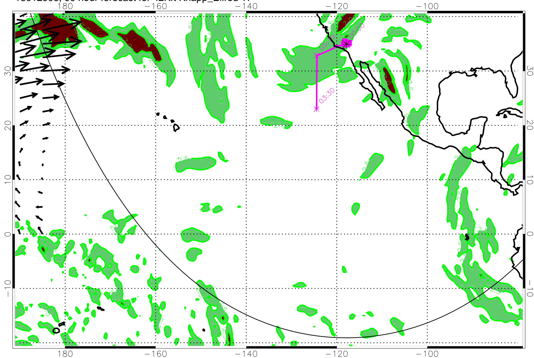
13012906, 90 hour forecast for 42Kft Knapp_Ellrod TI
