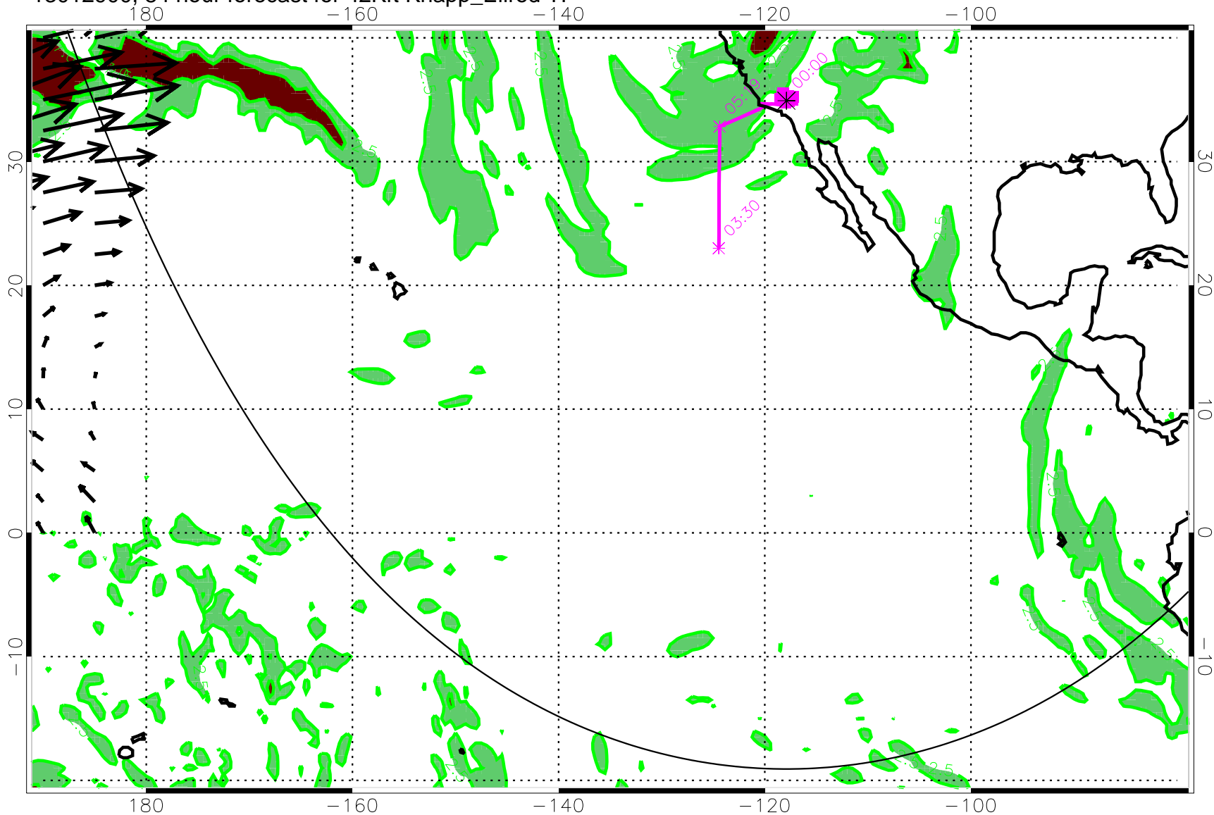
13012900, 84 hour forecast for 42Kft Knapp_Ellrod TI
