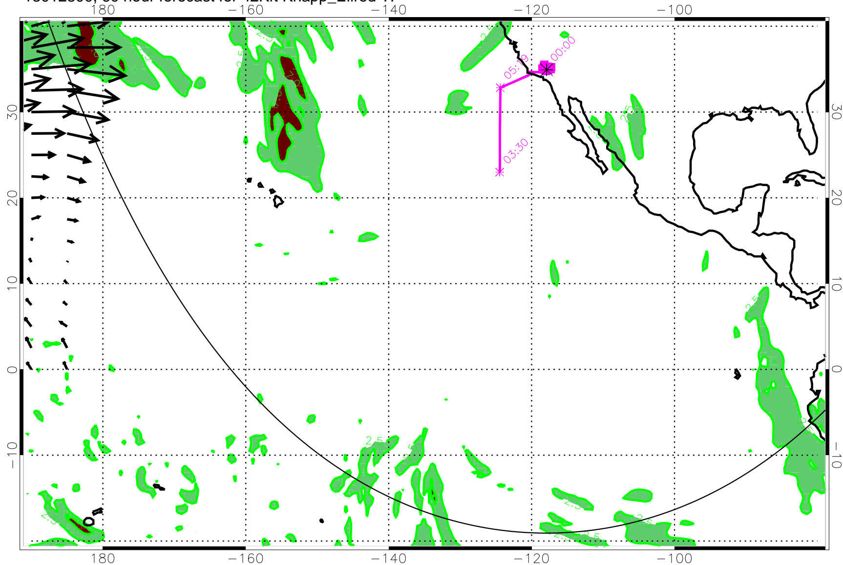
13012800, 60 hour forecast for 42Kft Knapp_Ellrod TI
