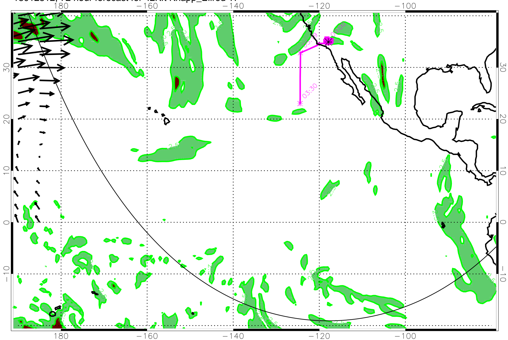
13012812, 72 hour forecast for 42Kft Knapp_Ellrod TI
