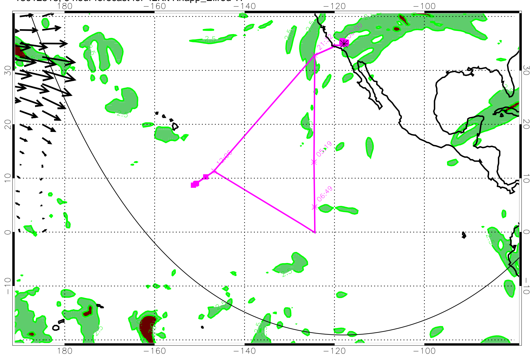
13012518, 6 hour forecast for 42Kft Knapp_Ellrod TI
