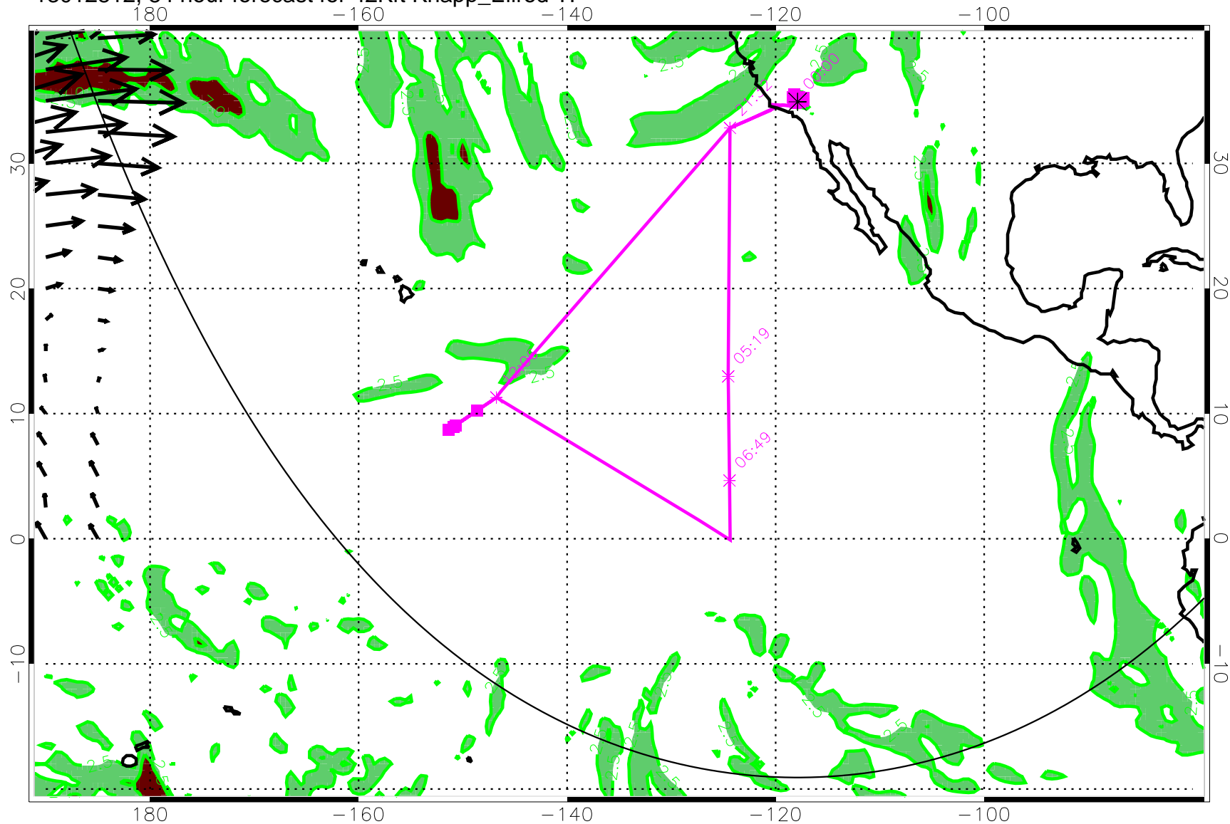
13012812, 84 hour forecast for 42Kft Knapp_Ellrod TI
