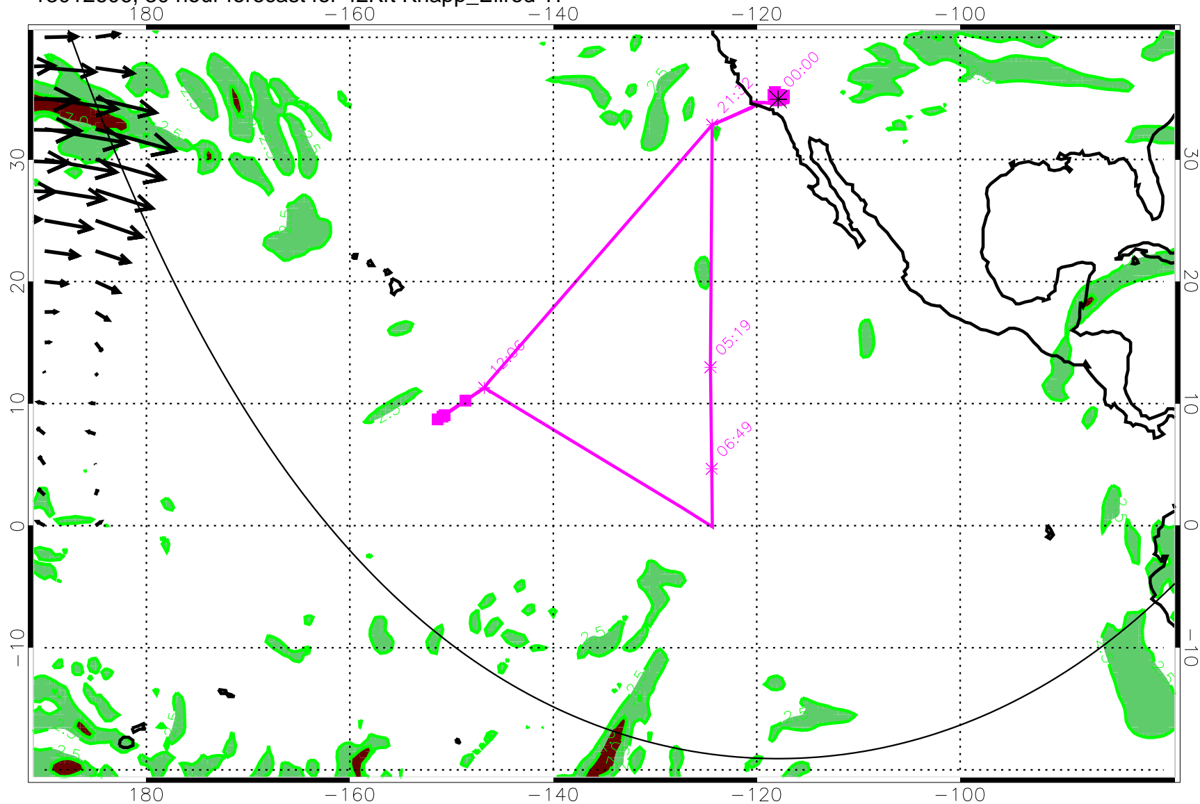
13012606, 30 hour forecast for 42Kft Knapp_Ellrod TI
