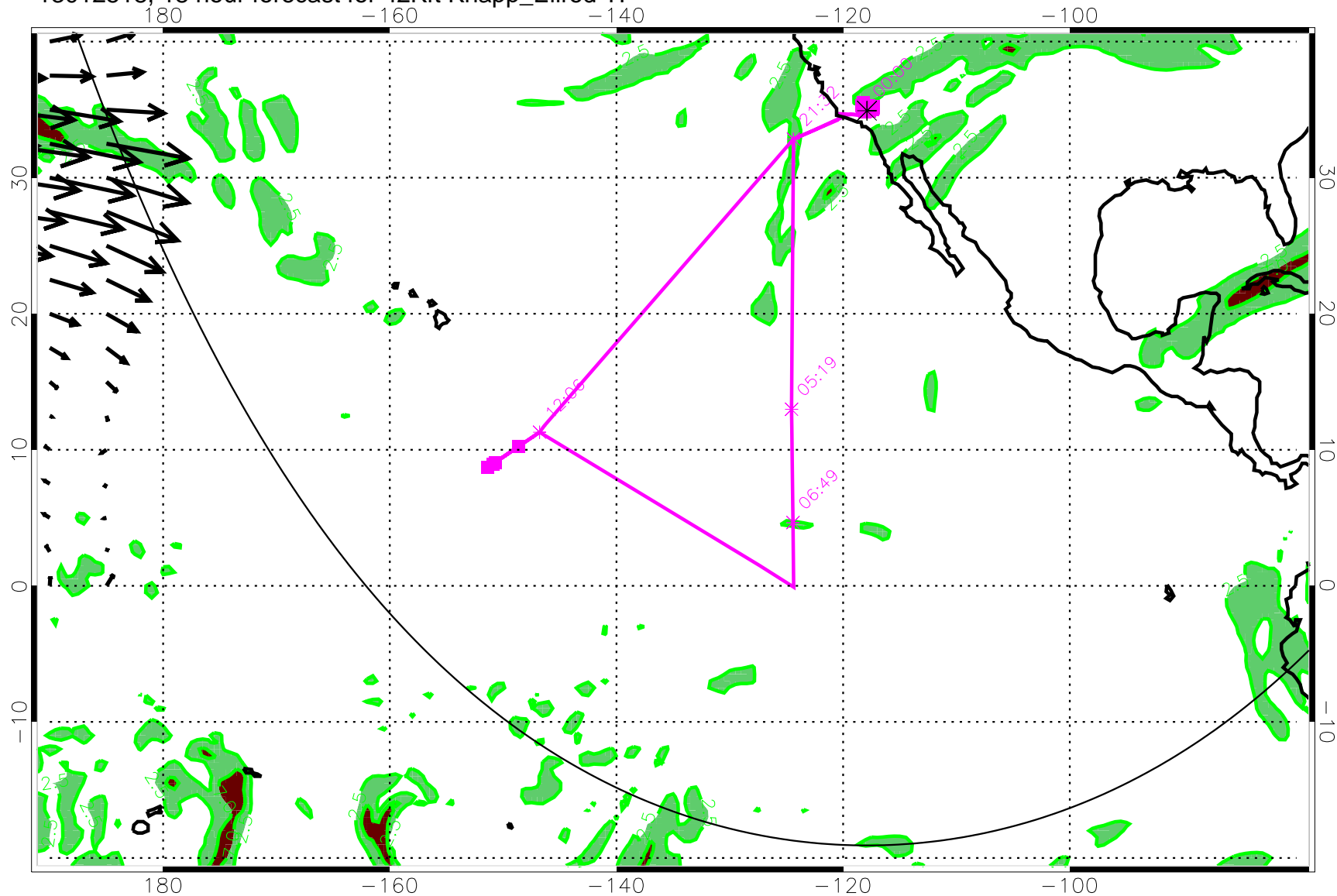
13012518, 18 hour forecast for 42Kft Knapp_Ellrod TI
