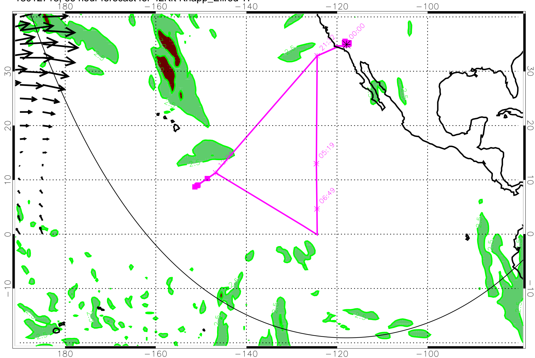
13012718, 66 hour forecast for 42Kft Knapp_Ellrod TI
