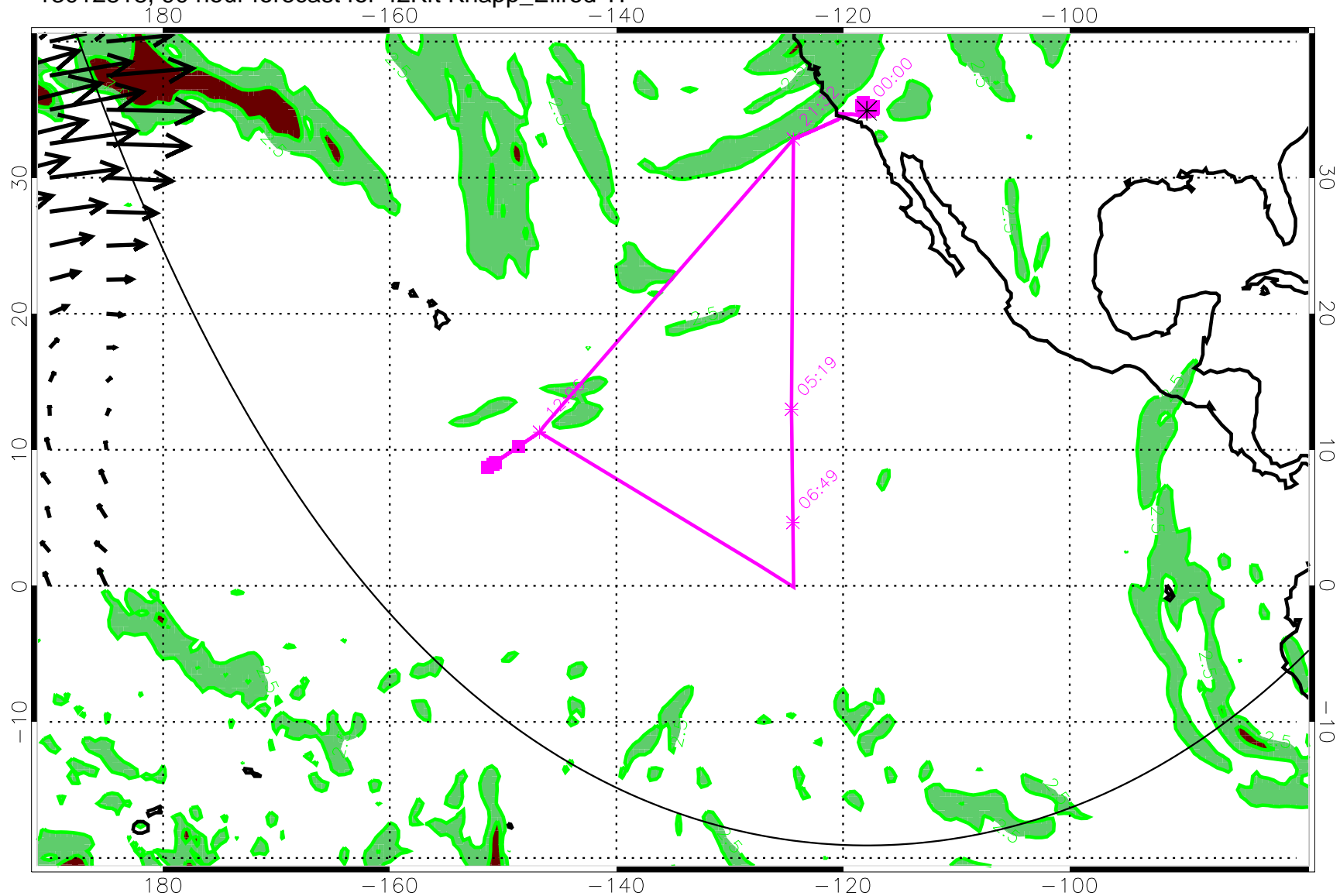
13012818, 90 hour forecast for 42Kft Knapp_Ellrod TI
