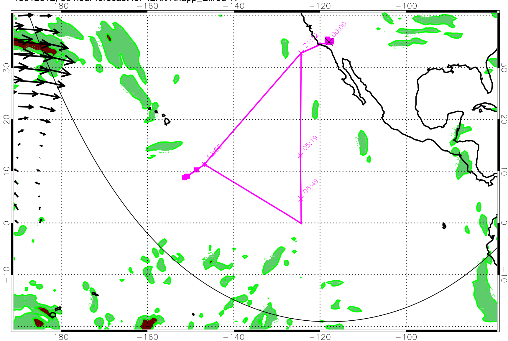
13012612, 36 hour forecast for 42Kft Knapp_Ellrod TI
