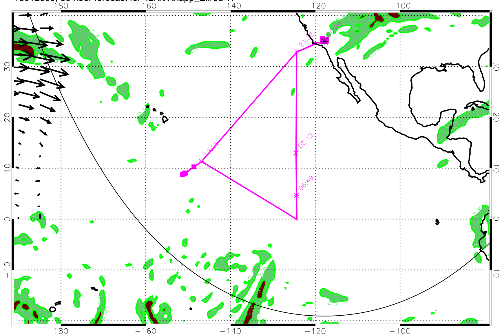
13012600, 36 hour forecast for 42Kft Knapp_Ellrod TI
