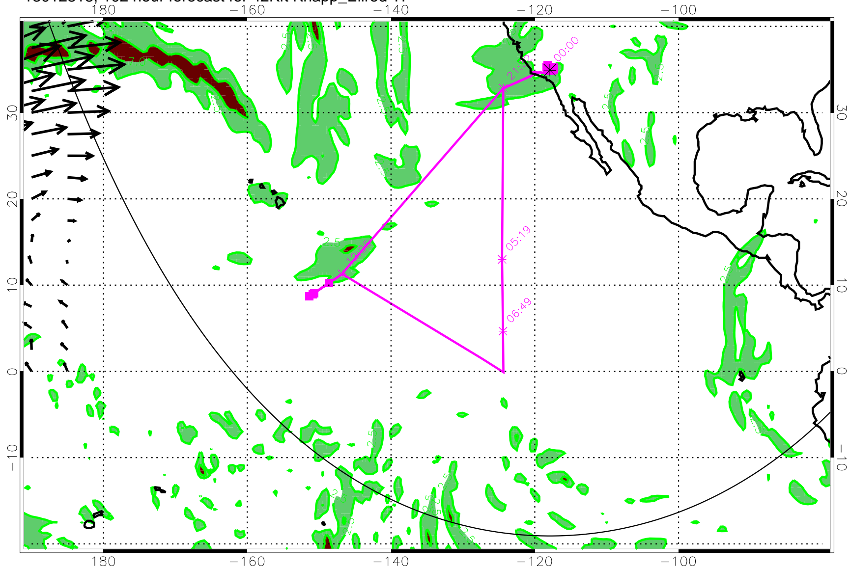
13012818, 102 hour forecast for 42Kft Knapp_Ellrod TI
