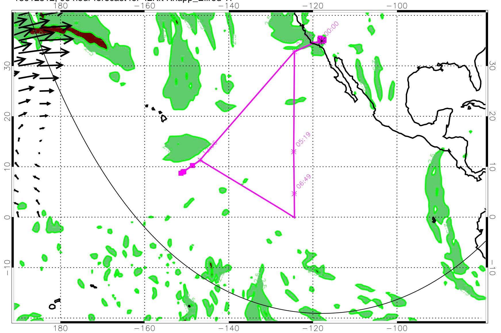
13012812, 96 hour forecast for 42Kft Knapp_Ellrod TI
