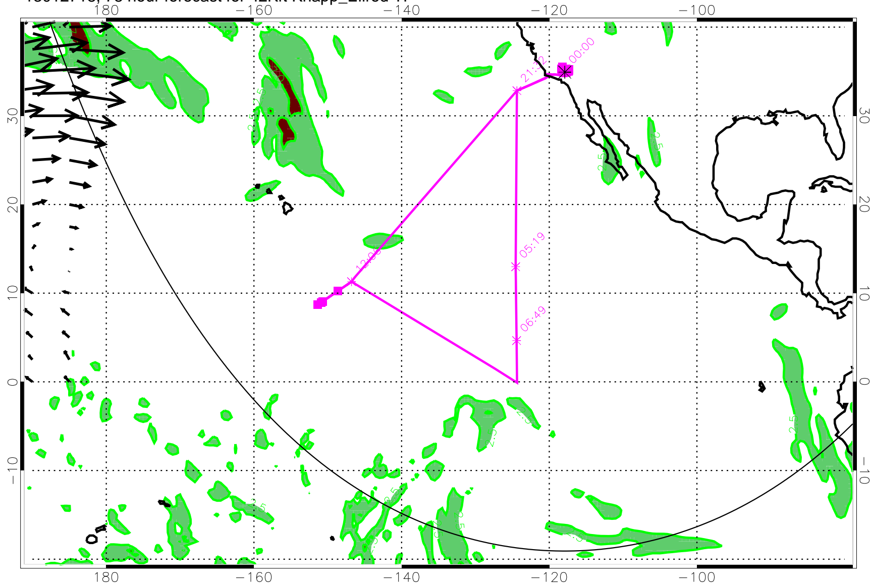
13012718, 78 hour forecast for 42Kft Knapp_Ellrod TI
