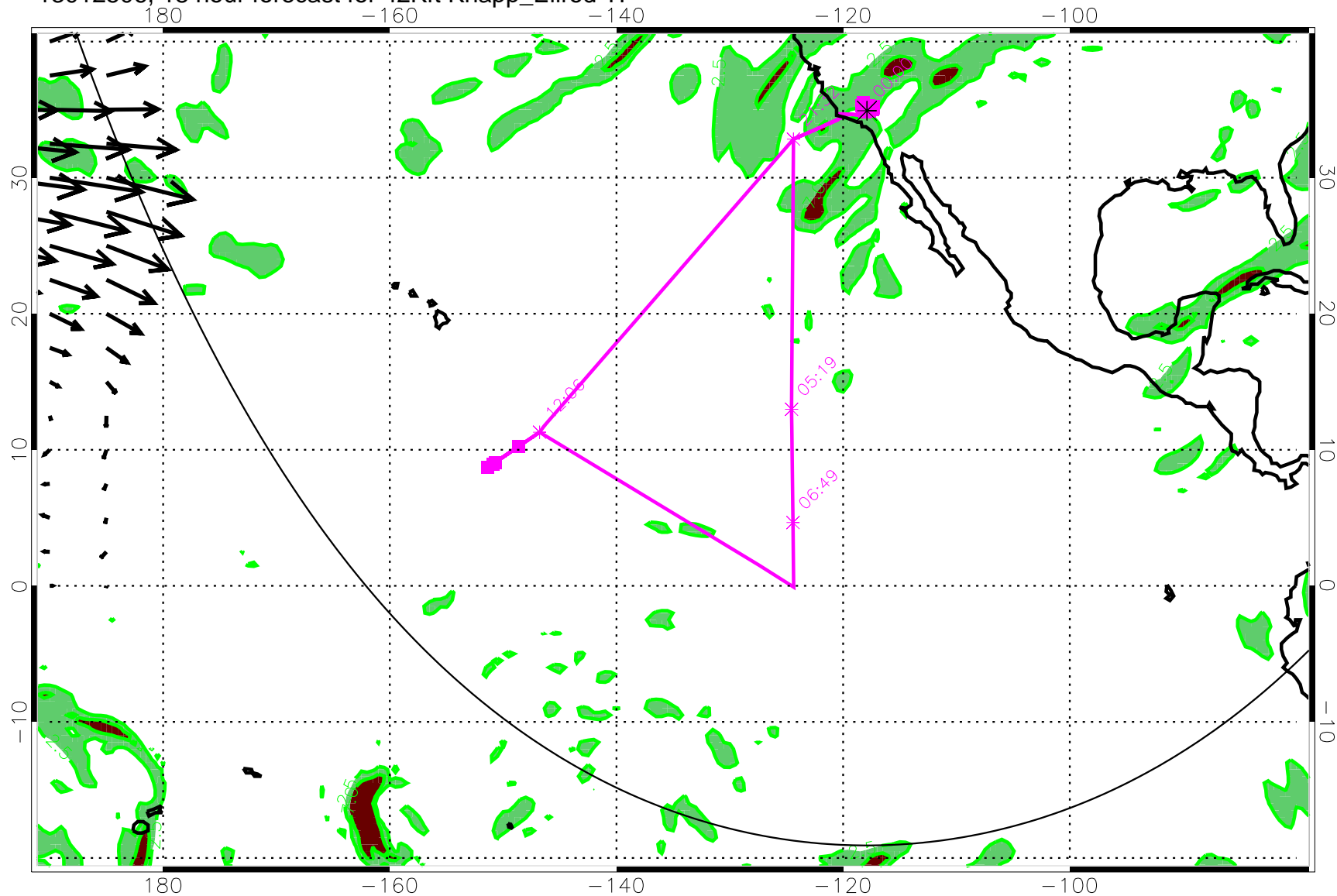
13012506, 18 hour forecast for 42Kft Knapp_Ellrod TI
