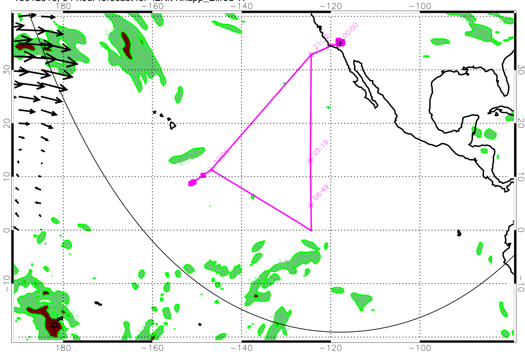
13012618, 54 hour forecast for 42Kft Knapp_Ellrod TI
