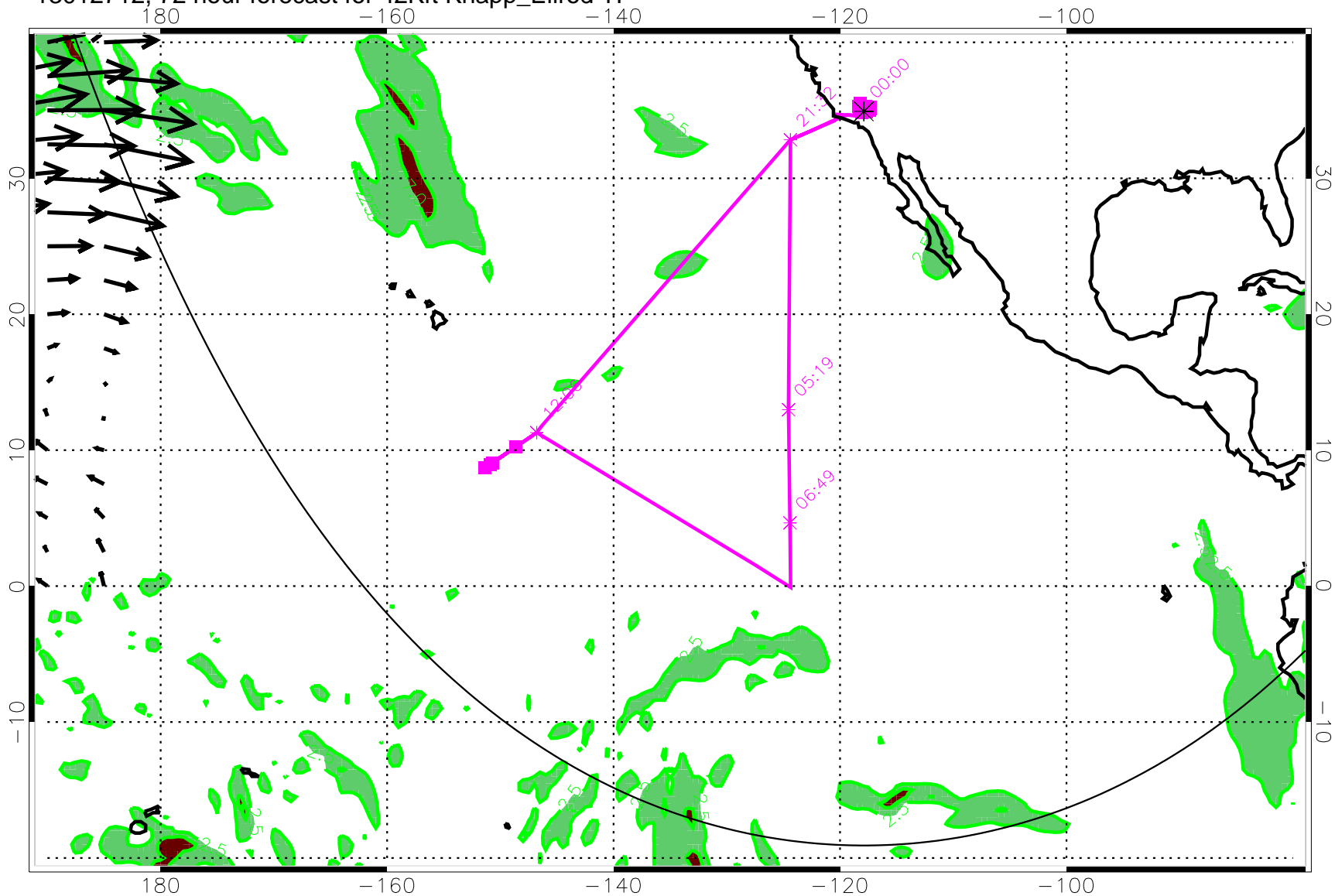
13012712, 72 hour forecast for 42Kft Knapp_Ellrod TI
