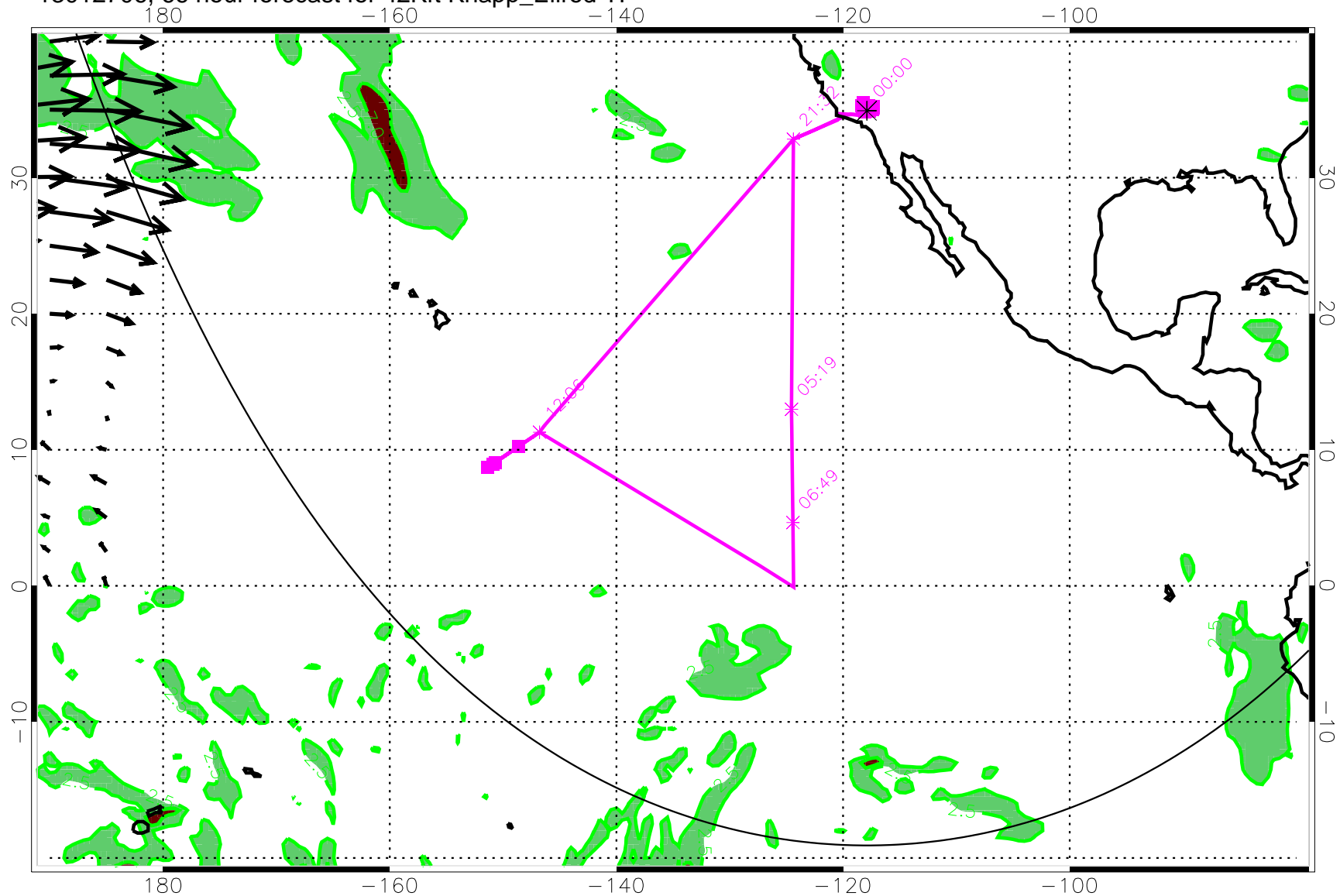
13012706, 66 hour forecast for 42Kft Knapp_Ellrod TI
