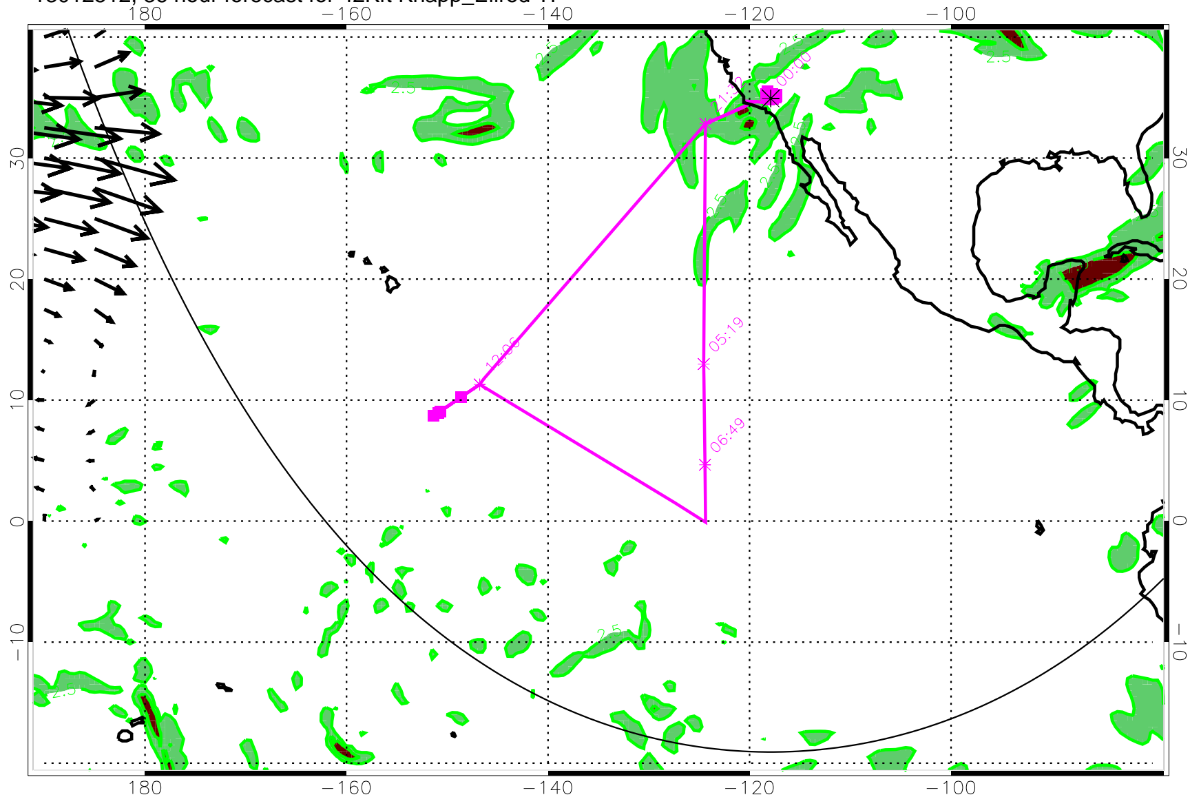
13012512, 36 hour forecast for 42Kft Knapp_Ellrod TI
