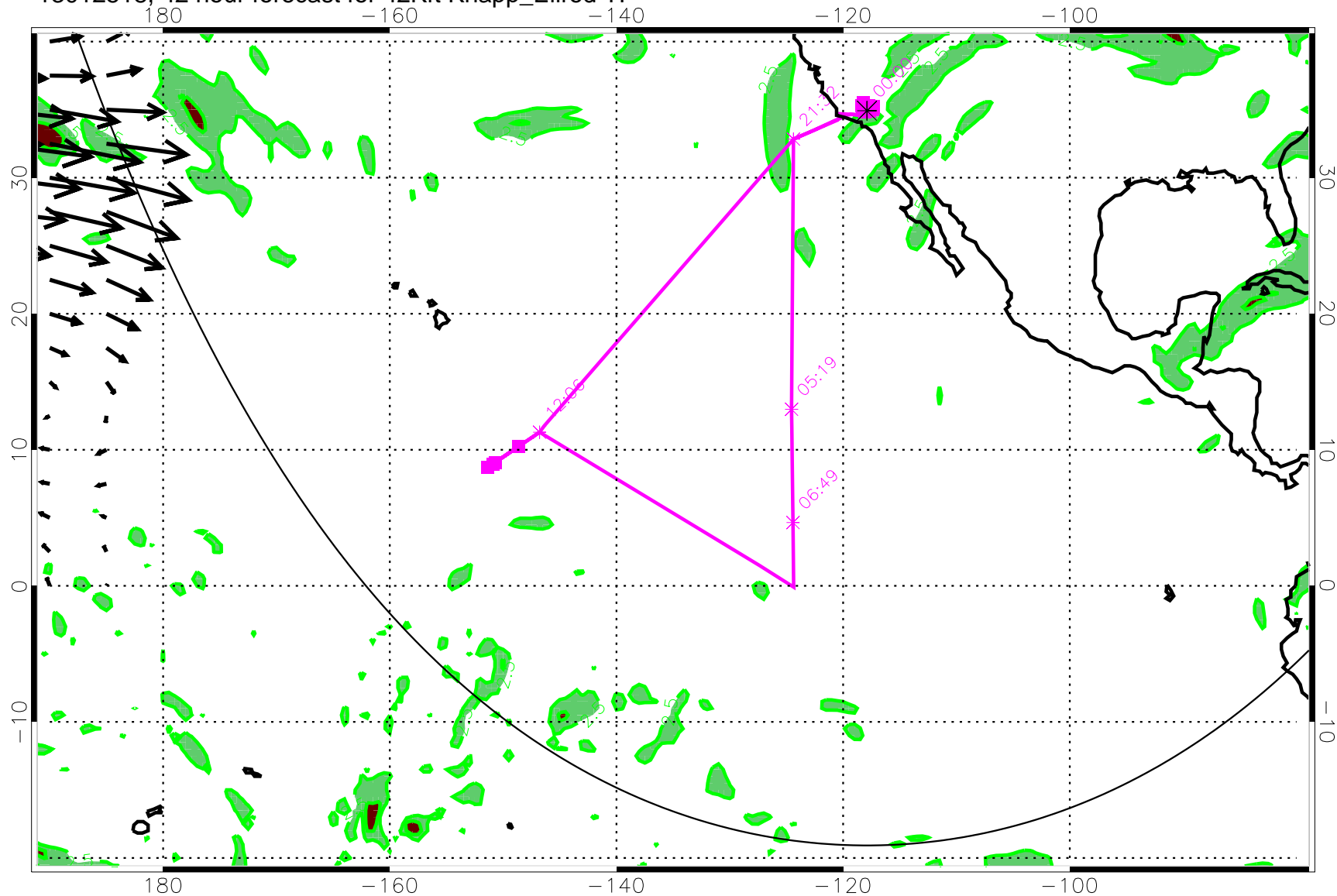
13012518, 42 hour forecast for 42Kft Knapp_Ellrod TI
