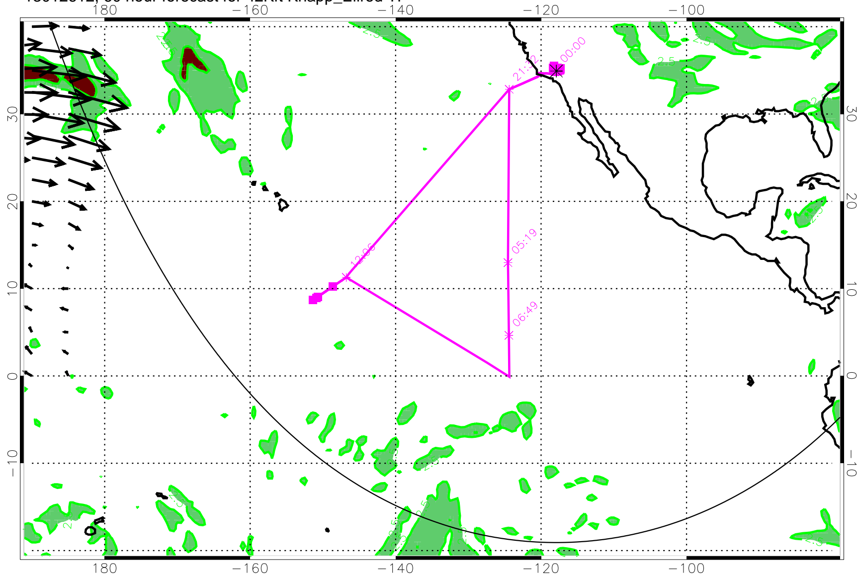
13012612, 60 hour forecast for 42Kft Knapp_Ellrod TI
