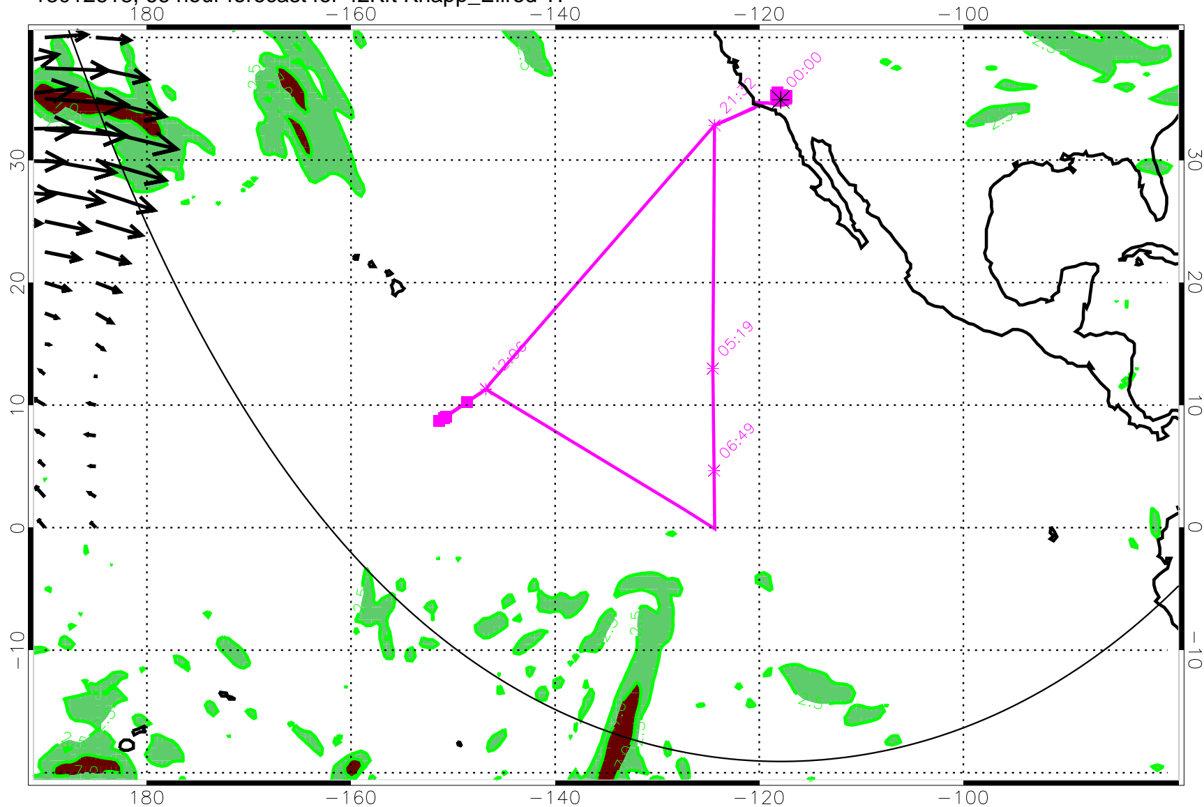
13012618, 66 hour forecast for 42Kft Knapp_Ellrod TI
