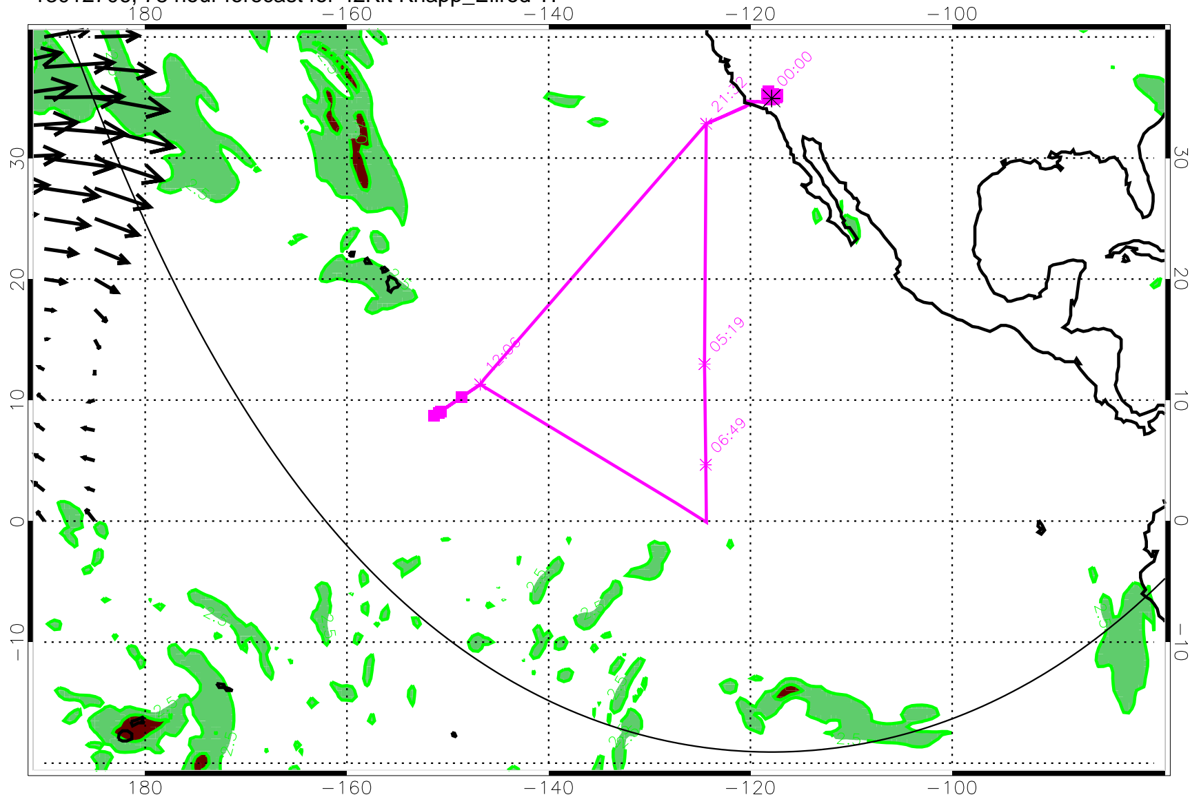
13012706, 78 hour forecast for 42Kft Knapp_Ellrod TI
