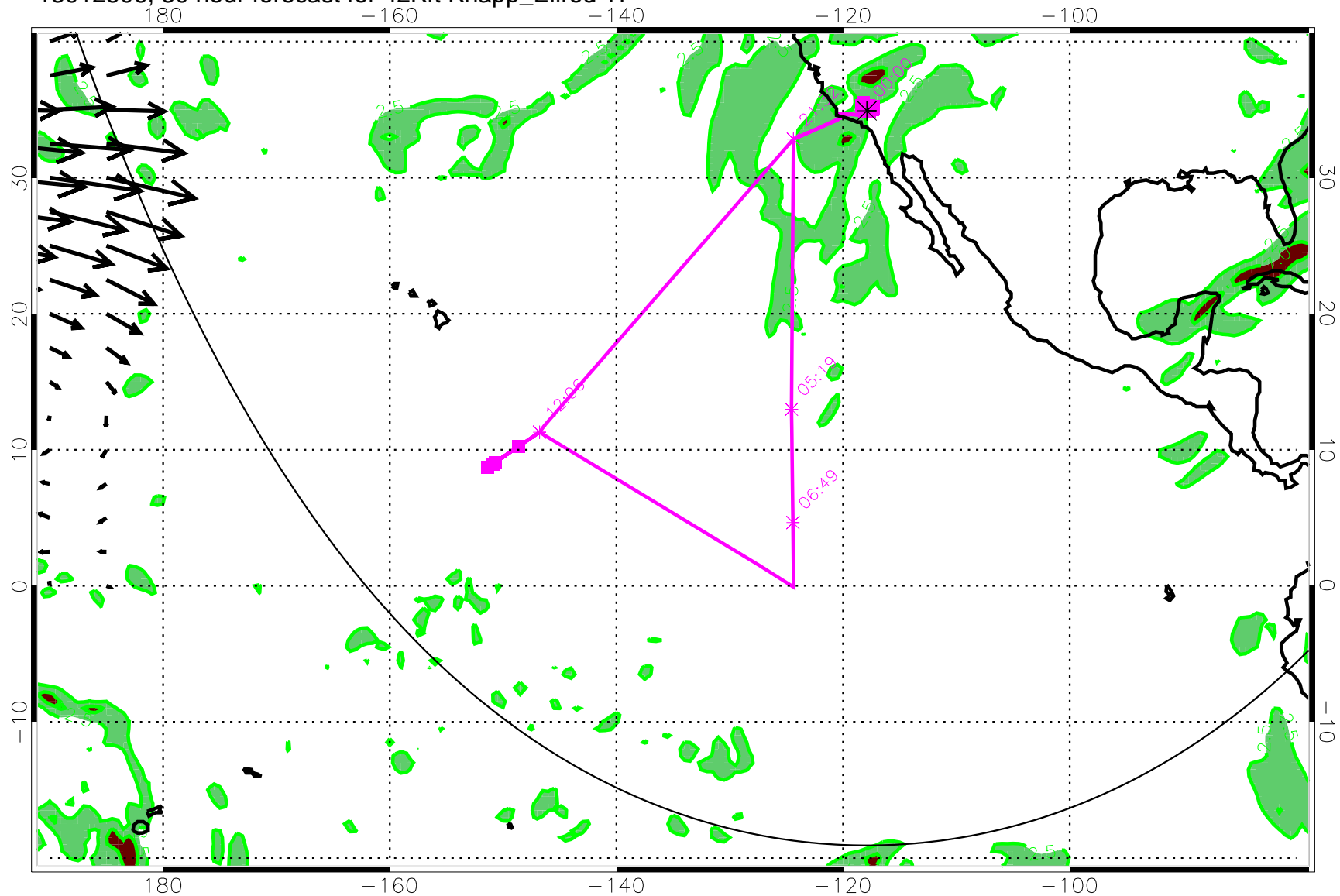
13012506, 30 hour forecast for 42Kft Knapp_Ellrod TI
