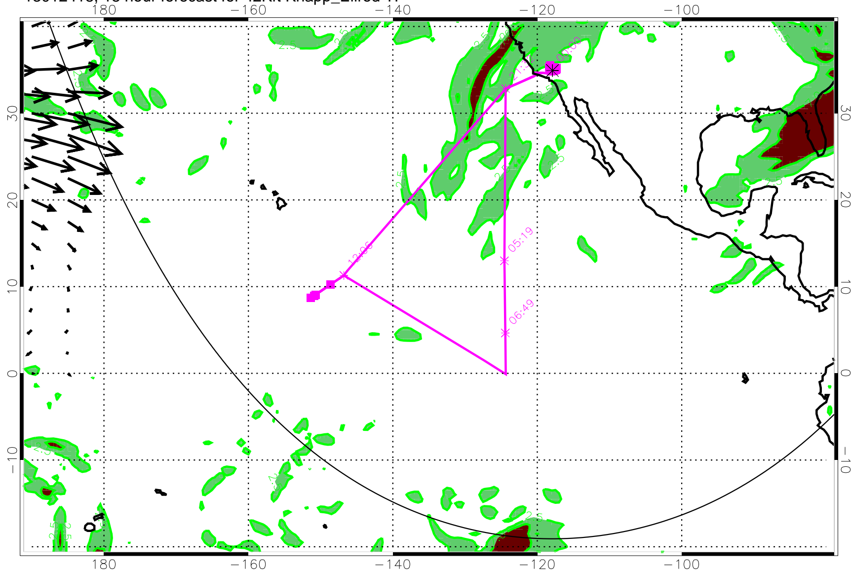
13012418, 18 hour forecast for 42Kft Knapp_Ellrod TI
