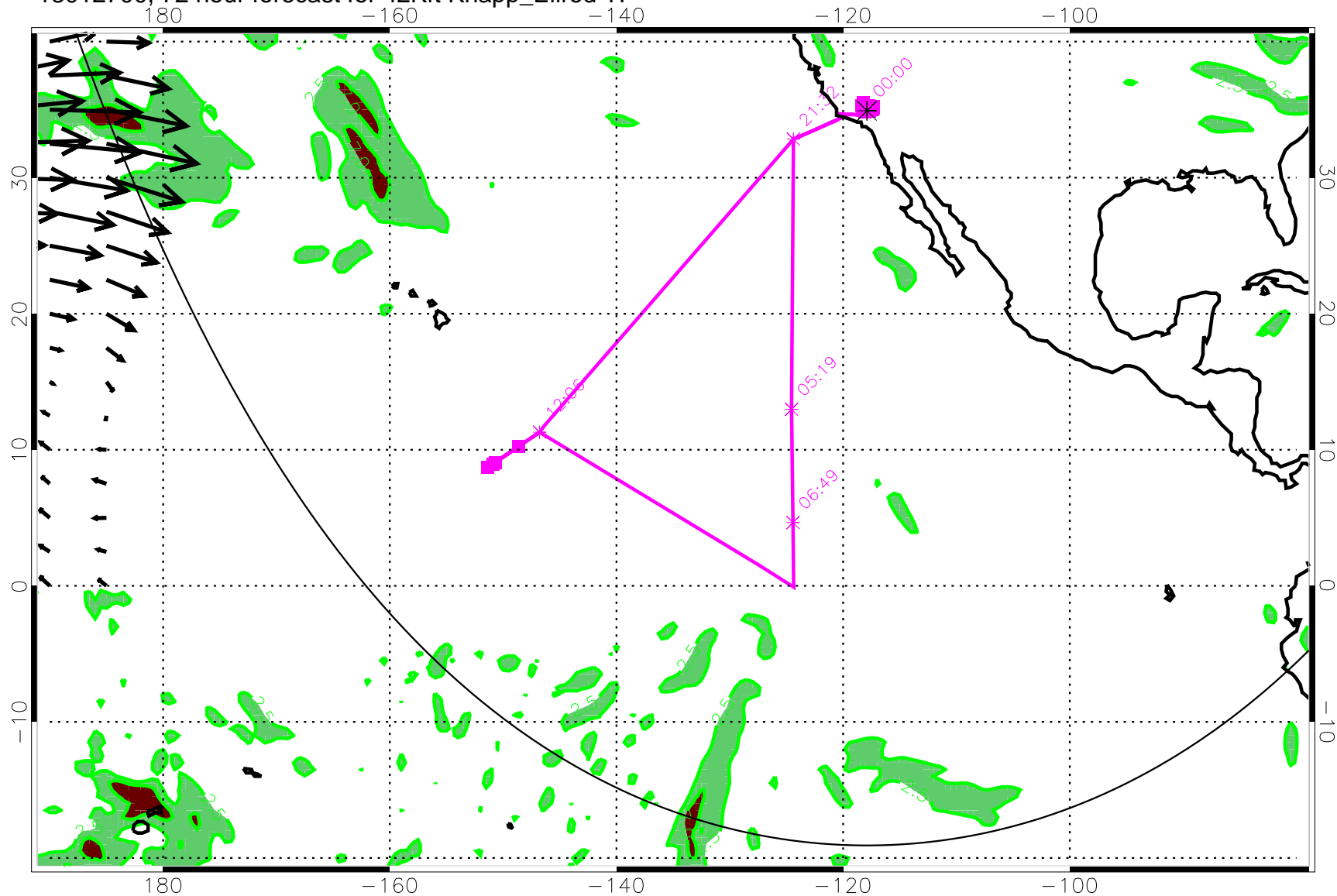
13012700, 72 hour forecast for 42Kft Knapp_Ellrod TI
