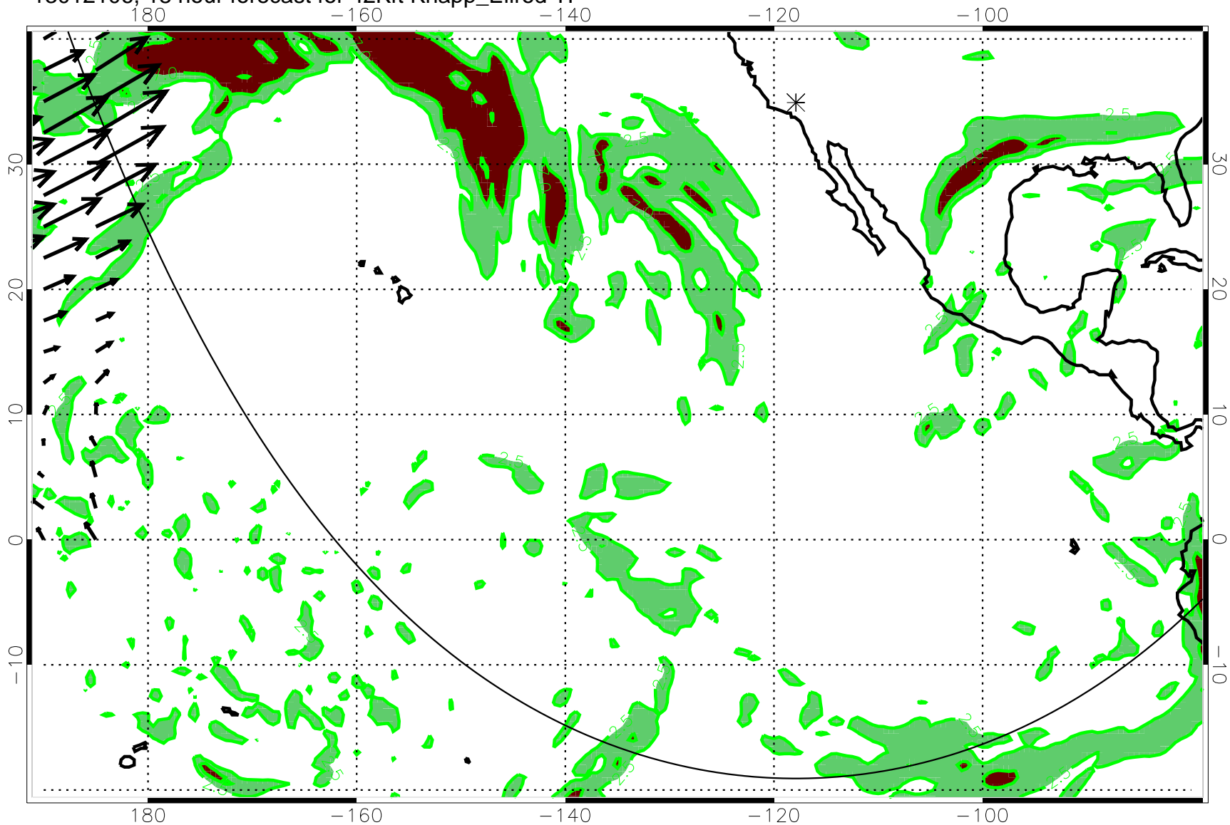
13012106, 18 hour forecast for 42Kft Knapp_Ellrod TI
