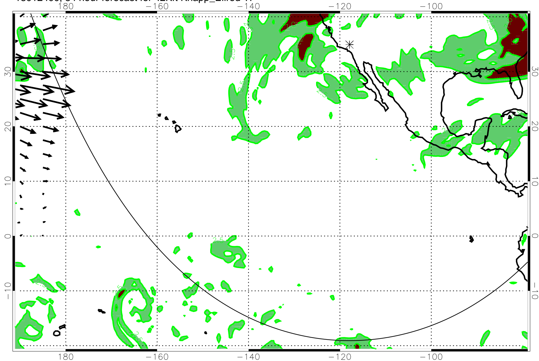
13012400, 84 hour forecast for 42Kft Knapp_Ellrod TI
