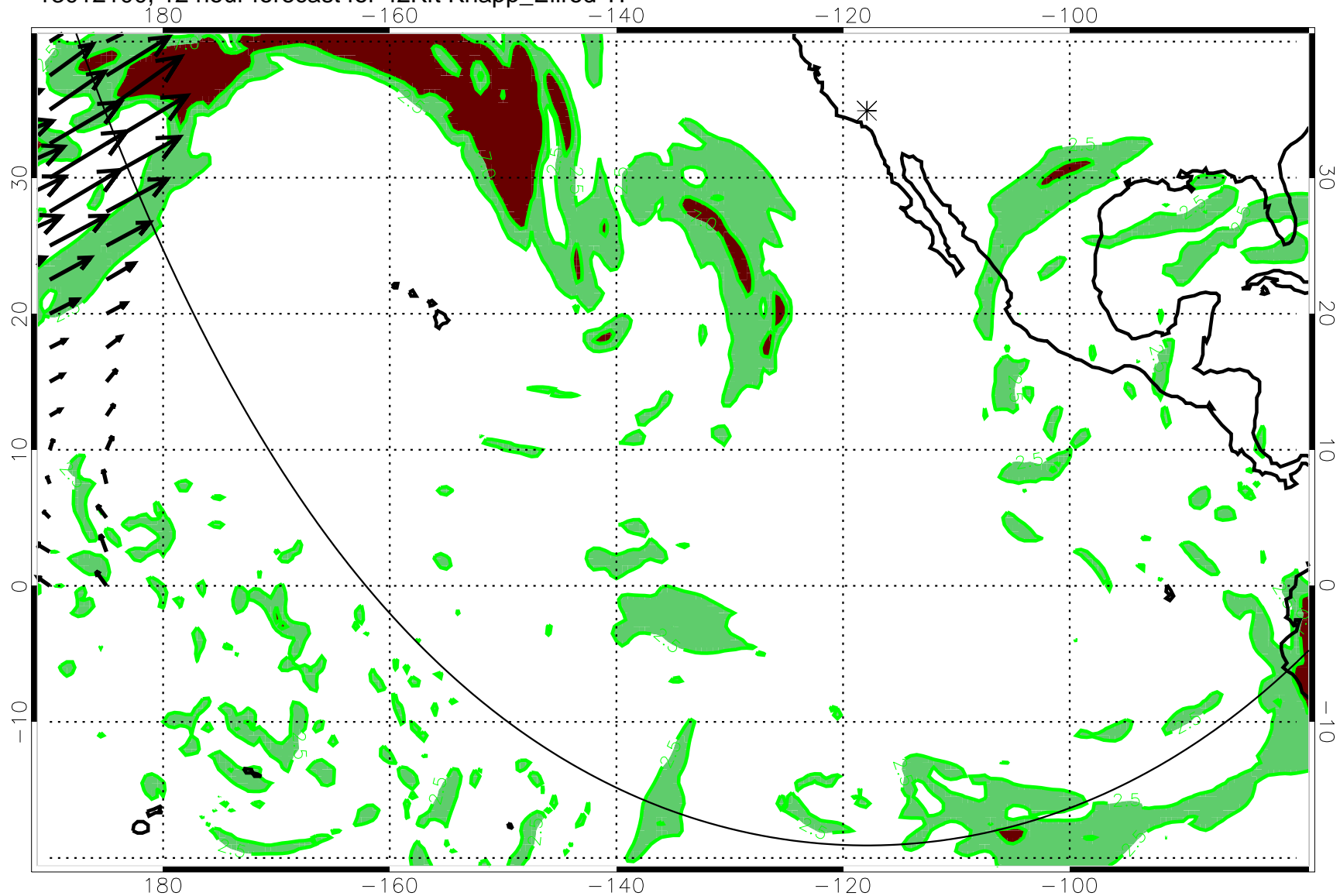
13012100, 12 hour forecast for 42Kft Knapp_Ellrod TI
