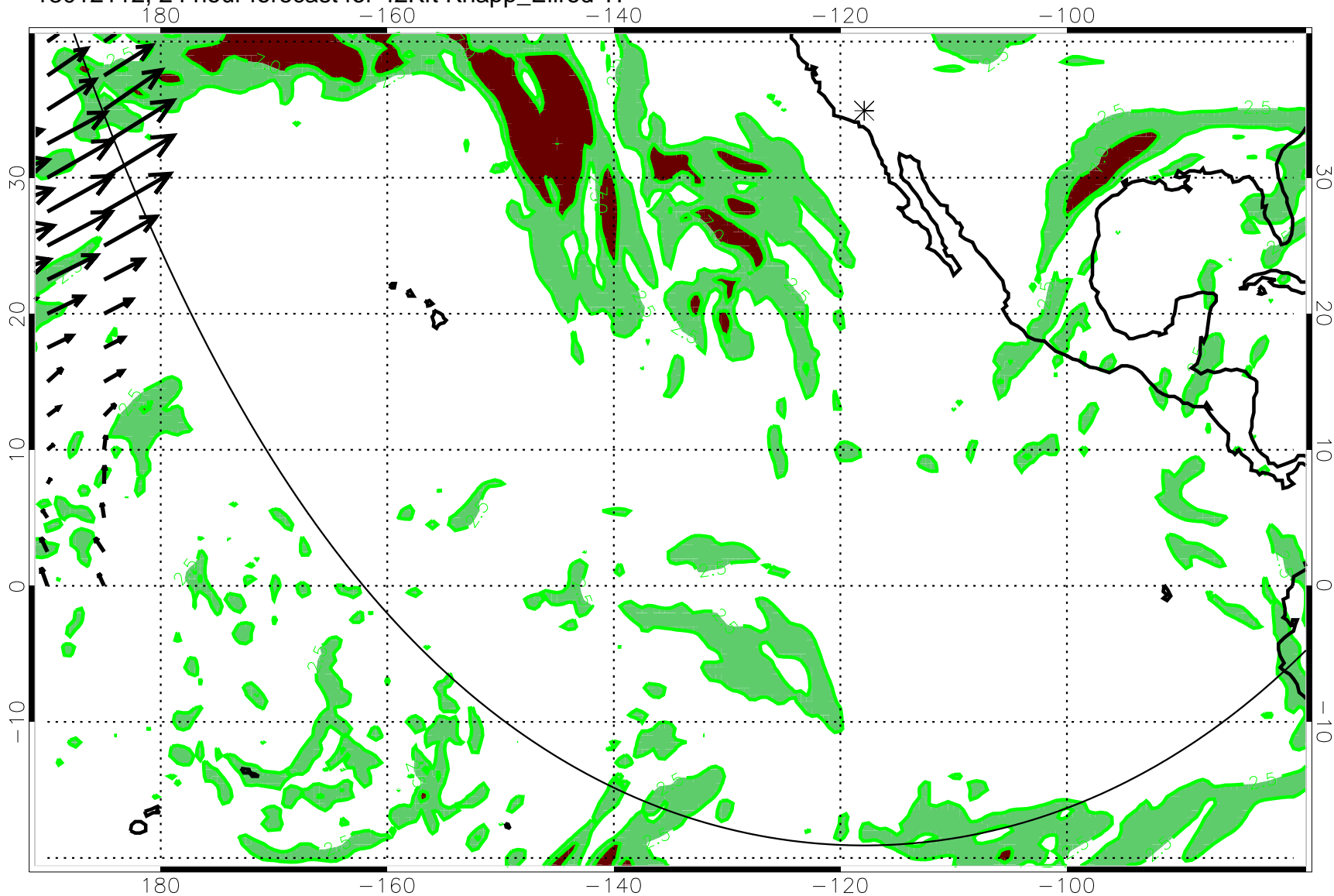
13012112, 24 hour forecast for 42Kft Knapp_Ellrod TI
