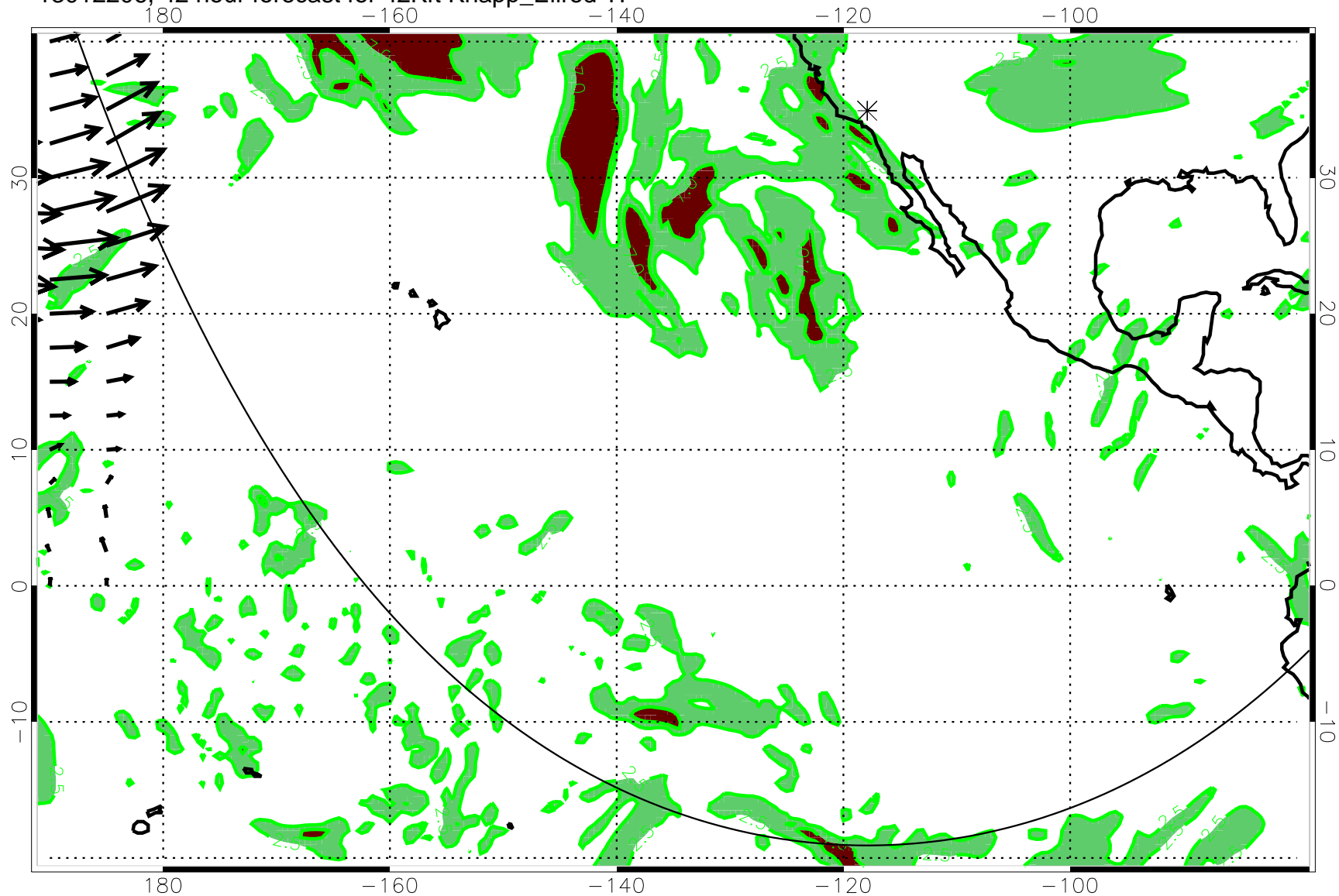
13012206, 42 hour forecast for 42Kft Knapp_Ellrod TI
