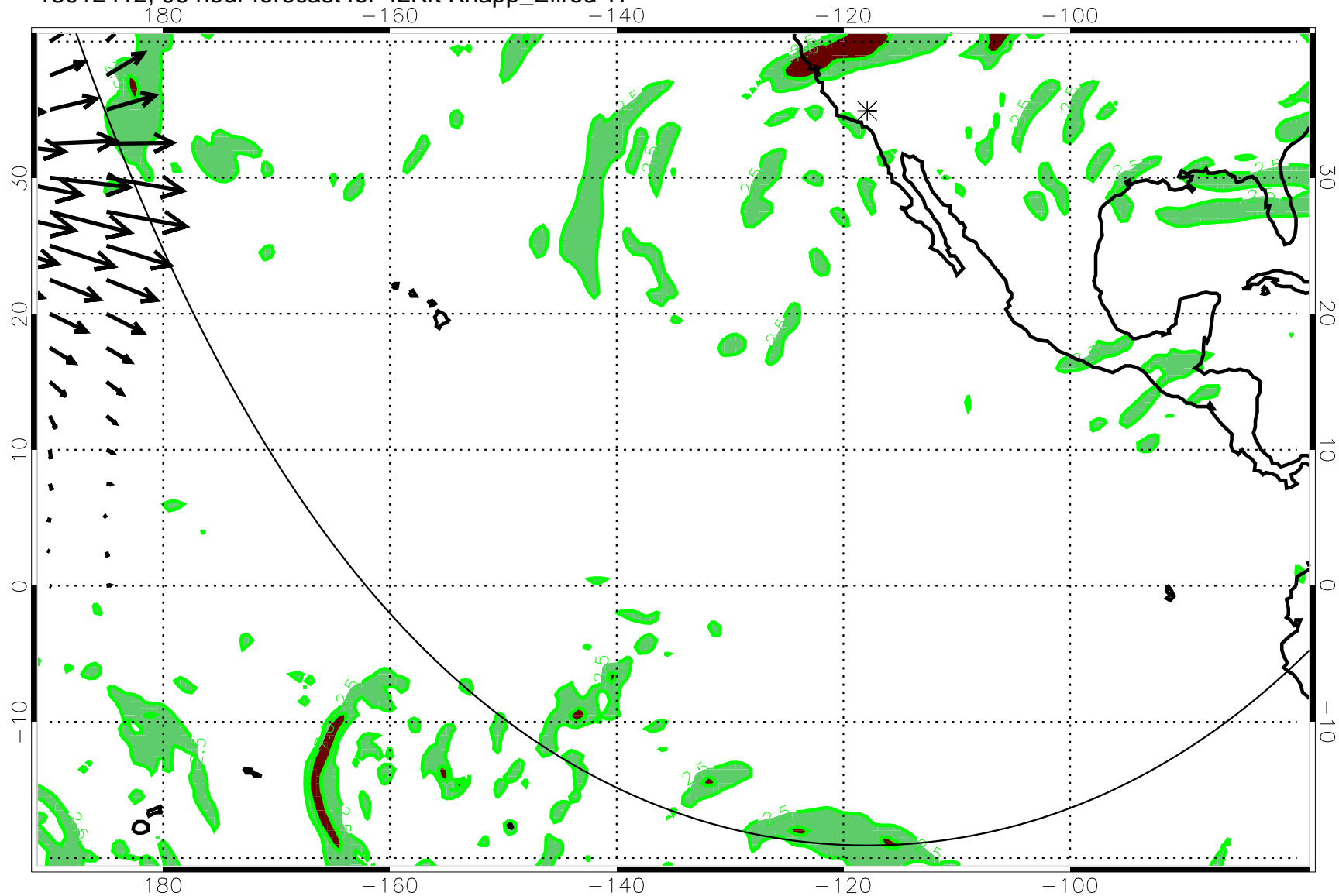
13012412, 96 hour forecast for 42Kft Knapp_Ellrod TI
