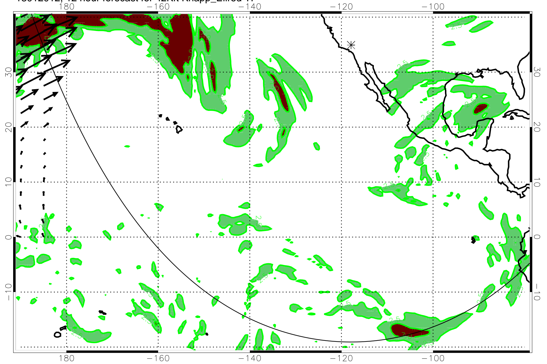
13012012, 12 hour forecast for 42Kft Knapp_Ellrod TI
