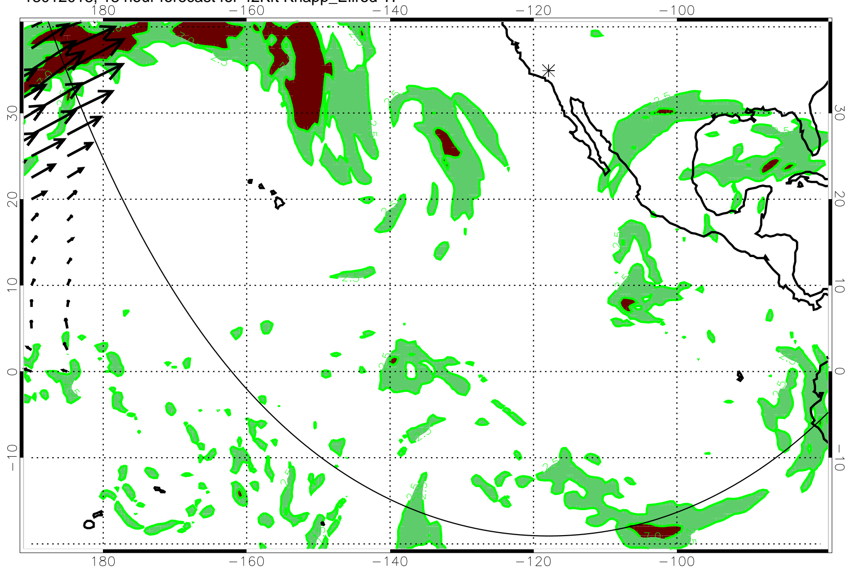
13012018, 18 hour forecast for 42Kft Knapp_Ellrod TI
