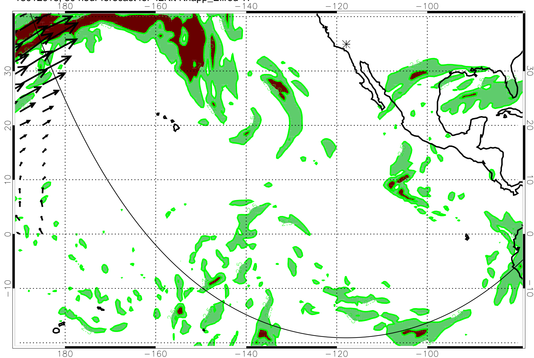
13012018, 30 hour forecast for 42Kft Knapp_Ellrod TI
