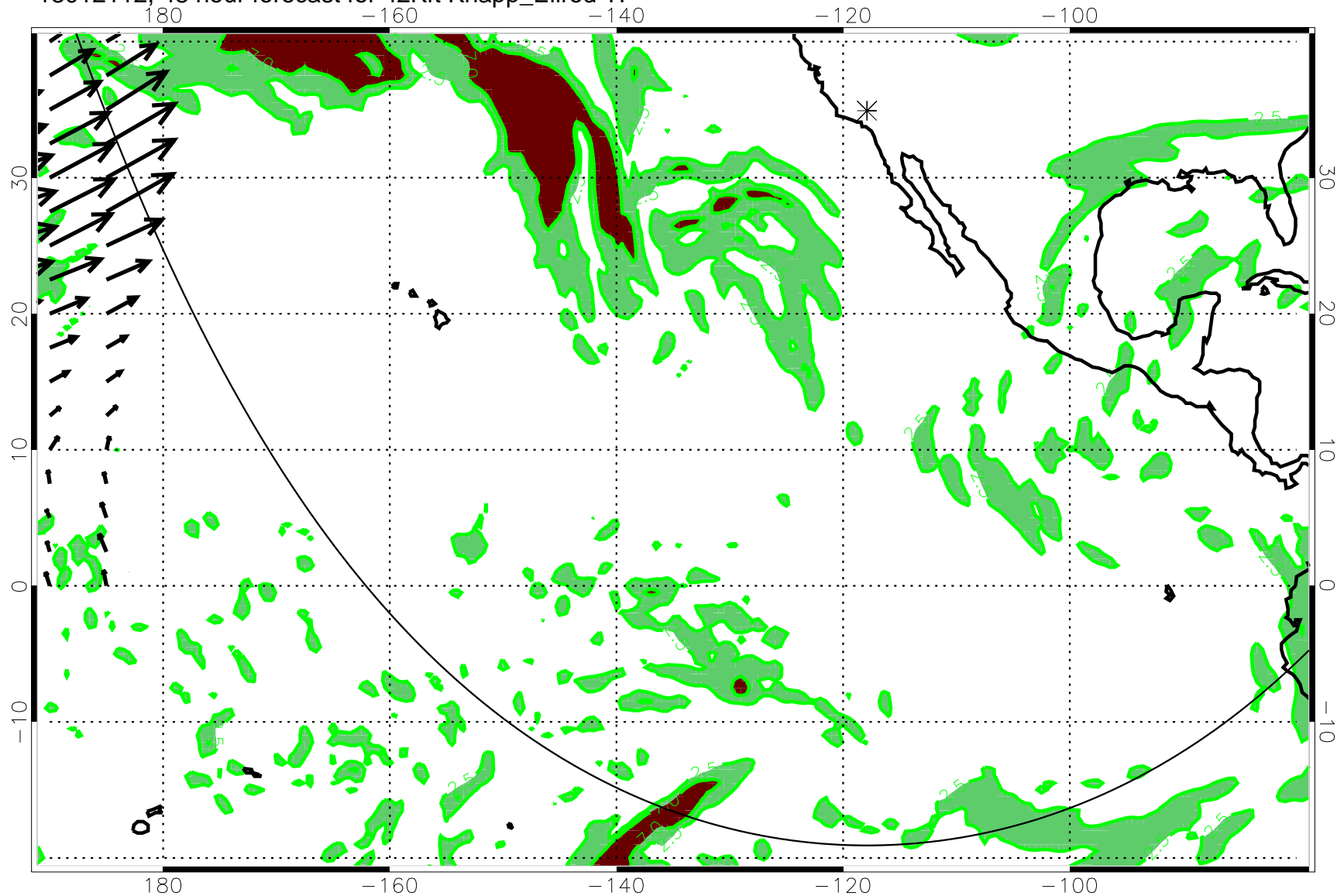
13012112, 48 hour forecast for 42Kft Knapp_Ellrod TI
