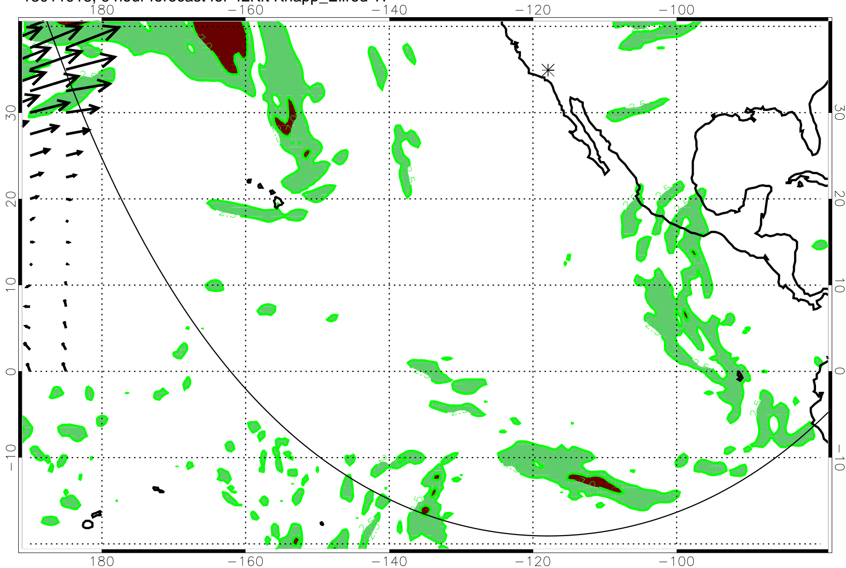
13011918, 6 hour forecast for 42Kft Knapp_Ellrod TI
