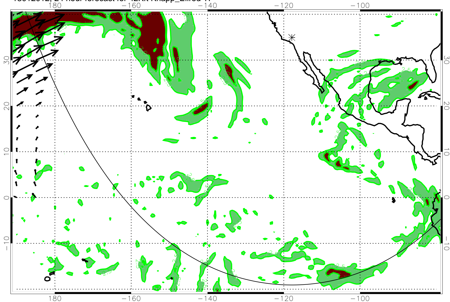
13012012, 24 hour forecast for 42Kft Knapp_Ellrod T1
