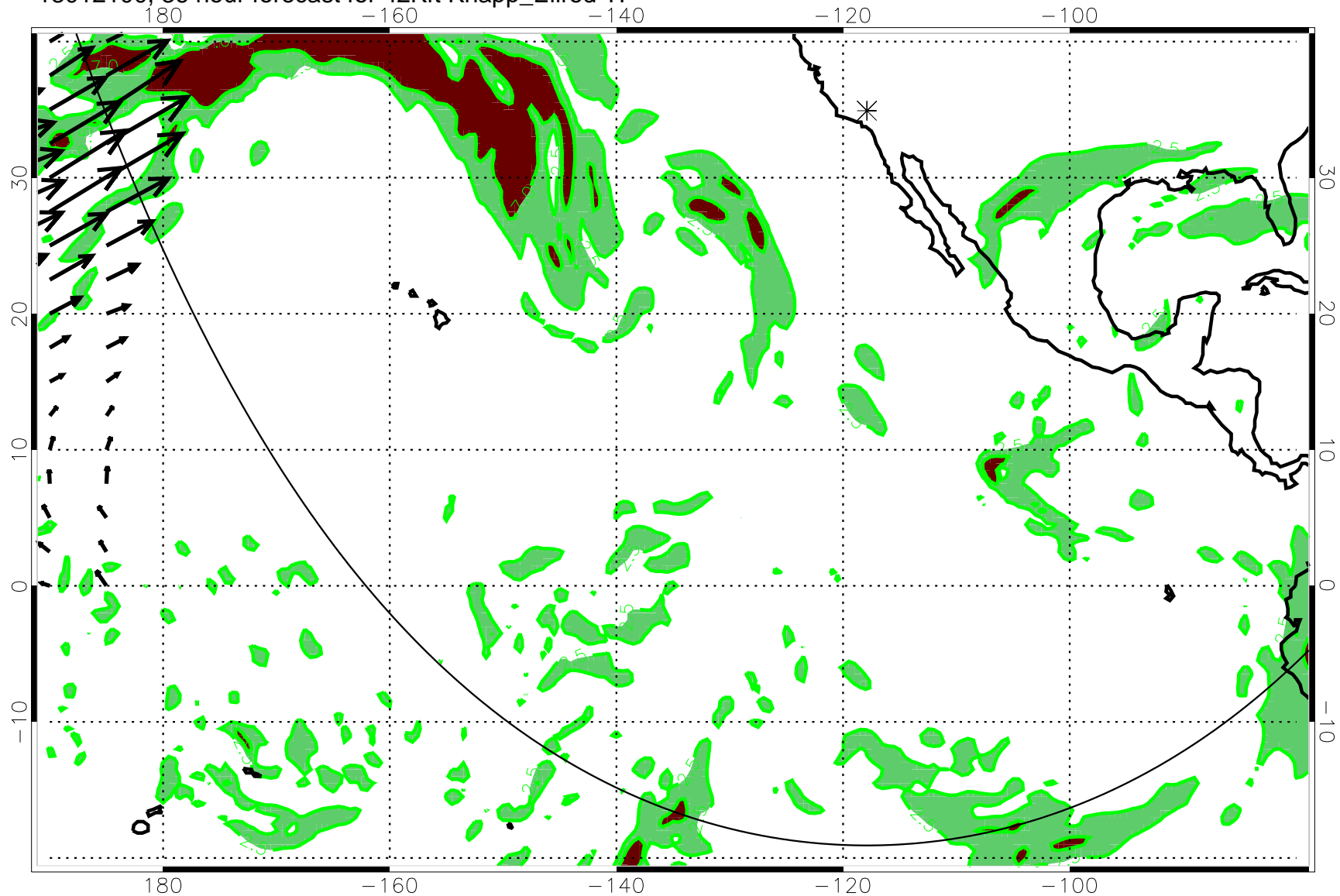
13012100, 36 hour forecast for 42Kft Knapp_Ellrod TI
