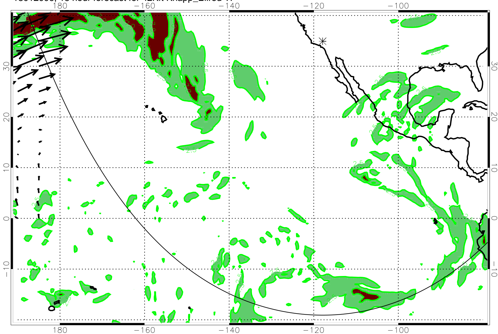
13012006, 18 hour forecast for 42Kft Knapp_Ellrod TI
