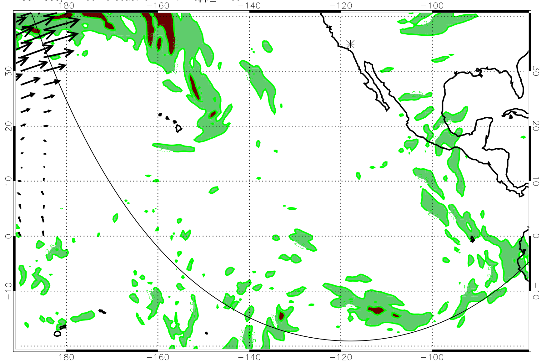
13012000, 12 hour forecast for 42Kft Knapp_Ellrod TI
