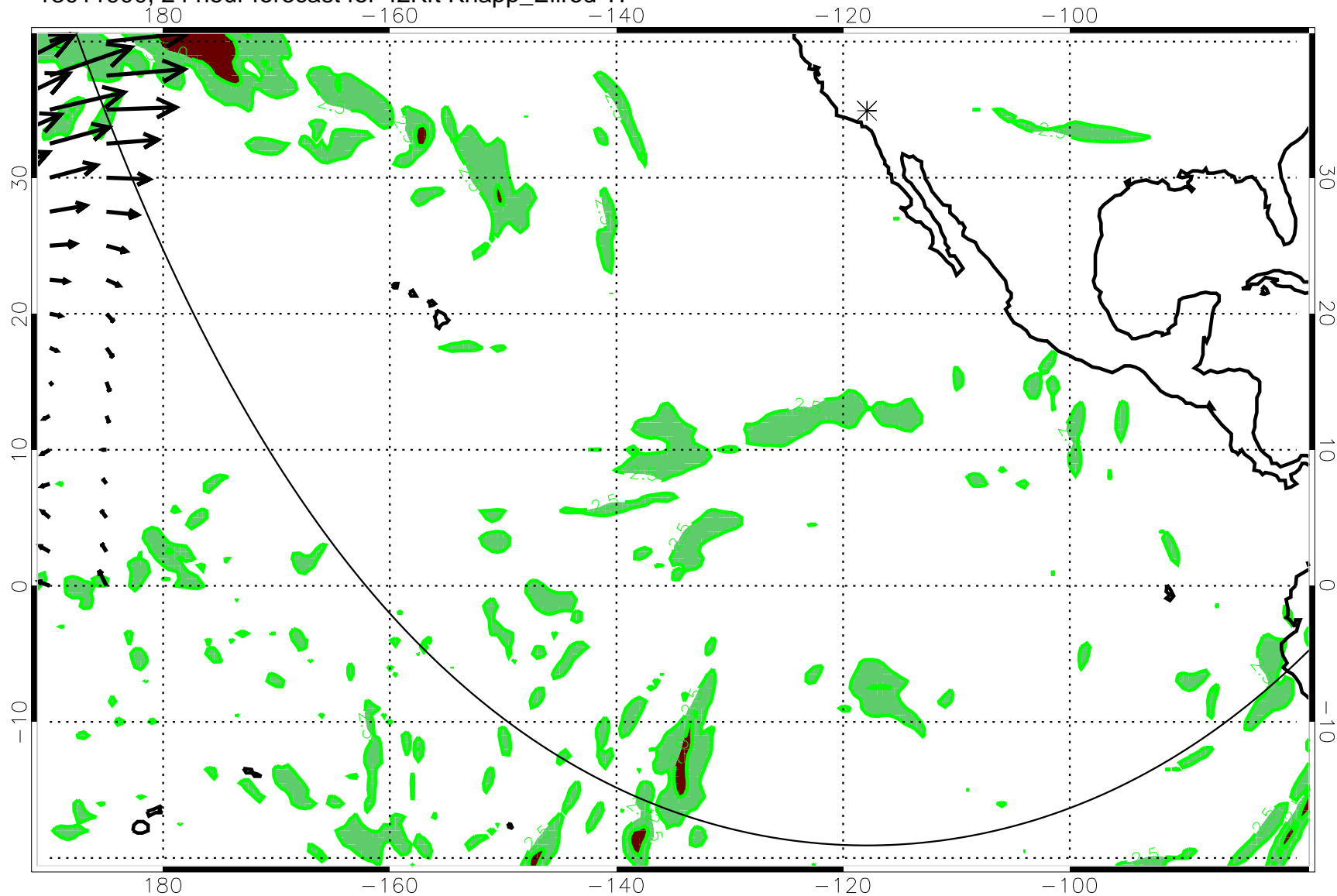
13011900, 24 hour forecast for 42Kft Knapp_Ellrod TI
