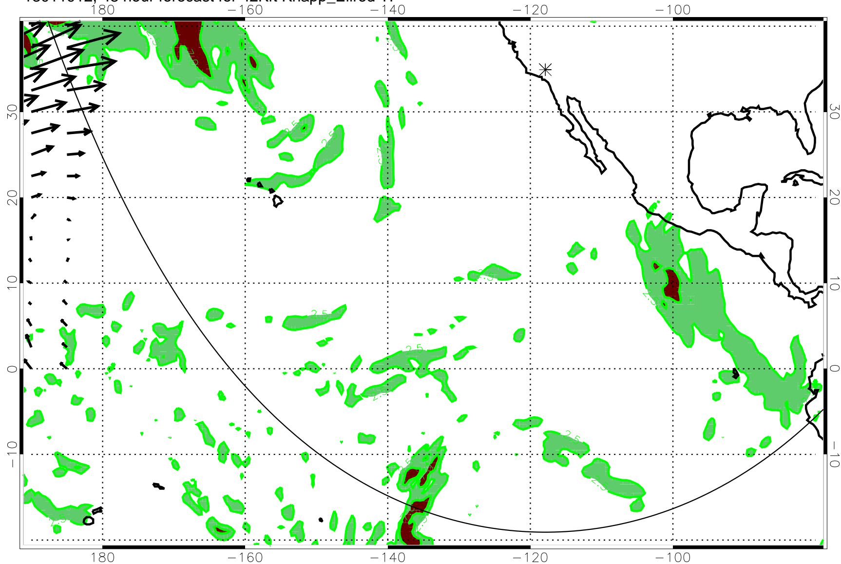
13011912, 48 hour forecast for 42Kft Knapp_Ellrod TI
