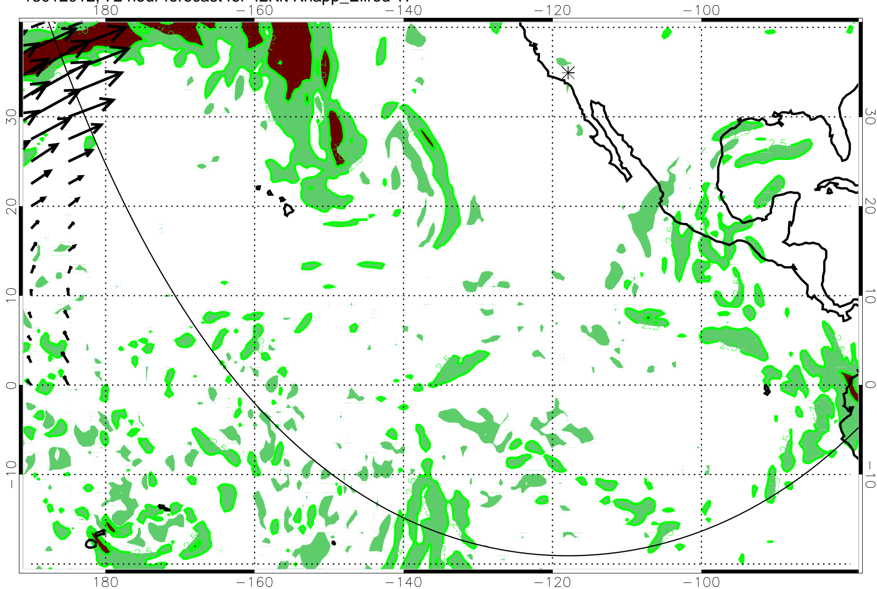
13012012, 72 hour forecast for 42Kft Knapp_Ellrod TI
