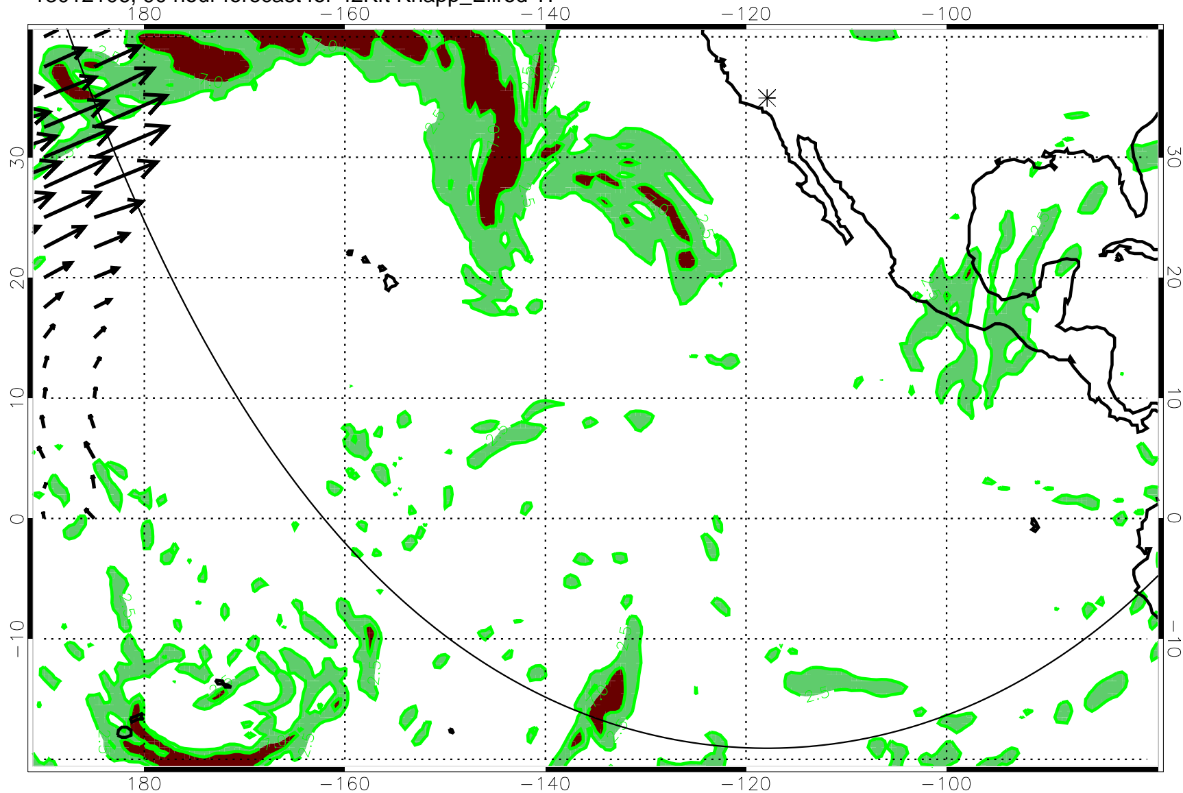
13012106, 90 hour forecast for 42Kft Knapp_Ellrod TI
