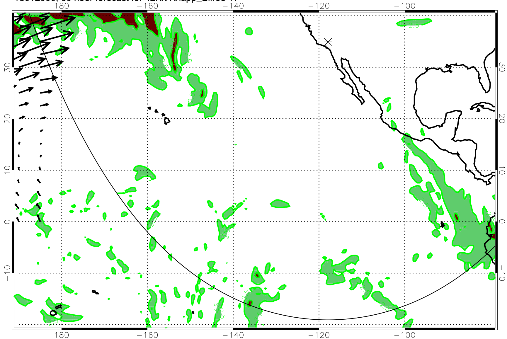
13012000, 60 hour forecast for 42Kft Knapp_Ellrod TI
