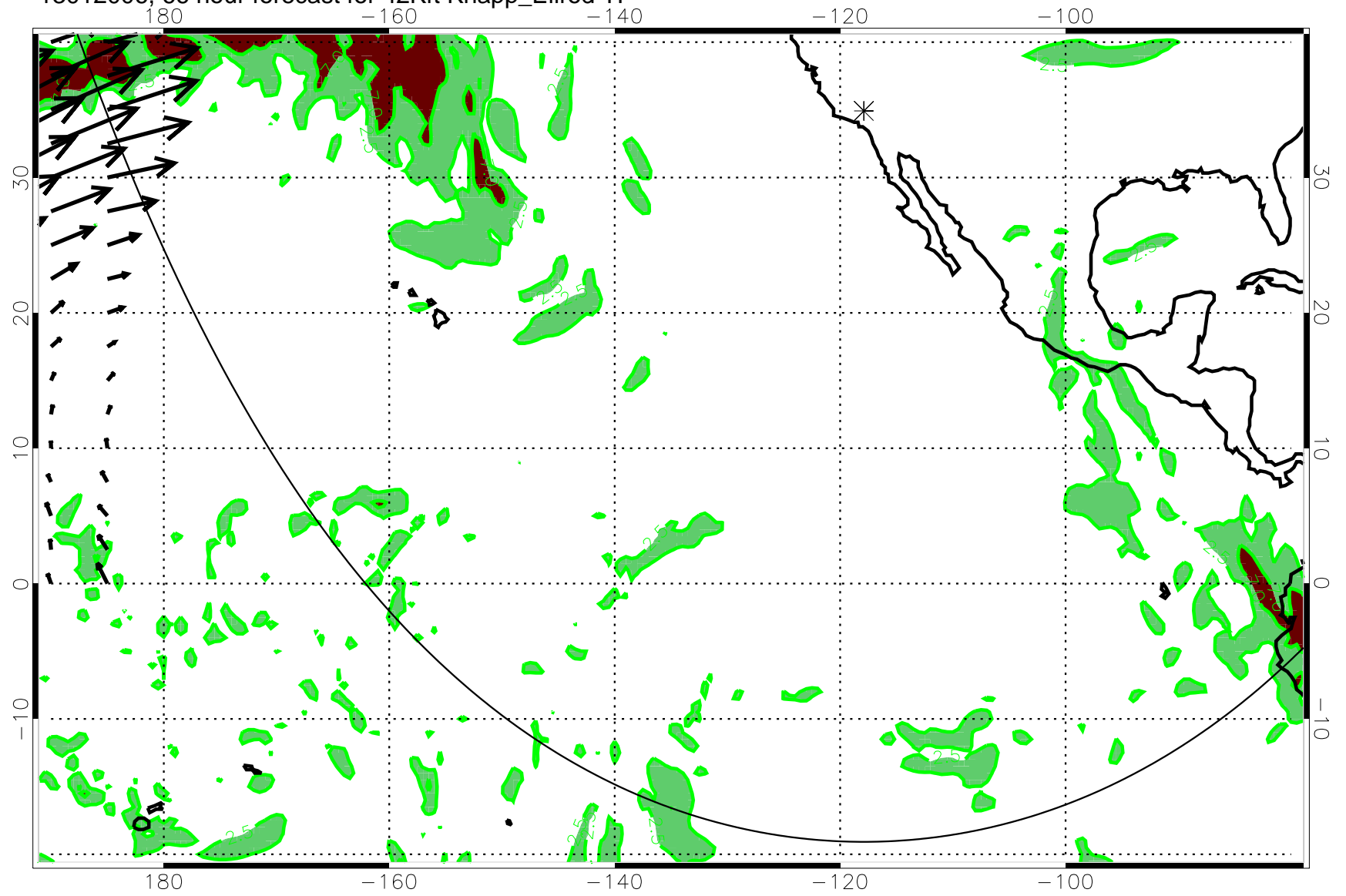
13012006, 66 hour forecast for 42Kft Knapp_Ellrod TI
