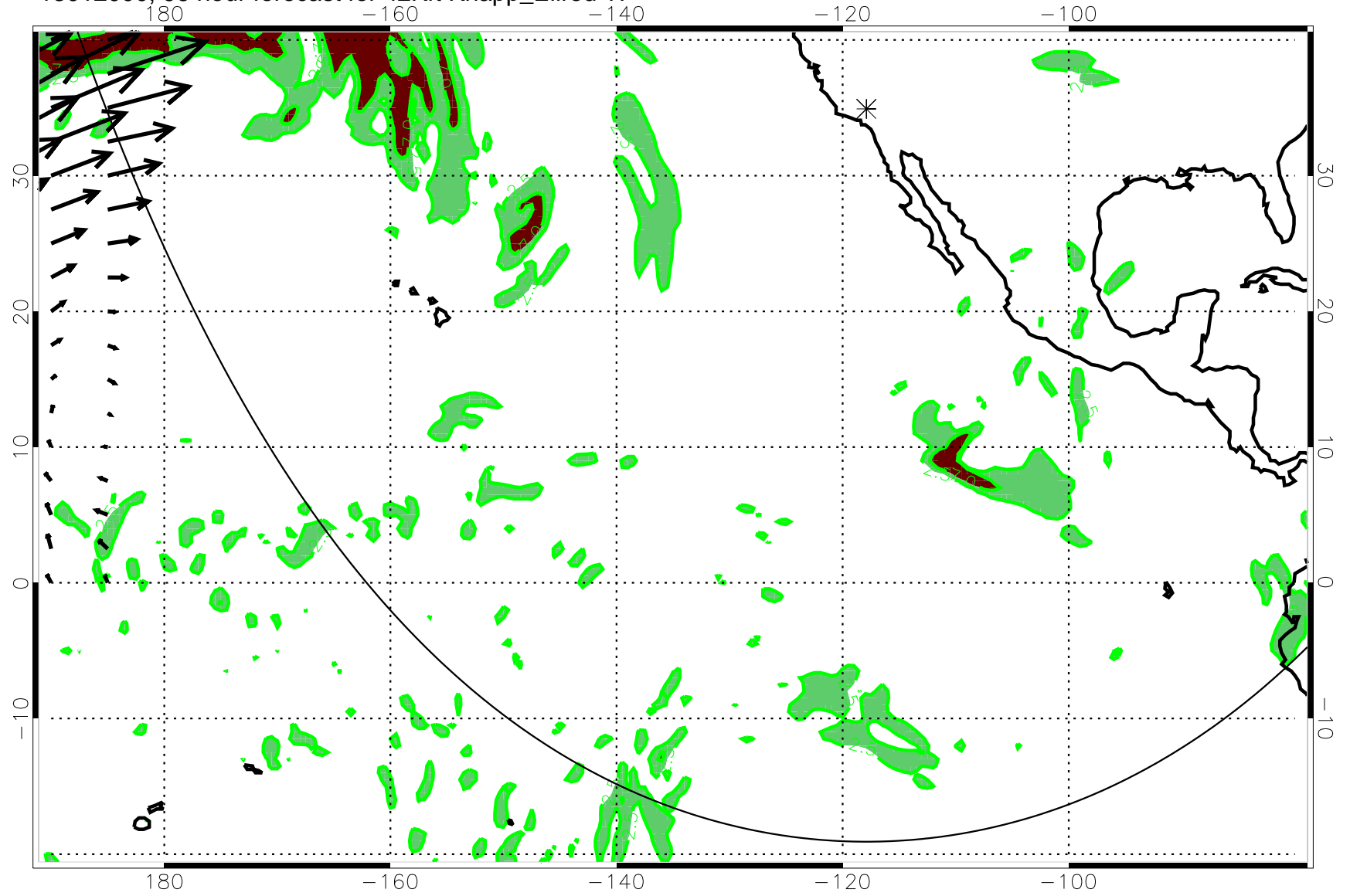
13012000, 96 hour forecast for 42Kft Knapp_Ellrod TI
