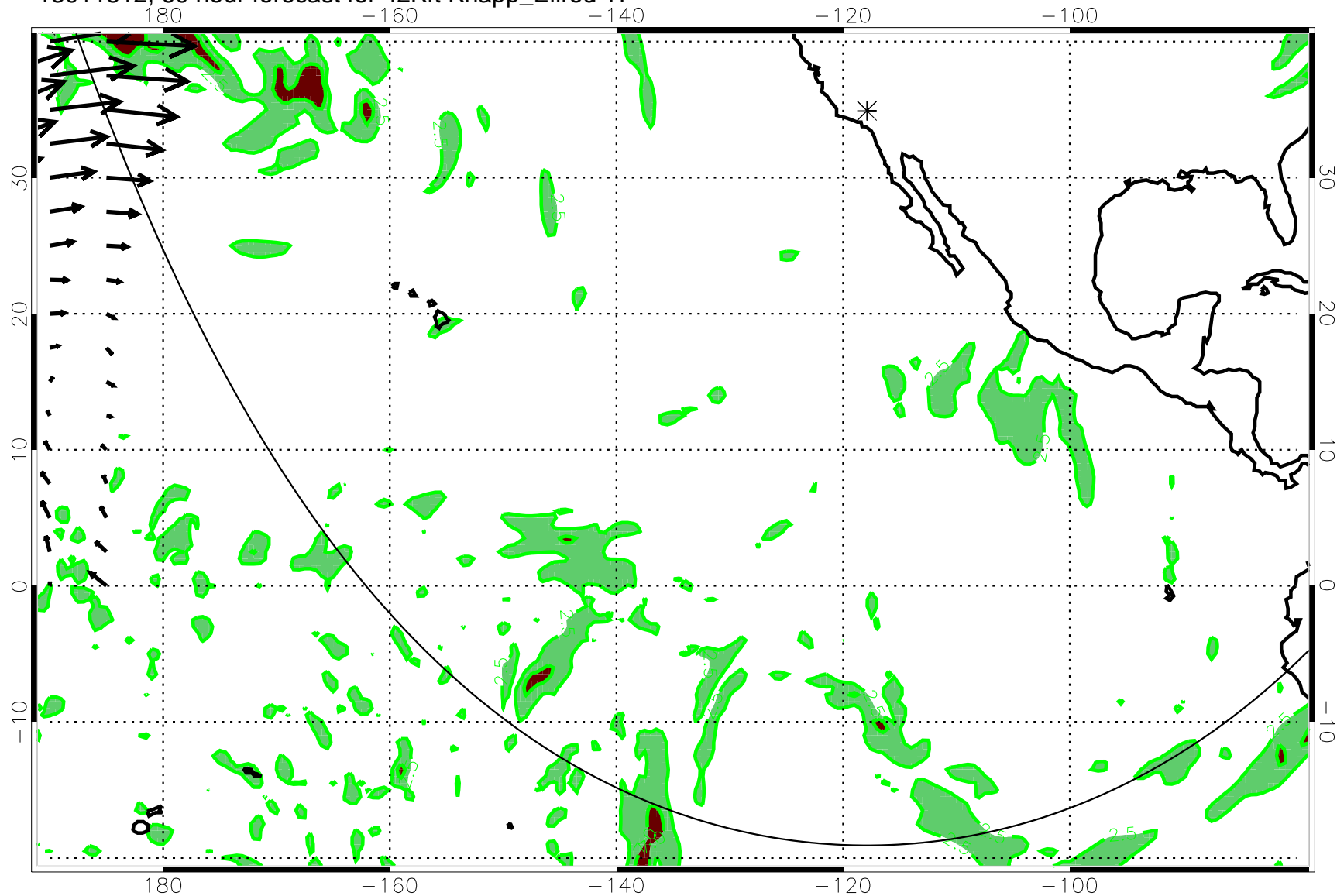
13011812, 60 hour forecast for 42Kft Knapp_Ellrod TI
