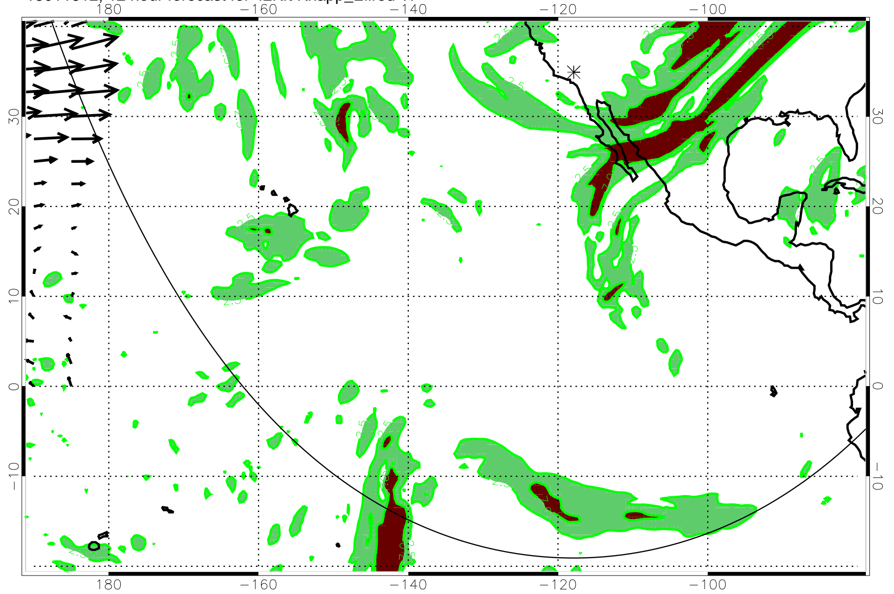
13011612, 12 hour forecast for 42Kft Knapp_Ellrod TI
