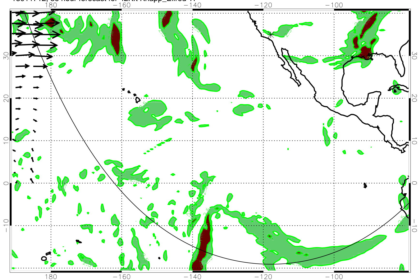
13011712, 36 hour forecast for 42Kft Knapp_Ellrod TI
