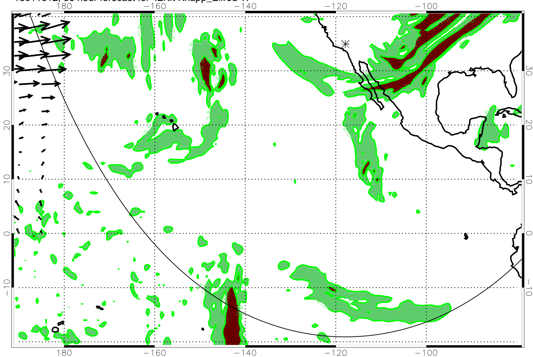
13011612, 36 hour forecast for 42Kft Knapp_Ellrod TI
