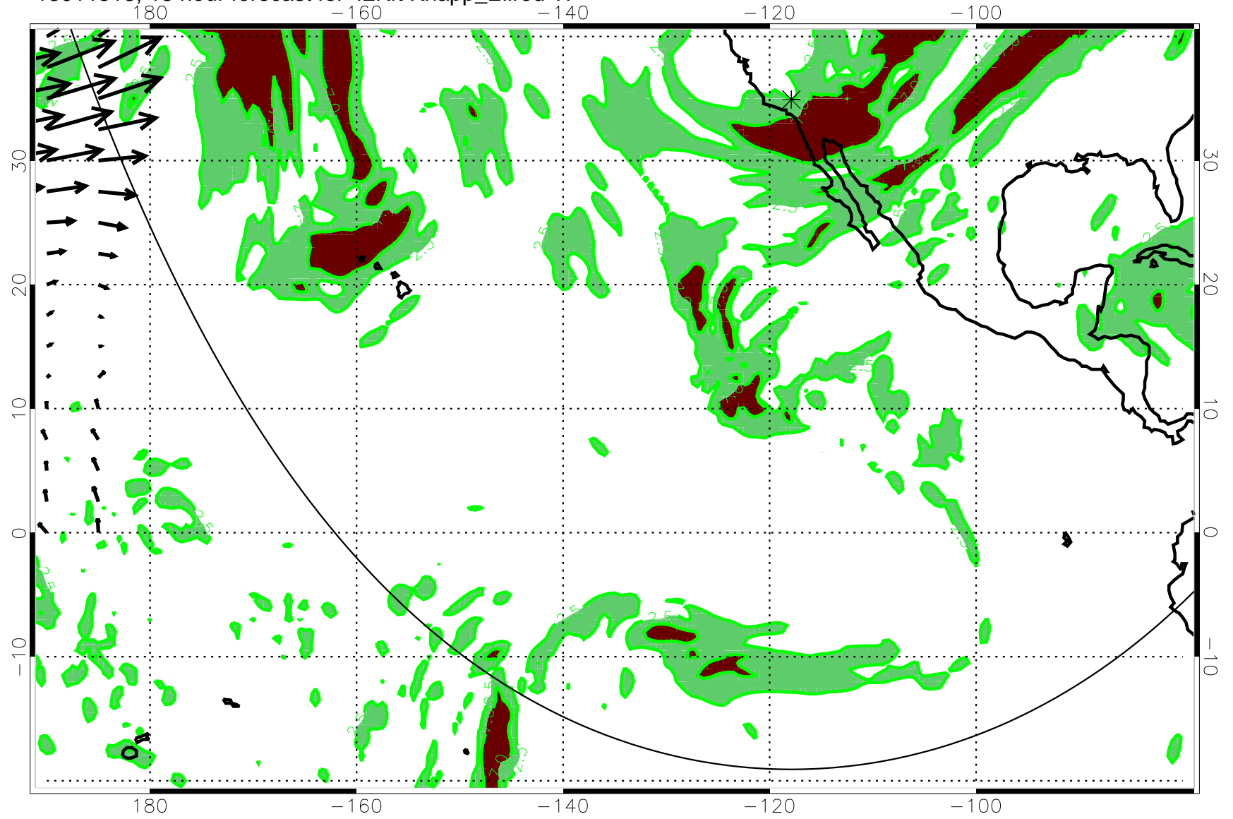
13011518, 18 hour forecast for 42Kft Knapp_Ellrod TI
