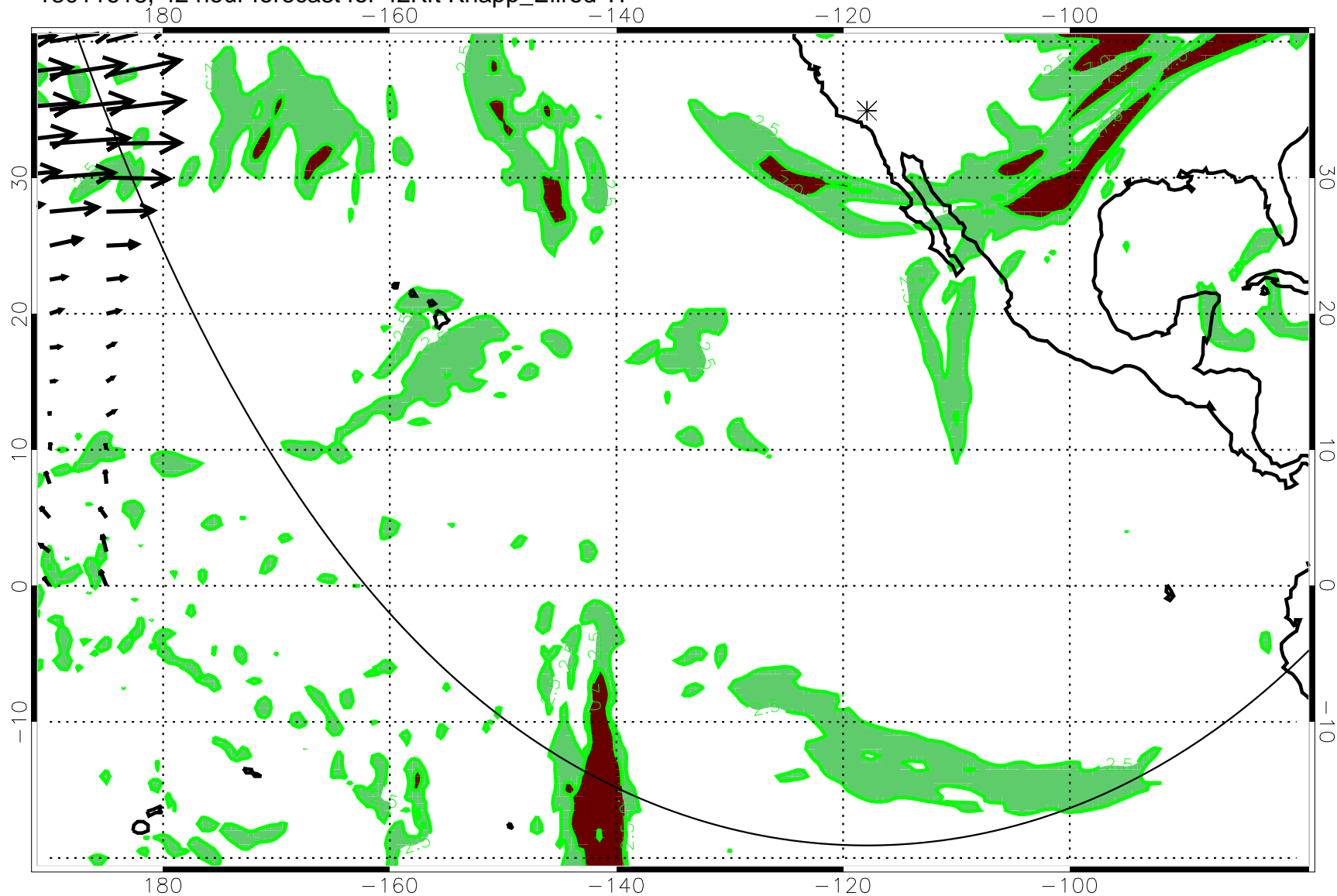
13011618, 42 hour forecast for 42Kft Knapp_Ellrod TI
