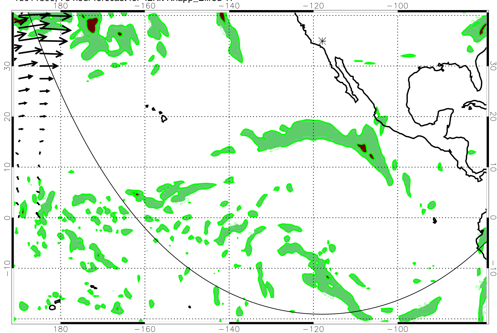
13011806, 78 hour forecast for 42Kft Knapp_Ellrod TI
