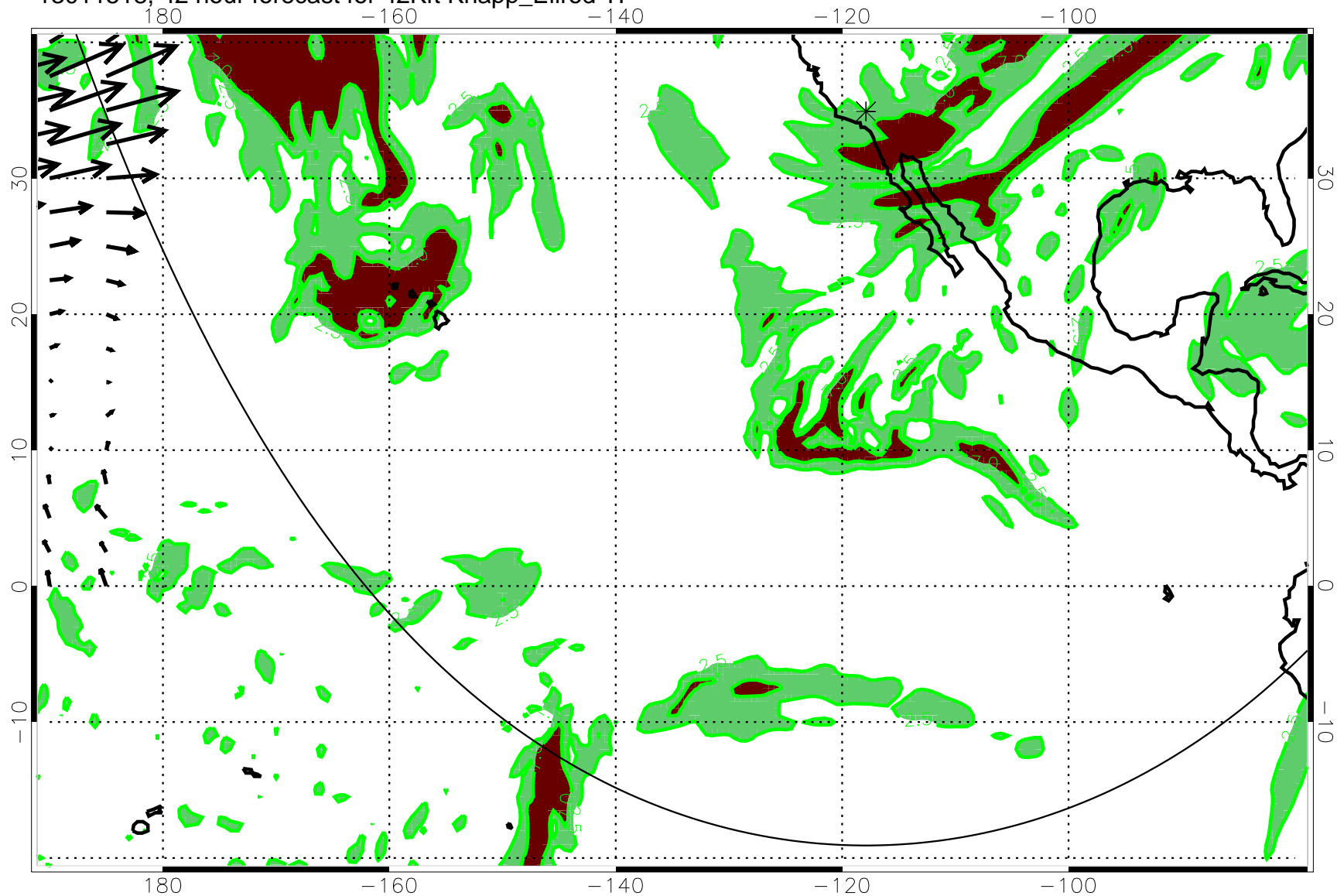
13011518, 42 hour forecast for 42Kft Knapp_Ellrod TI
