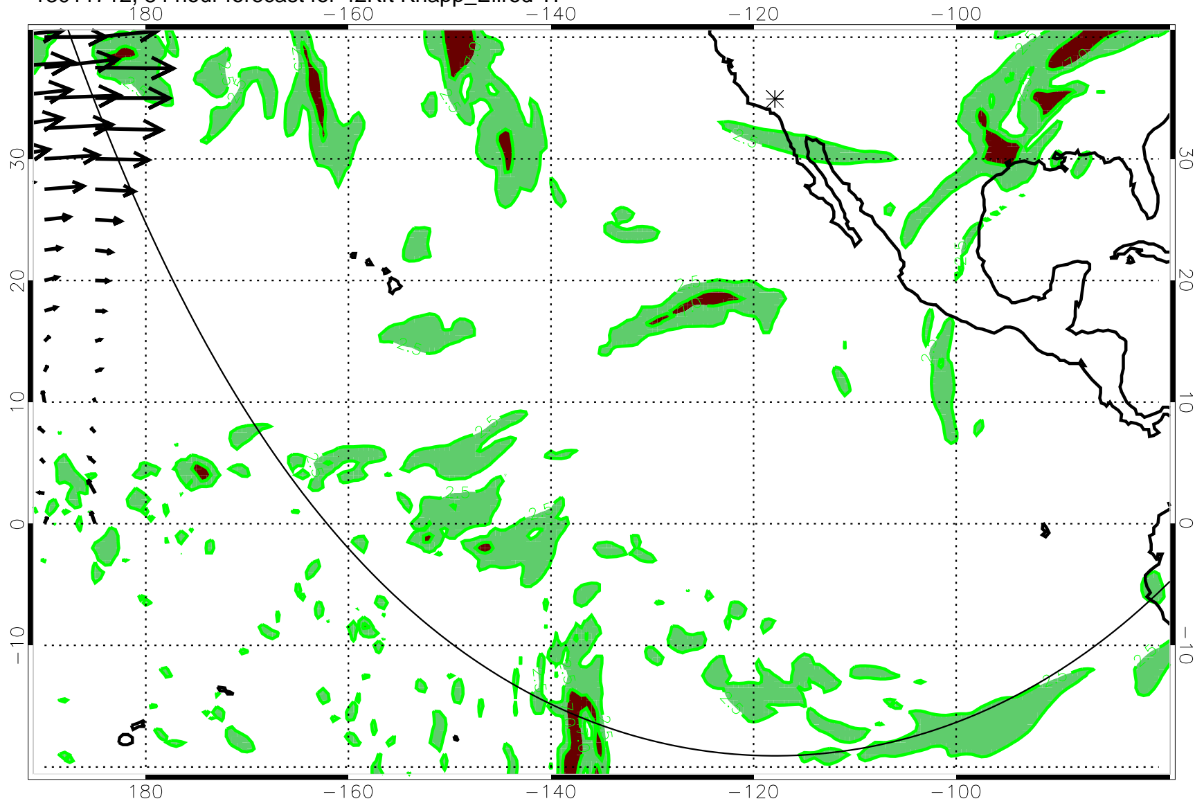
13011712, 84 hour forecast for 42Kft Knapp_Ellrod TI
