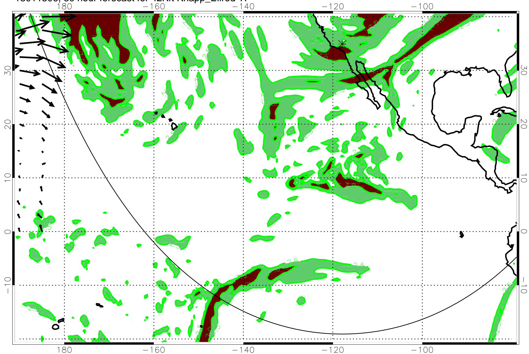
13011506, 30 hour forecast for 42Kft Knapp_Ellrod TI
