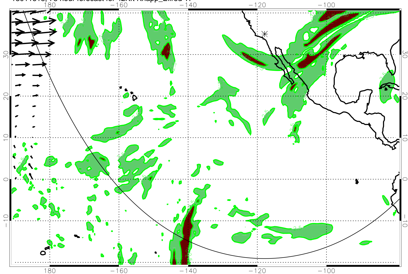
13011618, 78 hour forecast for 42Kft Knapp_Ellrod TI
