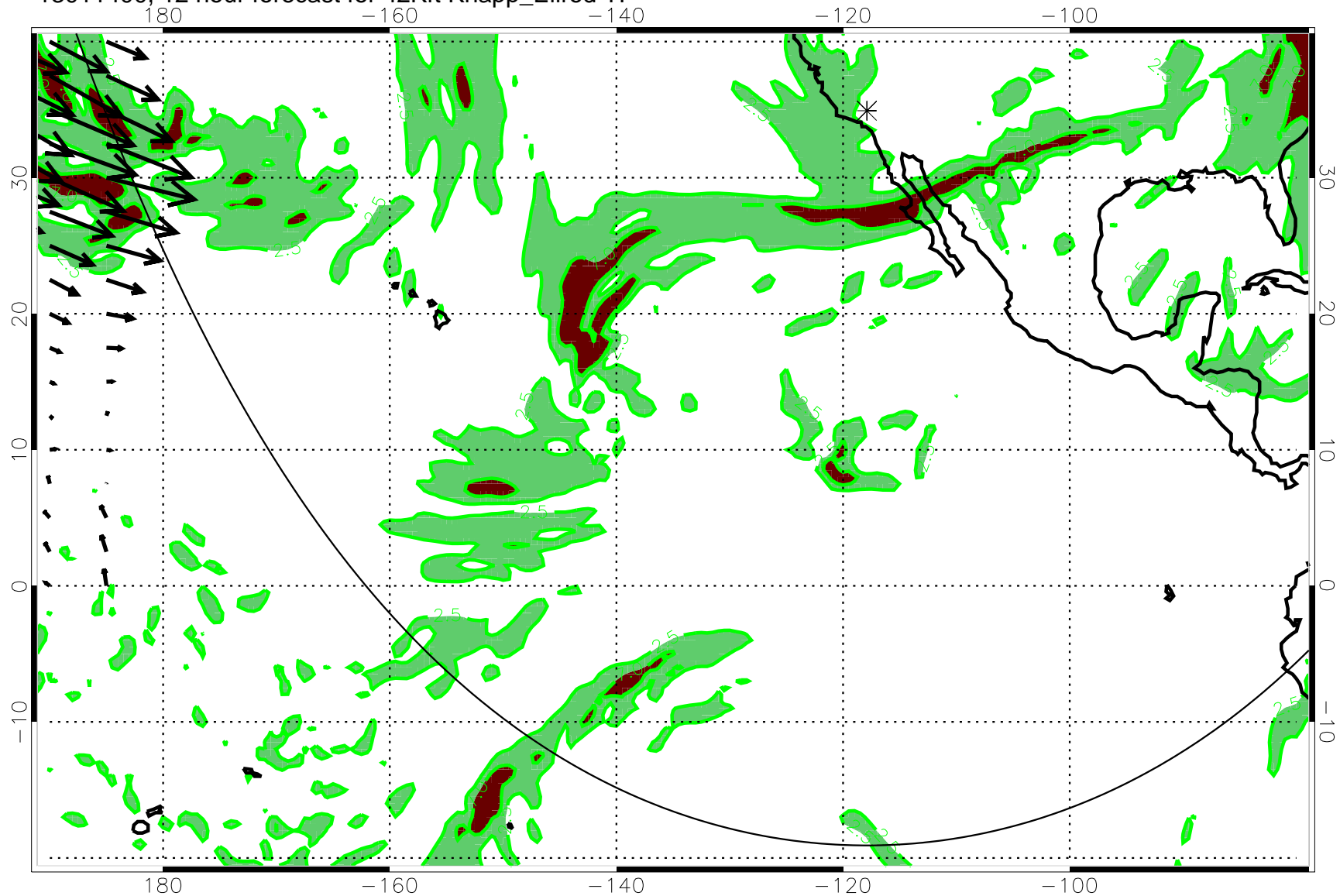
13011400, 12 hour forecast for 42Kft Knapp_Ellrod TI
