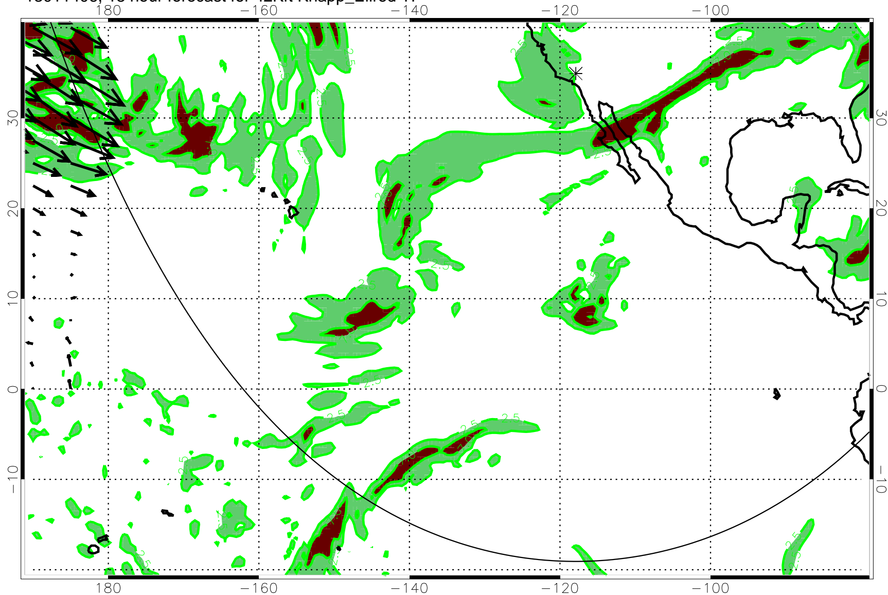
13011406, 18 hour forecast for 42Kft Knapp_Ellrod TI
