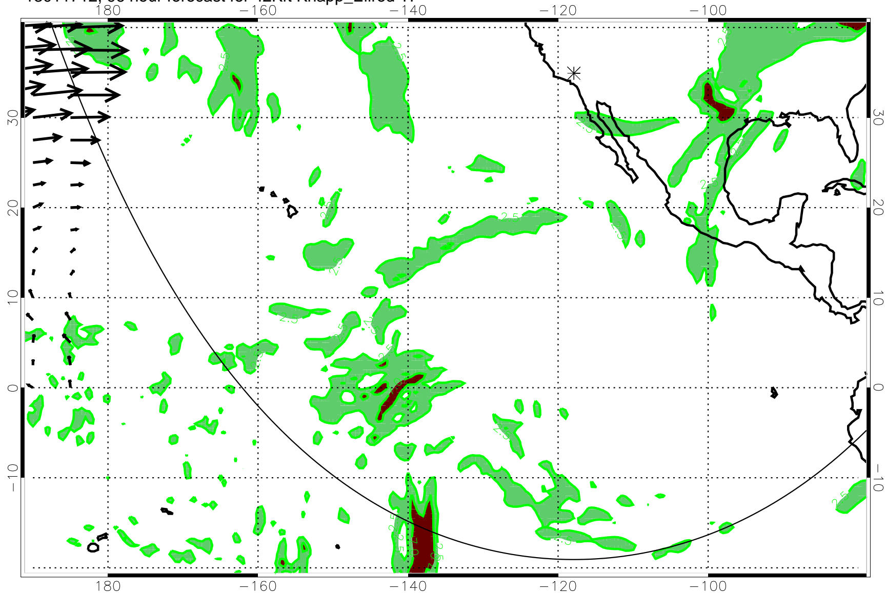
13011712, 96 hour forecast for 42Kft Knapp_Ellrod TI
