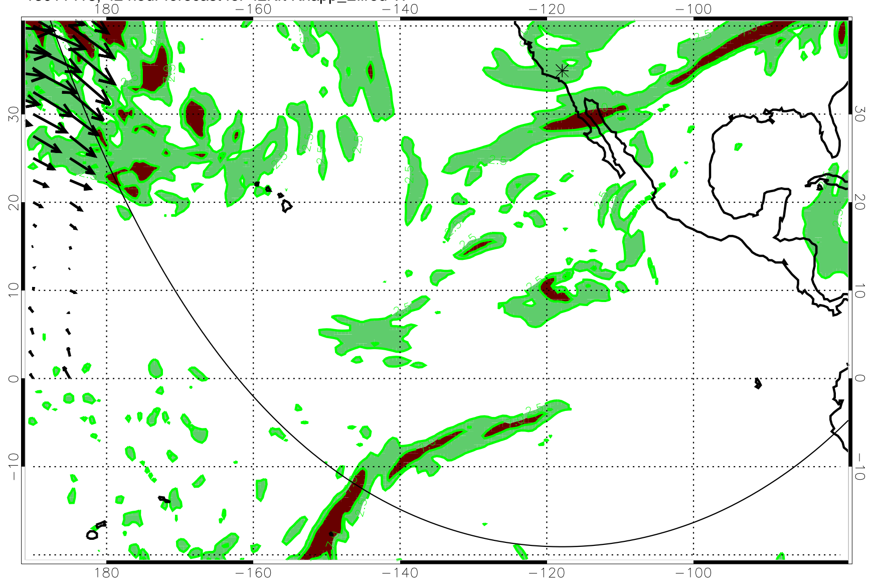
13011418, 42 hour forecast for 42Kft Knapp_Ellrod TI
