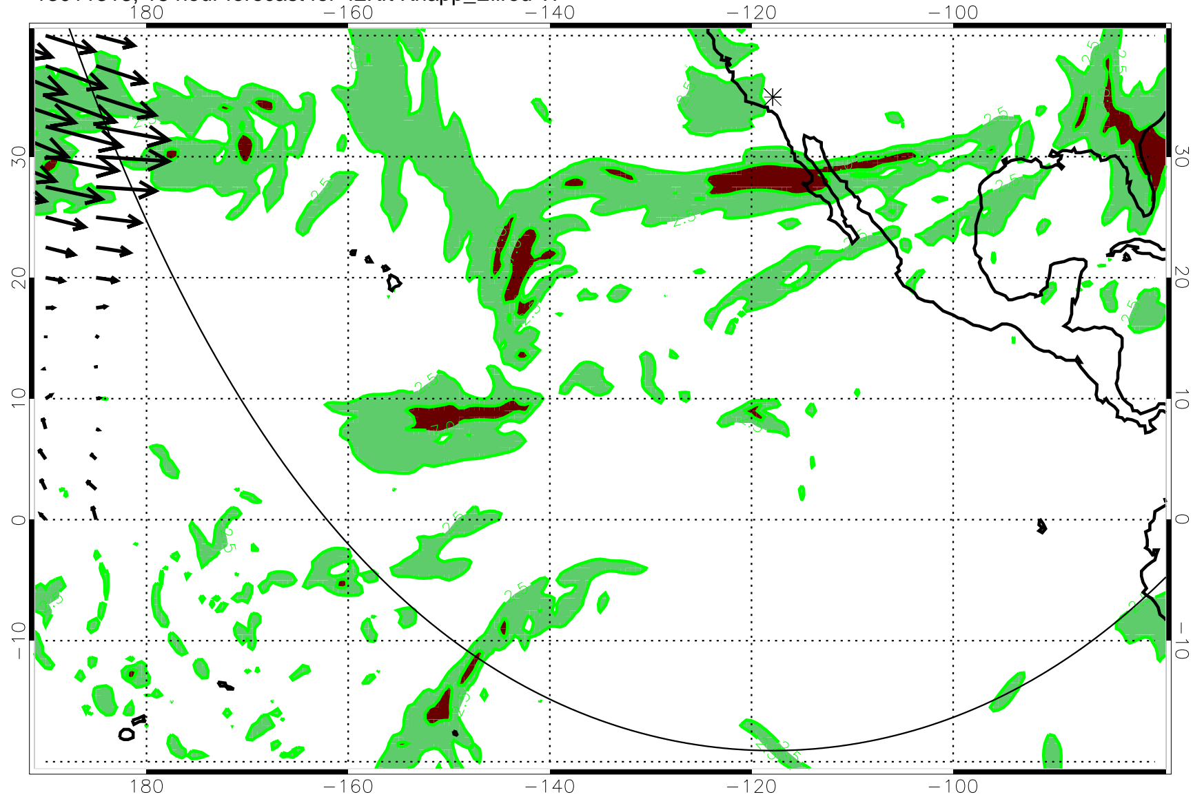
13011318, 18 hour forecast for 42Kft Knapp_Ellrod TI
