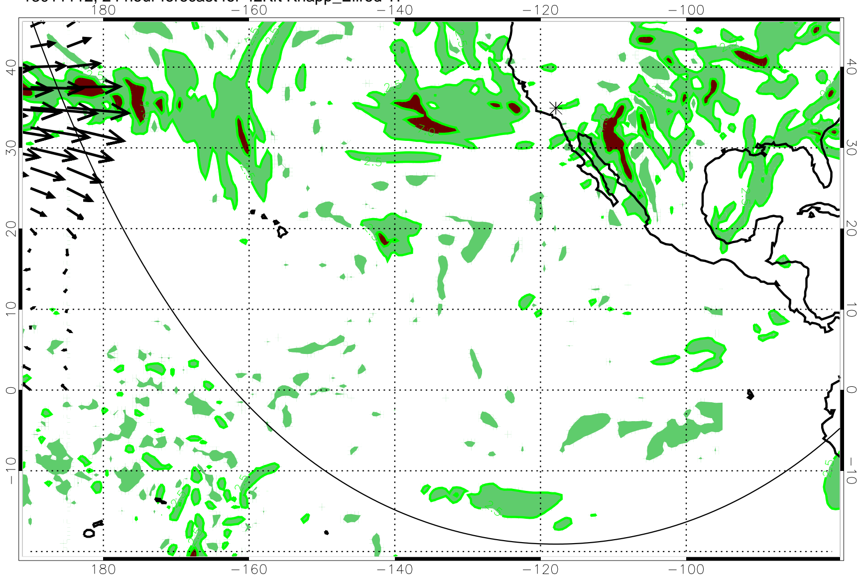
13011112, 24 hour forecast for 42Kft Knapp_Ellrod TI
