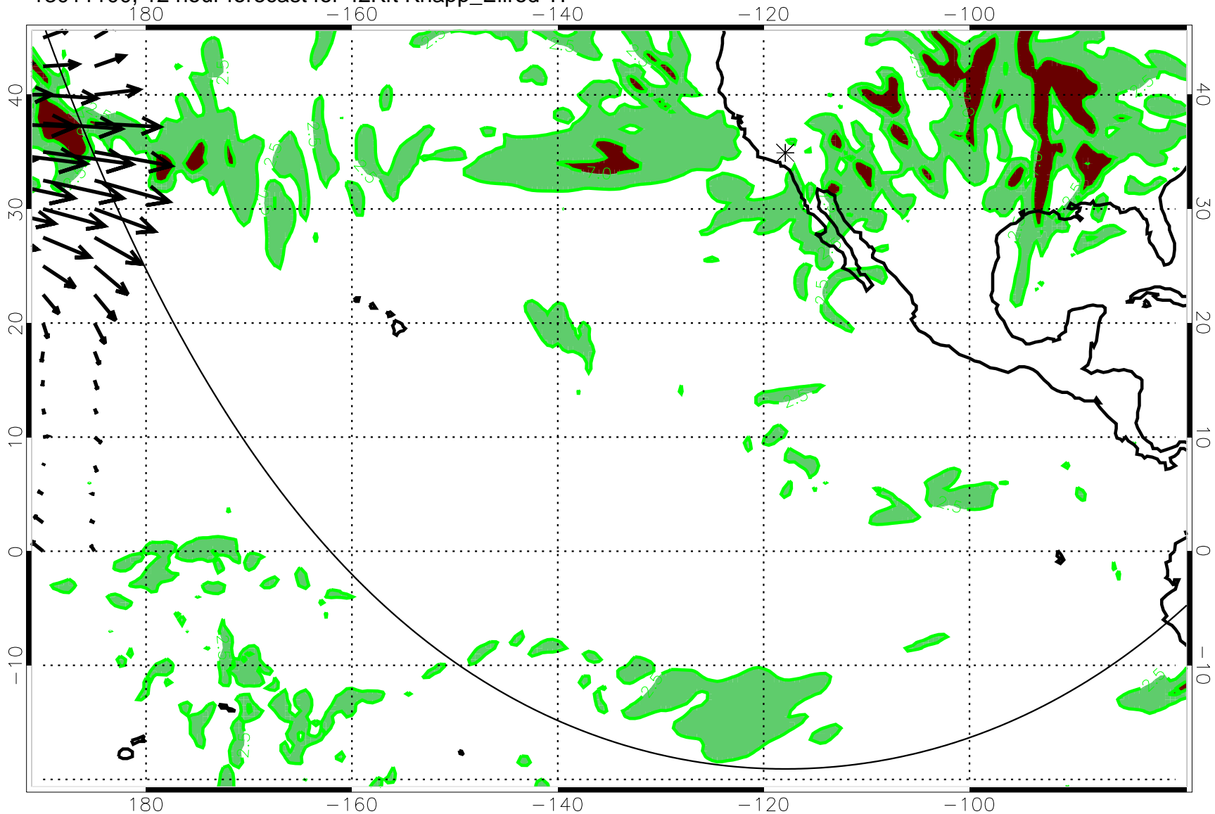
13011100, 12 hour forecast for 42Kft Knapp_Ellrod TI
