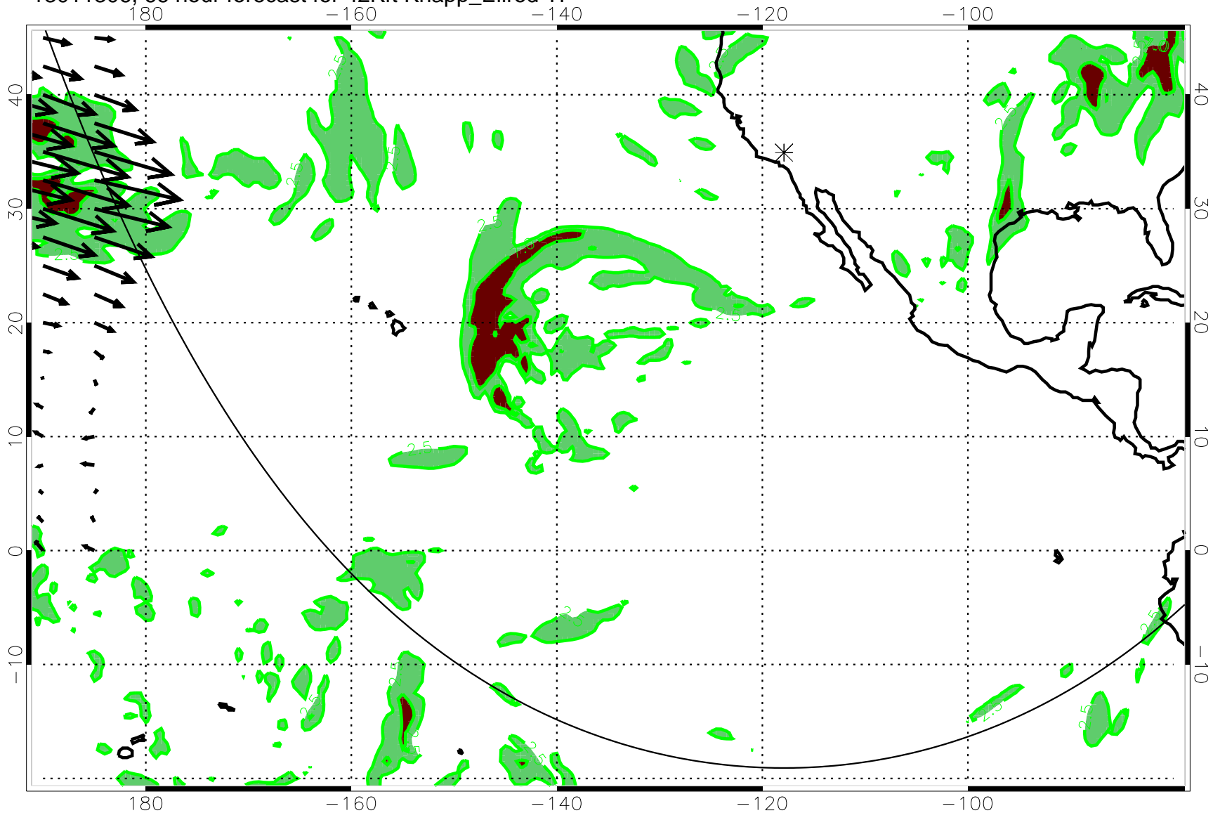
13011306, 66 hour forecast for 42Kft Knapp_Ellrod TI
