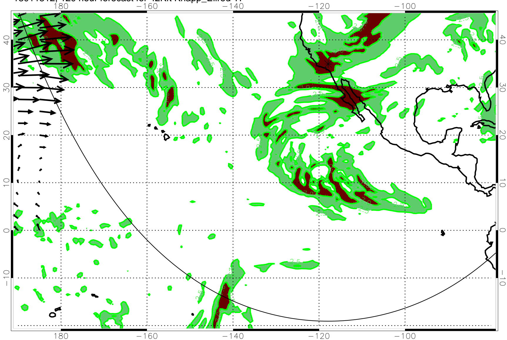
13011512, 120 hour forecast for 42Kft Knapp_Ellrod TI
