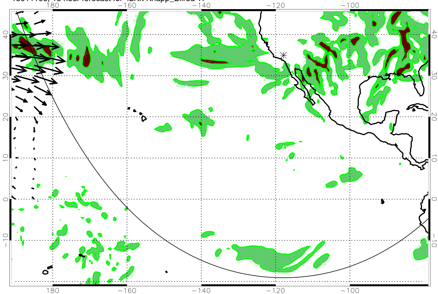
13011106, 18 hour forecast for 42Kft Knapp_Ellrod TI
