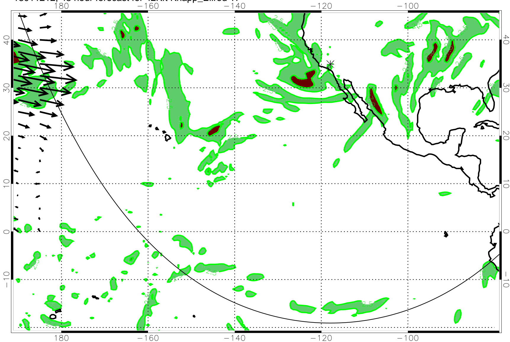
13011212, 48 hour forecast for 42Kft Knapp_Ellrod TI
