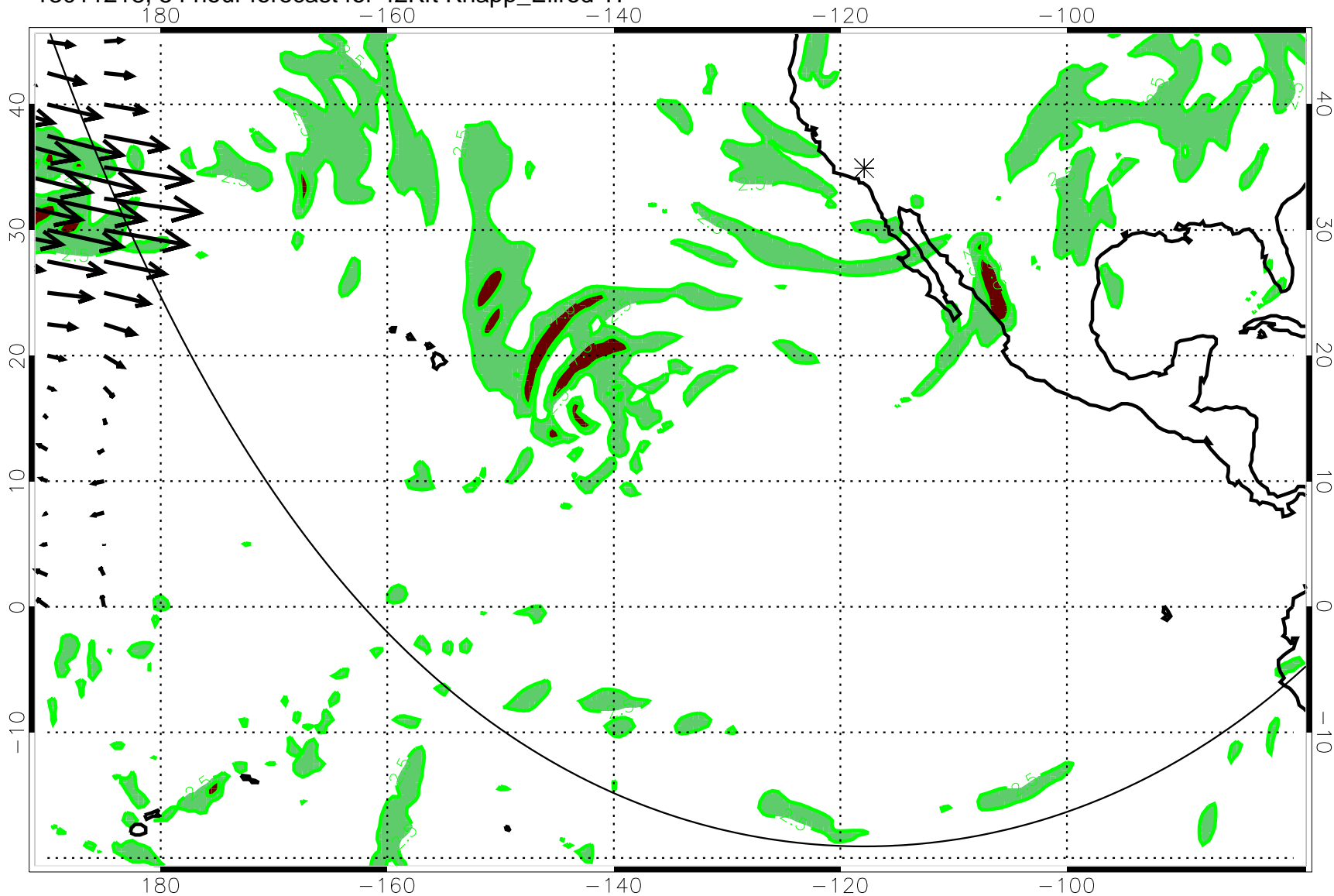
13011218, 54 hour forecast for 42Kft Knapp_Ellrod TI
