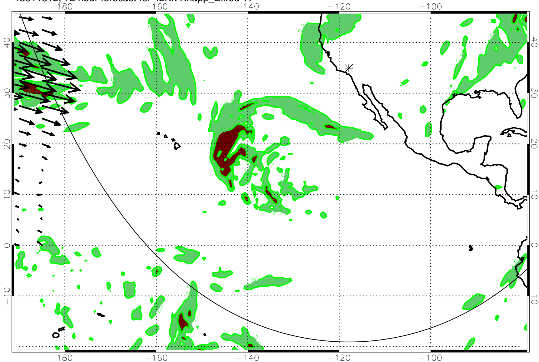
13011312, 72 hour forecast for 42Kft Knapp_Ellrod TI
