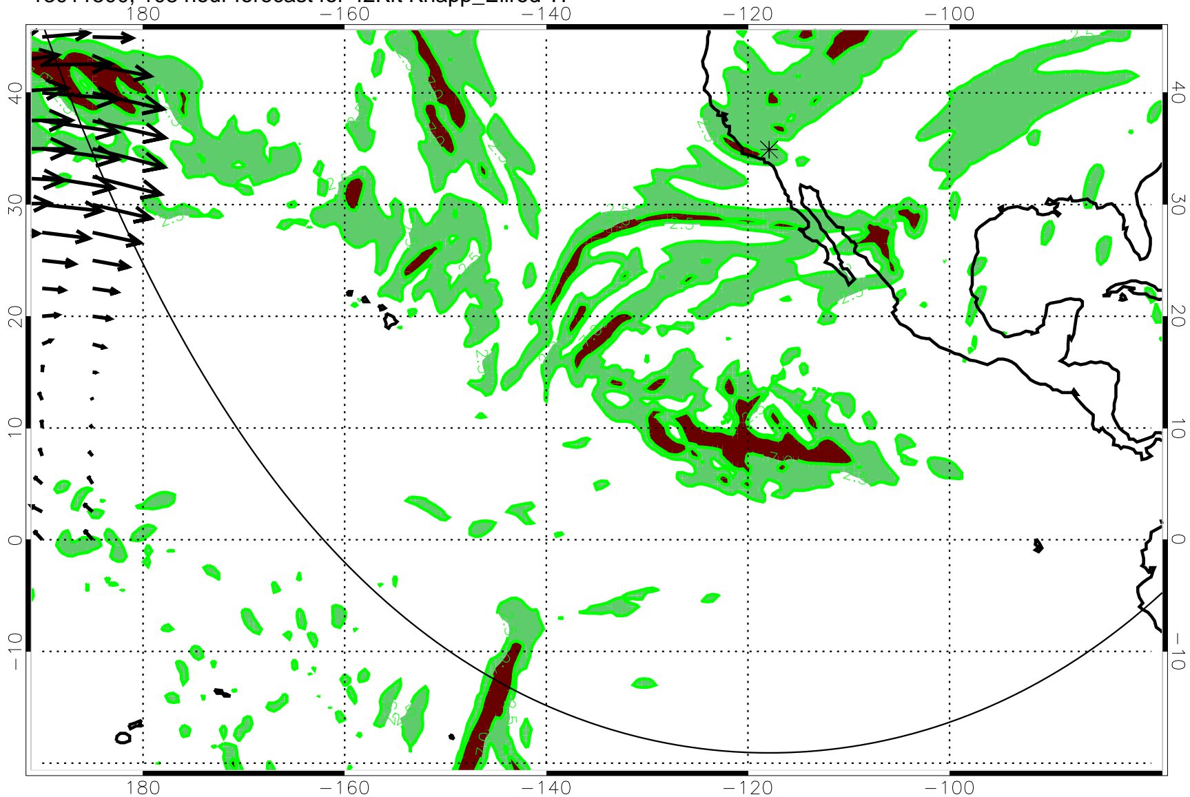
13011500, 108 hour forecast for 42Kft Knapp_Ellrod T1
