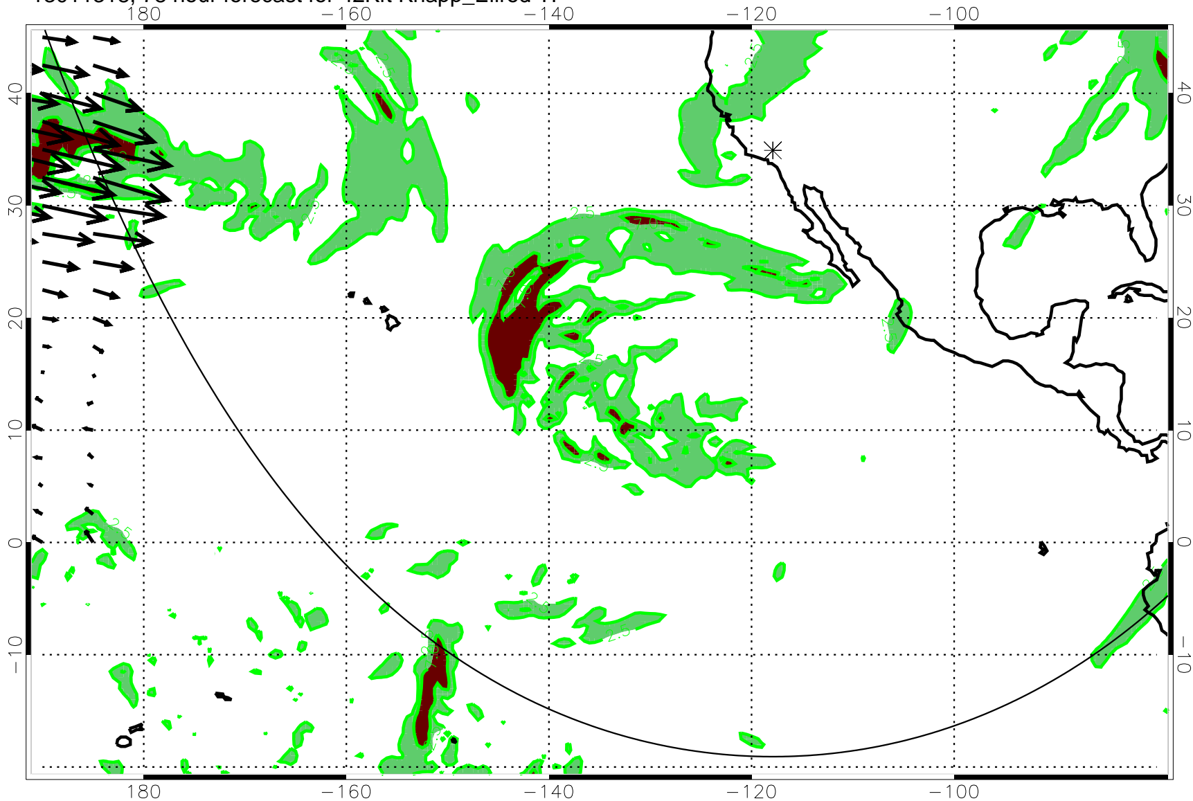
13011318, 78 hour forecast for 42Kft Knapp_Ellrod TI
