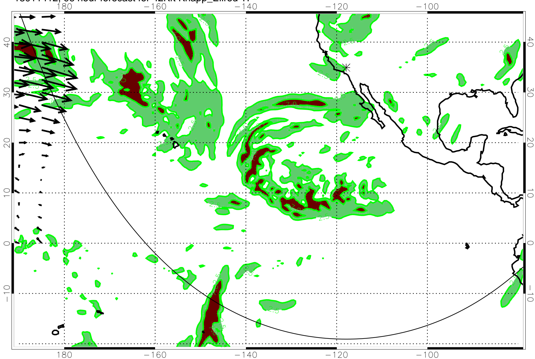
13011412, 96 hour forecast for 42Kft Knapp_Ellrod TI
