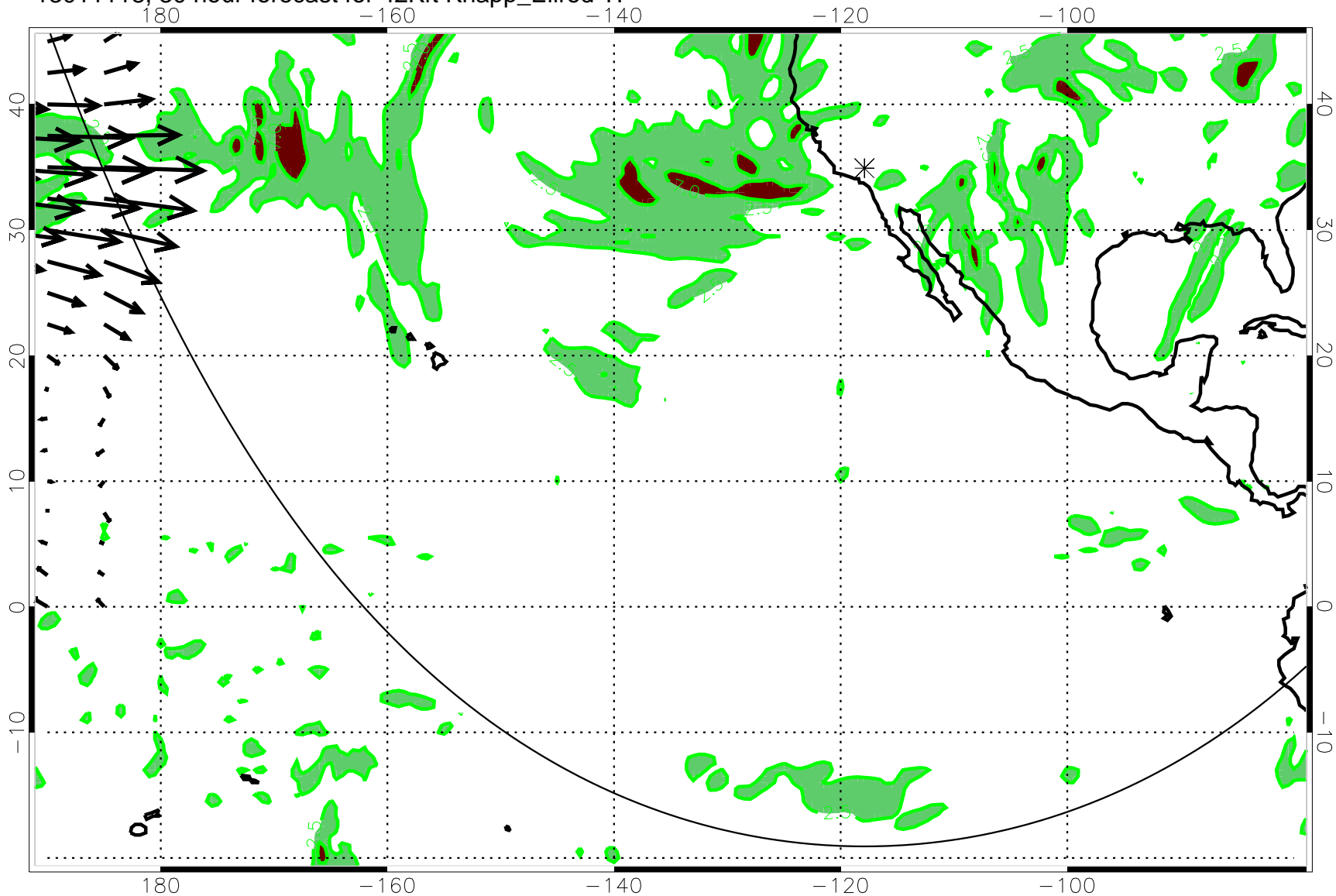
13011118, 30 hour forecast for 42Kft Knapp_Ellrod TI
