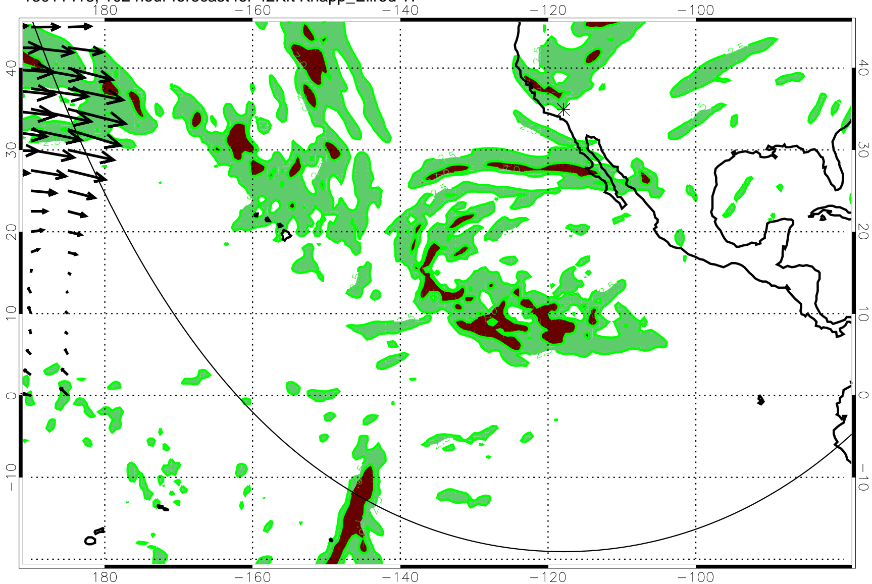
13011418, 102 hour forecast for 42Kft Knapp_Ellrod TI
