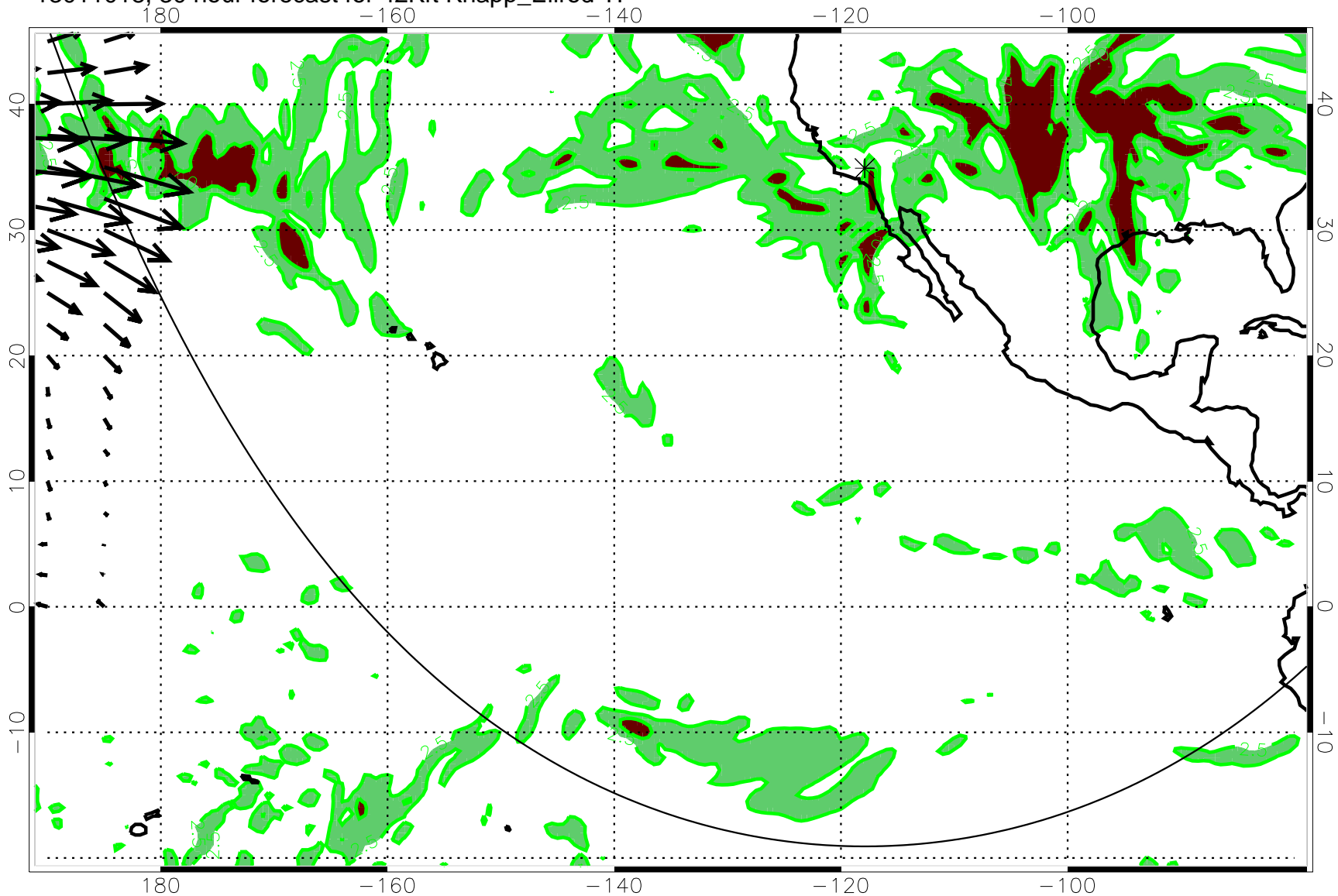
13011018, 30 hour forecast for 42Kft Knapp_Ellrod TI
