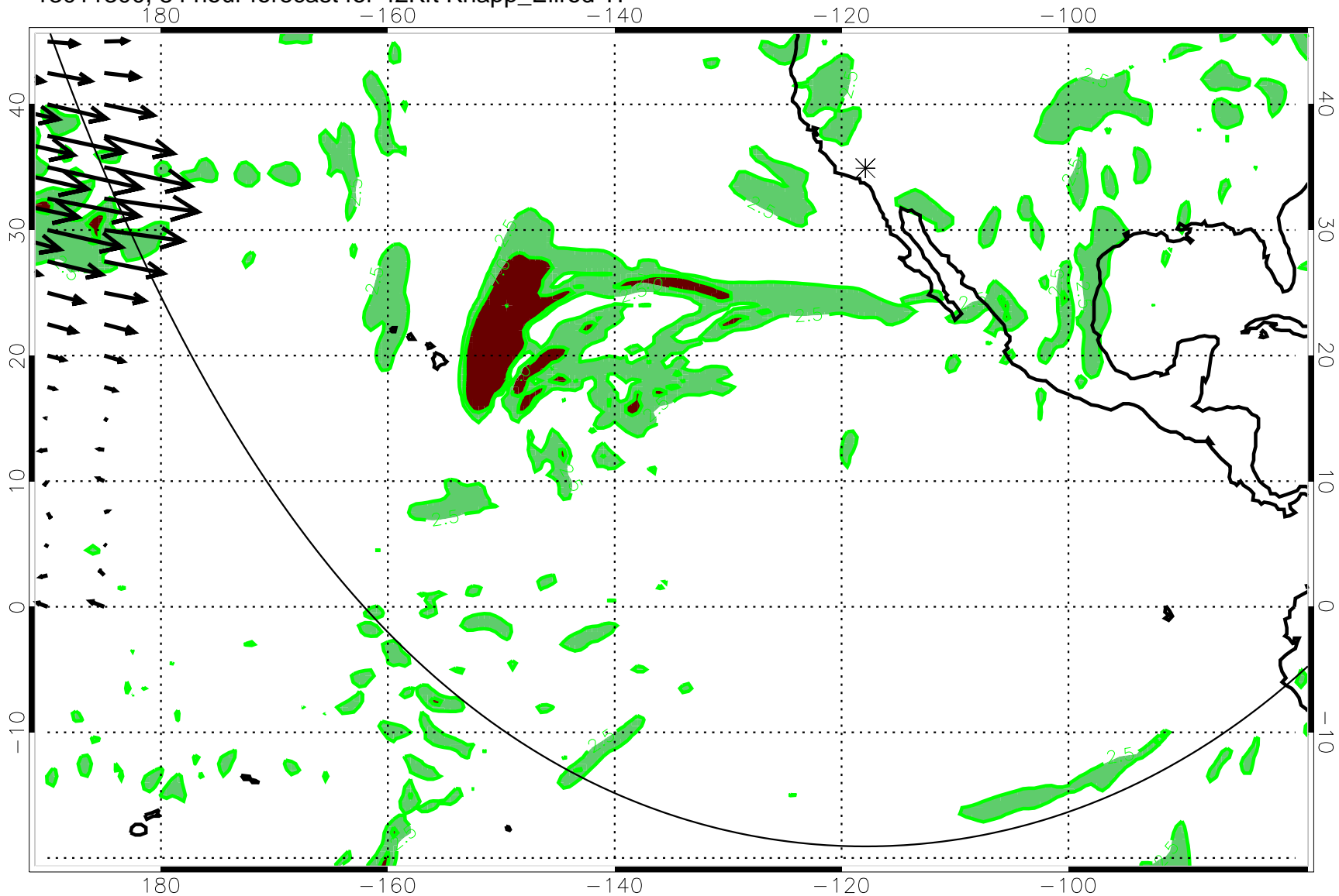
13011300, 84 hour forecast for 42Kft Knapp_Ellrod TI
