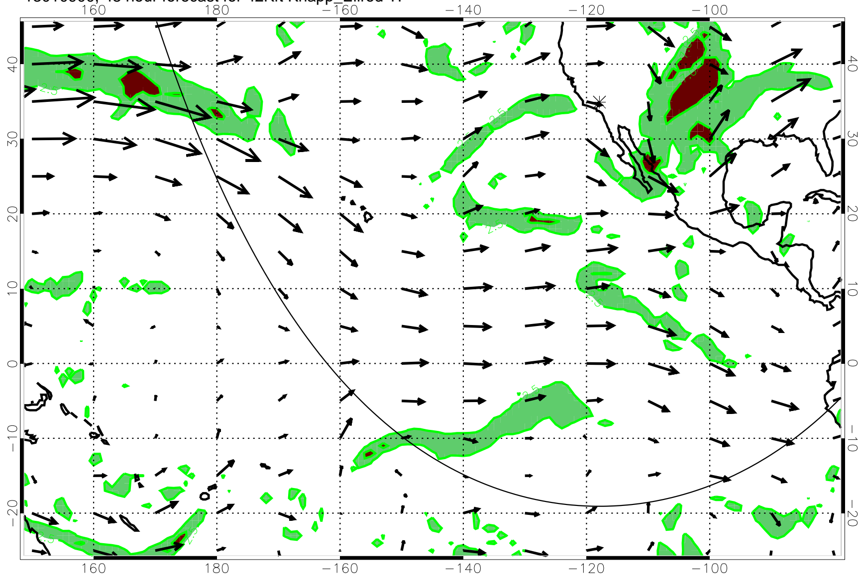
13010900, 48 hour forecast for 42Kft Knapp_Ellrod T1
