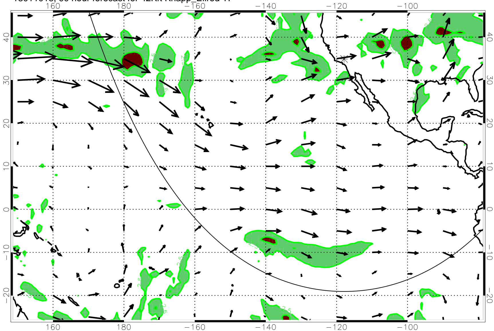
13011018, 90 hour forecast for 42Kft Knapp_Ellrod T1
