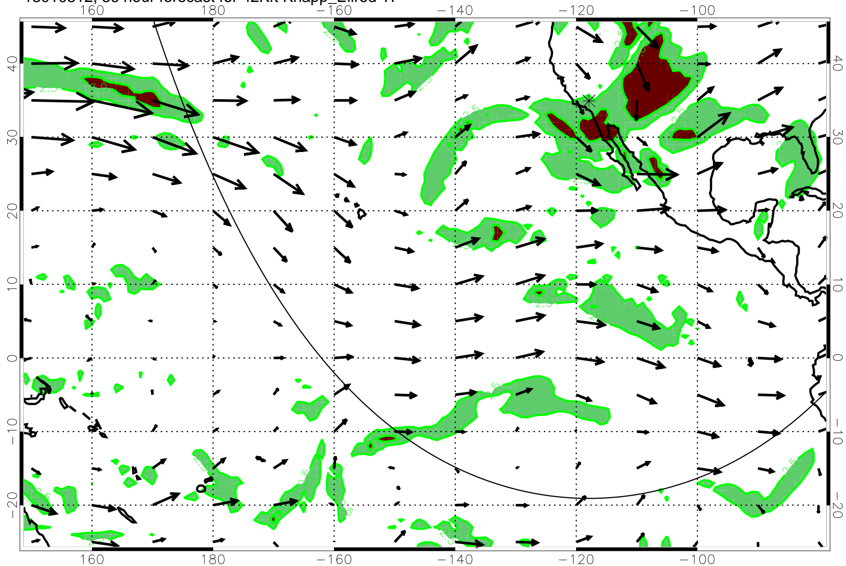
13010812, 36 hour forecast for 42Kft Knapp_Ellrod T1
