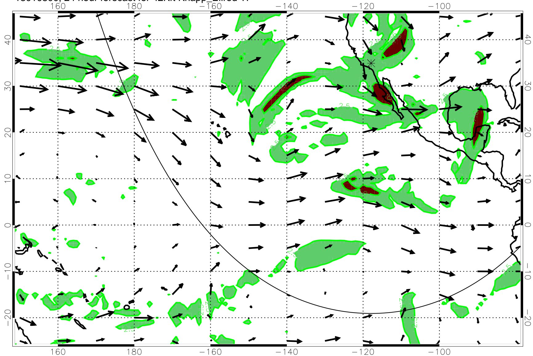
13010800, 24 hour forecast for 42Kft Knapp_Ellrod T1
