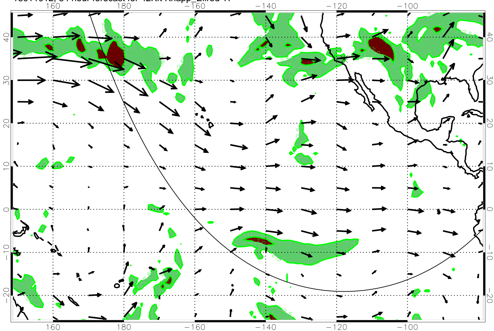
13011012, 84 hour forecast for 42Kft Knapp_Ellrod T1
