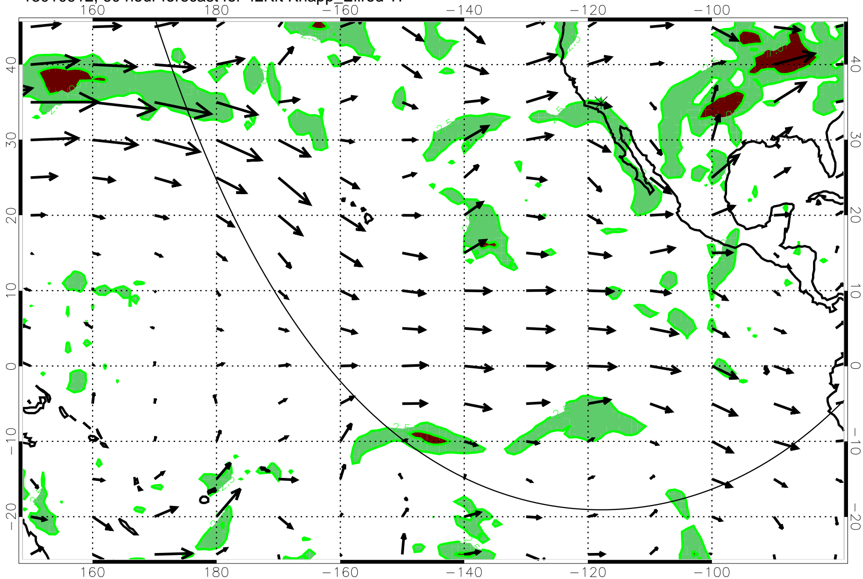
13010912, 60 hour forecast for 42Kft Knapp_Ellrod T1
