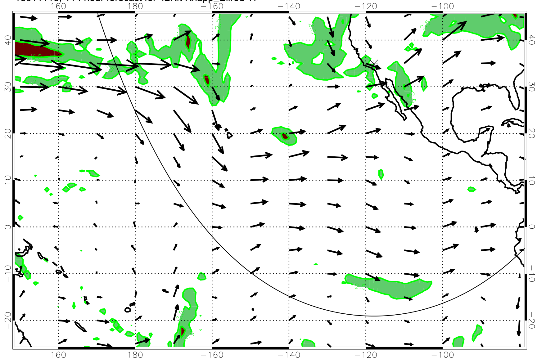
13011118, 114 hour forecast for 42Kft Knapp_Ellrod T1
