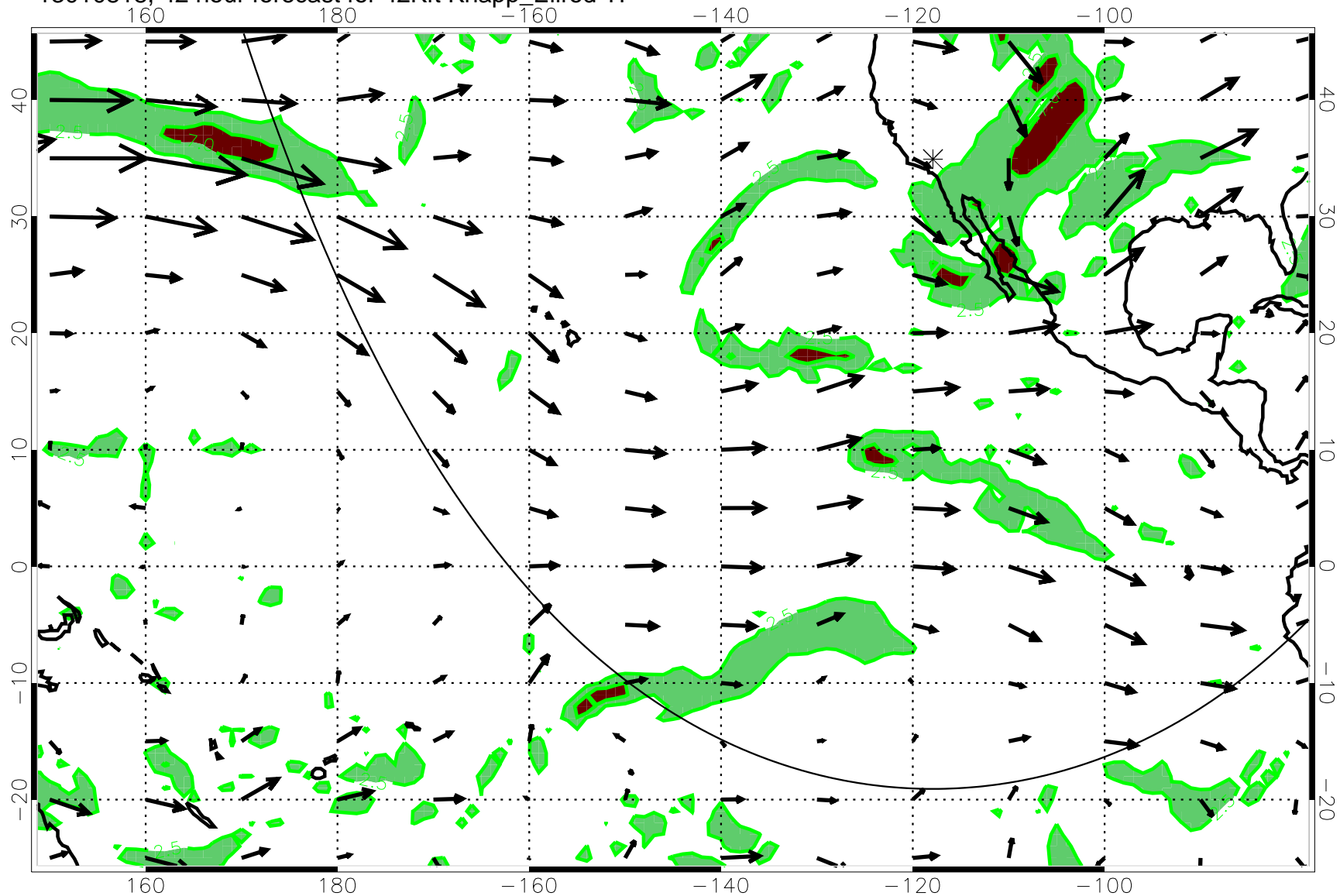
13010818, 42 hour forecast for 42Kft Knapp_Ellrod T1
