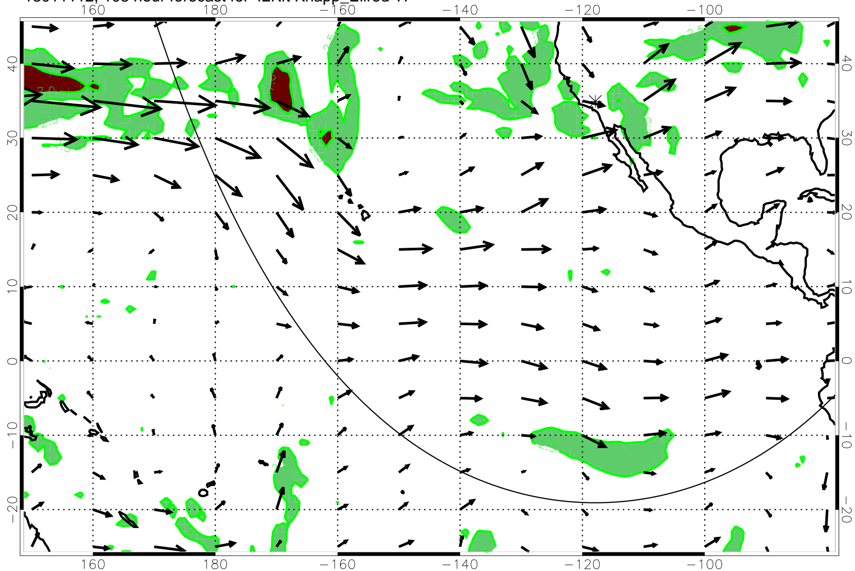
13011112, 108 hour forecast for 42Kft Knapp_Ellrod T1
