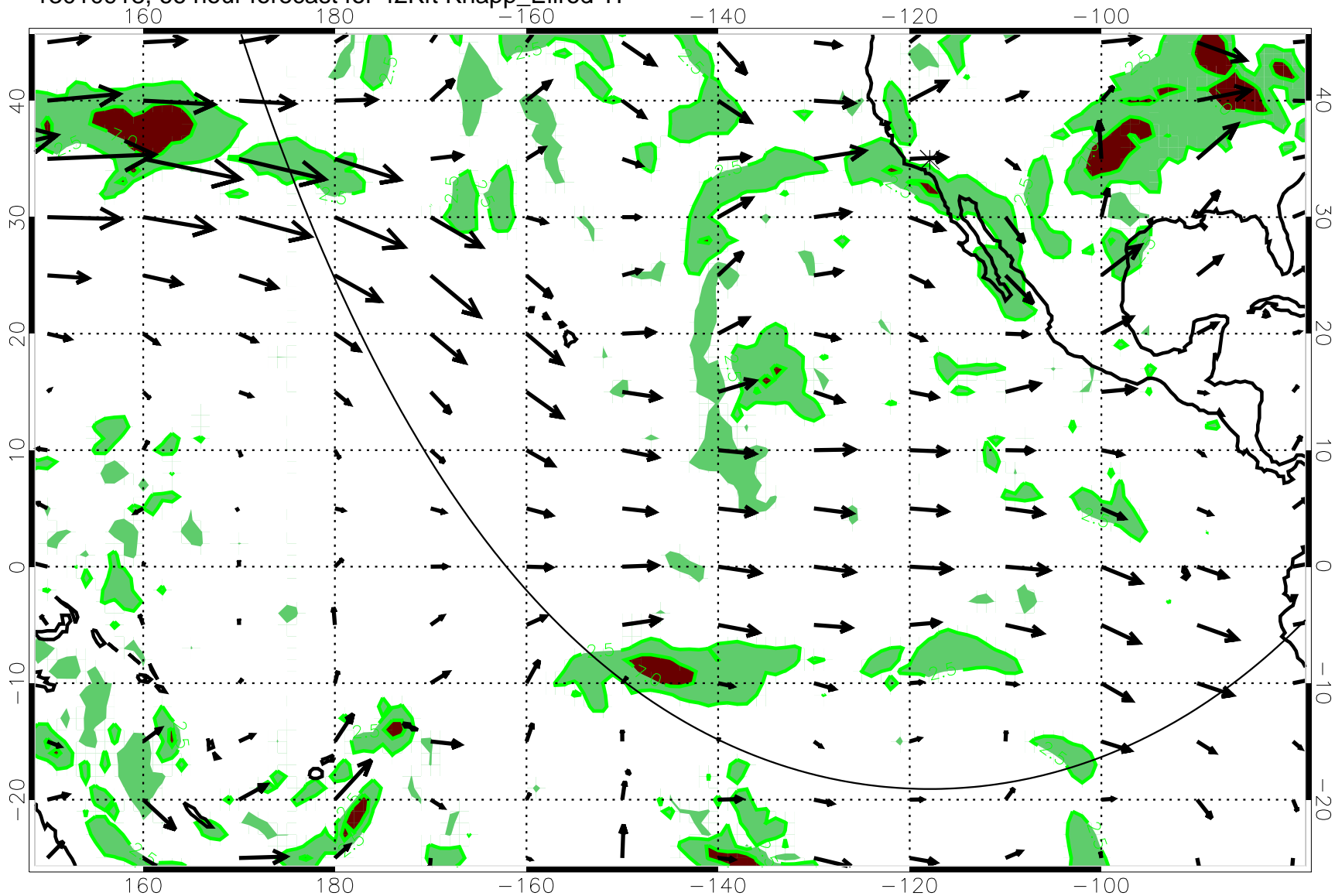
13010918, 66 hour forecast for 42Kft Knapp_Ellrod T1
