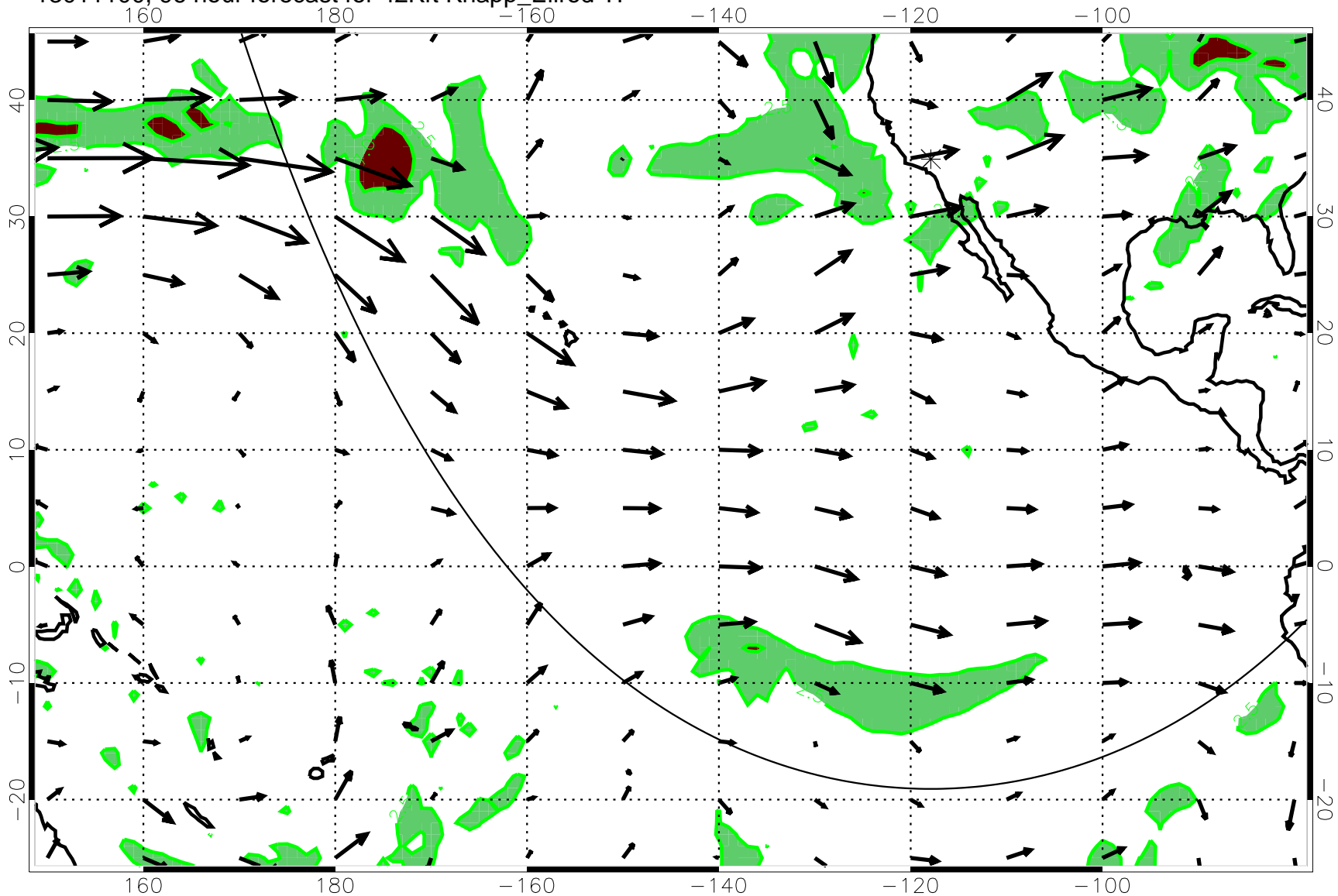
13011100, 96 hour forecast for 42Kft Knapp_Ellrod T1
