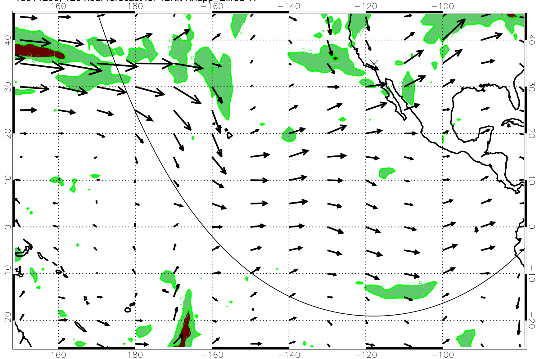
13011200, 120 hour forecast for 42Kft Knapp_Ellrod T1
