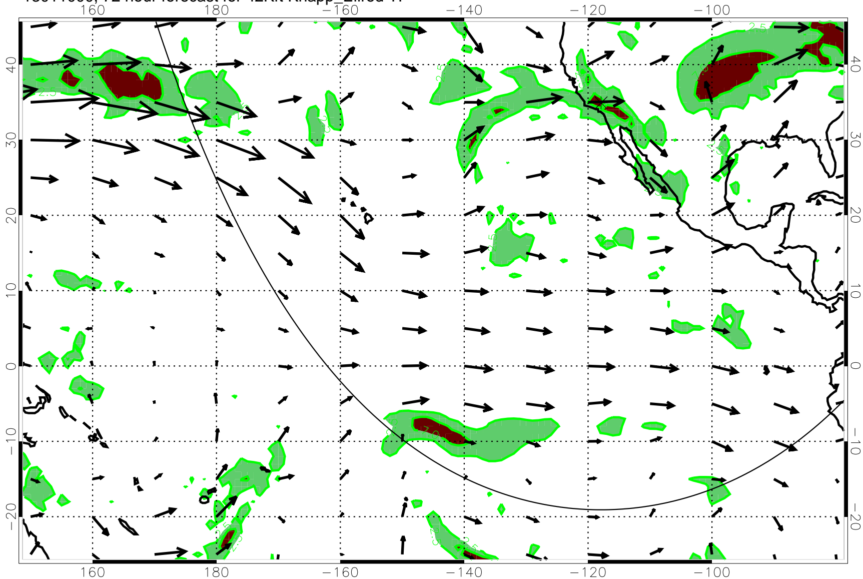
13011000, 72 hour forecast for 42Kft Knapp_Ellrod T1
