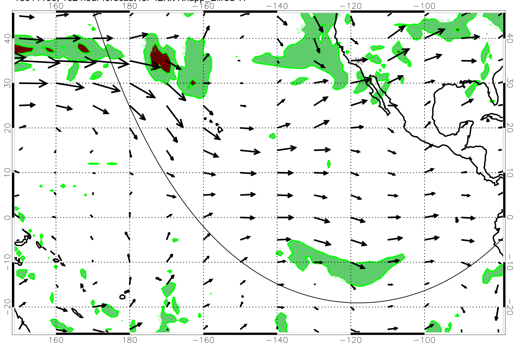
13011106, 102 hour forecast for 42Kft Knapp_Ellrod T1
