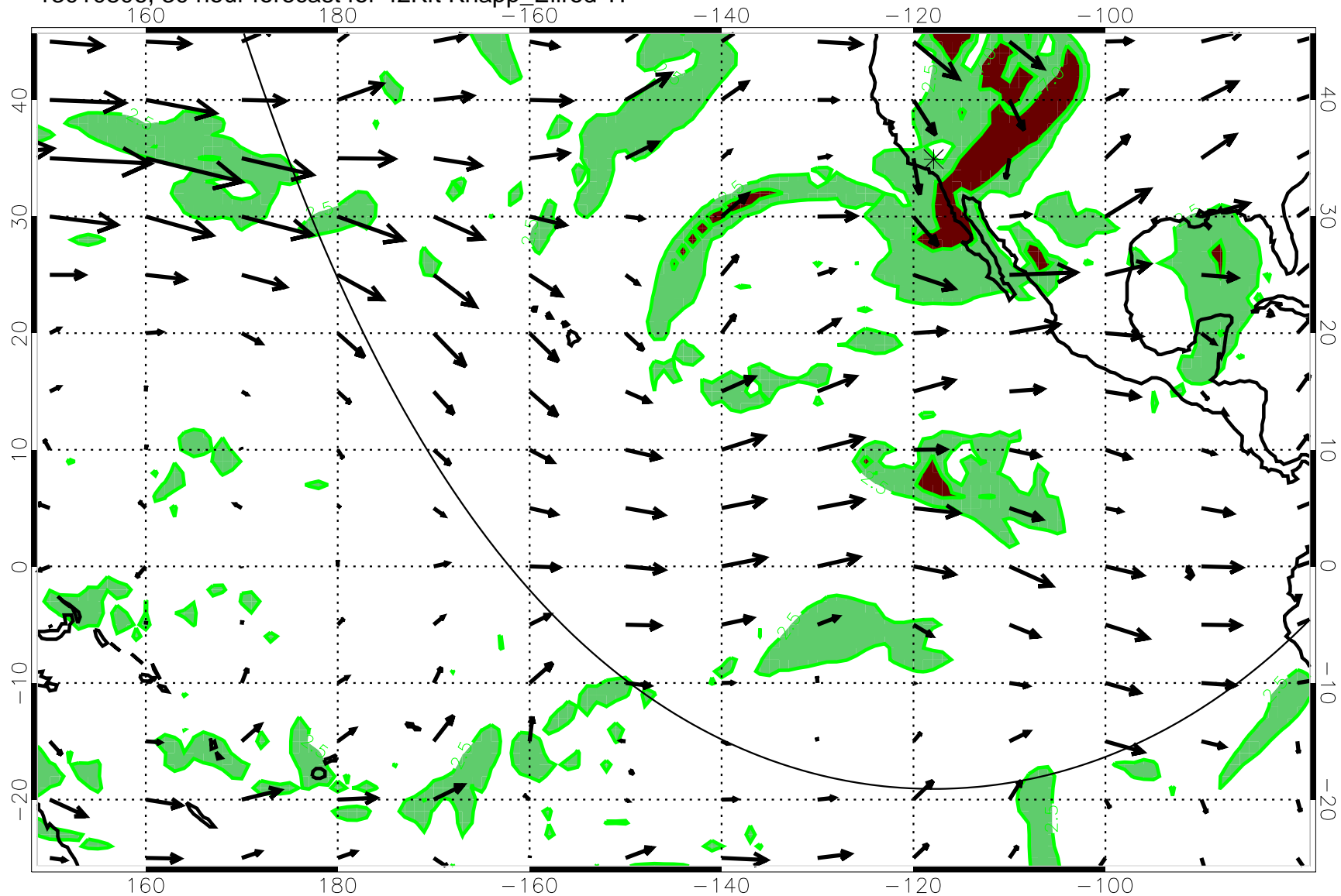
13010806, 30 hour forecast for 42Kft Knapp_Ellrod T1
