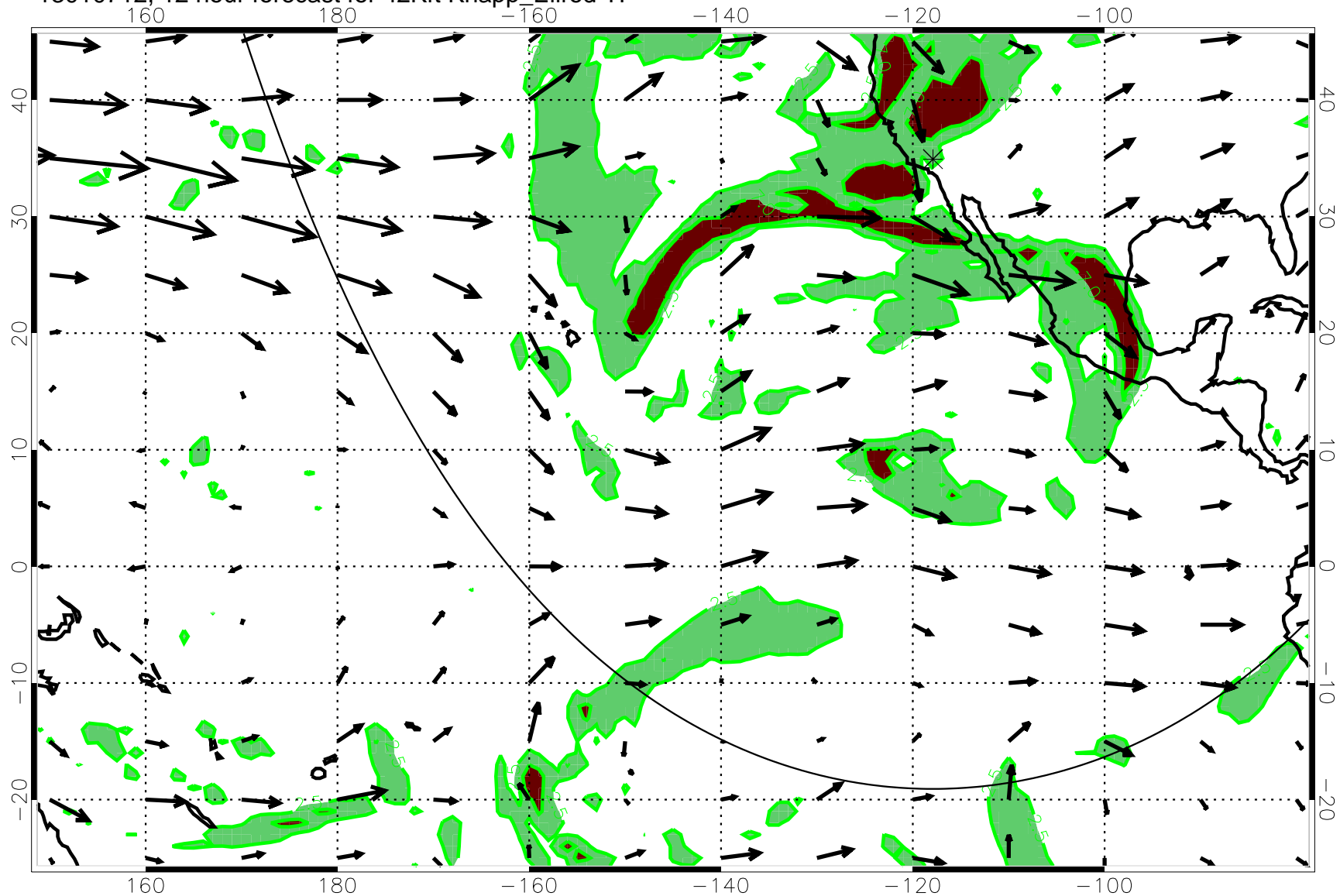
13010712, 12 hour forecast for 42Kft Knapp_Ellrod TI
