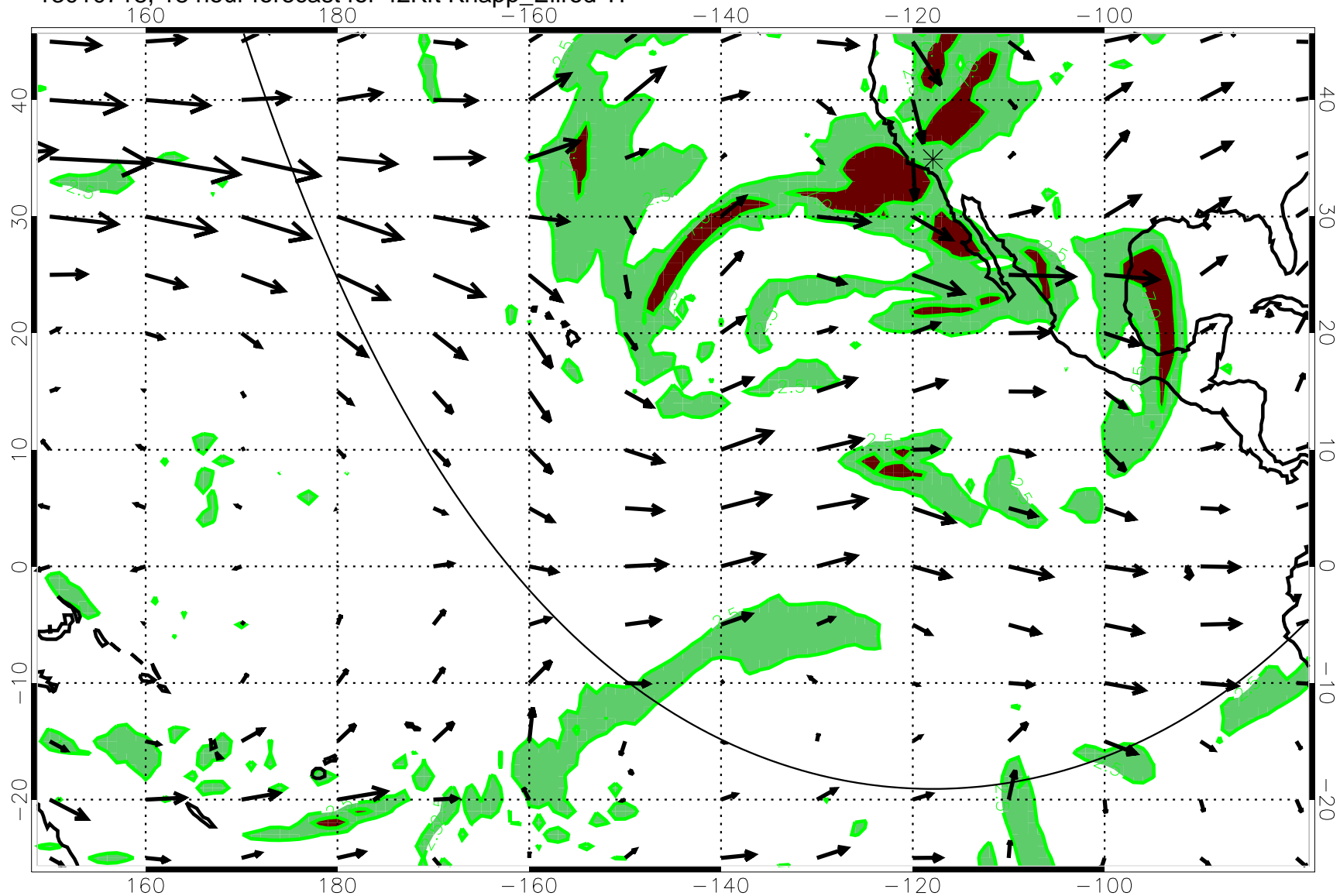
13010718, 18 hour forecast for 42Kft Knapp_Ellrod TI
