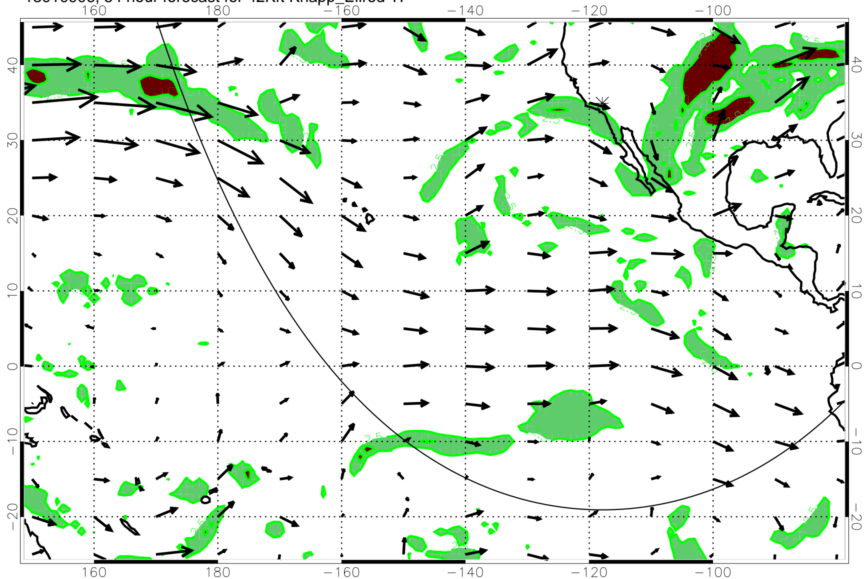
13010906, 54 hour forecast for 42Kft Knapp_Ellrod T1
