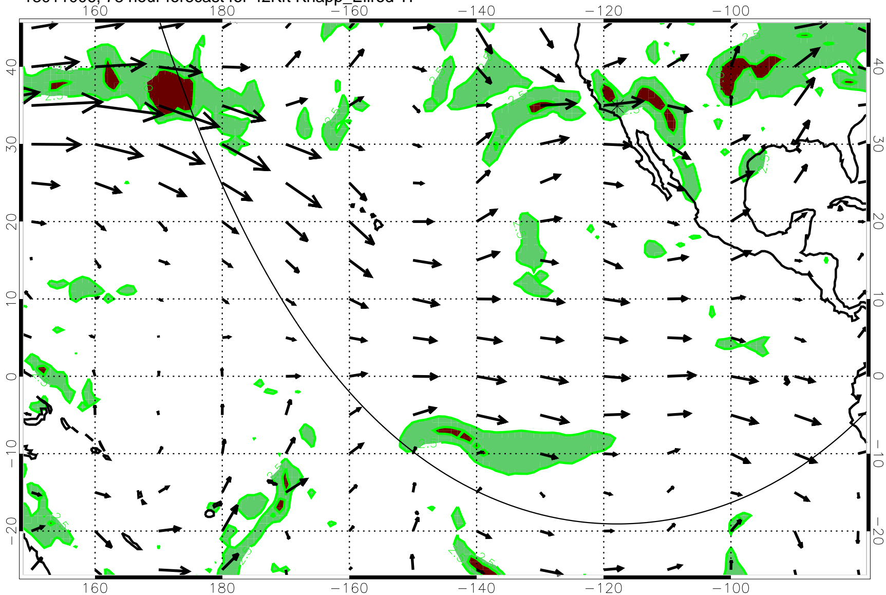
13011006, 78 hour forecast for 42Kft Knapp_Ellrod T1
