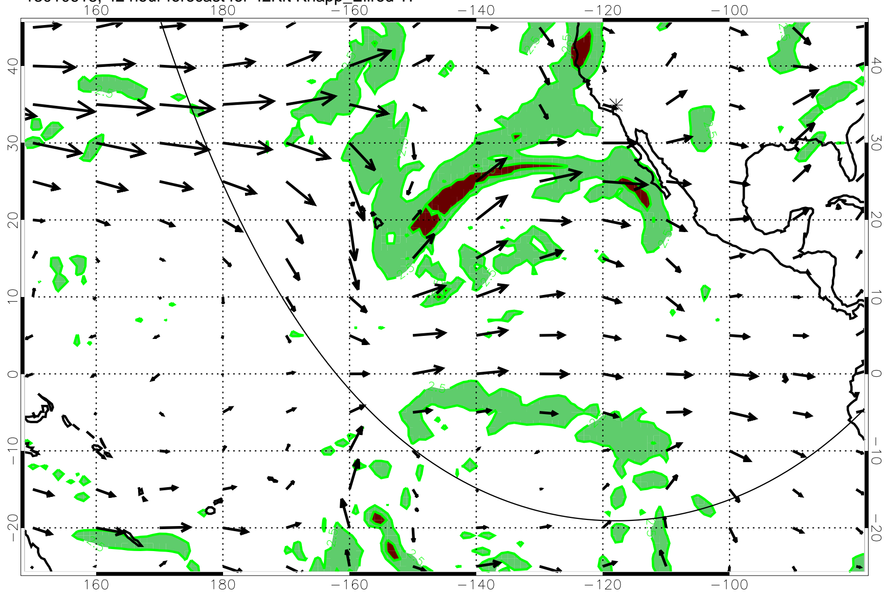
13010618, 42 hour forecast for 42Kft Knapp_Ellrod T1
