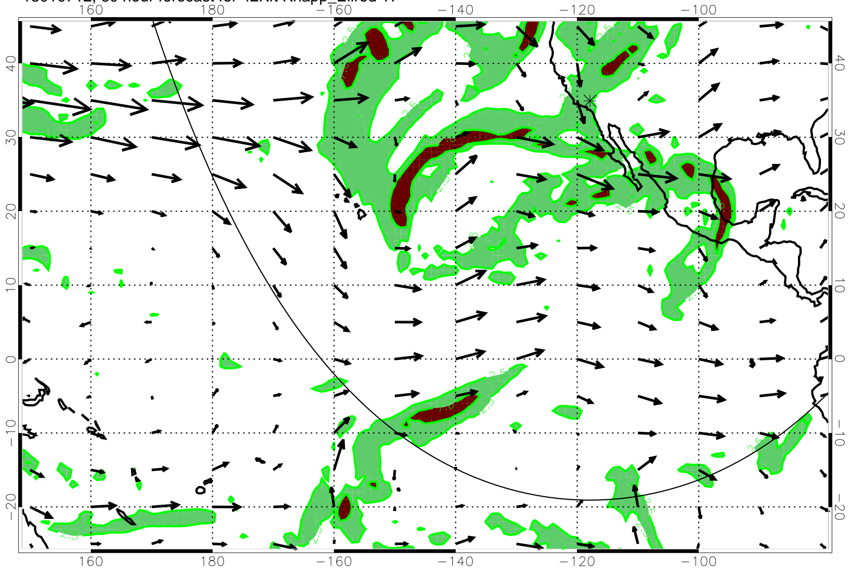
13010712, 60 hour forecast for 42Kft Knapp_Ellrod TI
