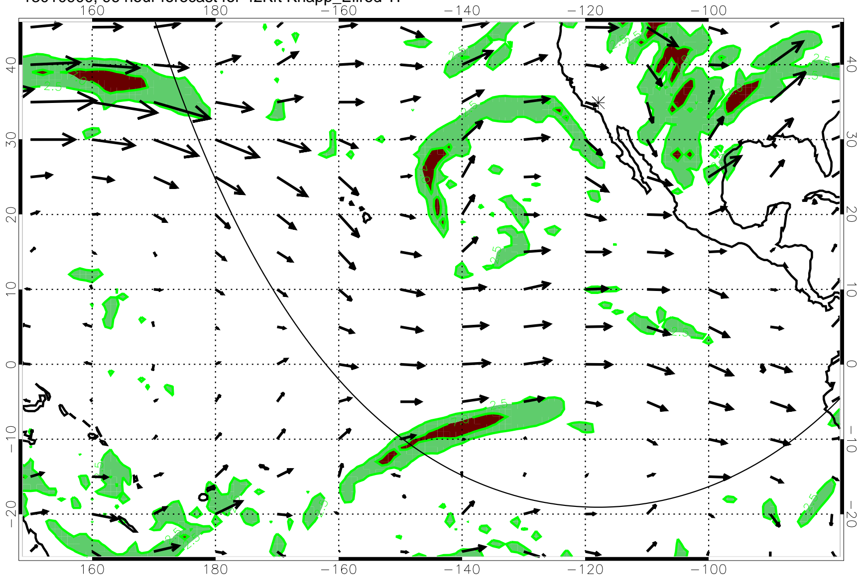
13010900, 96 hour forecast for 42Kft Knapp_Ellrod T1
