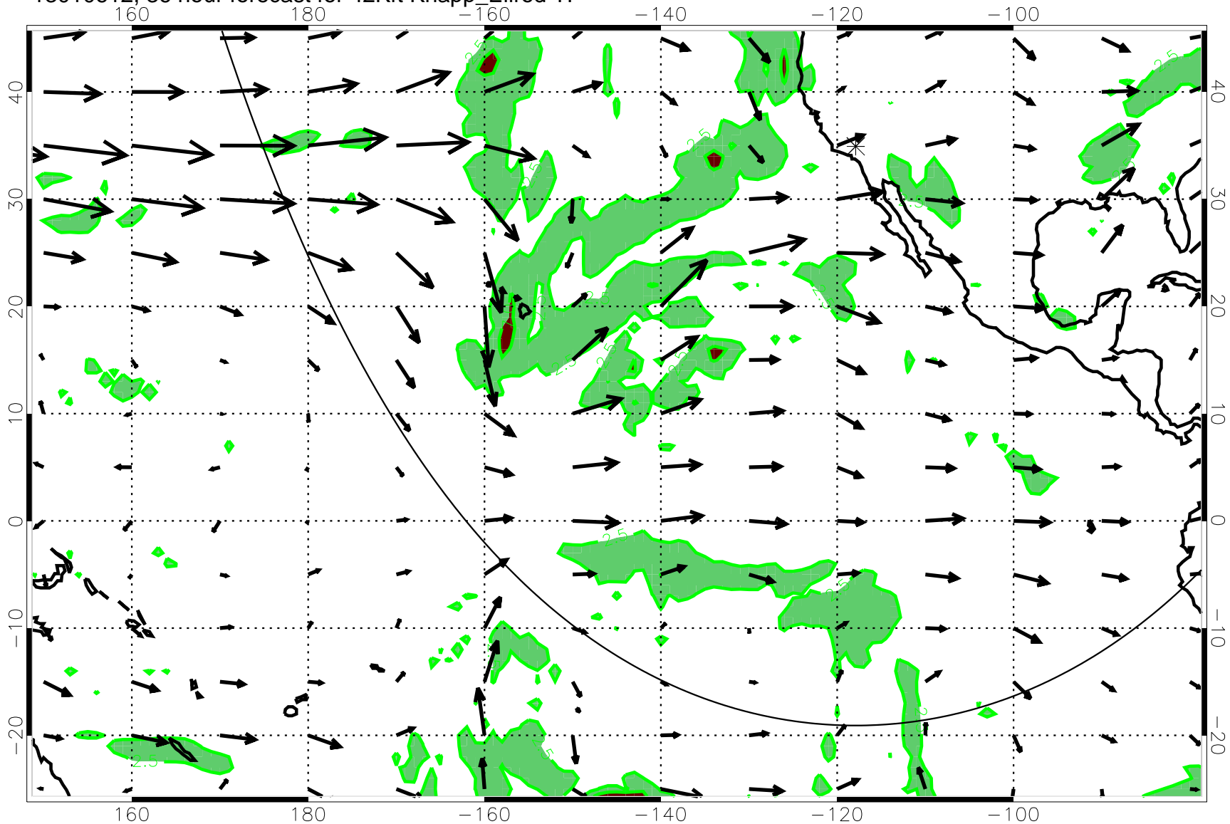
13010612, 36 hour forecast for 42Kft Knapp_Ellrod T1
