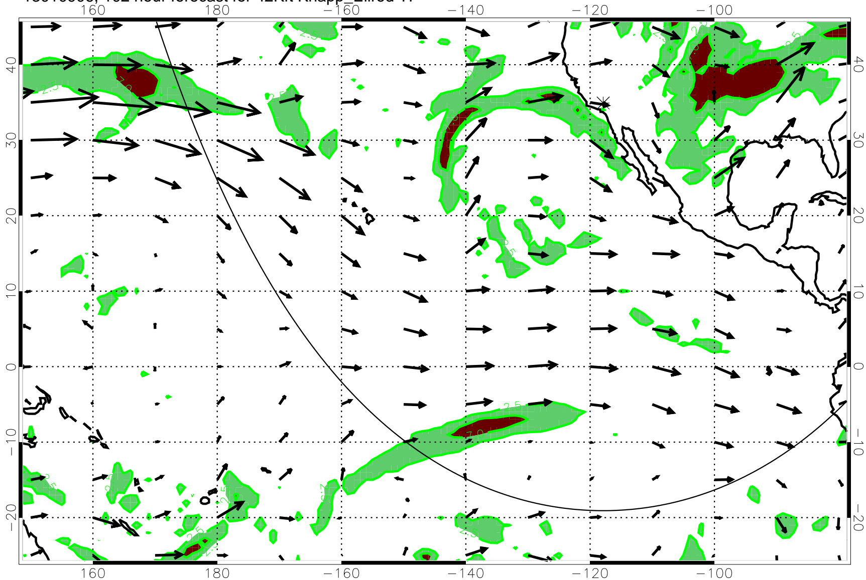
13010906, 102 hour forecast for 42Kft Knapp_Ellrod T1
