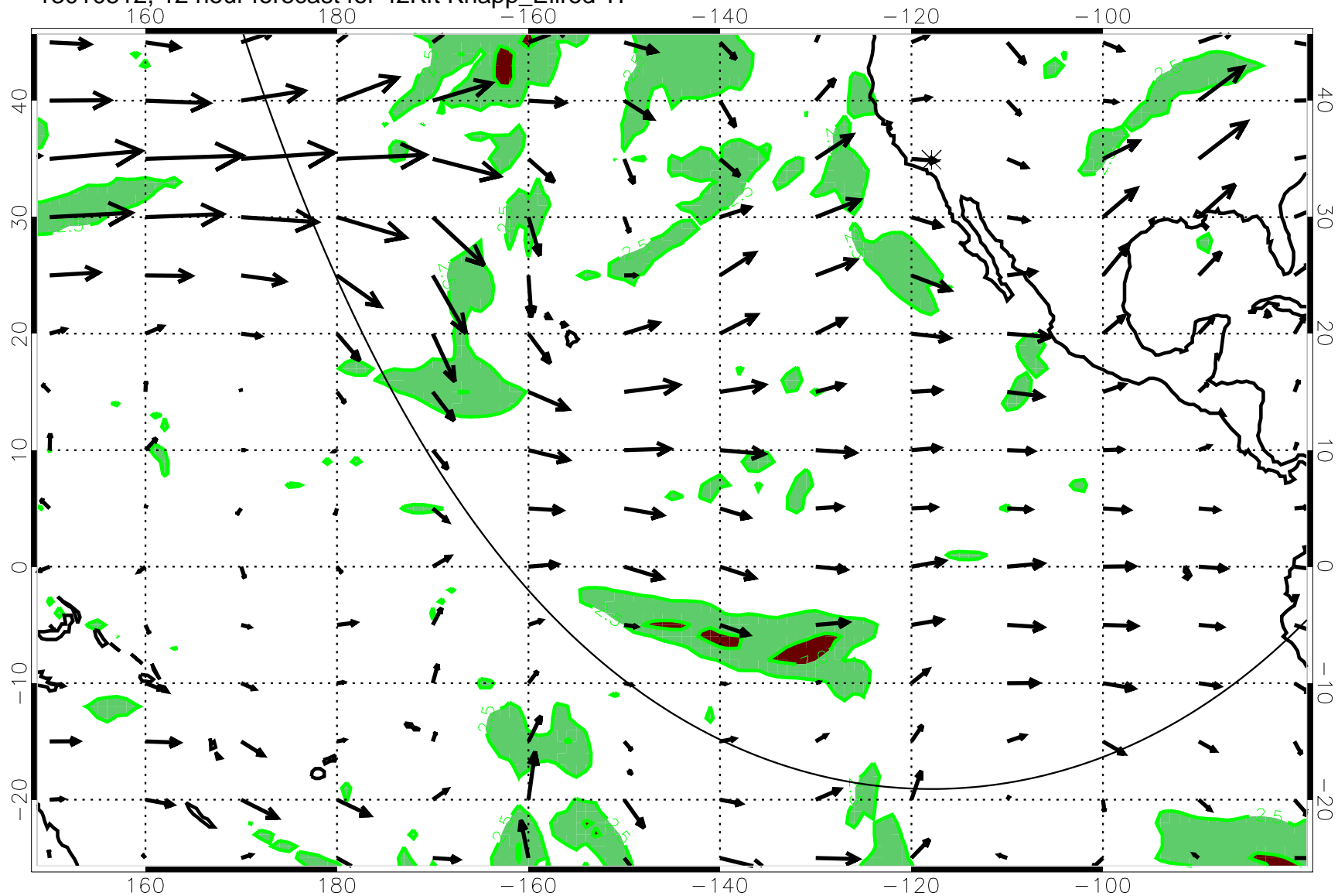
13010512, 12 hour forecast for 42Kft Knapp_Ellrod T1
