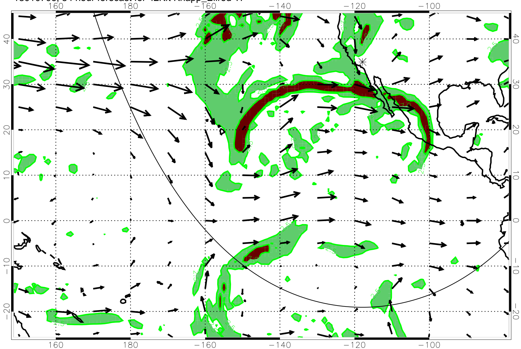
13010706, 54 hour forecast for 42Kft Knapp_Ellrod TI
