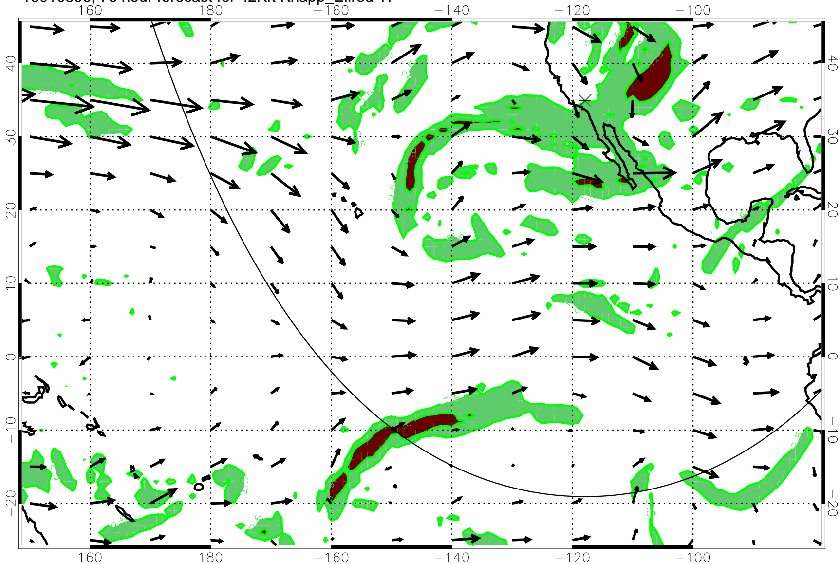
13010806, 78 hour forecast for 42Kft Knapp_Ellrod T1
