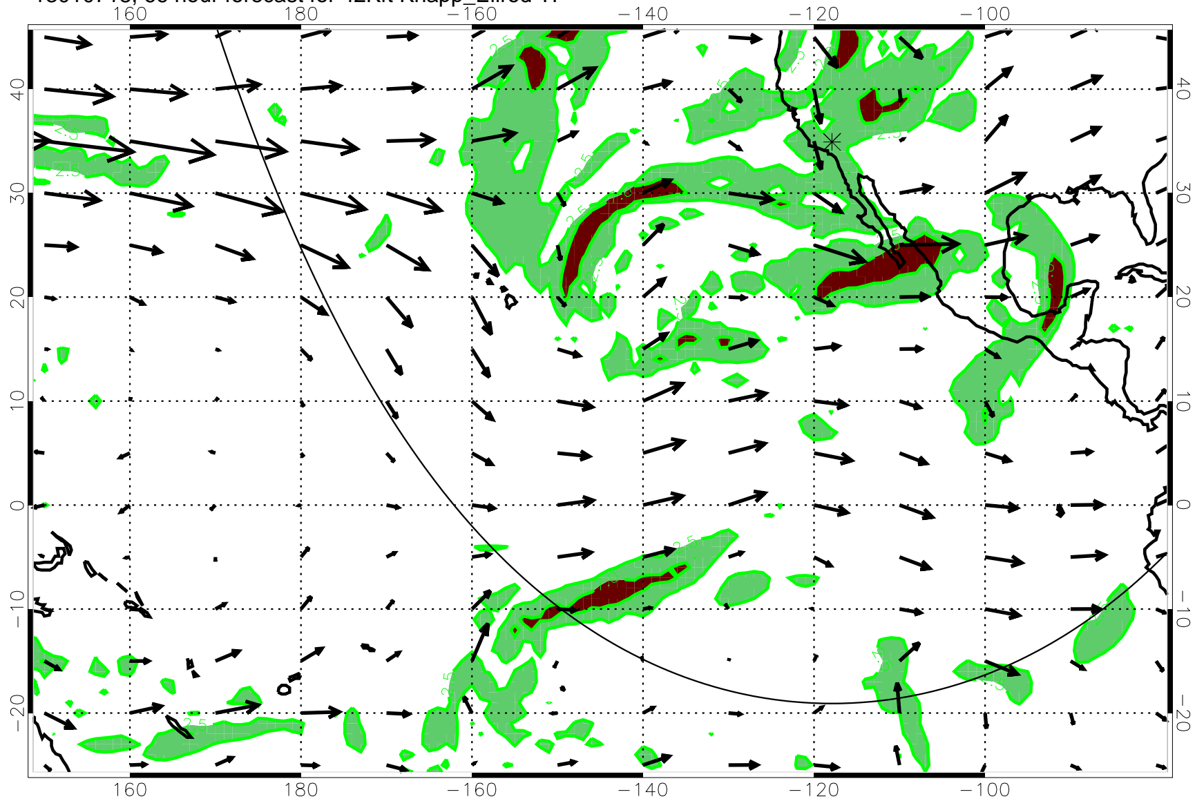
13010718, 66 hour forecast for 42Kft Knapp_Ellrod T1
