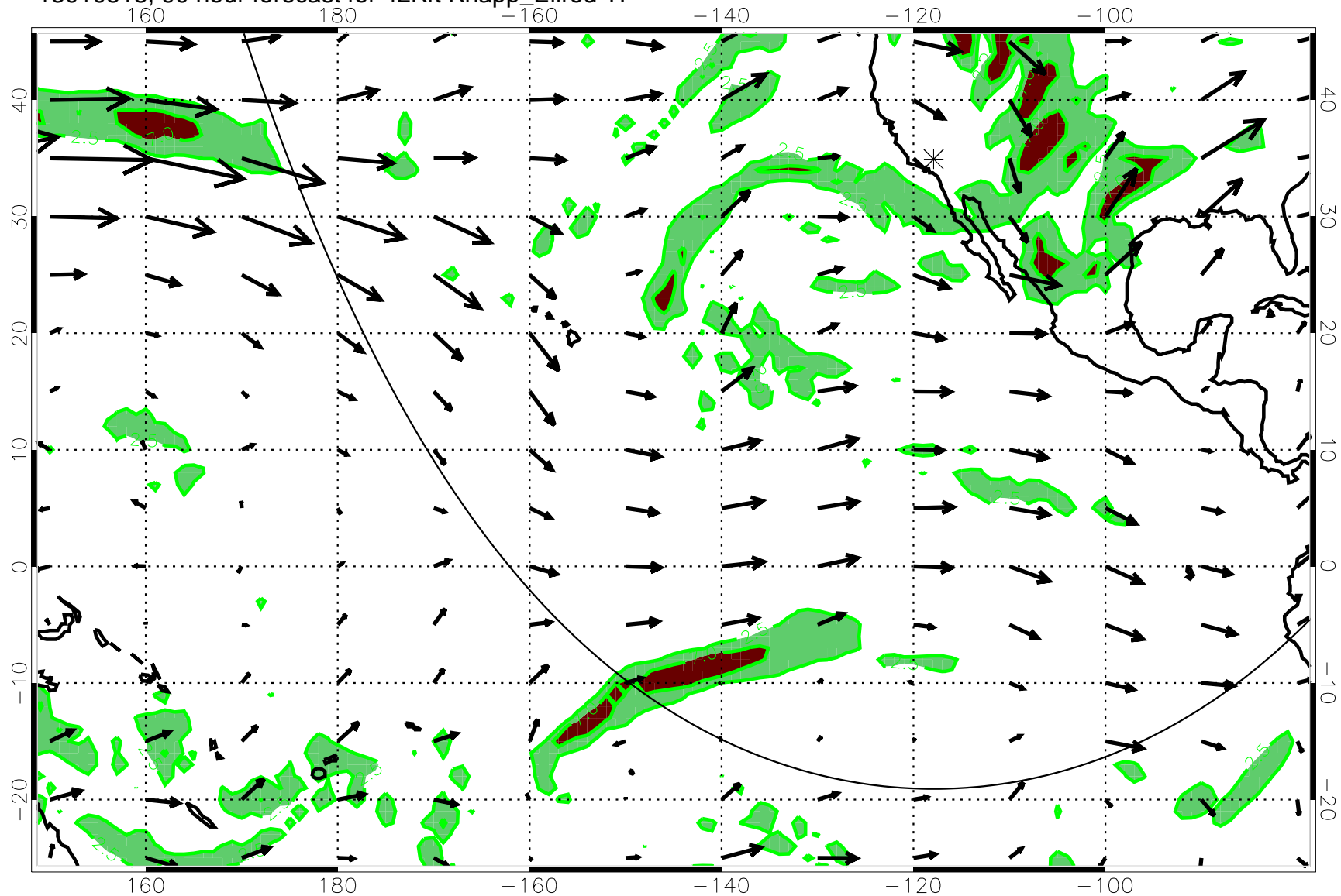
13010818, 90 hour forecast for 42Kft Knapp_Ellrod T1
