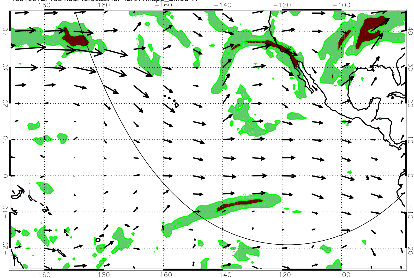
13010912, 108 hour forecast for 42Kft Knapp_Ellrod T1
