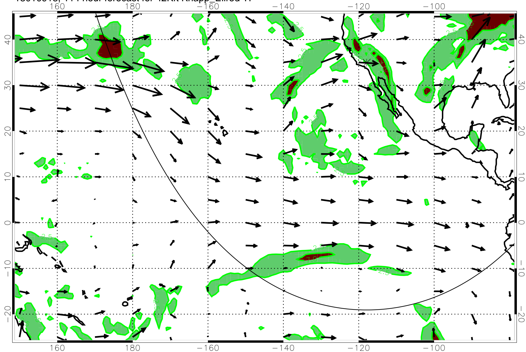
13010918, 114 hour forecast for 42Kft Knapp_Ellrod T1
