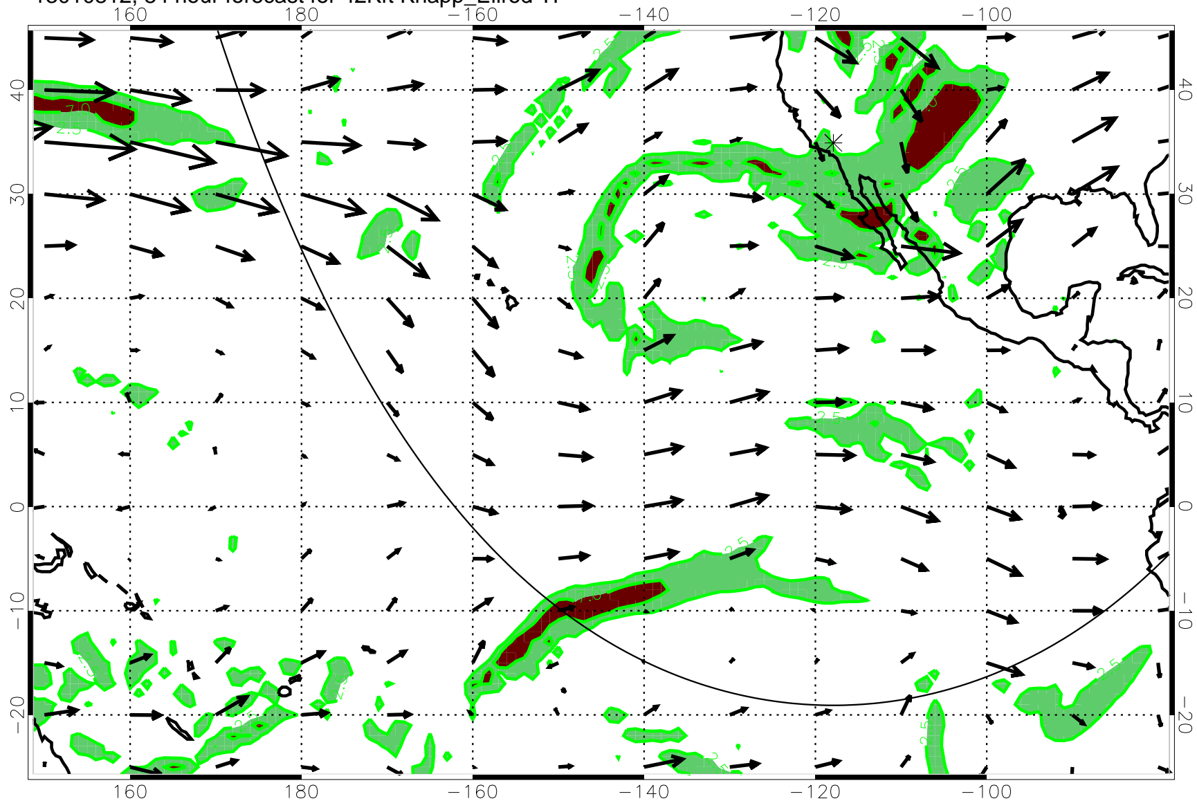
13010812, 84 hour forecast for 42Kft Knapp_Ellrod T1
