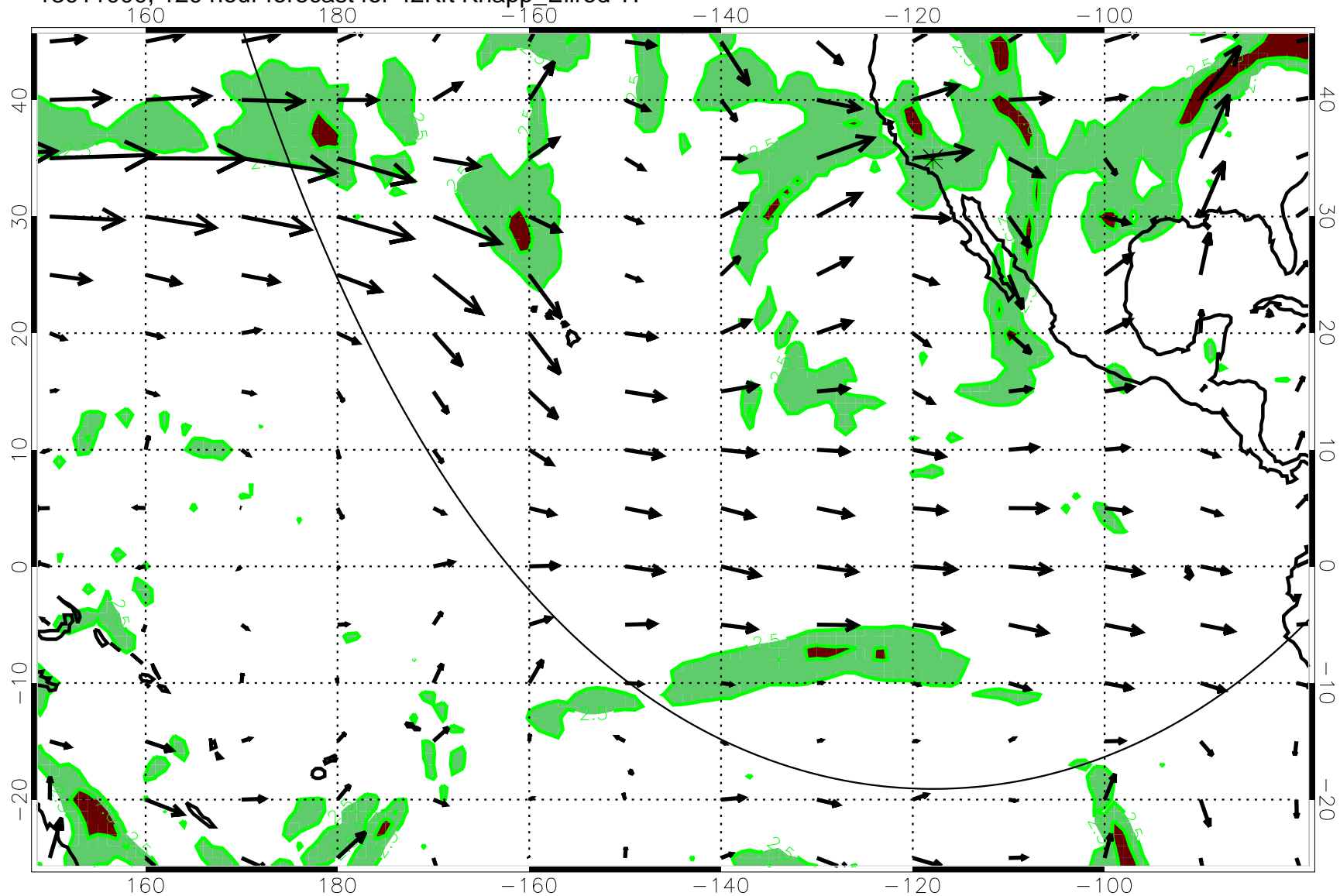
13011000, 120 hour forecast for 42Kft Knapp_Ellrod T1
