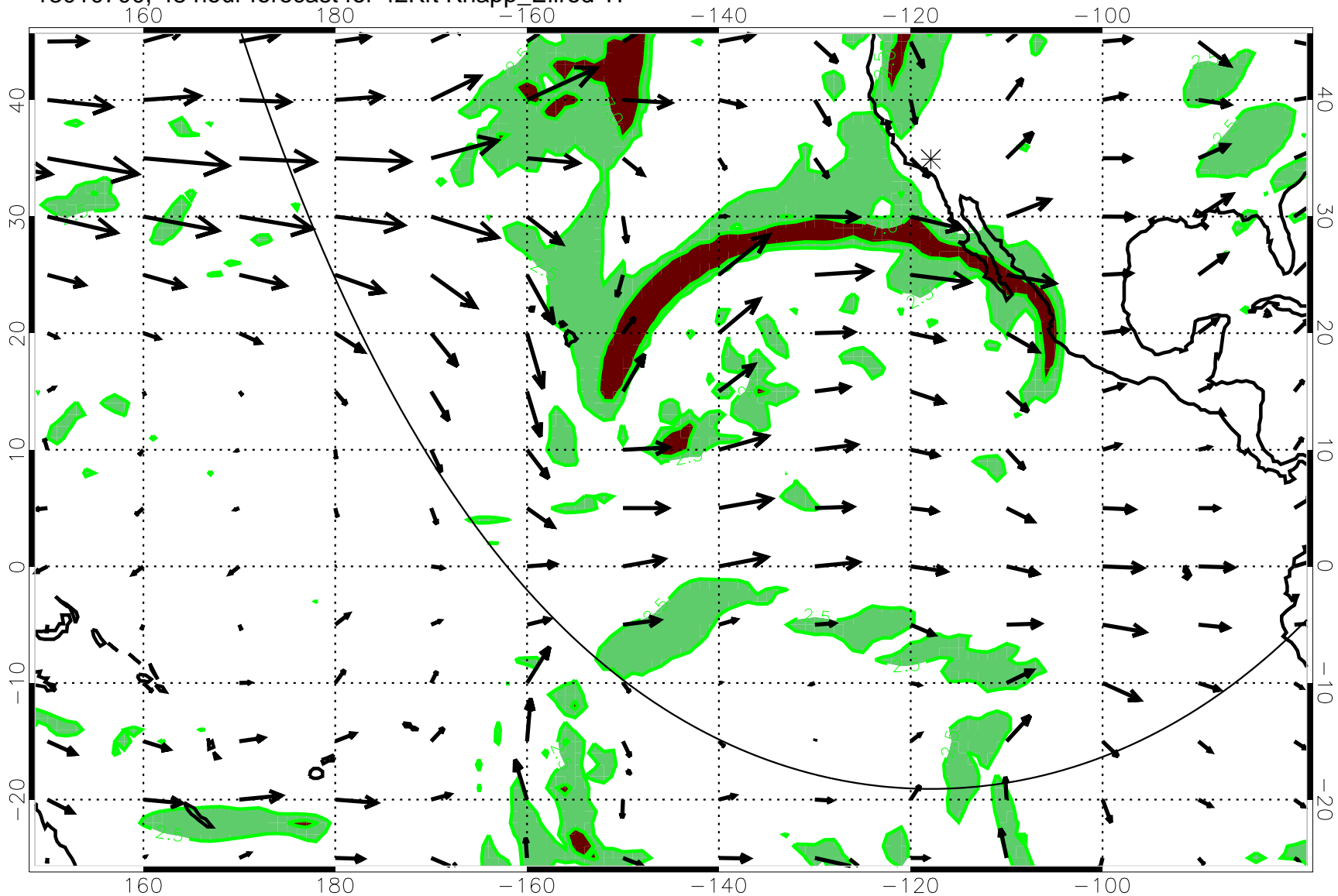
13010700, 48 hour forecast for 42Kft Knapp_Ellrod T1
