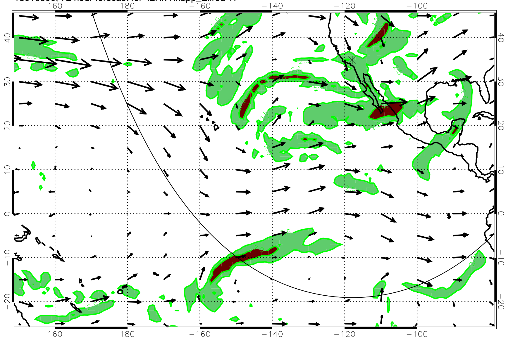
13010800, 72 hour forecast for 42Kft Knapp_Ellrod T1
