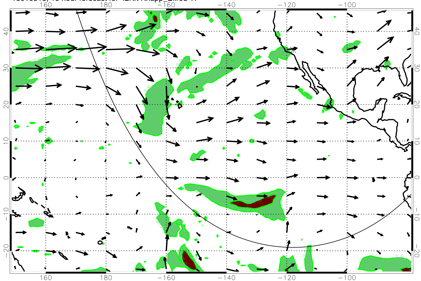
13010518, 18 hour forecast for 42Kft Knapp_Ellrod TI
