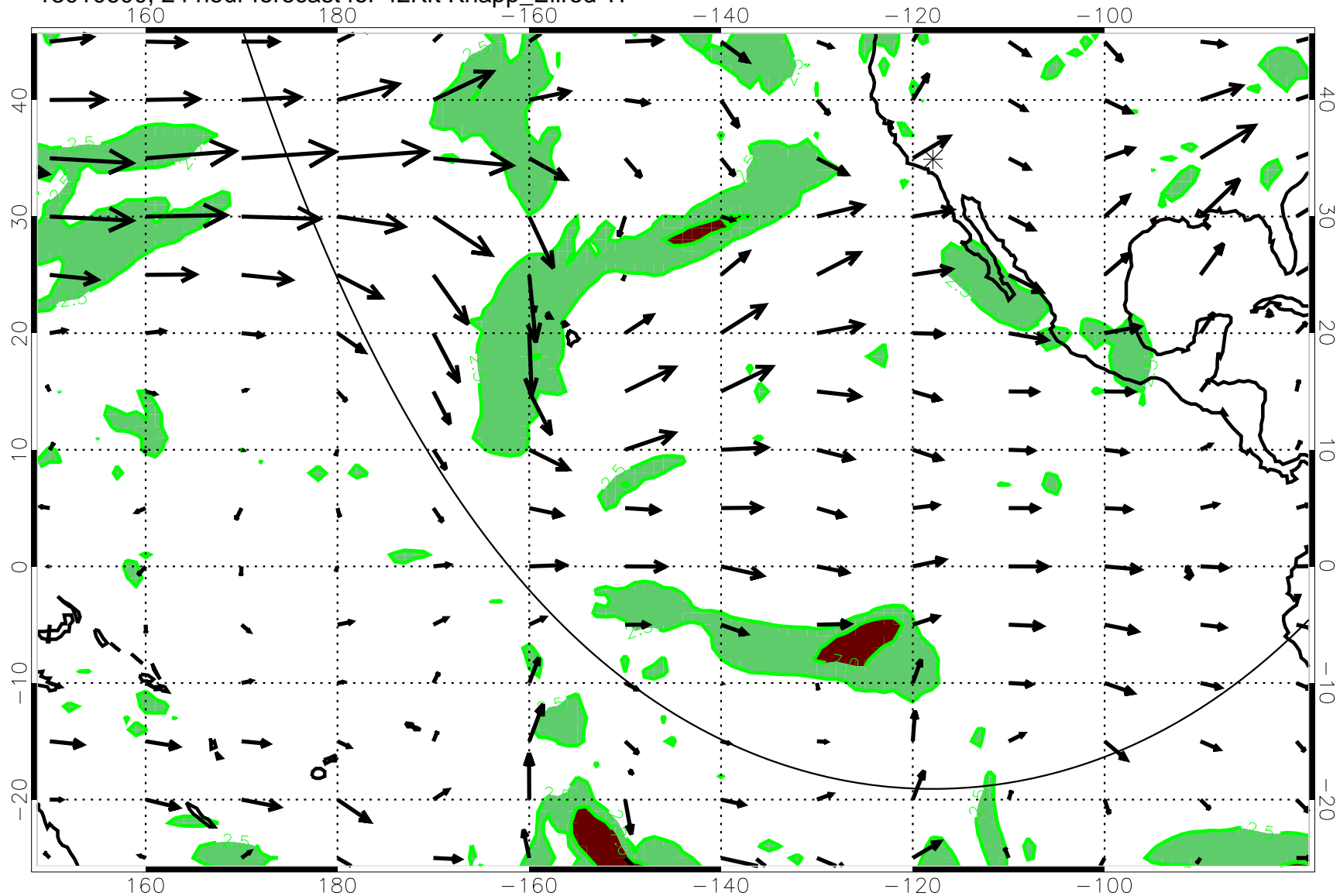
13010600, 24 hour forecast for 42Kft Knapp_Ellrod T1
