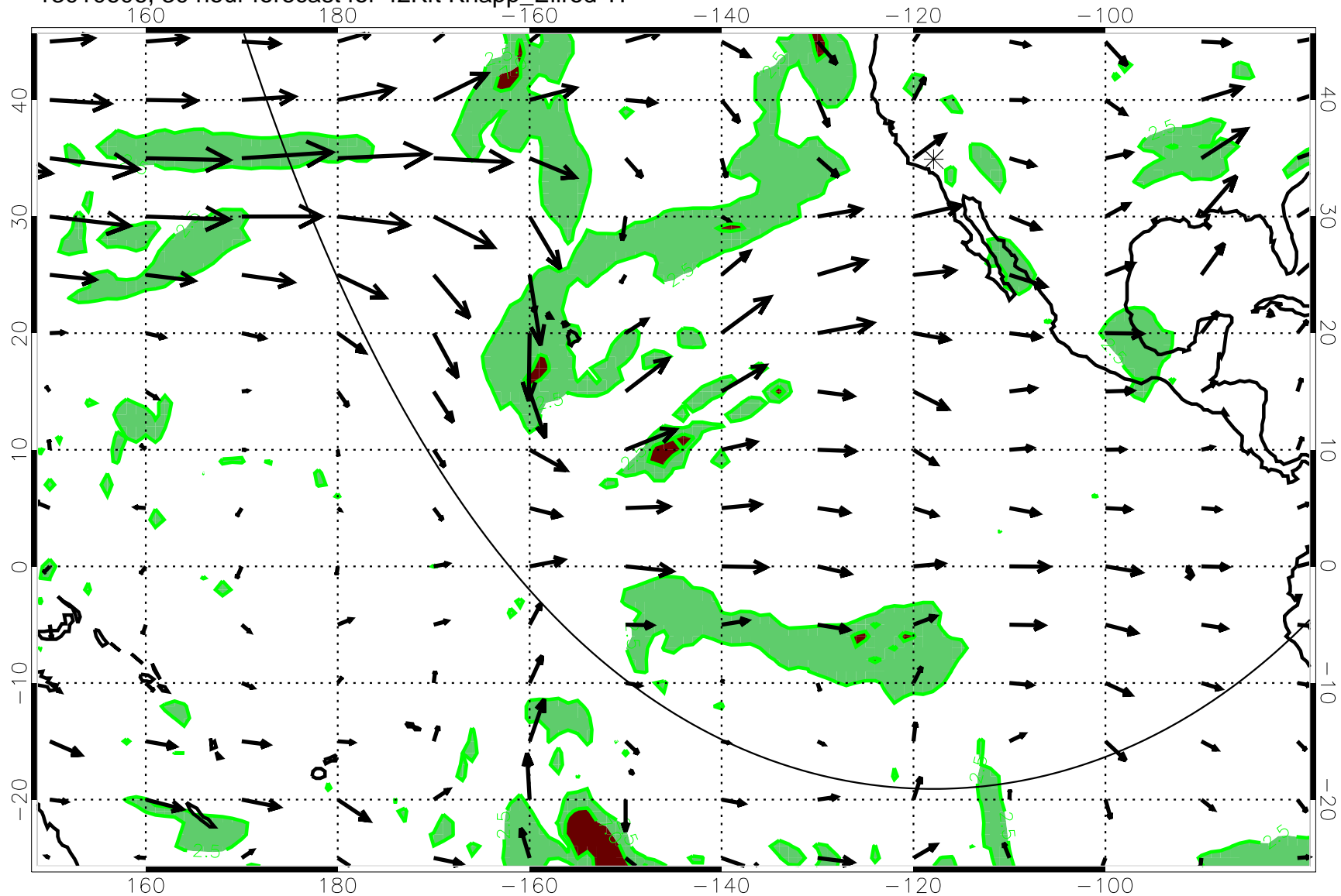
13010606, 30 hour forecast for 42Kft Knapp_Ellrod T1
