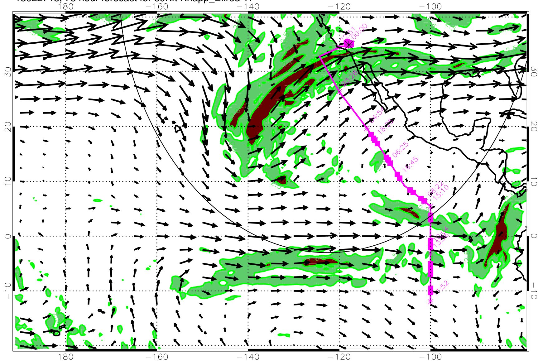
13022718, 78 hour forecast for 39Kft Knapp_Ellrod TI
