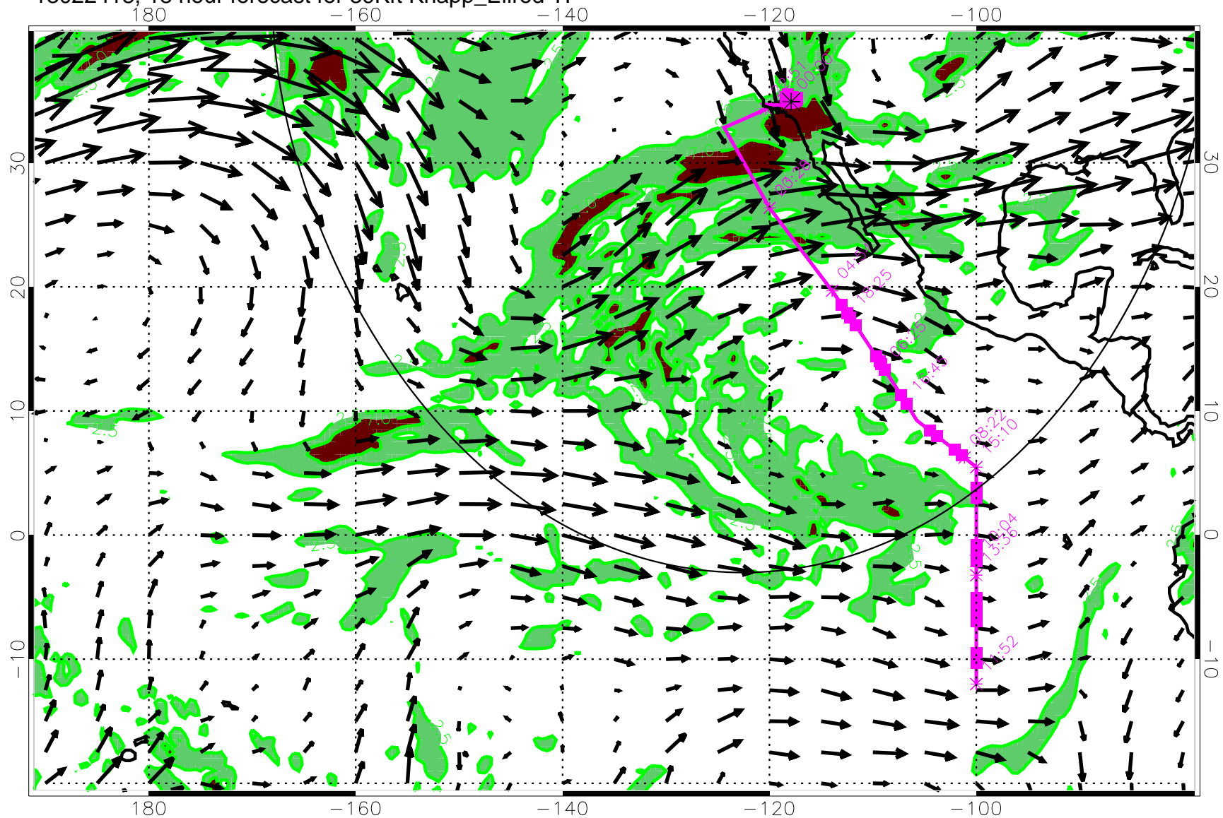
13022418, 18 hour forecast for 39Kft Knapp_Ellrod TI
