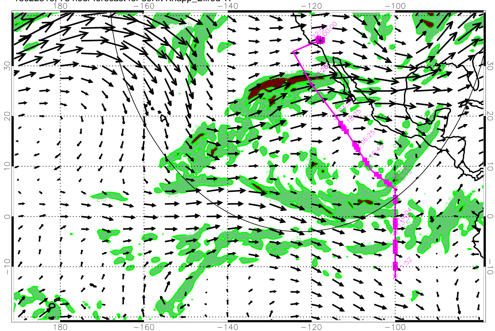
13022518, 78 hour forecast for 39Kft Knapp_Ellrod T1
