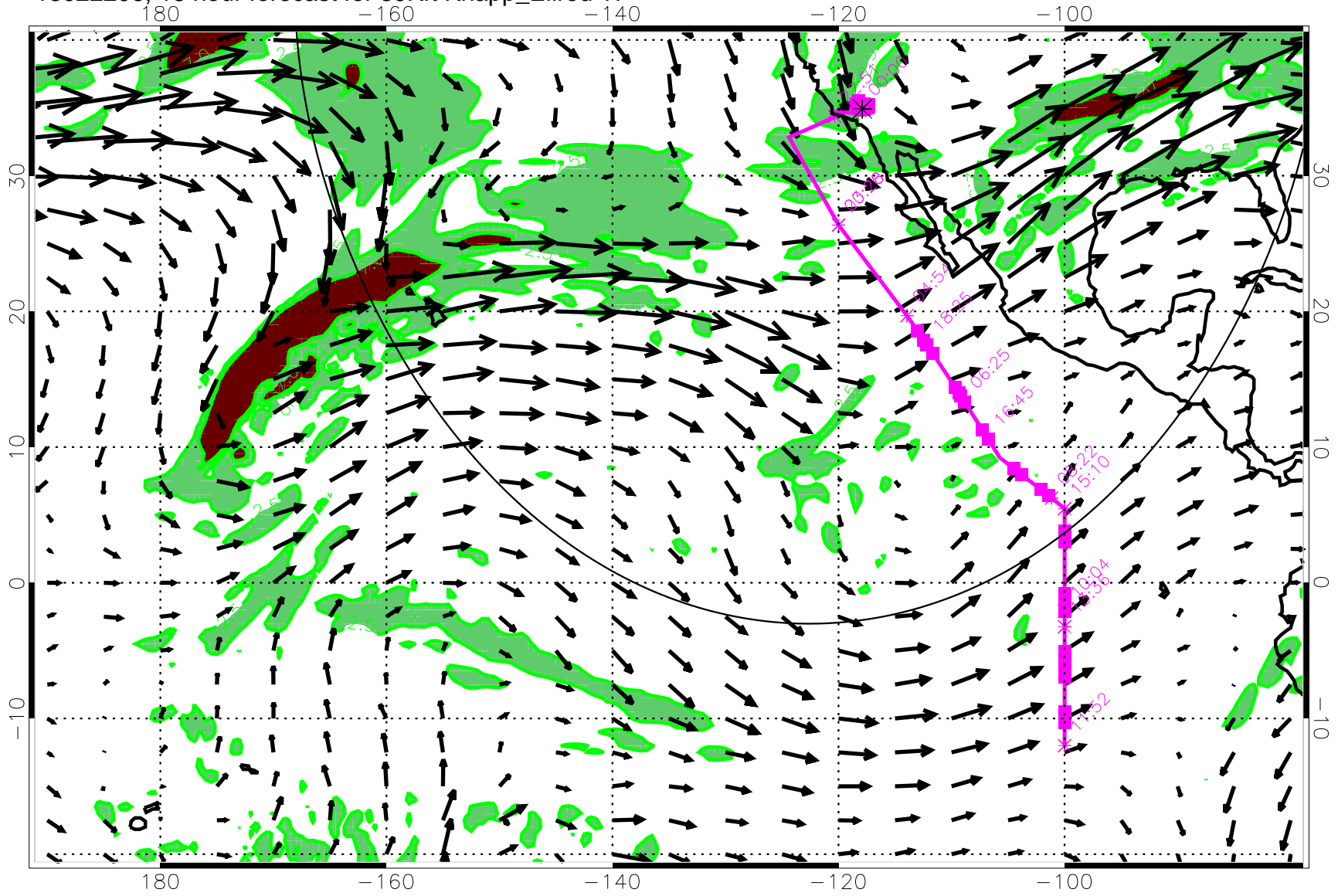
13022206, 18 hour forecast for 39Kft Knapp_Ellrod TI
