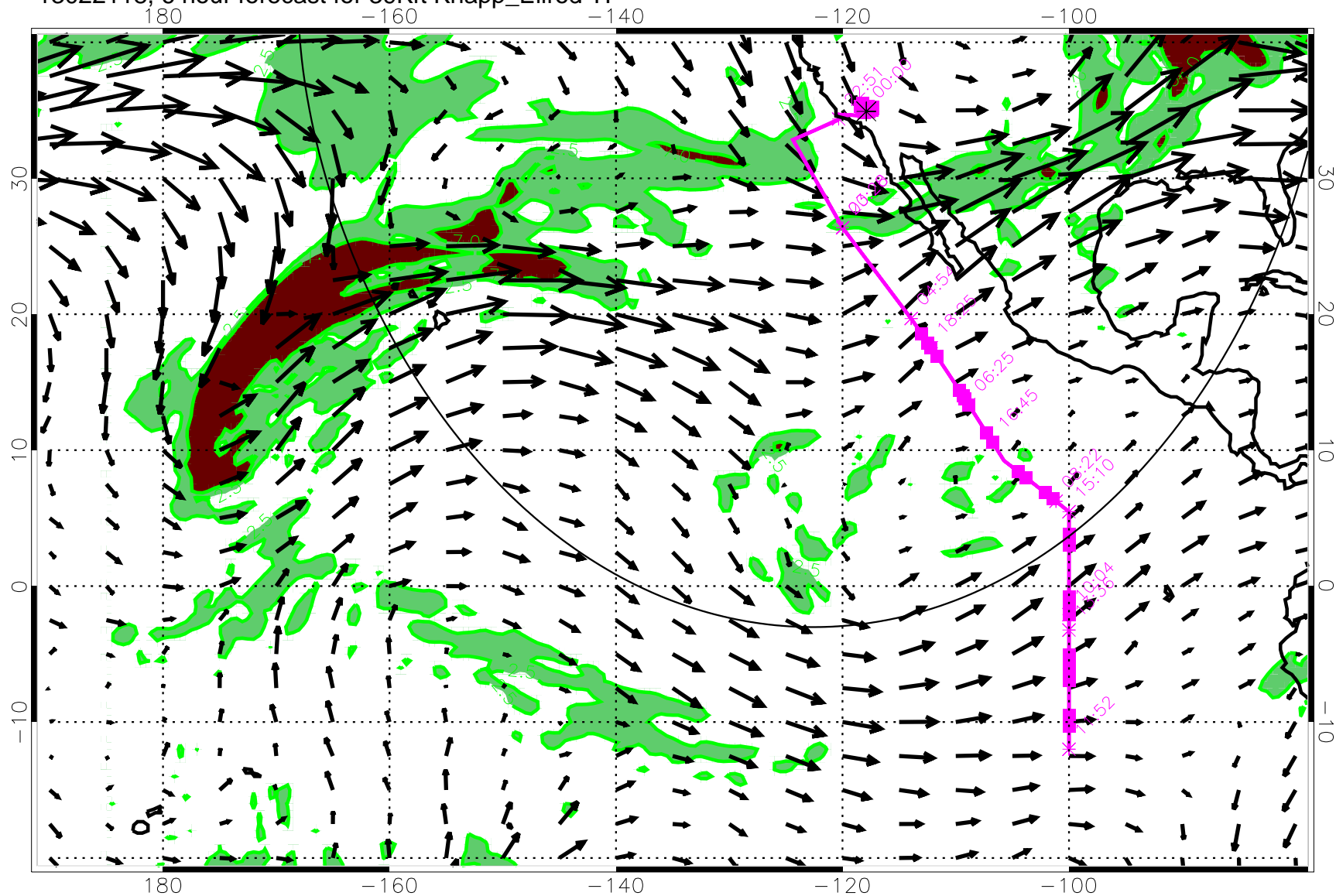
13022118, 6 hour forecast for 39Kft Knapp_Ellrod TI
