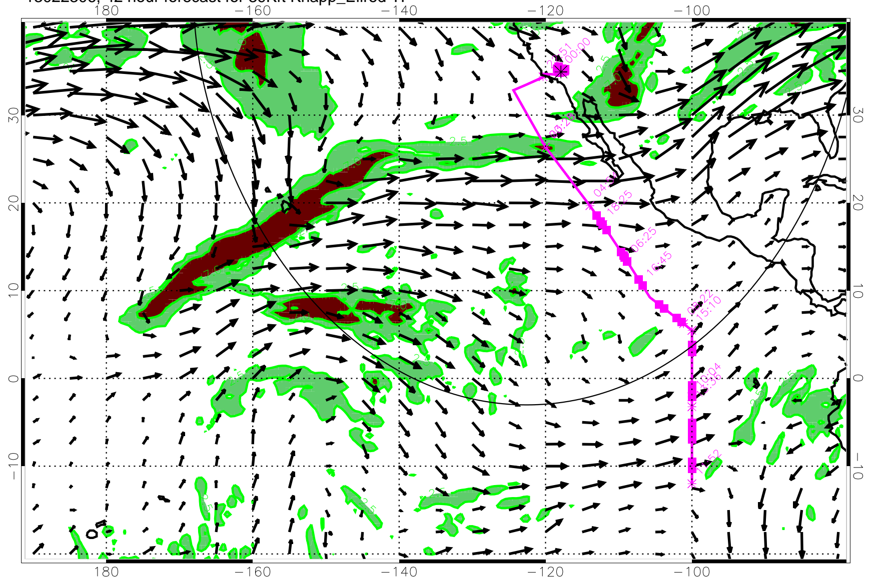
13022306, 42 hour forecast for 39Kft Knapp_Ellrod TI
