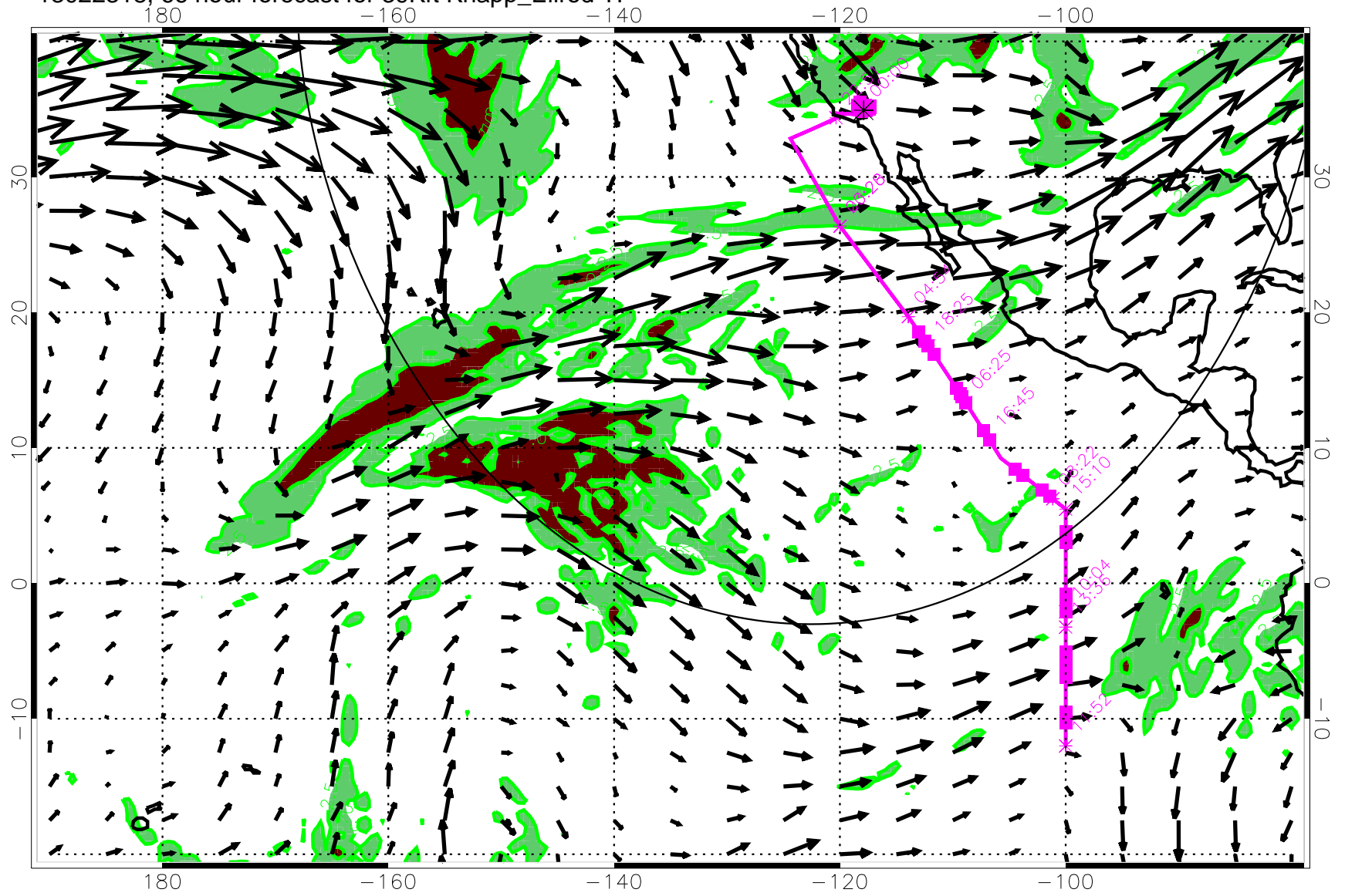
13022318, 66 hour forecast for 39Kft Knapp_Ellrod TI
