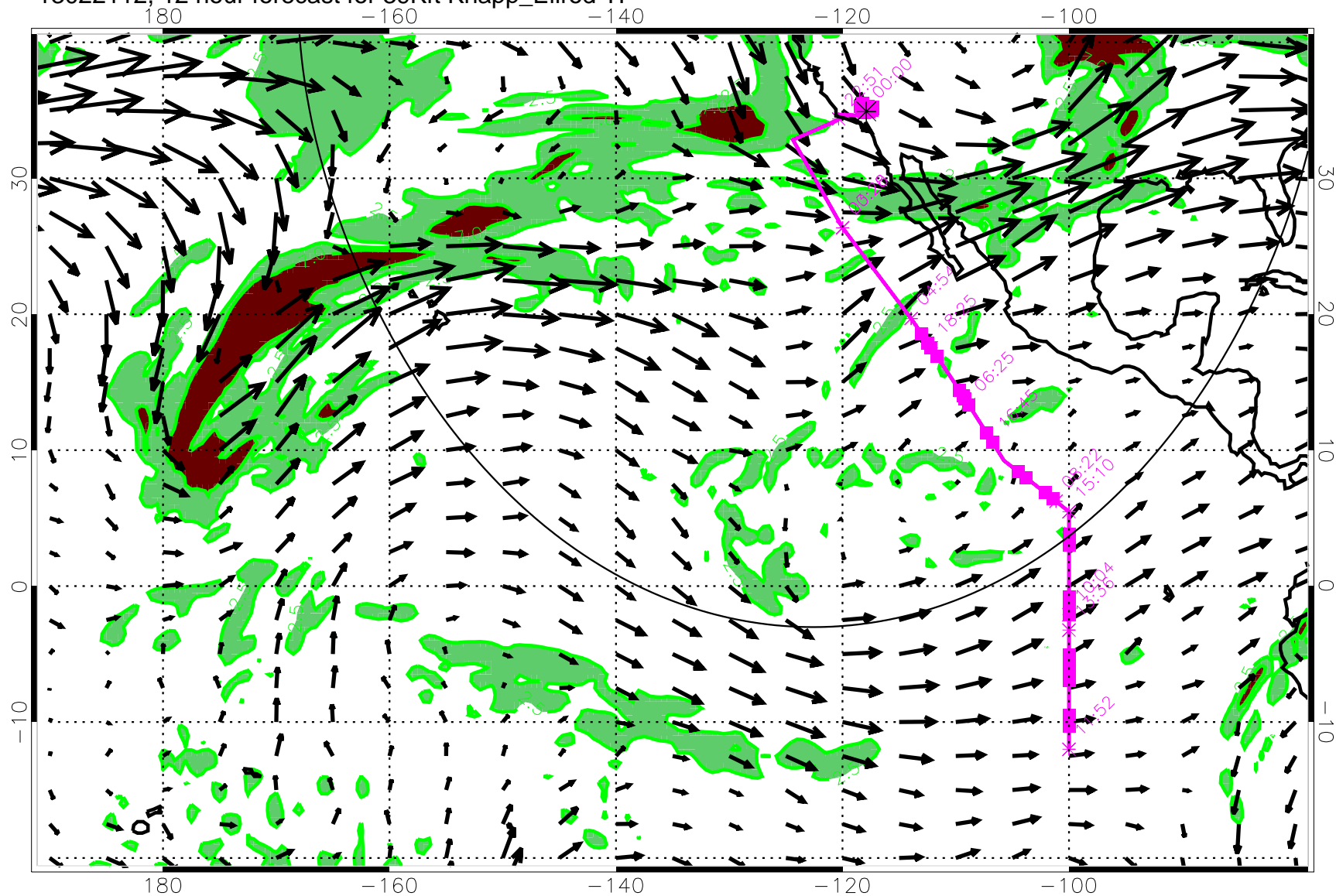
13022112, 12 hour forecast for 39Kft Knapp_Ellrod TI
