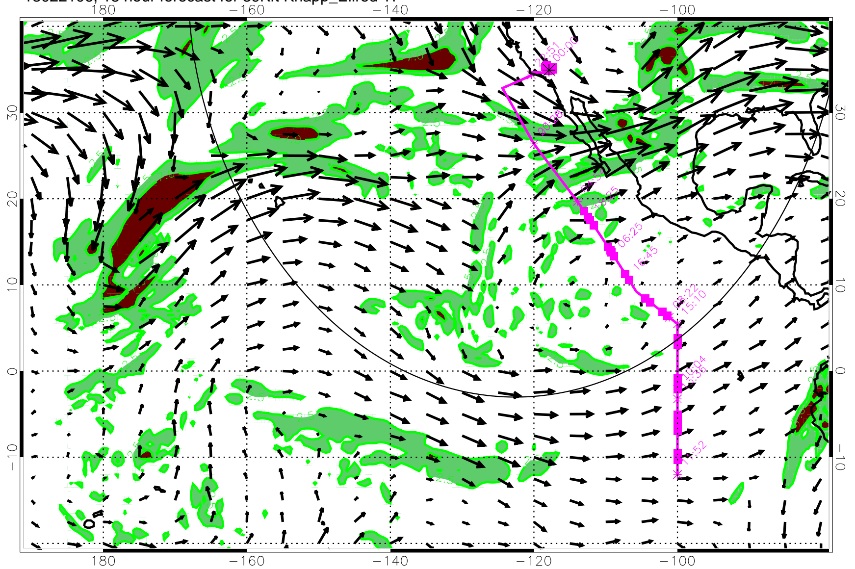
13022106, 18 hour forecast for 39Kft Knapp_Ellrod T1
