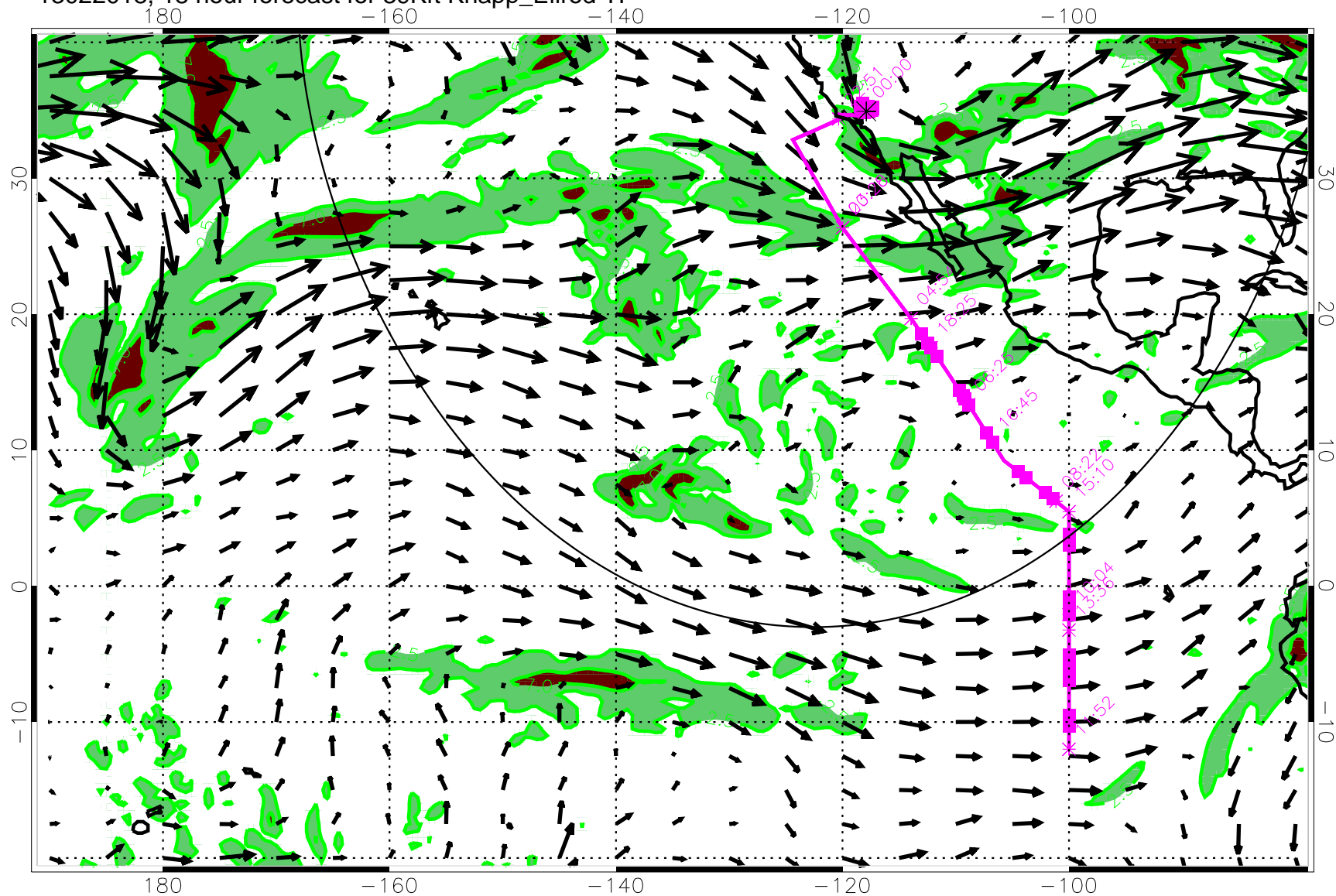
13022018, 18 hour forecast for 39Kft Knapp_Ellrod TI
