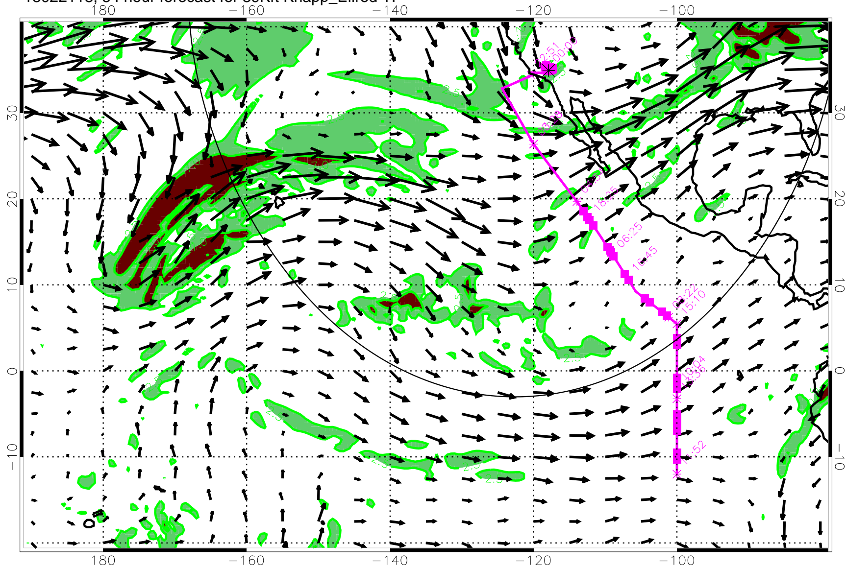
13022118, 54 hour forecast for 39Kft Knapp_Ellrod TI
