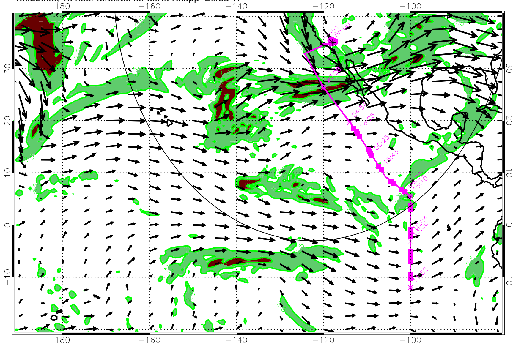
13022006, 18 hour forecast for 39Kft Knapp_Ellrod TI
