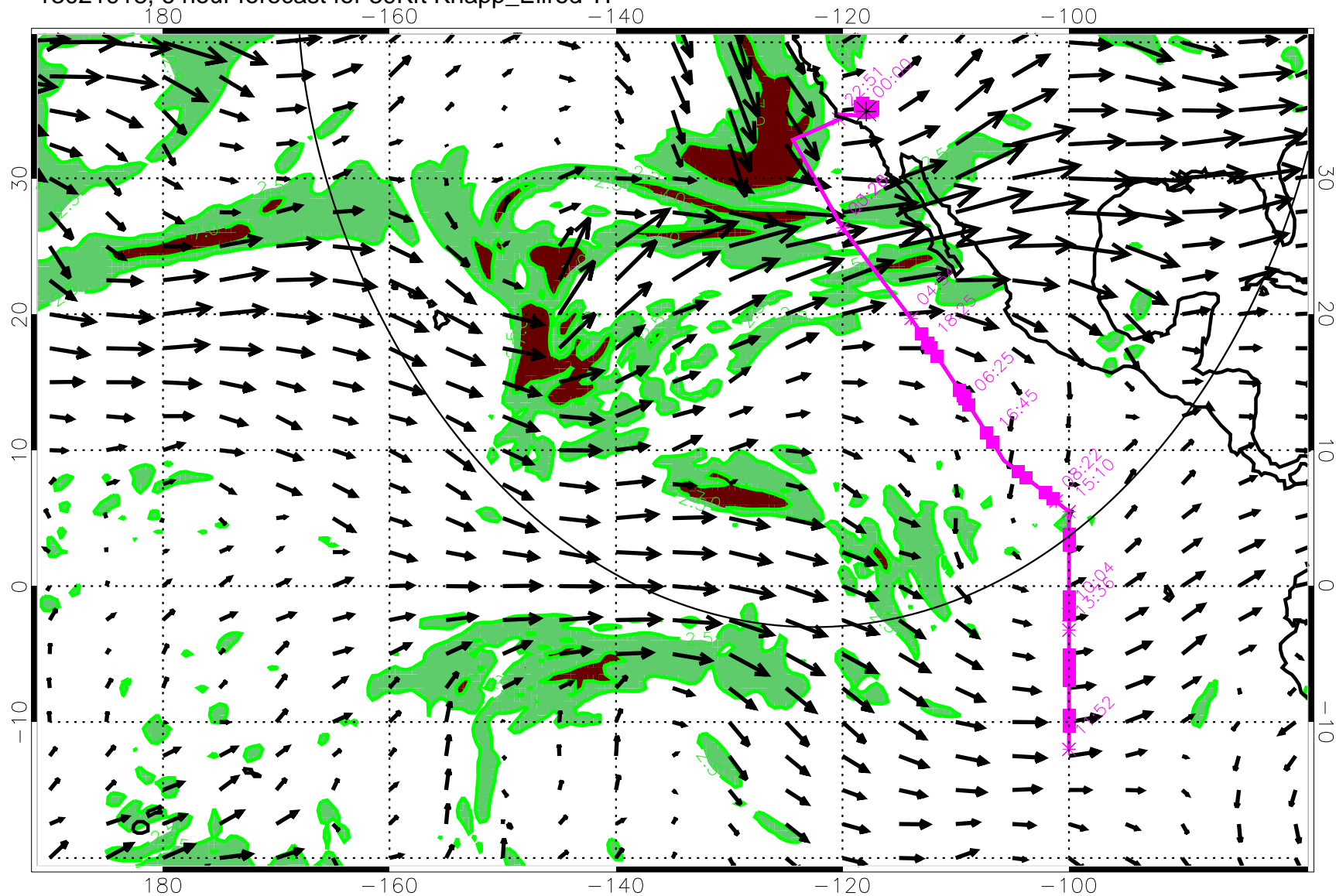
13021918, 6 hour forecast for 39Kft Knapp_Ellrod TI
